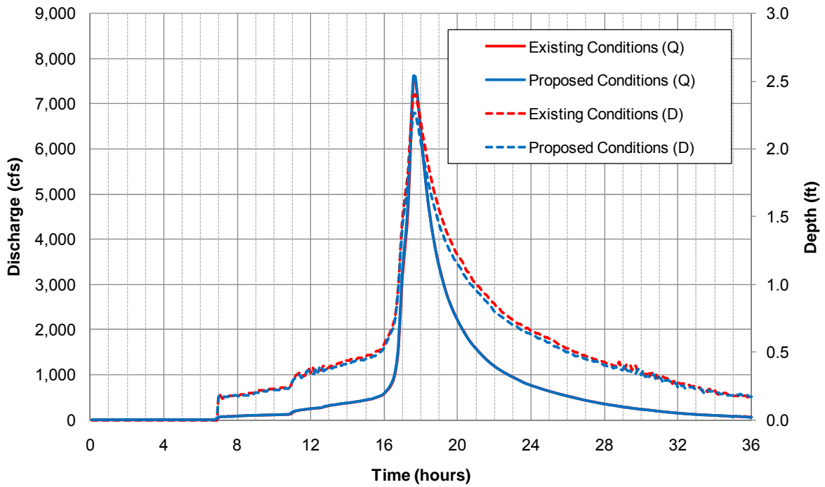
24-hour 100-year Hydrograph at a Cross Section on Main Access Road
