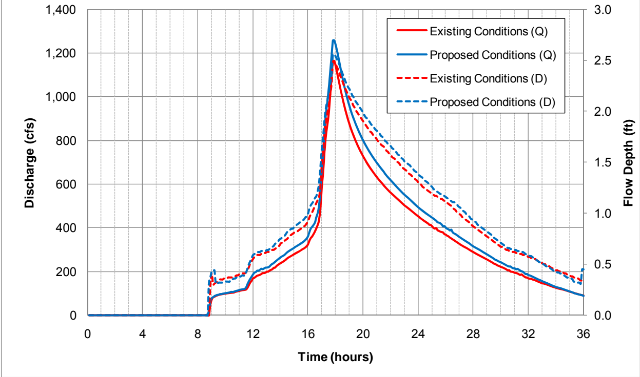
24-hour 100-year Hydrograph at Trestle 2
