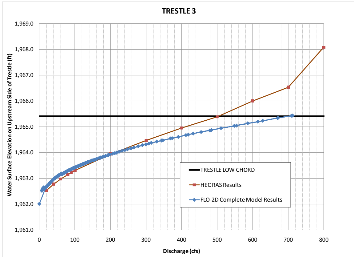
Figure 3.4a. Water-surface elevation versus discharge rating curves from the local HEC-RAS model and the FLO-2D model for Trestle 3.
