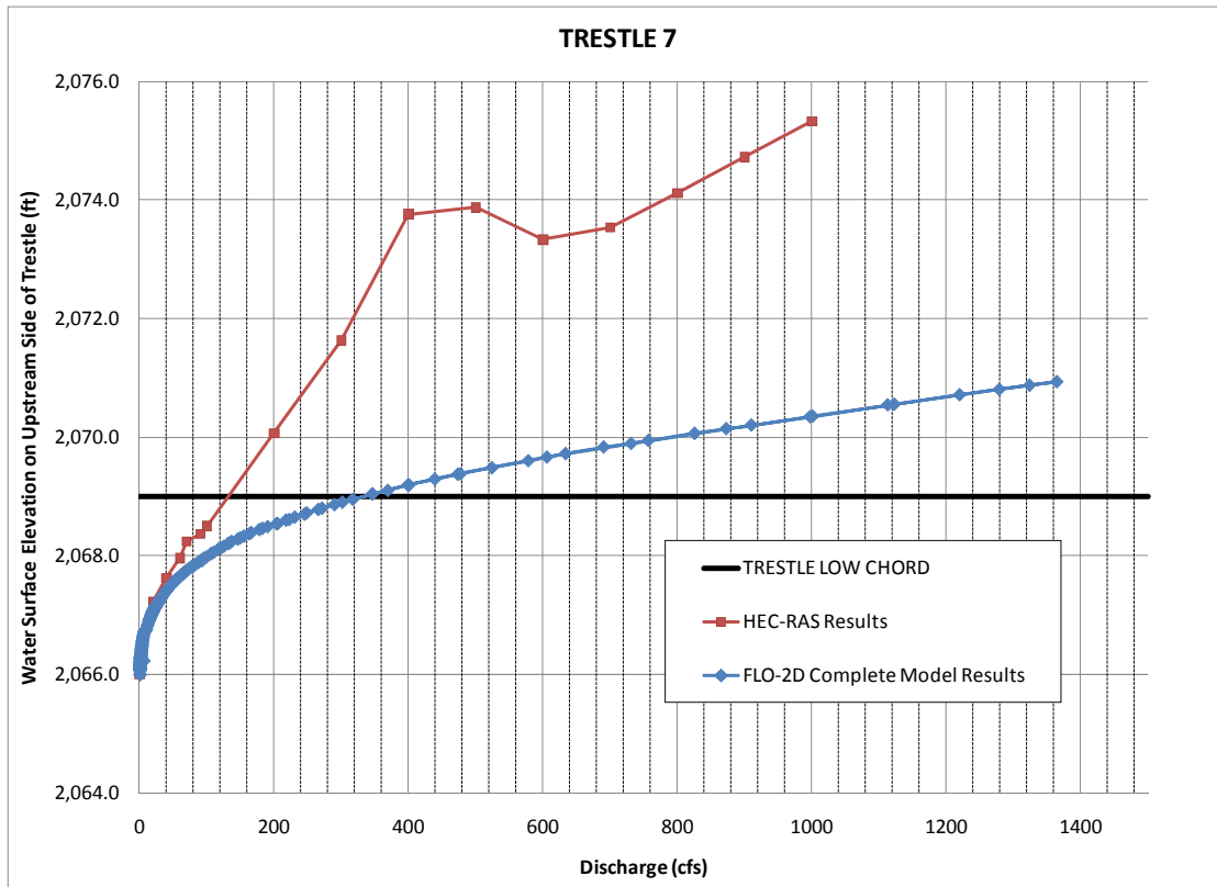
Figure 3.5a. Water-surface elevation versus discharge rating curves from the local HEC-RAS model and the FLO-2D model for Trestle 7.
