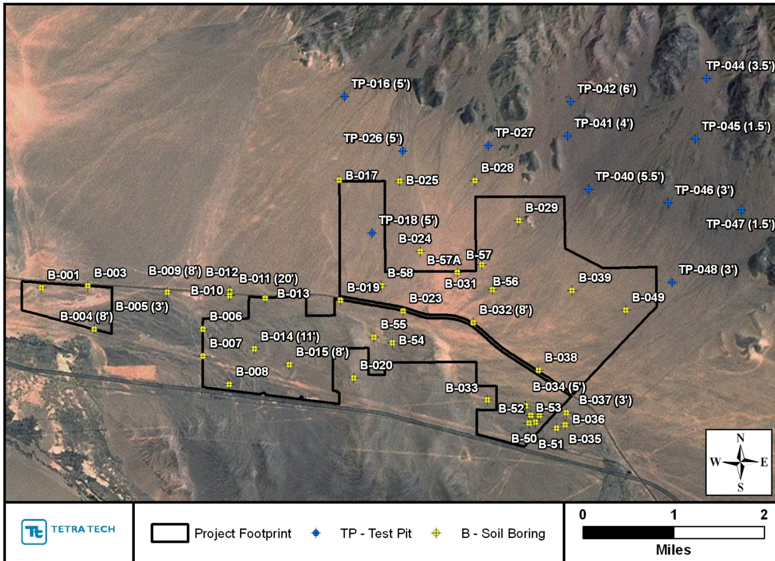
Figure 2.8. Location of soil borings and test pits reported by Terracon (2011) (Most of the borings and test pits were completed in 2009.) Parenthetical numbers after some of the labels indicate approximate depth below existing ground surface to the upper-most calcium carbonate deposits. Calcium carbonate deposits not encountered at sites with no parenthetical number after the label.
