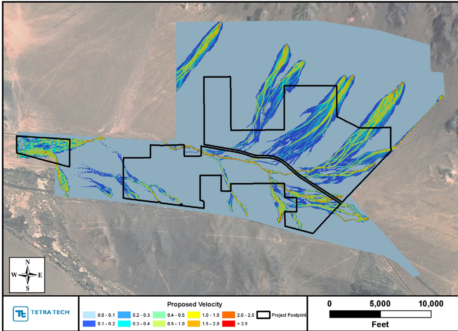
Maximum velocity during the 5-year, 24-hour storm.
