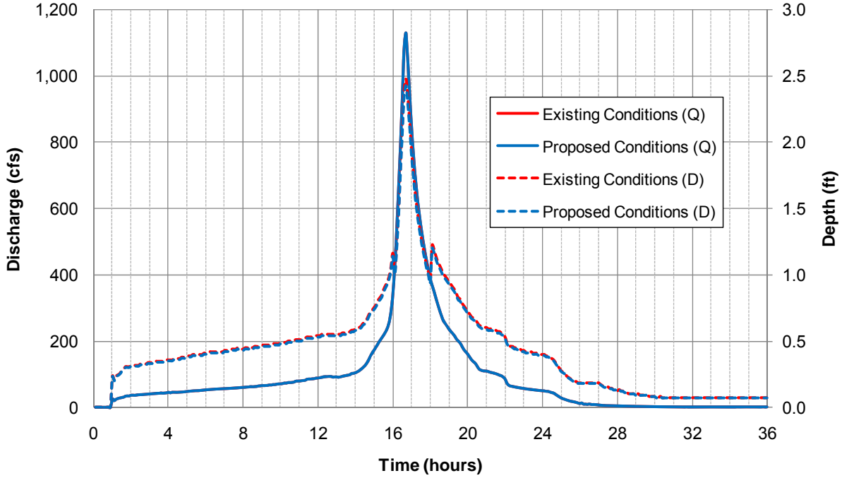
24-hour 100-year Hydrograph at Trestle 8
