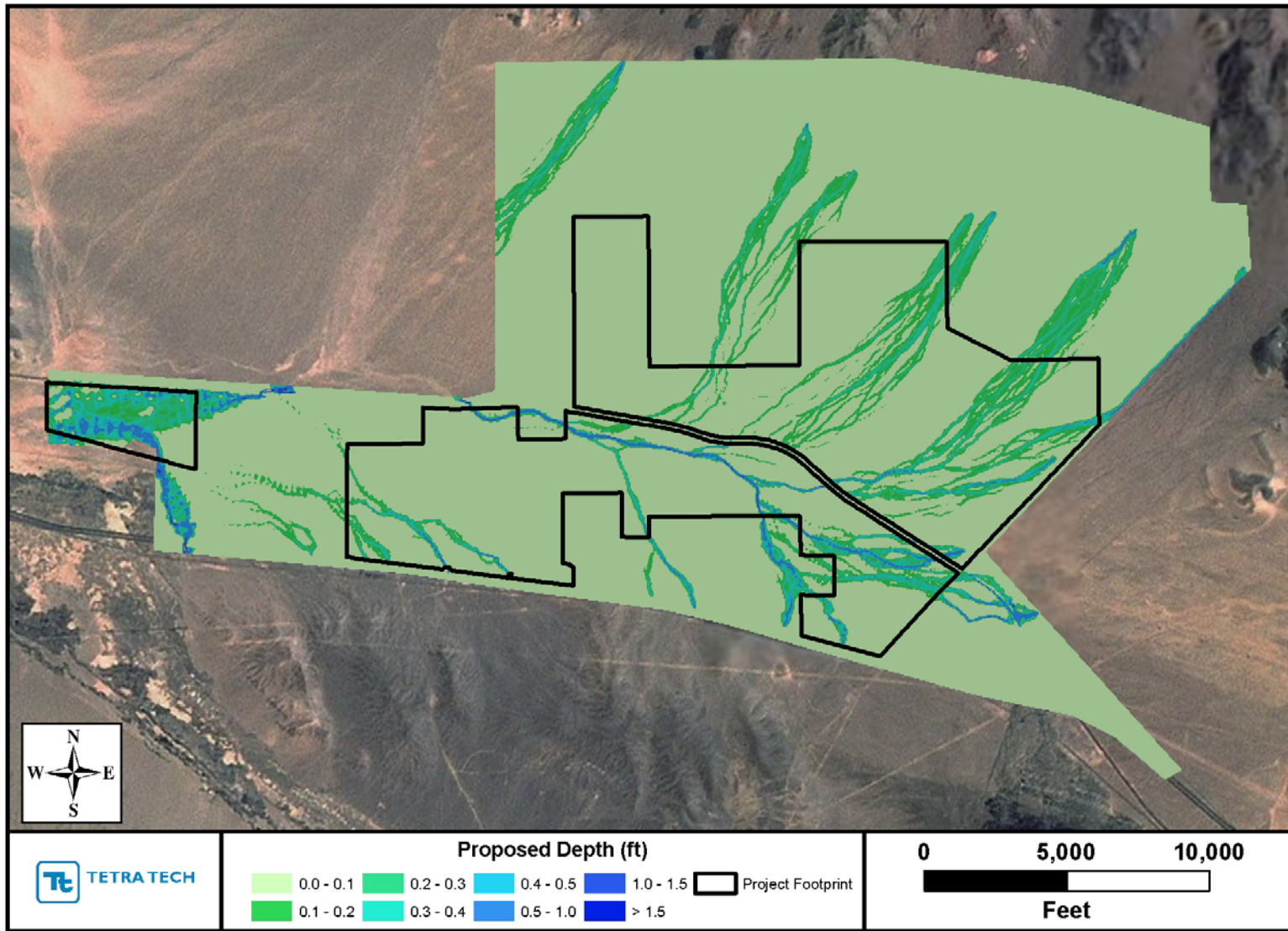
Maximum depths during the 5-year, 24-hour storm.
