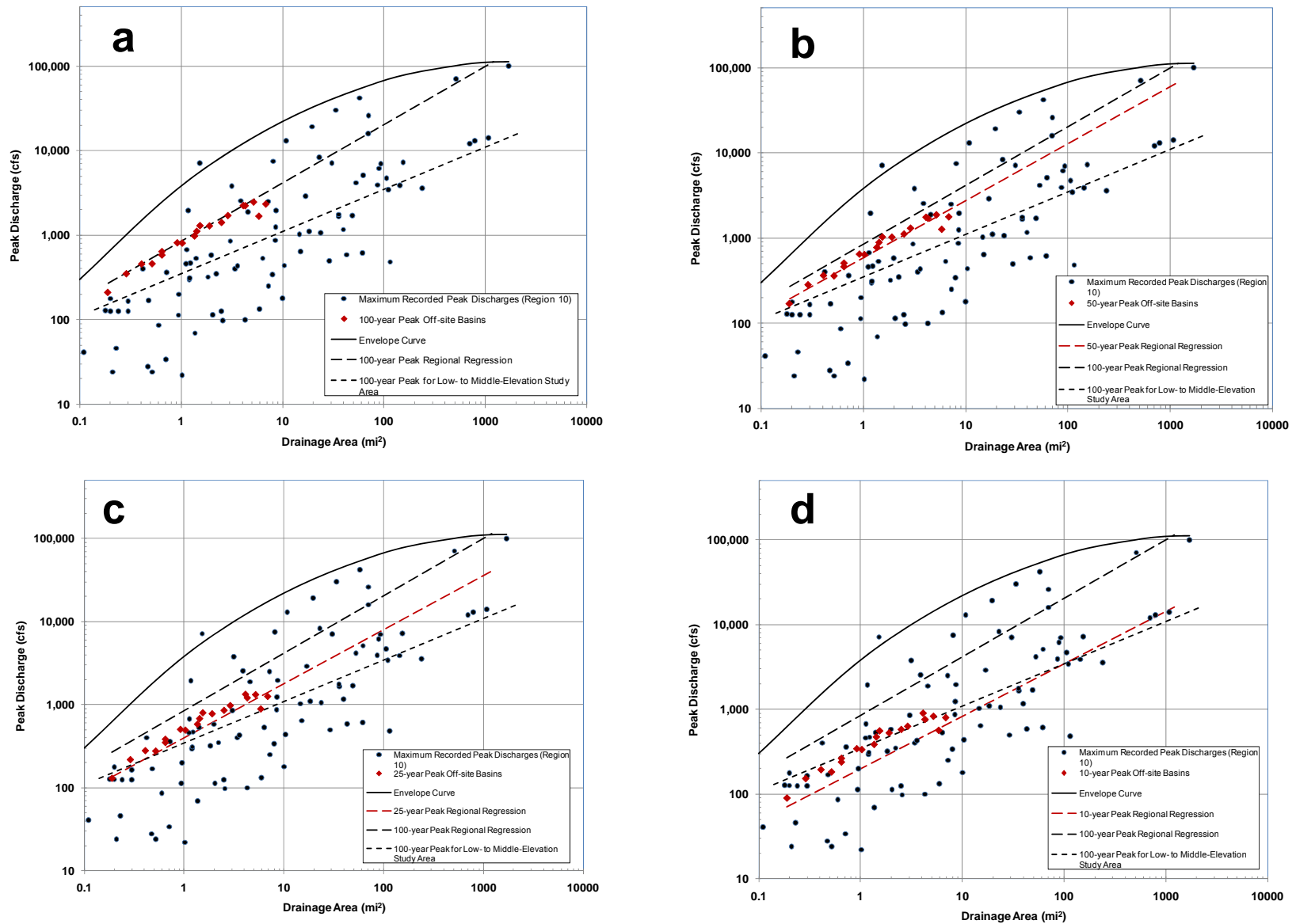
Figure 2.13. Comparison of regional regression equations and underlying data for Region 10 from Blakemore et al. (1997) with modeled peak discharges for the offsite basins at the project site. Maximum recorded peak discharges and regression curves reproduced from Figure 37 and the data appendix from Blakemore et al. (1997): (a) 100-year, (b) 50-year, (c) 25-year, (d) 10-year, (e) 5-year, and (f) 2-year.
