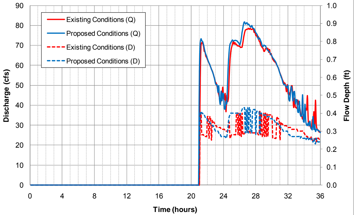
24-hour 5-year Hydrograph at Trestle 2
