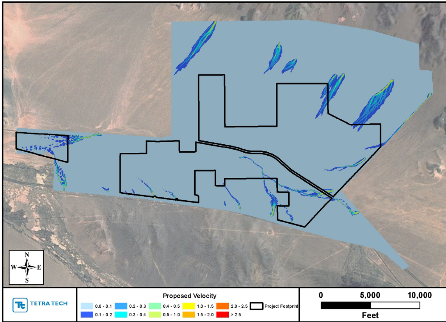
Maximum velocity during the 2-year, 24-hour storm.
