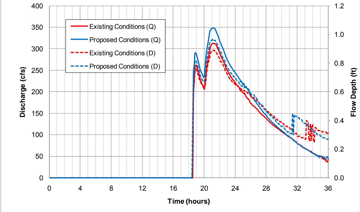
24-hour 10-year Hydrograph at Trestle 2
