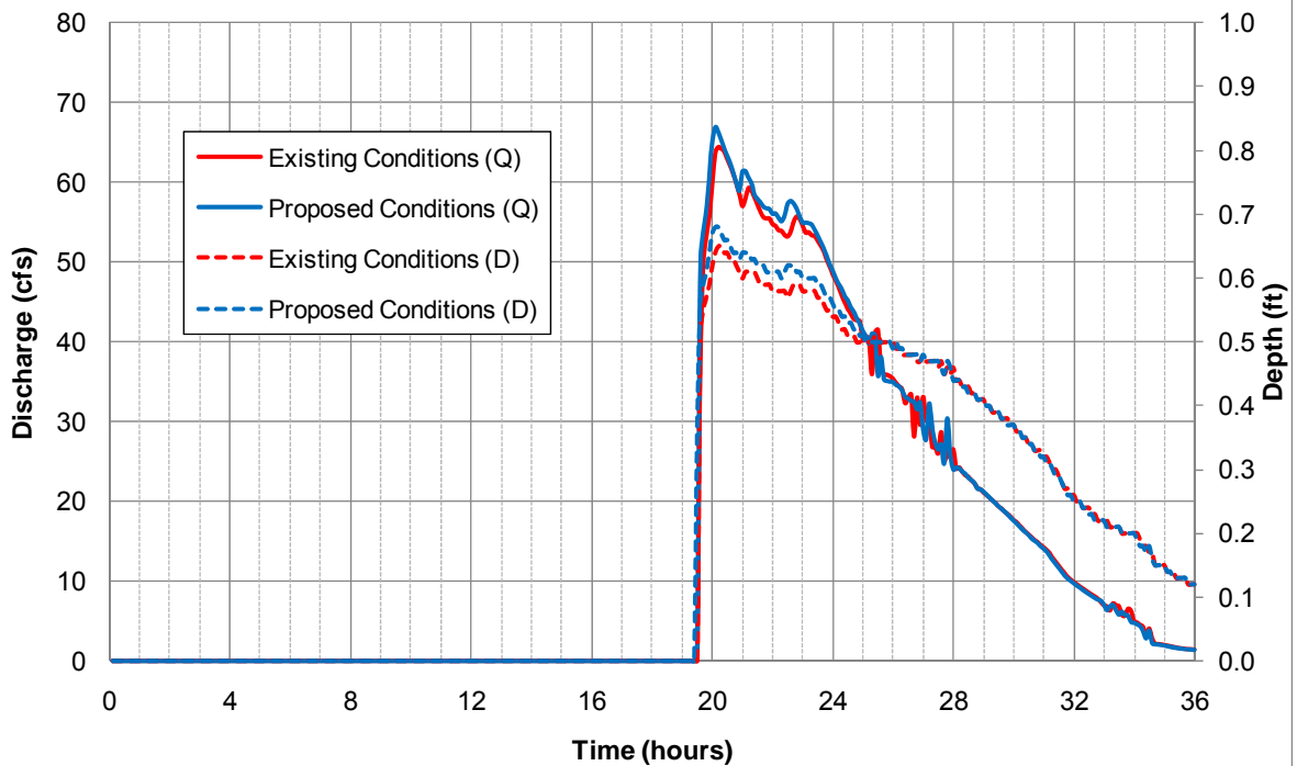
24-hour 10-year Hydrograph at Trestle 4
