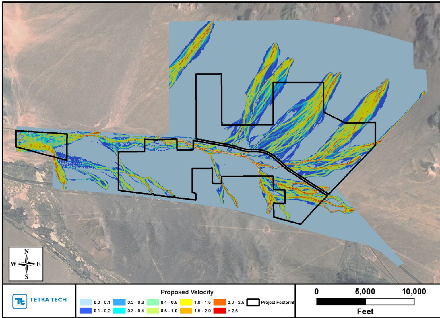
Maximum velocity during the 10-year, 24-hour storm.
