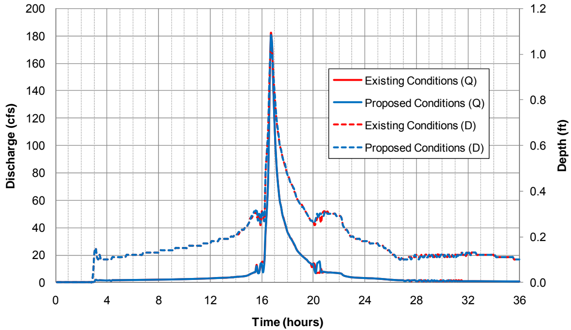
24-hour 5-year Hydrograph at Trestle 8
