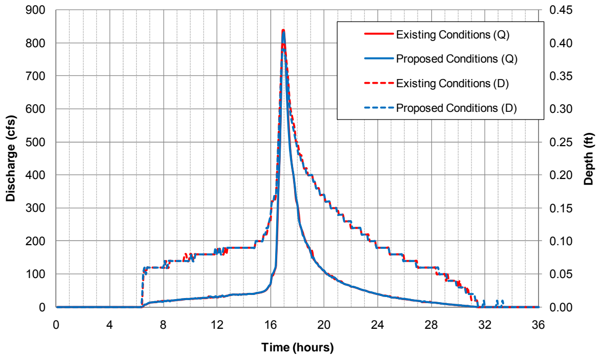
24-hour 100-year Hydrograph at a Cross Section North of Railroad
