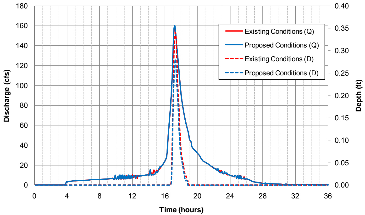
24-hour 5-year Hydrograph at Trestle 1
