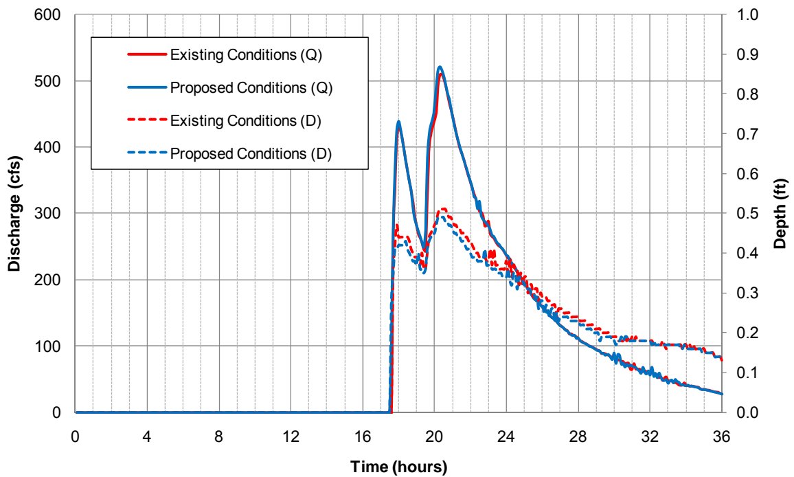
24-hour 10-year Hydrograph at a Cross Section on Main Access Road
