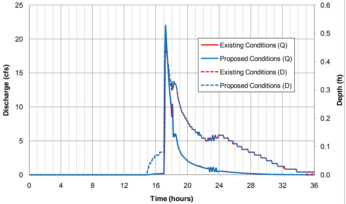
24-hour 5-year Hydrograph at Trestle 7
