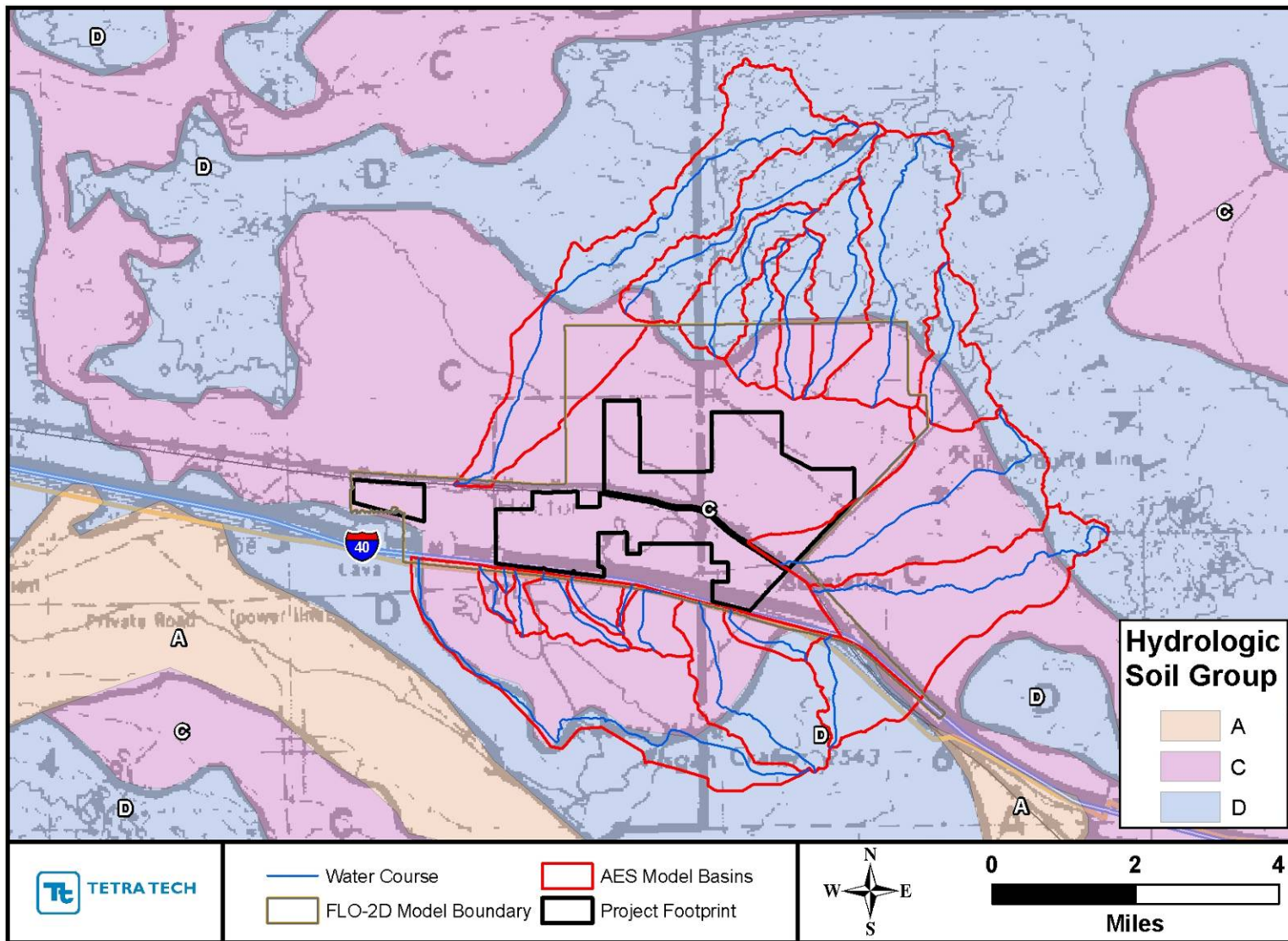
Figure 2.5. Hydrologic soil groups in the vicinity of the project, digitized from SBC (1986), Figure C-11.
