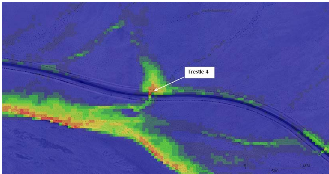
FLO-2D Results for the 100-year storm - Water ponds before flowing through trestle leading to lower WSELs than in the HEC-RAS model
