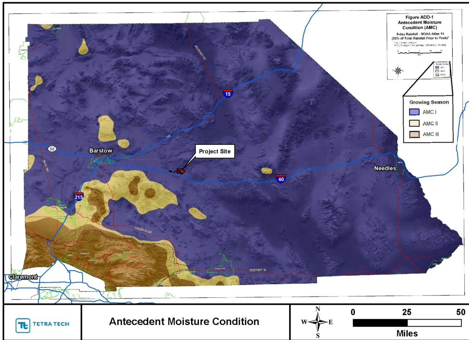
Figure 2.11. Figure ADD-1 from SBC (2010) showing the location of the project site in the portion of San Bernardino County where an AMC I condition can be used in rainfall-runoff modeling.
