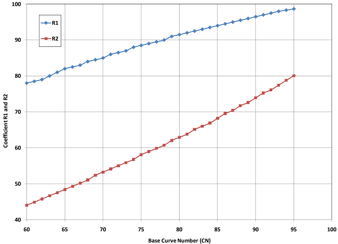
Figure 2.12. Coefficients R_1 and R_2 for use in determining CN^* based on total storm depth.
