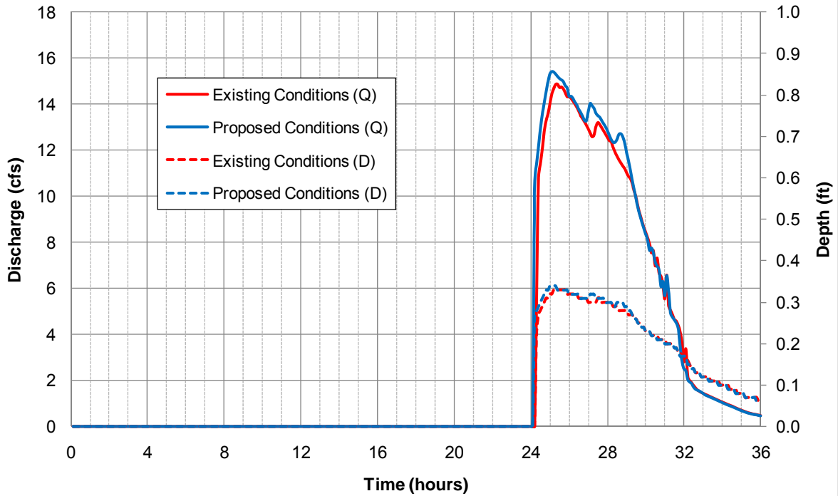
24-hour 5-year Hydrograph at Trestle 4
