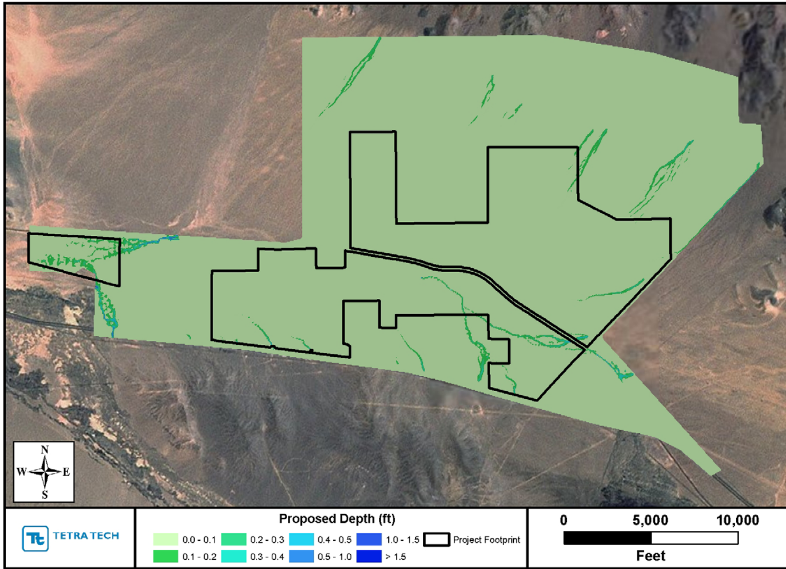
Maximum depths during the 2-year, 24-hour storm.
