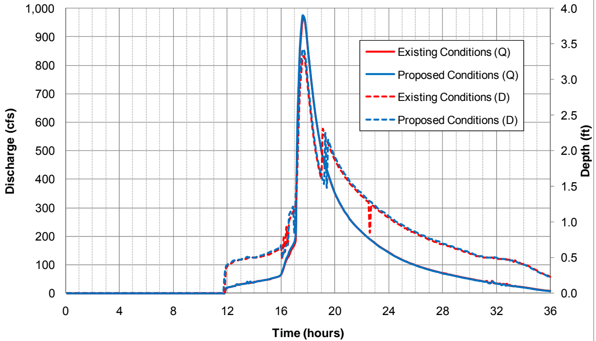
24-hour 100-year Hydrograph at Trestle 4
