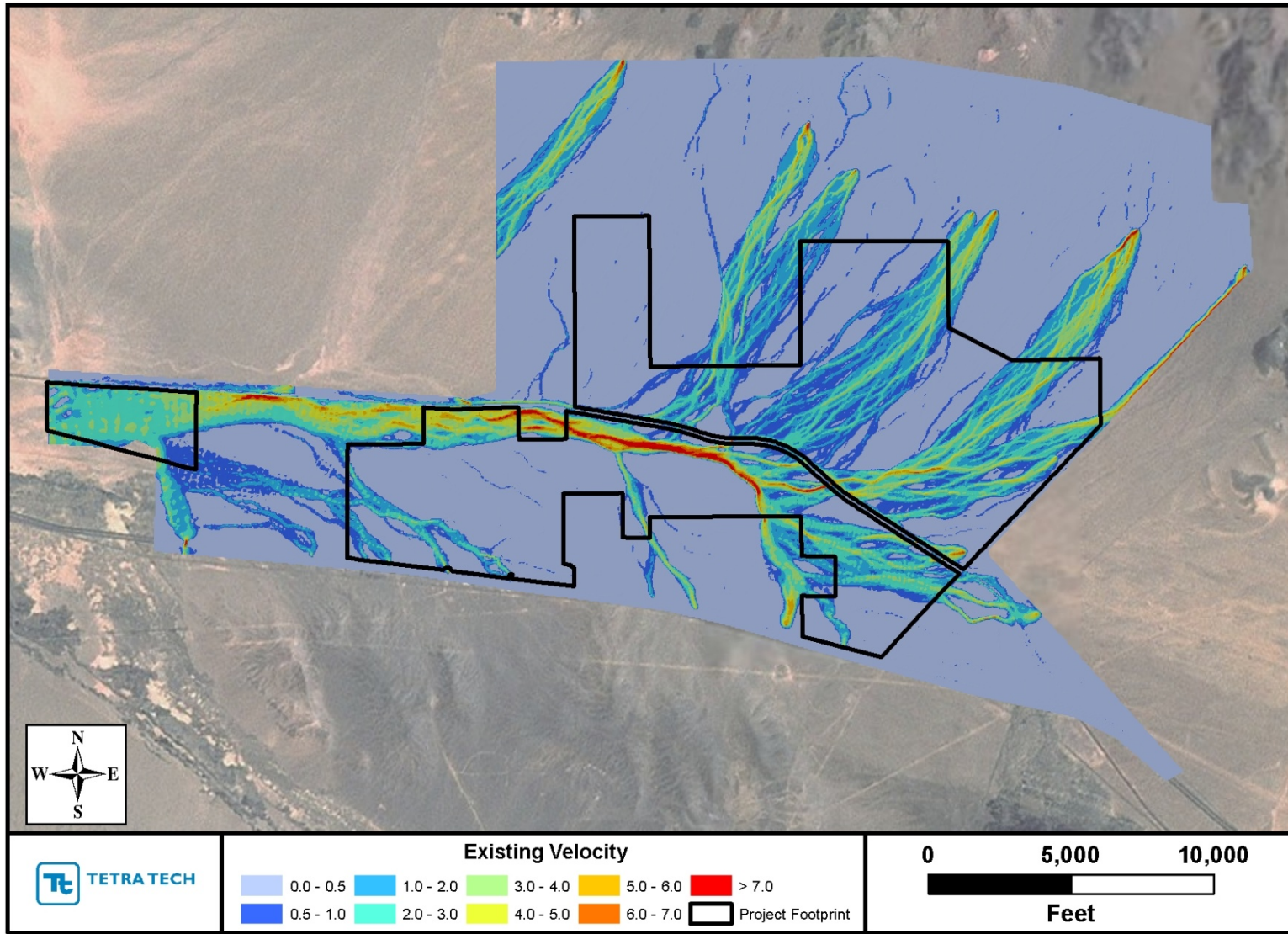
Figure 3.8b. Predicted maximum velocity during 100-year, 24-hour storm under existing conditions.
