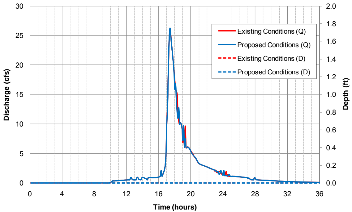
24-hour 2-year Hydrograph at Trestle 1
