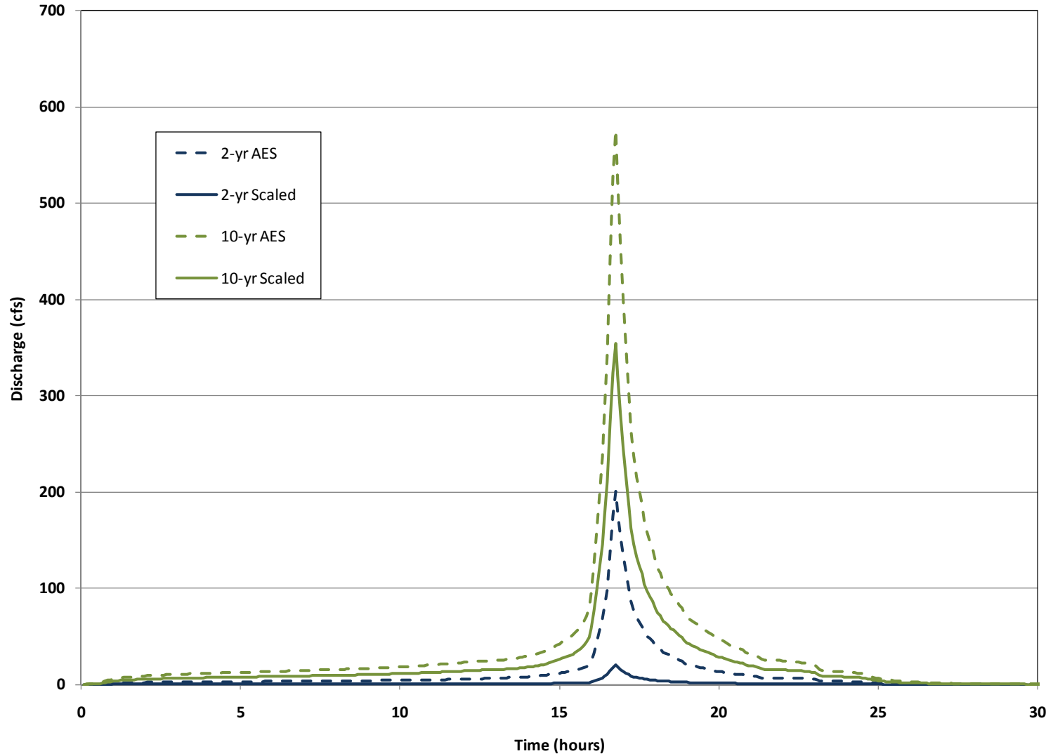
Figure 2.14. Typical modeled and scaled hydrographs for the 2- and 10-year storms (Basin 11).
