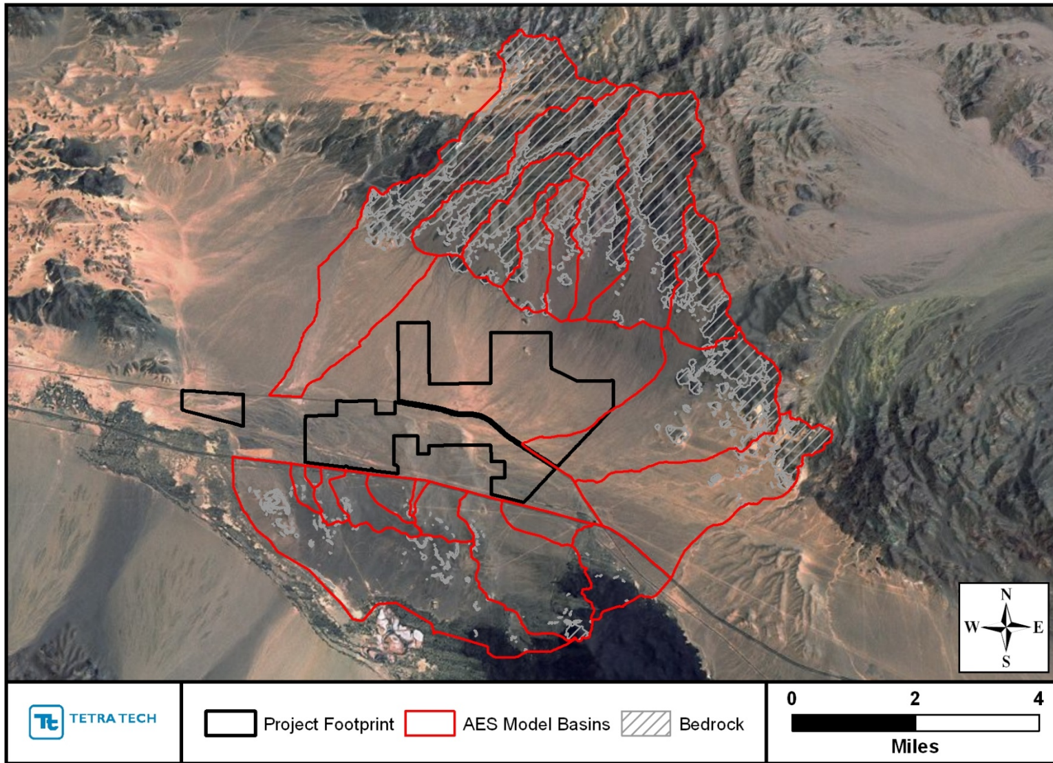
Figure 2.9. Aerial photograph (June 14, 2009) of watershed showing the bedrock and alluvial surfaces.
