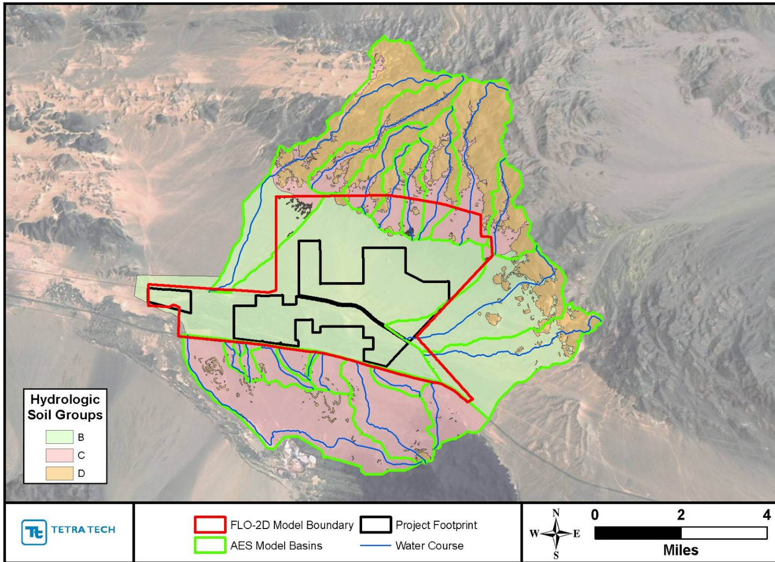
Figure 2.10. Boundaries of soil types used for the AES rainfall-runoff and FLO-2D modeling.
