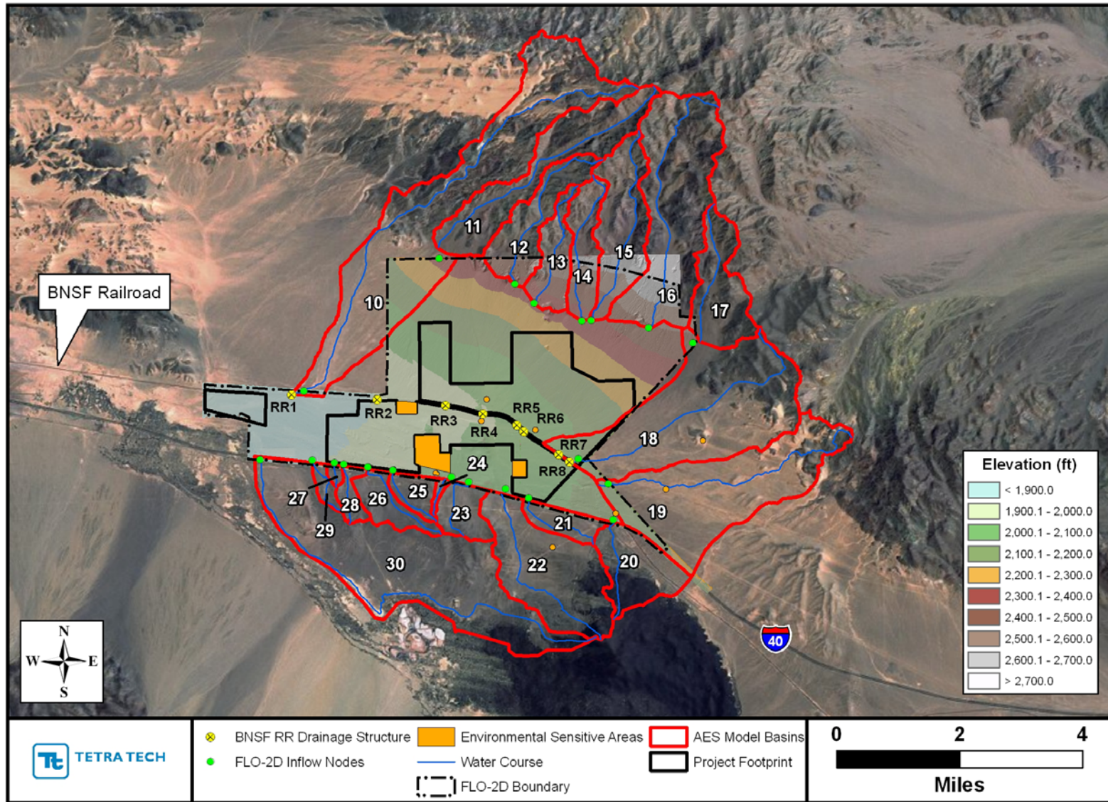
Figure 3.1. Map of project site and contributing drainage subbasins showing the locations of the FLO-2D inflow nodes for the off-site basins and the BNSF Railroad crossings.
