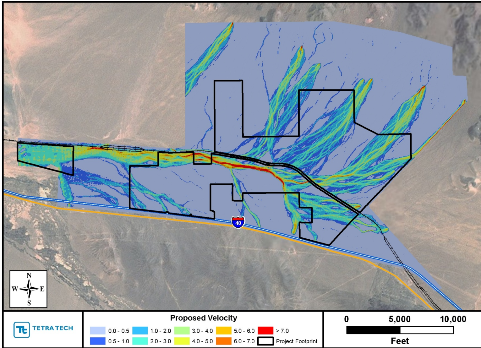
Figure 3.21b. Predicted maximum velocity during 100-year, 24-hour storm under full build-out conditions.
