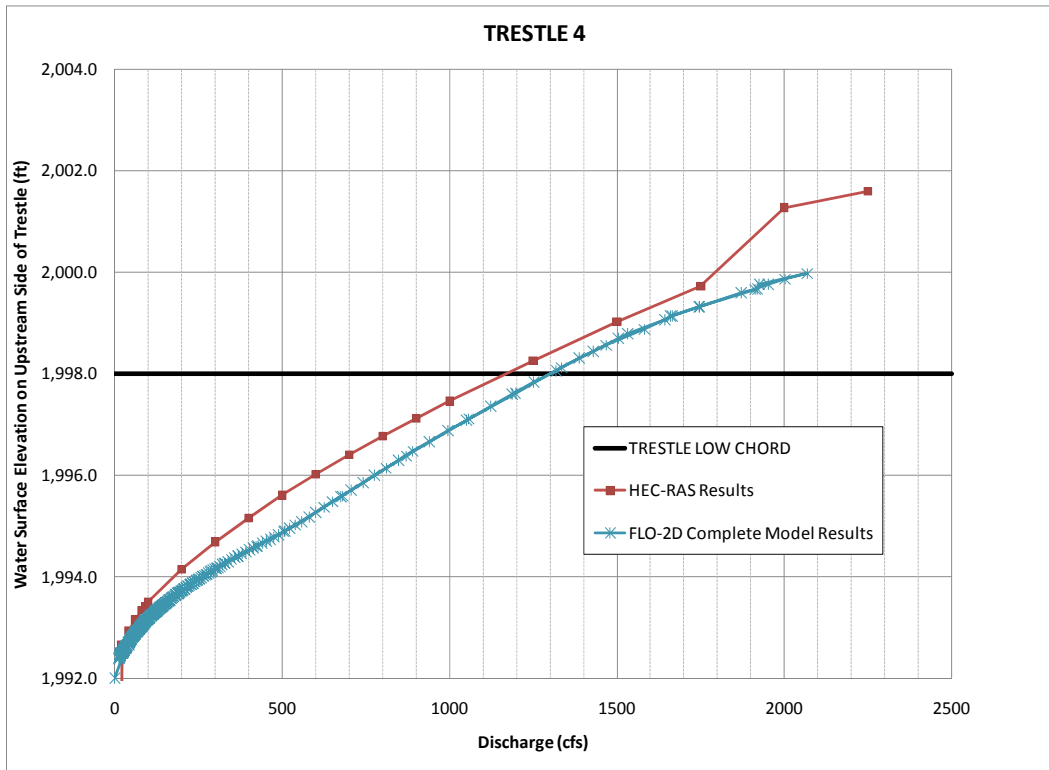
FLO-2D Results for the 100-year storm - Water ponds before flowing through trestle leading to lower WSELs than in the HEC-RAS model
