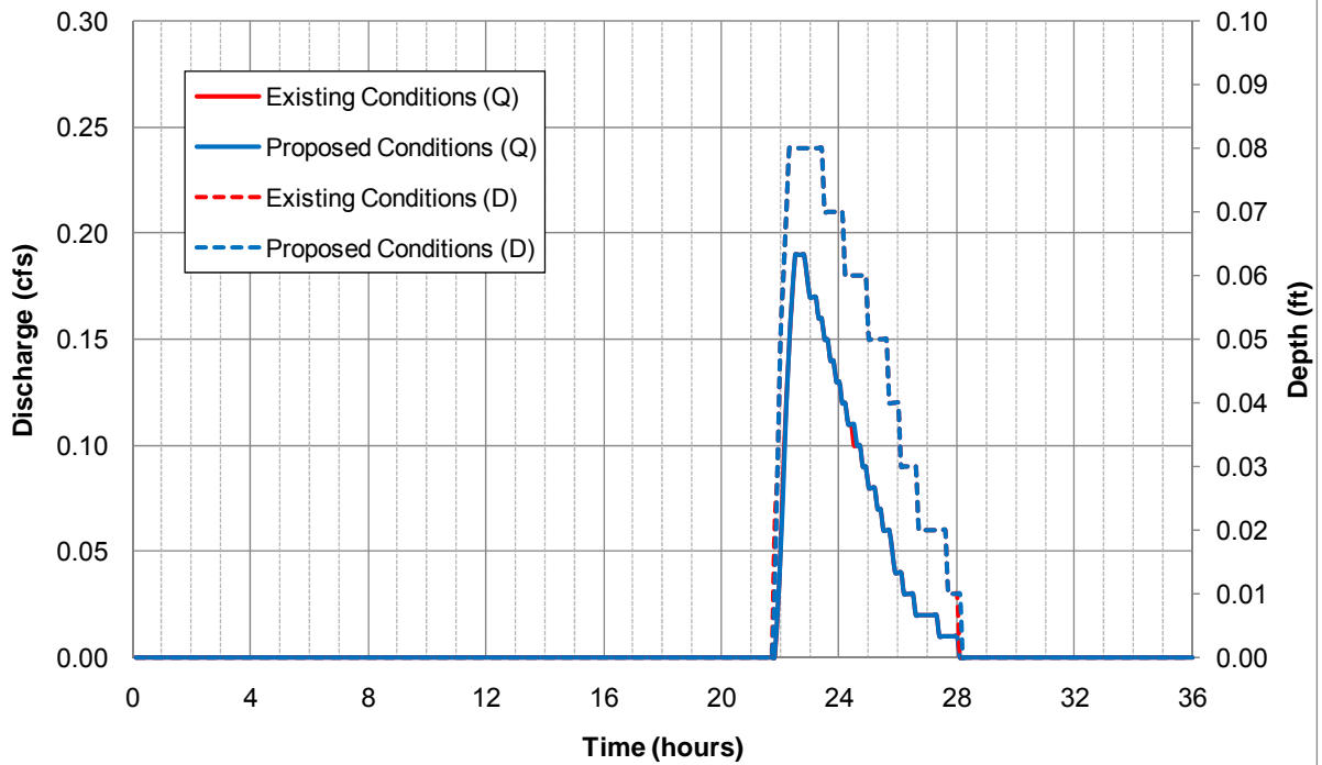
24-hour 2-year Hydrograph at Trestle 7
