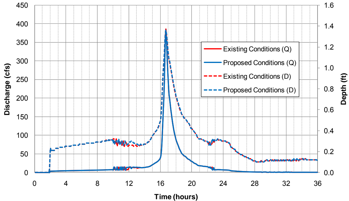
24-hour 10-year Hydrograph at Trestle 8
