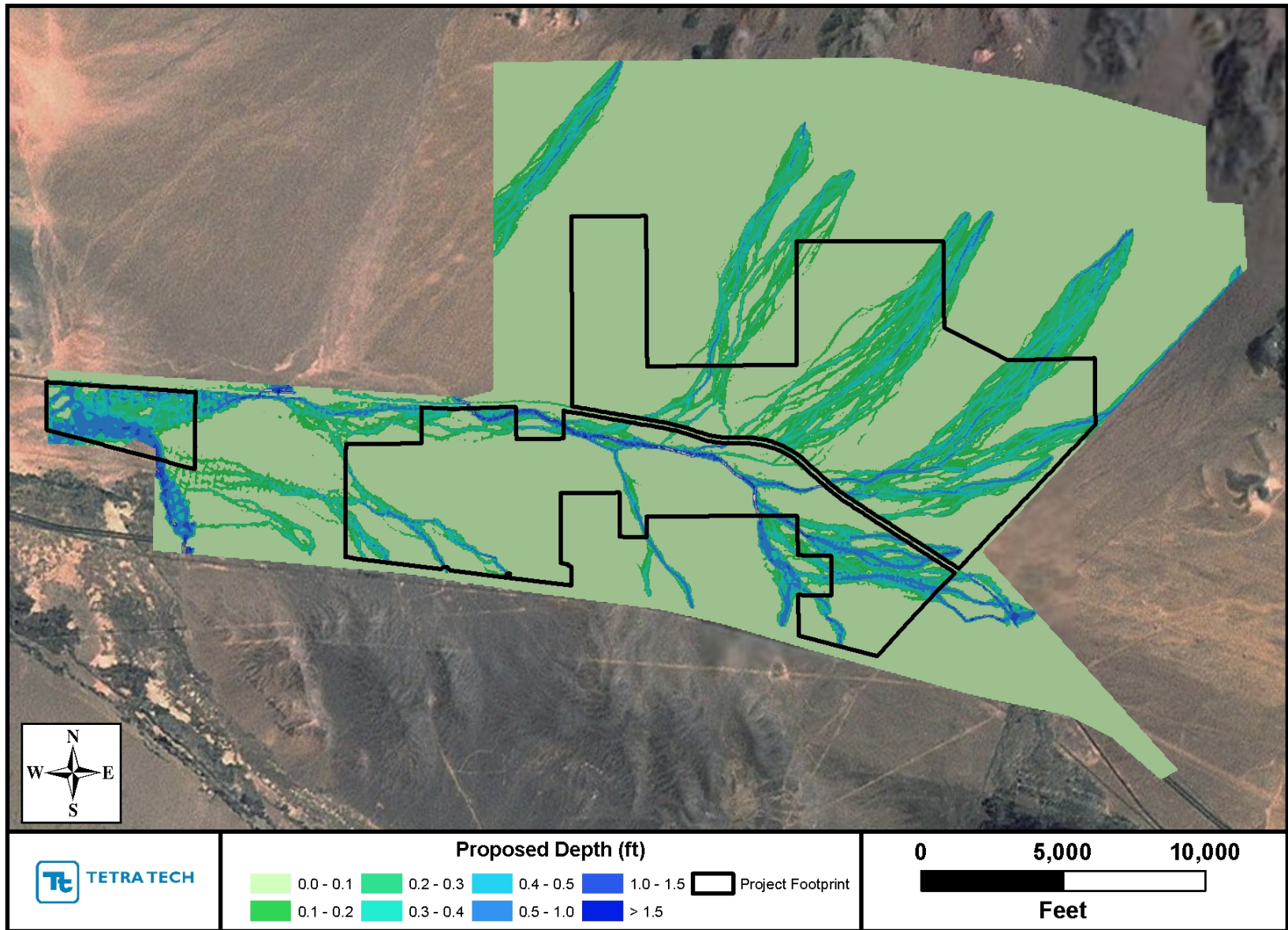
Maximum depths during the 10-year, 24-hour storm.
