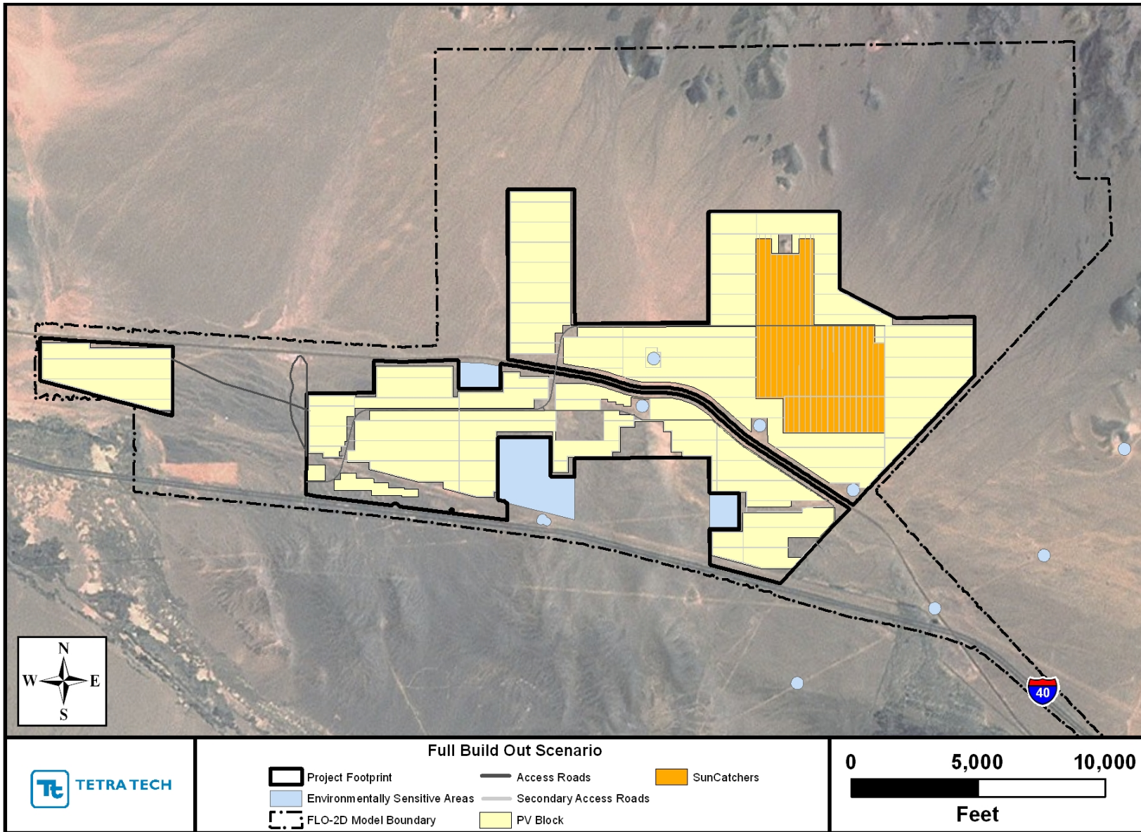
Figure 3.6. Project site map showing features under full build-out conditions.
