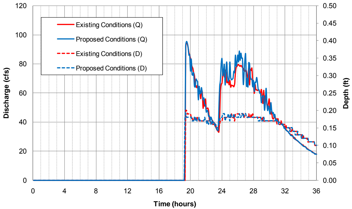
24-hour 5-year Hydrograph at a Cross Section on Main Access Road
