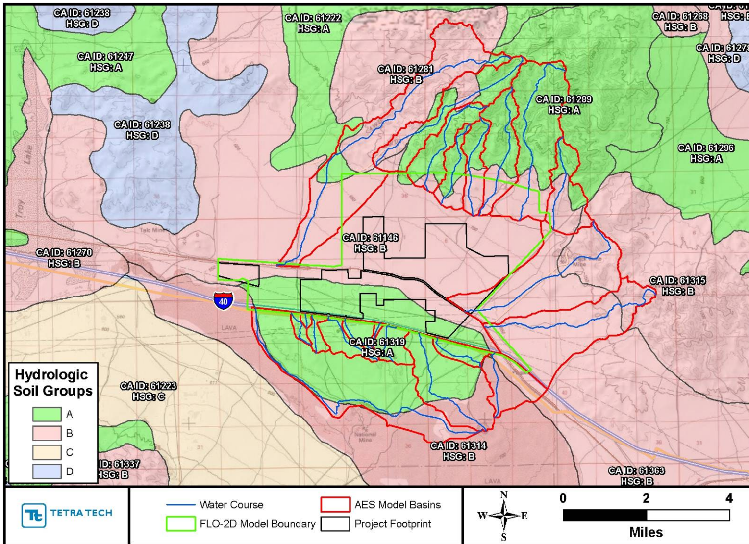
Figure 2.6. Hydrologic soil groups in the vicinity of the project from NRCS STATSGO2 website.
