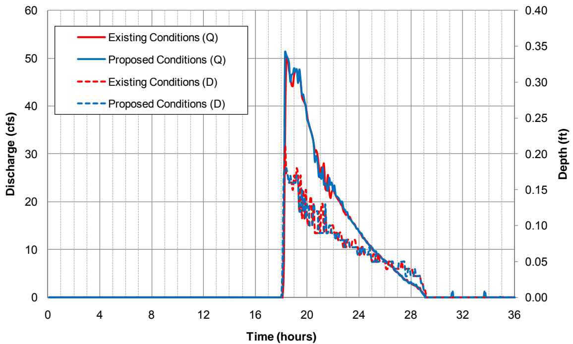
24-hour 10-year Hydrograph at a Cross Section North of Railroad
