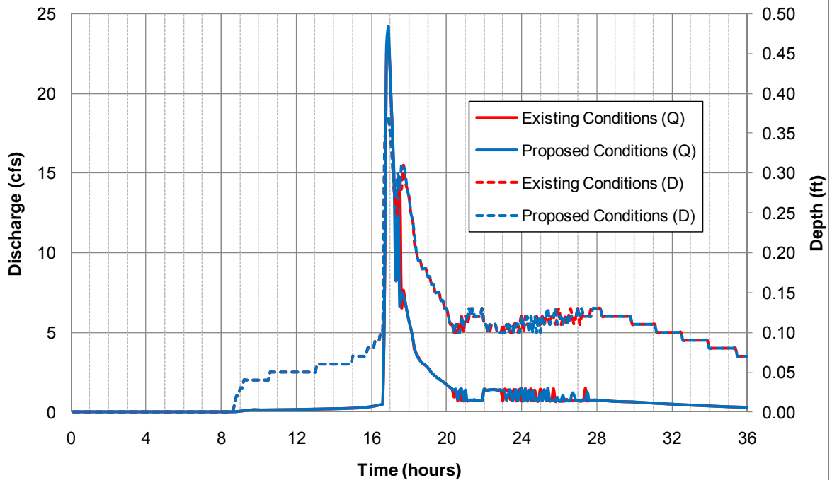
24-hour 100-year Hydrograph at Trestle 8
