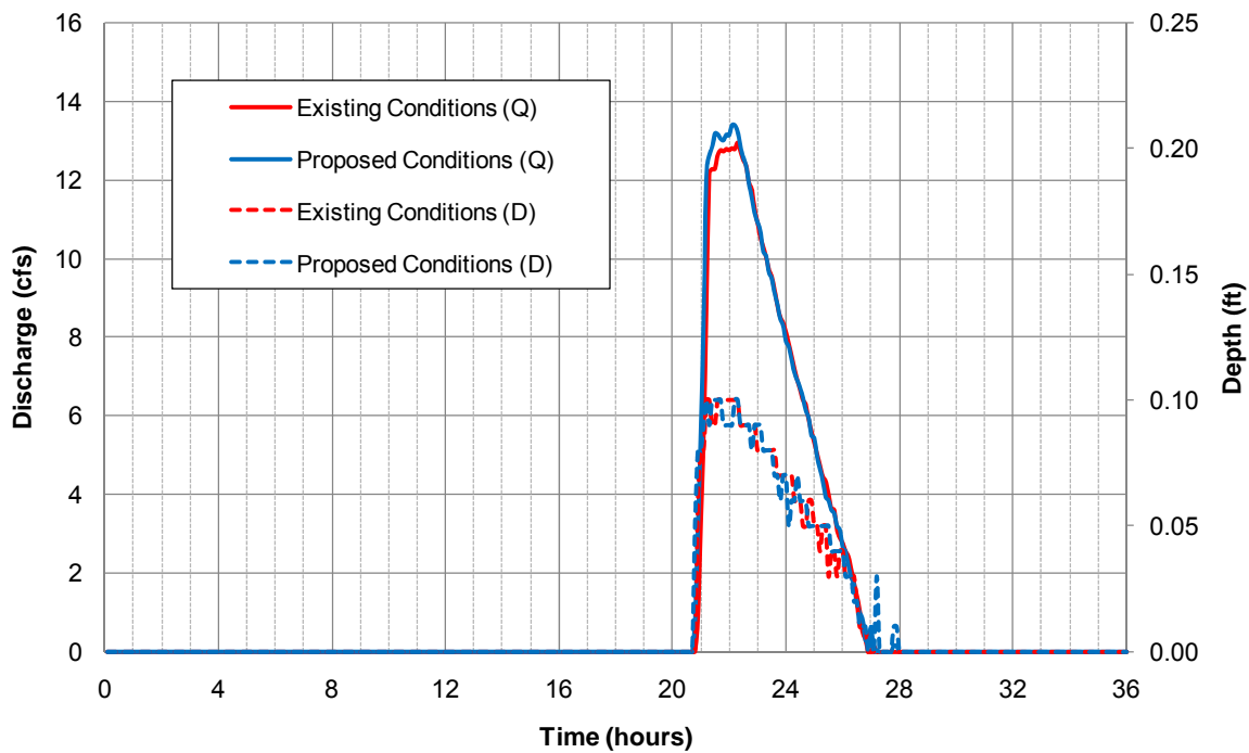
24-hour 5-year Hydrograph at a Cross Section North of Railroad
