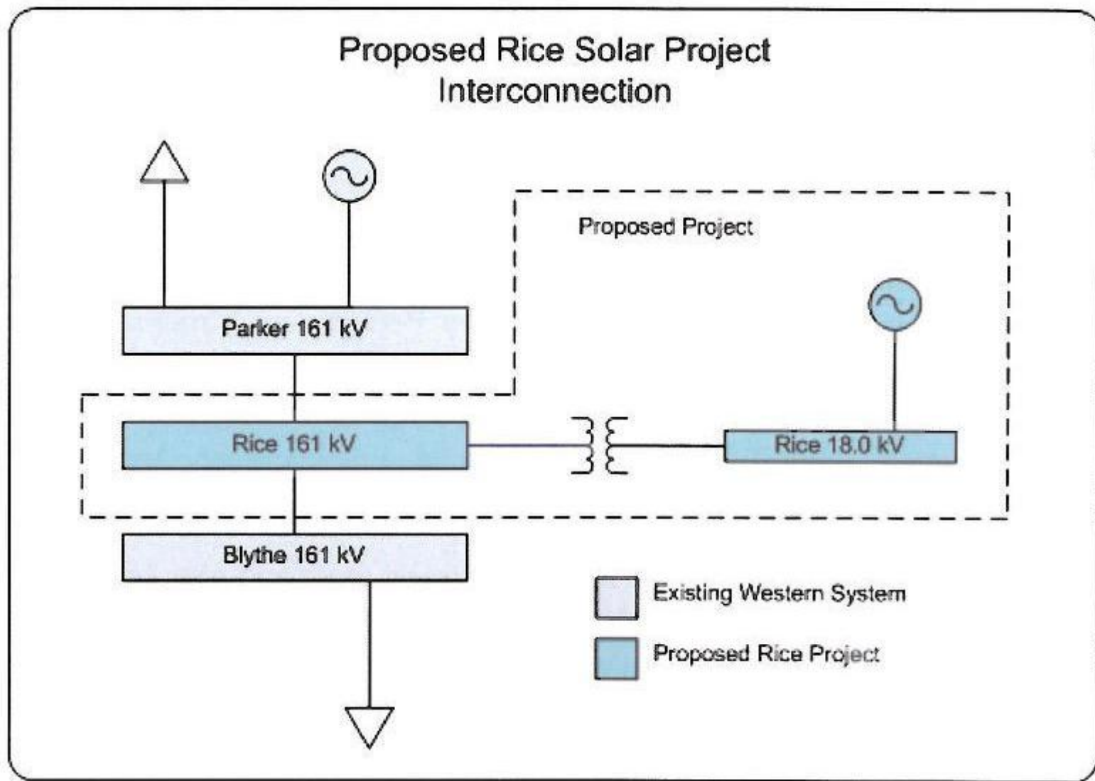
Figure 1: Project Interconnection Point
