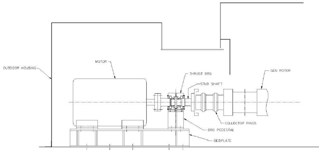
Detail - Pony Motor & Bearing Arrangement (1 ea. for Unit 3-HP & Unit 4-IP/LP )
