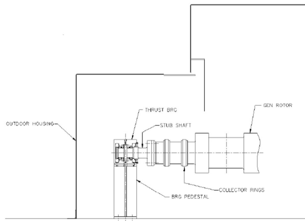
Detail - Bearing Only Arrangement (1 ea. for Unit 3-LP & Unit 4-HP/LP )
