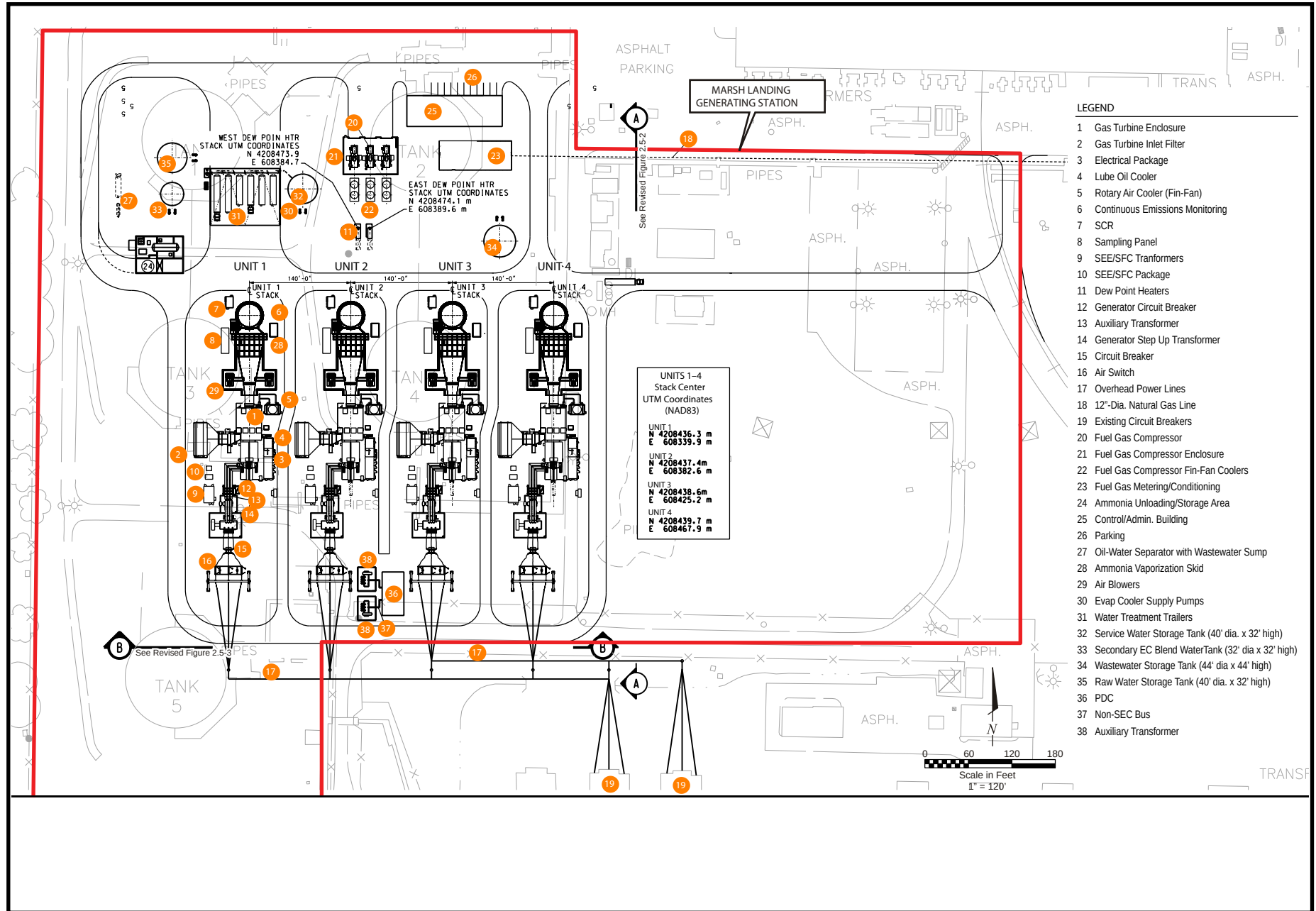
VISUAL RESOURCES - FIGURE 1 Marsh Landing Generating Station - General Plot Plan
