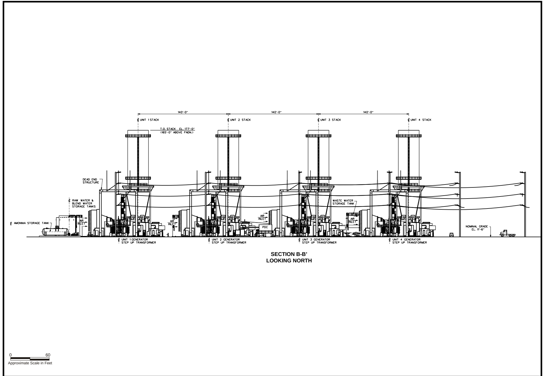
PROJECT DESCRIPTION - FIGURE 6 Marsh Landing Generating Station - Elevation View - Simple Cycle Units Looking North
