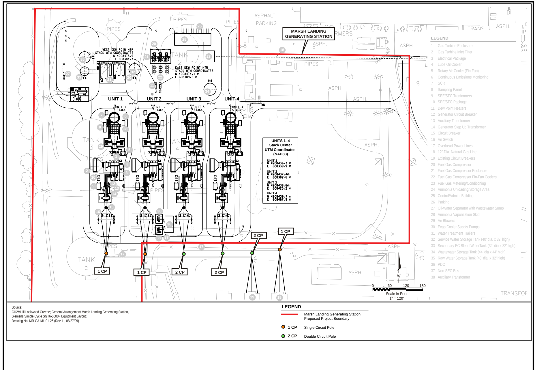
TRANSMISSION SYSTEM ENGINEERING - FIGURE 1 Marsh Landing Generating Station - Electrical Interconnection to the PG&E Switchyard
