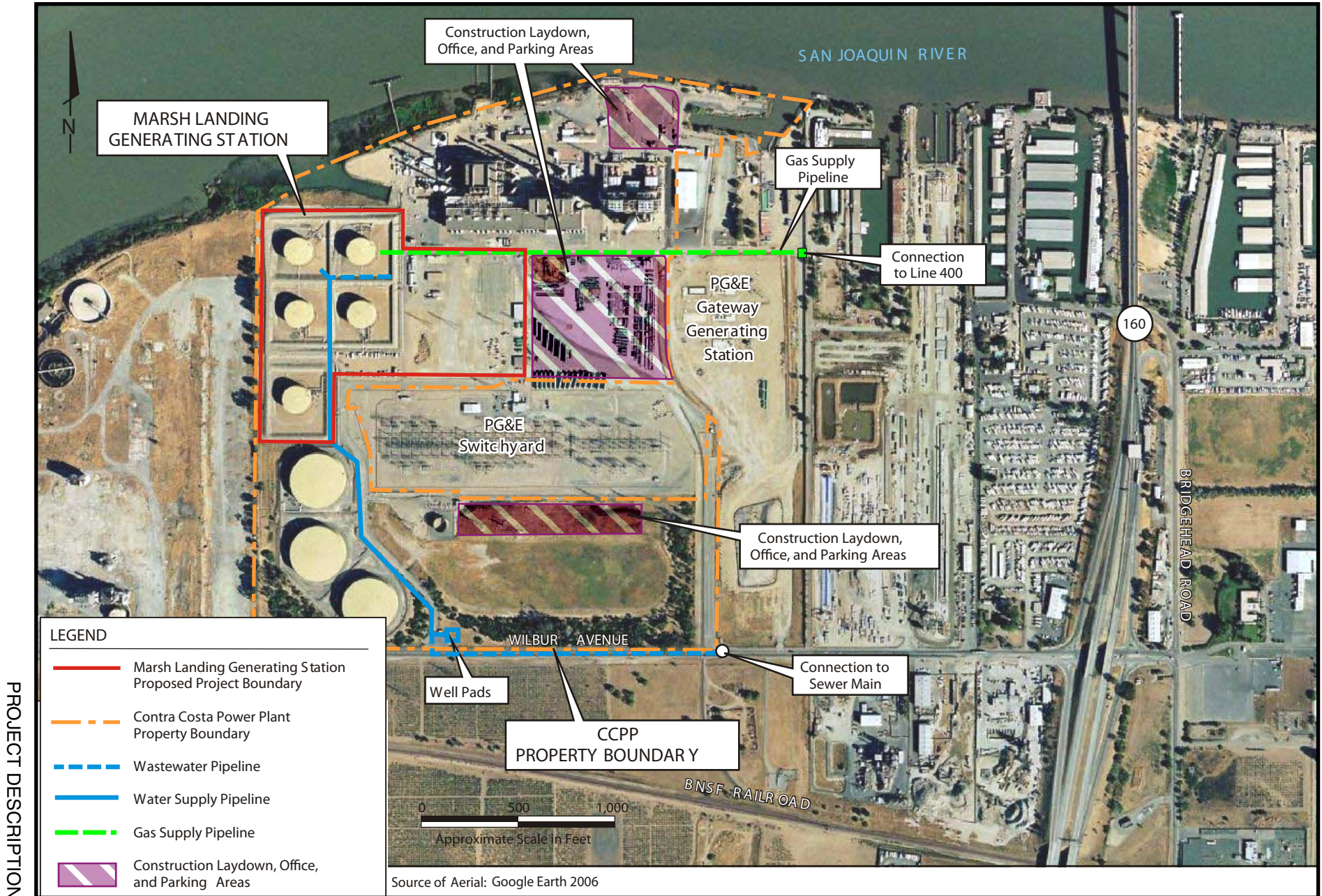
PROJECT DESCRIPTION - FIGURE 3 Marsh Landing Generating Station - Site Plan
