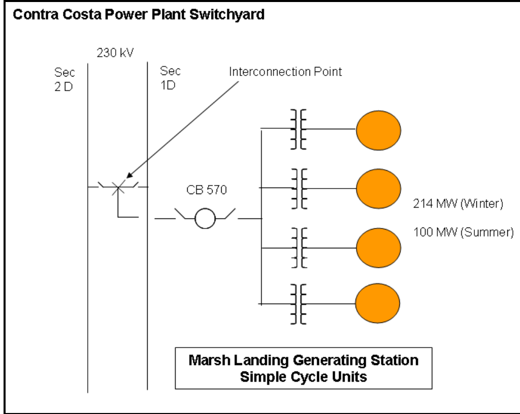
Figure 2-2: Proposed Single Line Diagram
