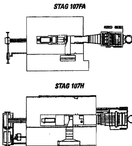
Figure 4. 7H and 7FA footprint comparison
