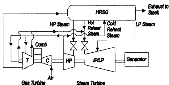
Figure 3. H Combined-cycle and steam description
