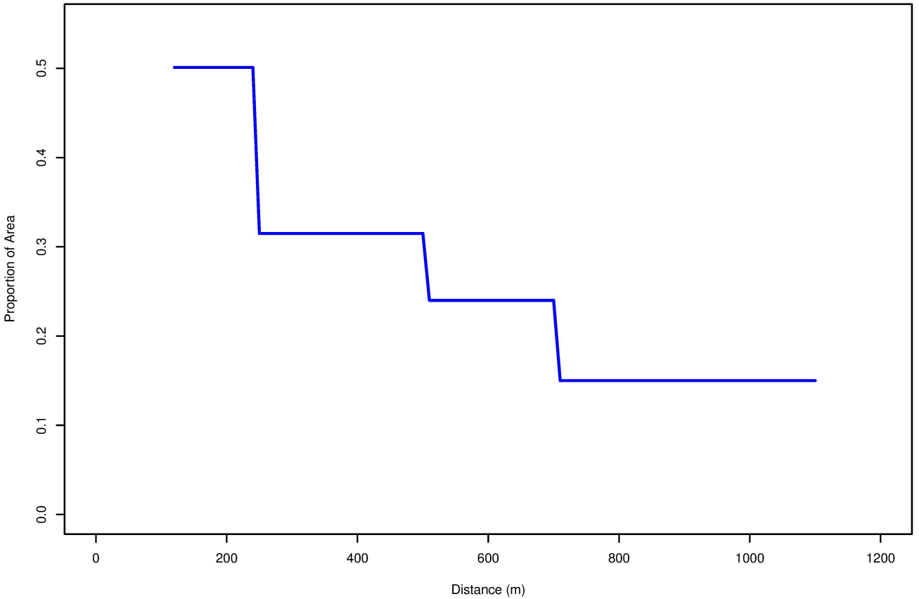
ISEGS: Proportion of Area Occupied by Heliostats
