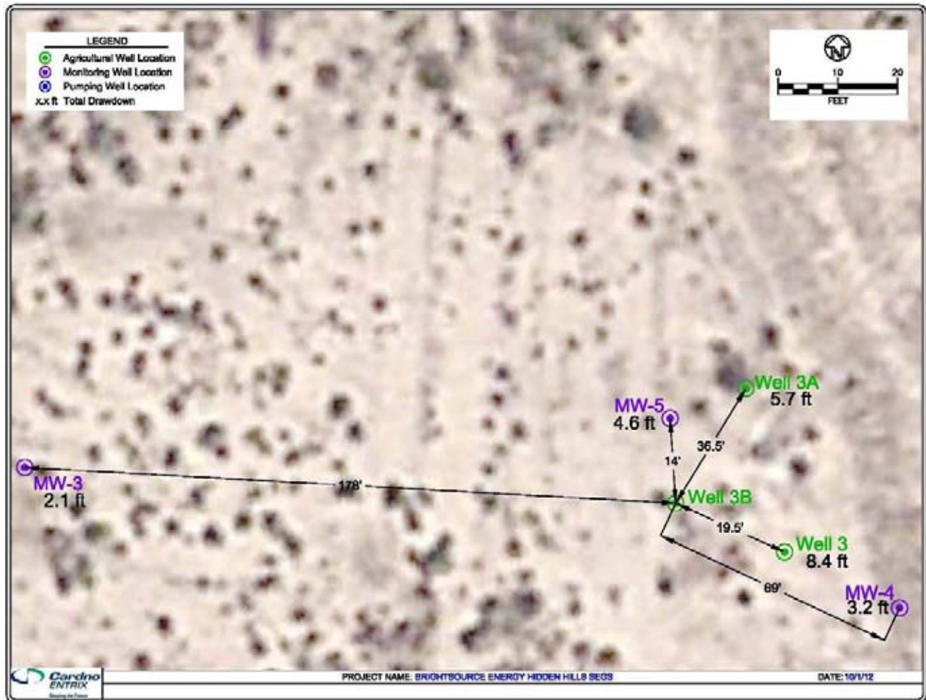
Figure 6-1 Schematic diagram of observed drawdowns in monitoring wells
