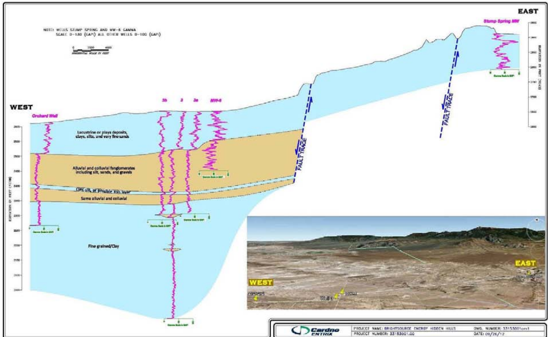
Figure 4-1 Geologic Cross-Section from Orchard Well to Stump Spring
