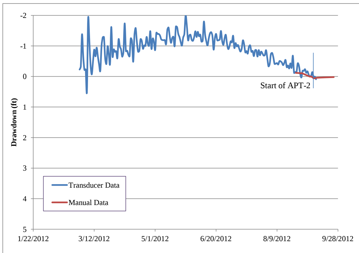
Figure 6-4 Drawdown measured in the Stump Spring Monitoring Well, March to September, 2012
