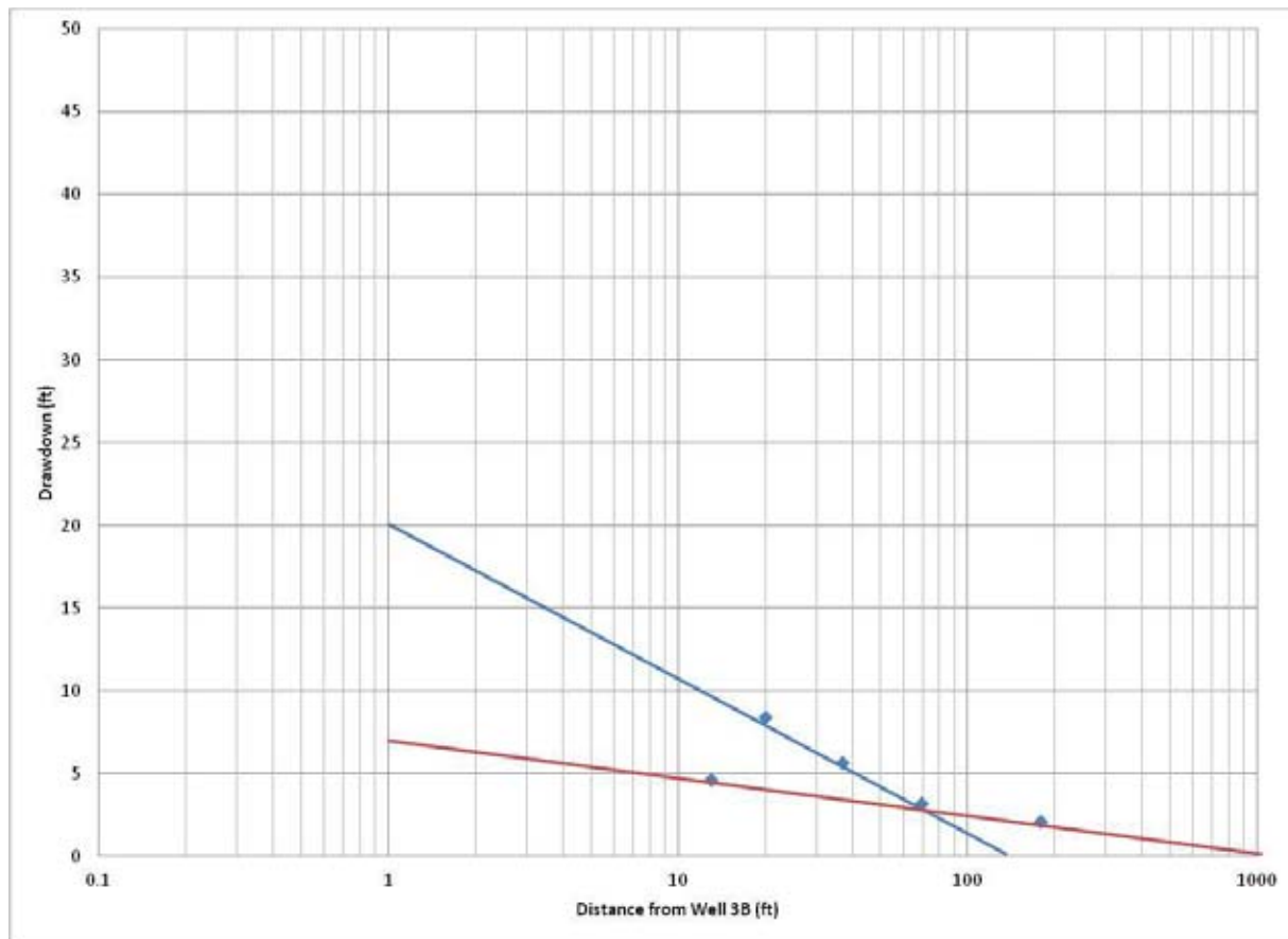
Figure 6-10 Drawdown vs. distance from Well 3B after 14 days of pumping at 45 gpm
