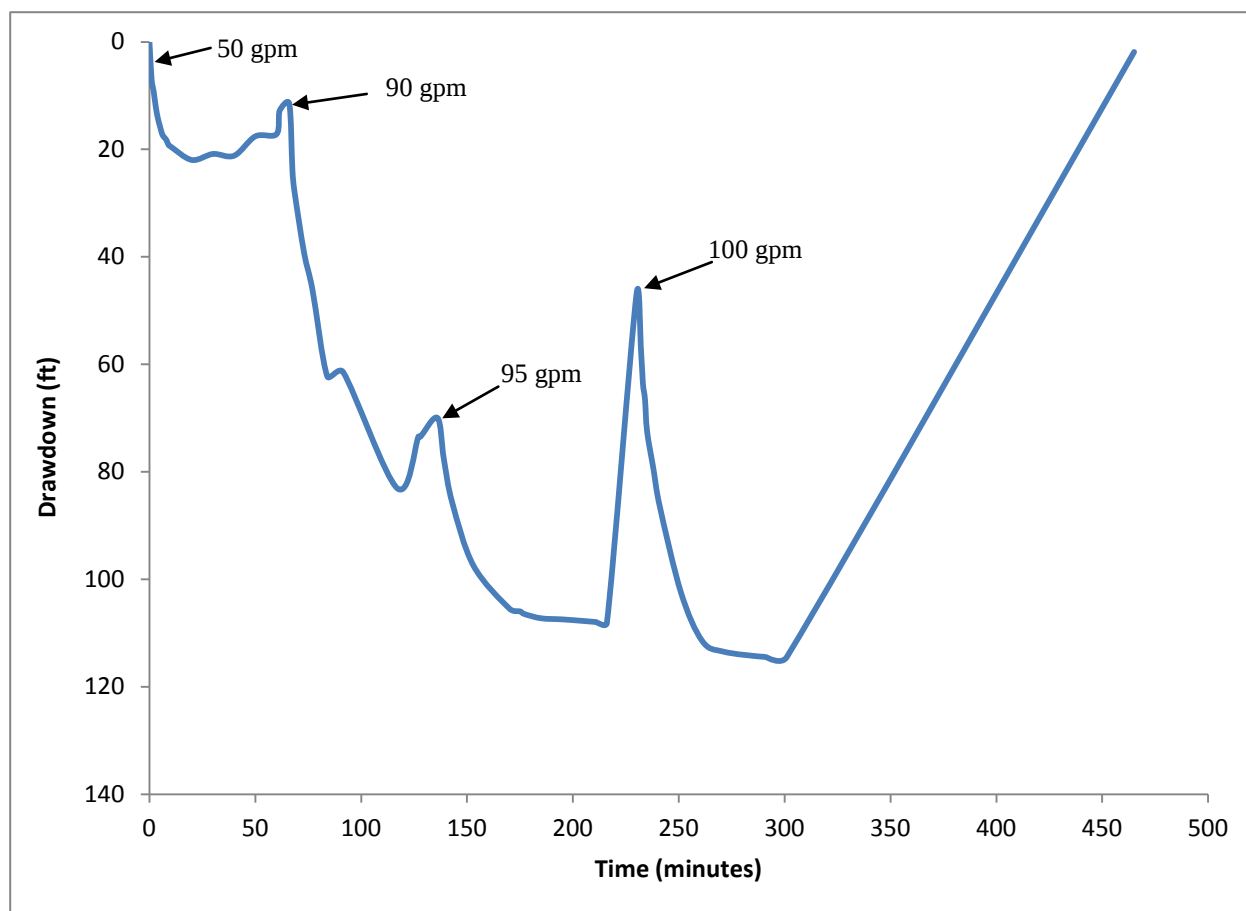
Figure 2-1 Well 3A Step Test Drawdown
