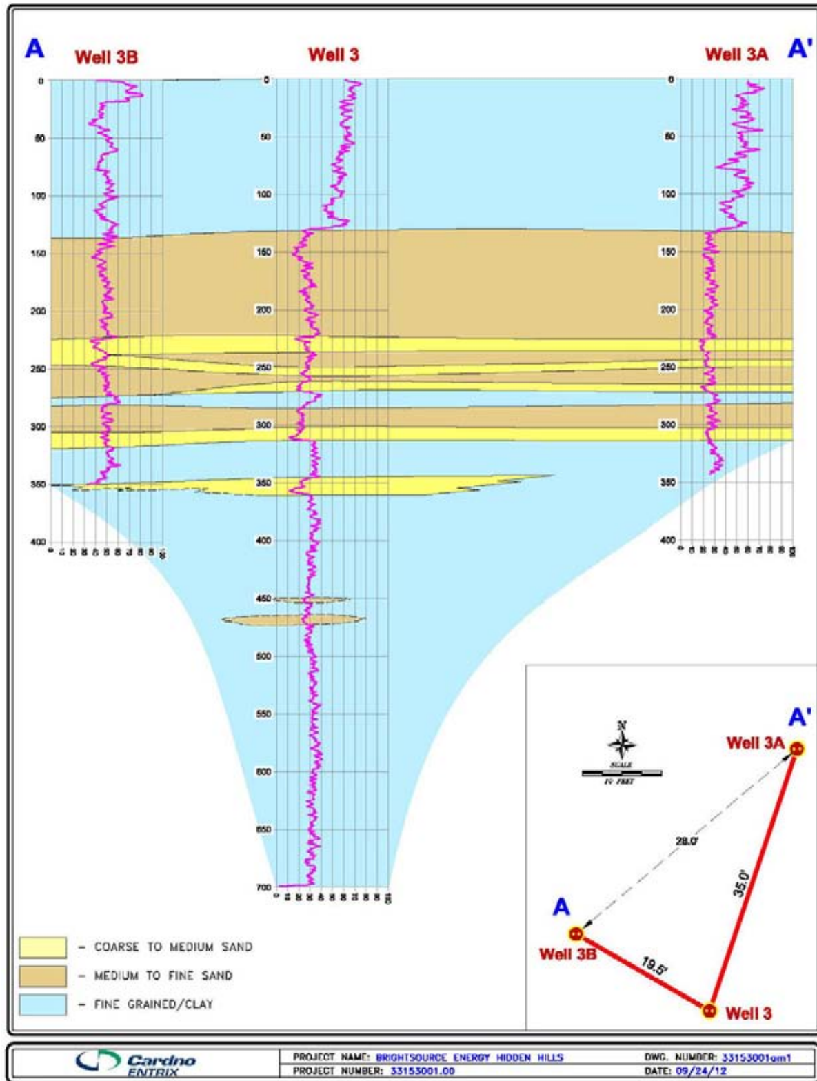
Figure 4-2 Geologic Cross-Section in Vicinity of Well 3
