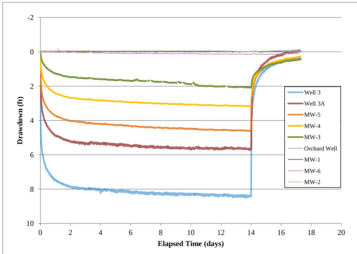
Figure 6-2 Observed water levels in monitoring wells during APT 2
