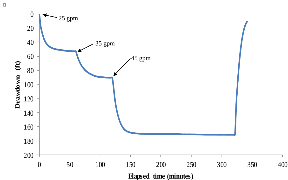
Figure 3-1 Drawdown during Well 3B Step Test
