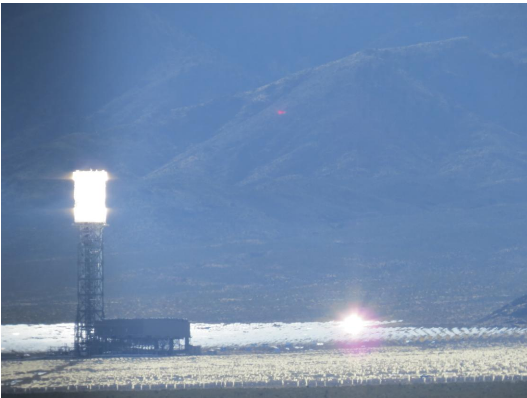
Two photos of flash-glare on Unit 3, Ivanpah Solar Electric Generating System, March 14 th , 2014 Taken with a Canon Powershot SX50 HS Optical Zoom, taken about two miles northeast near the turn off to Umberci Mine.
