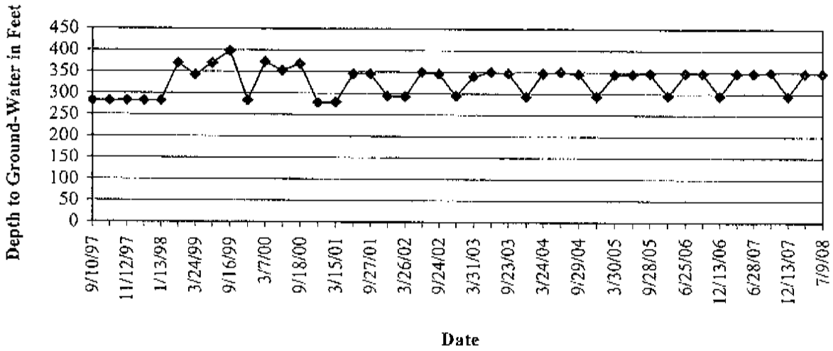
Graph 9: Well Colosseum #2 Hydrograph
