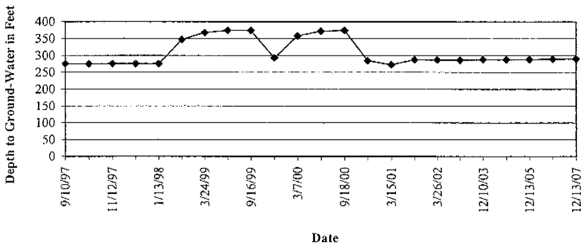
Graph 7: Well Colosseum #1 Hydrograph
