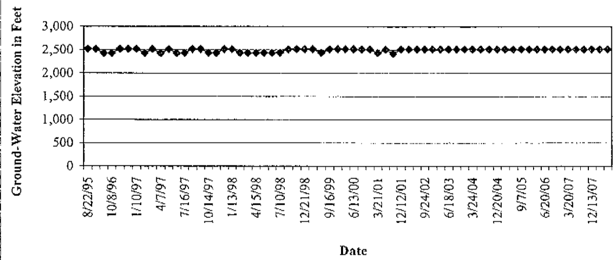
Graph 1: Well PVGC #7 Hydrograph
