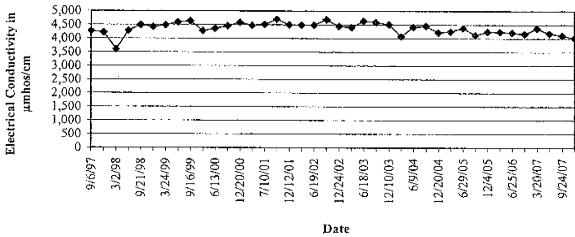
Graph 13: Well M-8 Electrical Conductivity Data
