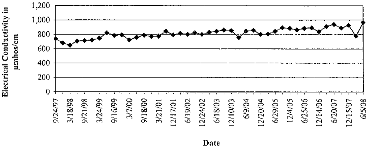
Graph 11: Well WP-5 Electrical Conductivity Data
