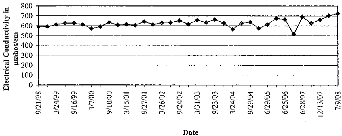
Graph 8: Well Colosseum #1 Electrical Conductivity Data
