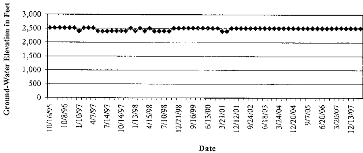
Graph 5: Well PVGC #9 Hydrograph
