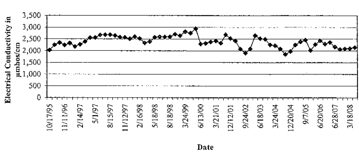
Graph 2: Well PVGC #7 Electrical Conductivity Data
