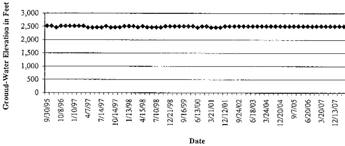
Graph 3: Well PVGC #8 Hydrograph
