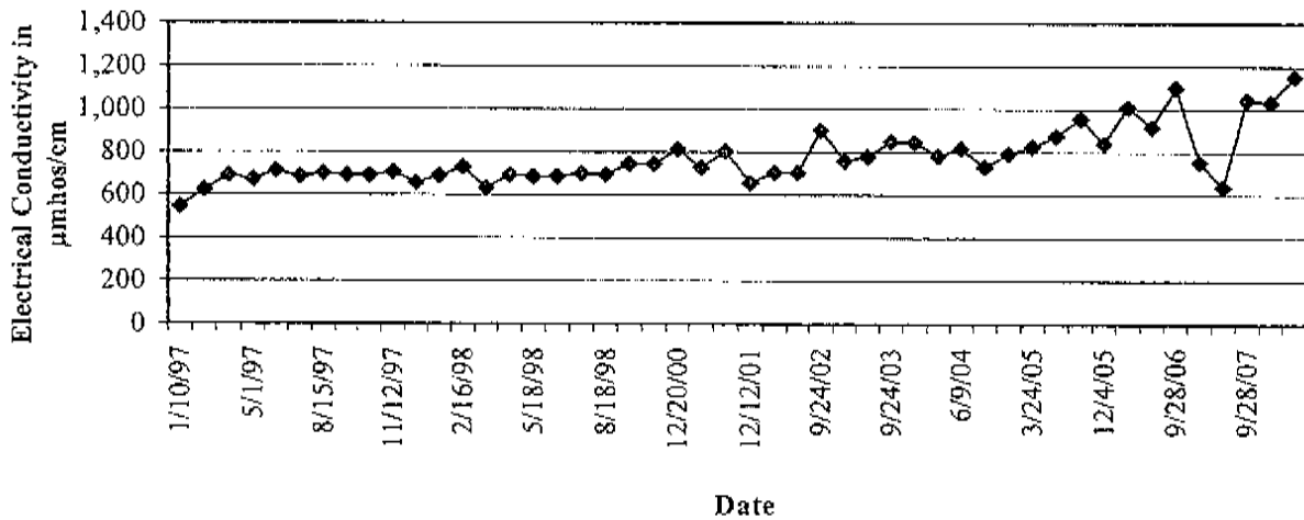
Graph 6: Well PVGC #9 Electrical Conductivity Data
