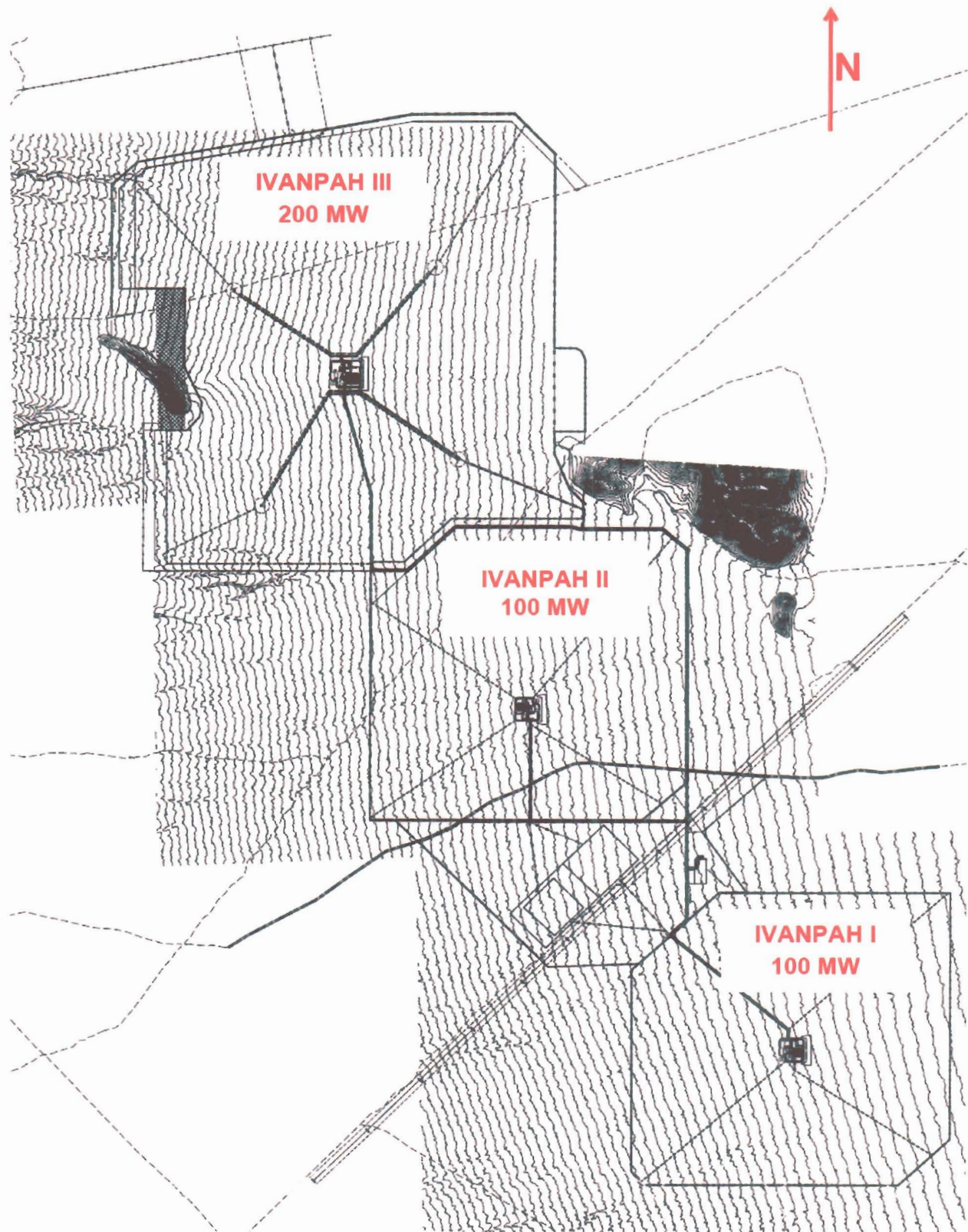
IVANPAH SEGS UNITS 1-3
