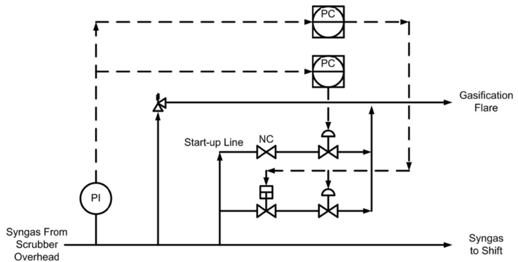
Figure 1 Syngas Relief Valve Configuration 3
