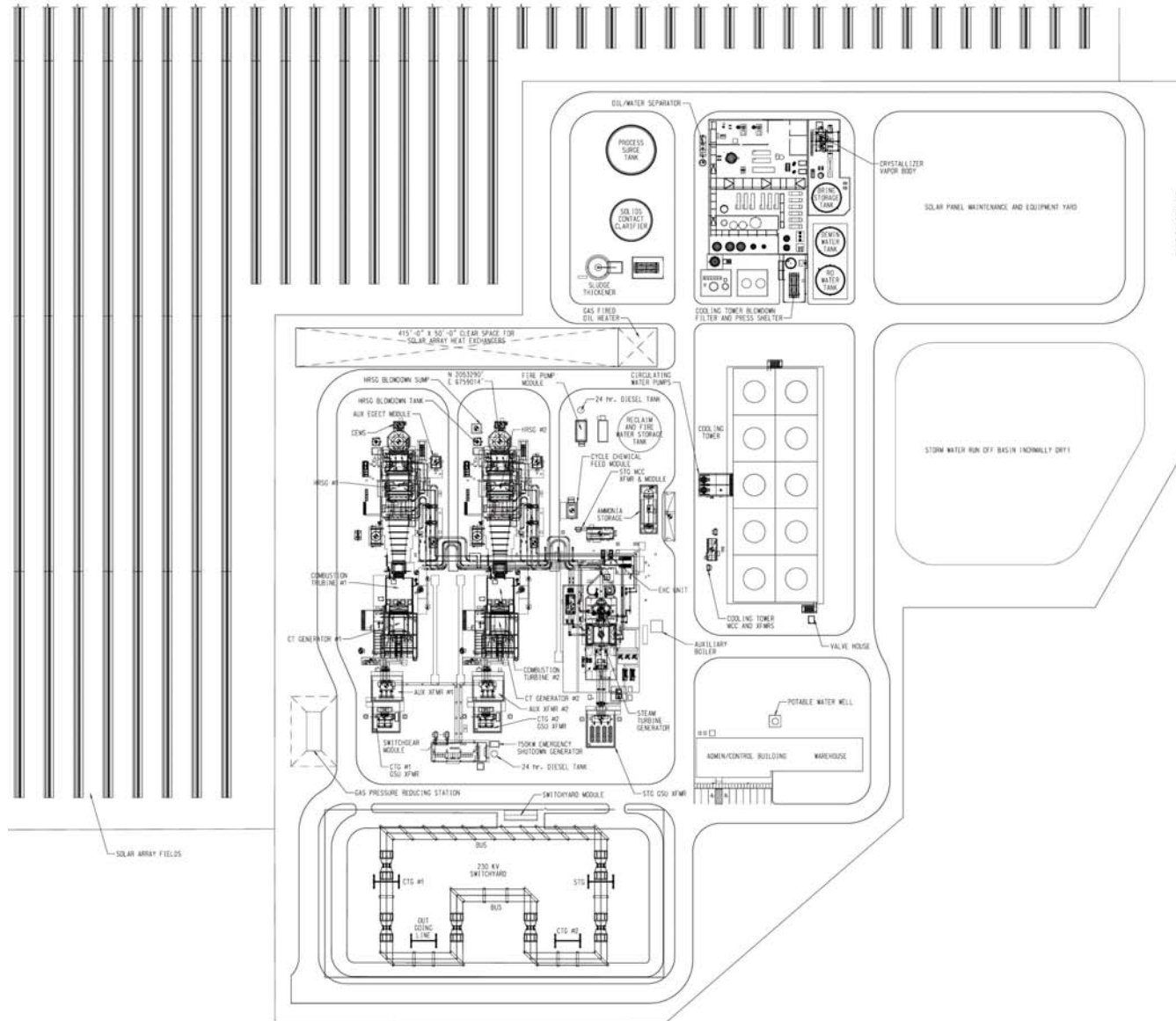
PROJECT DESCRIPTION - FIGURE 3 Victorville 2 Hybrid Power Project - General Arrangement of Project
