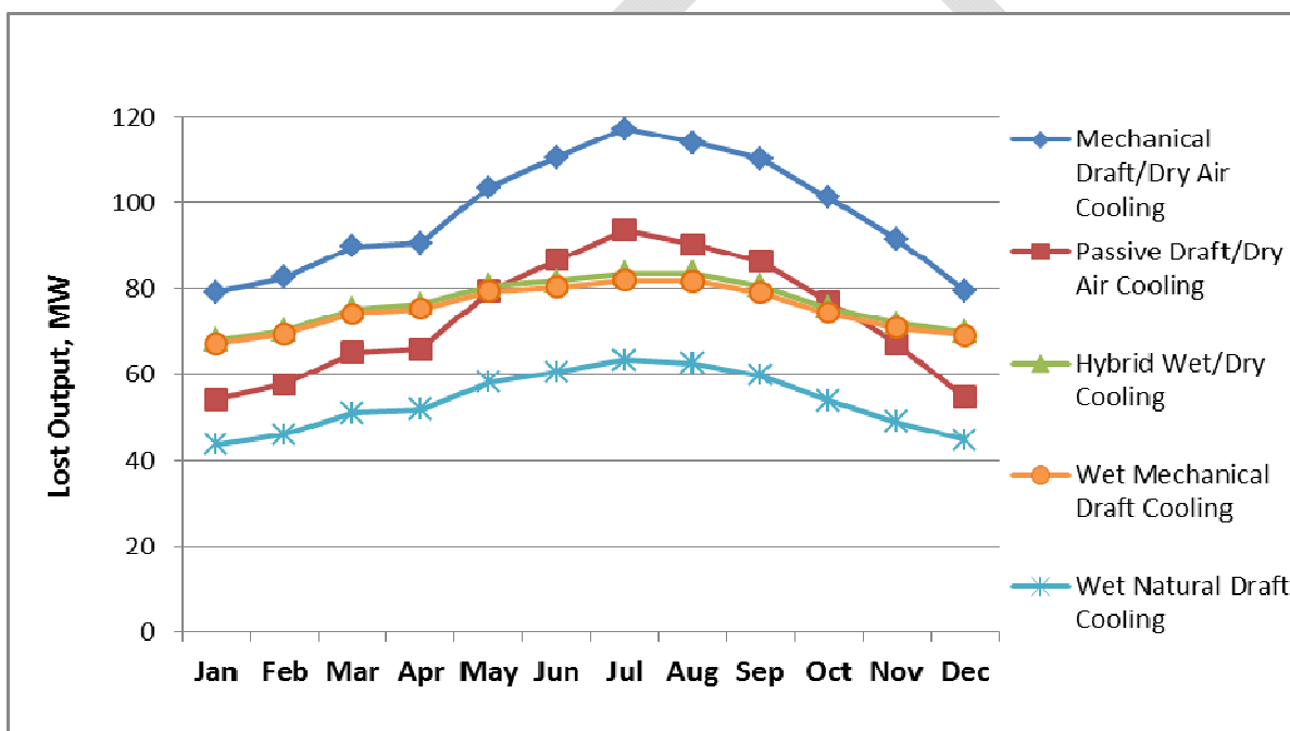
Figure 4.3-3. Average Lost Output per Month
