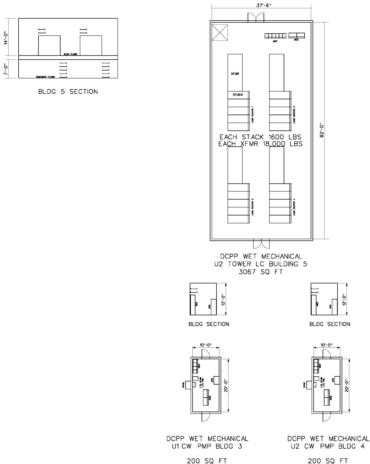
Figure 4.3-18. Wet Mechanical (Forced) Draft Cooling—Cooling Tower and Pumphouse Electrical Buildings
