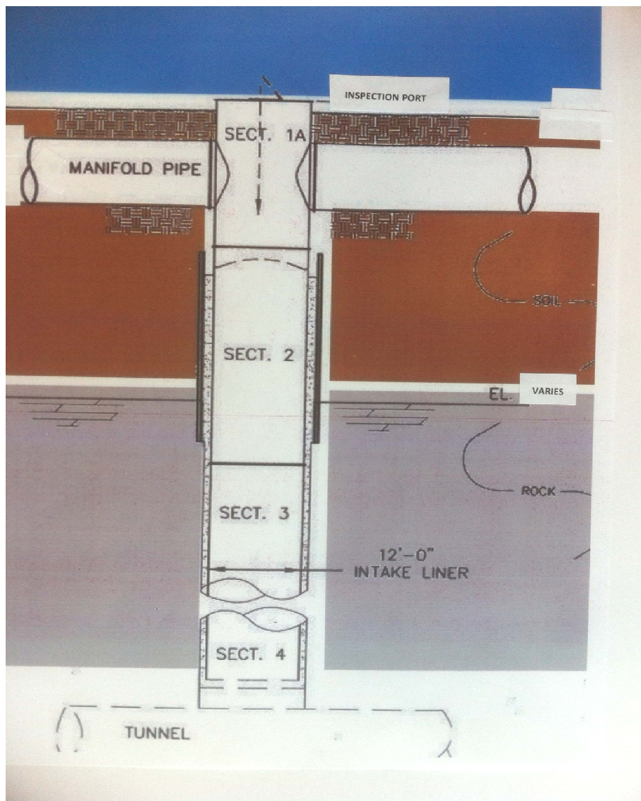
Figure 5.2-2. Installation of Offshore Intake Manifold Piping
