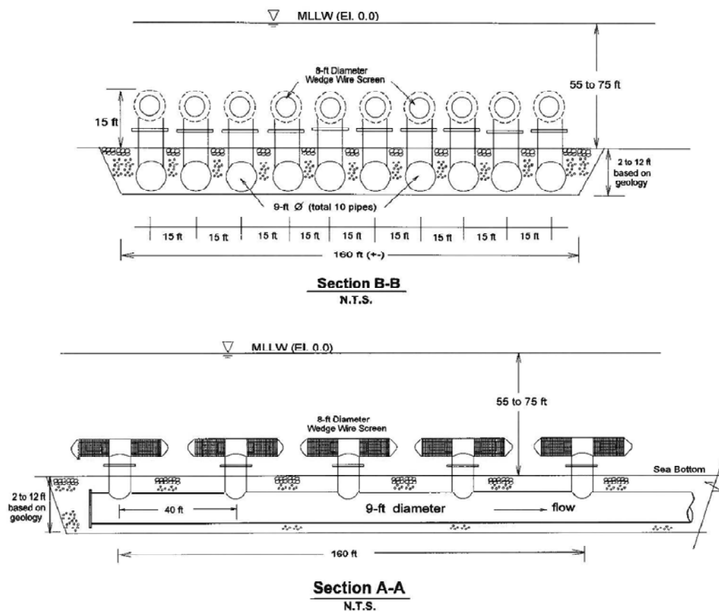
Figure 4.2-17. DCP 2-mm-Slot Modular Wedge Wire Screen Intake Assembly (Sectional Views)
