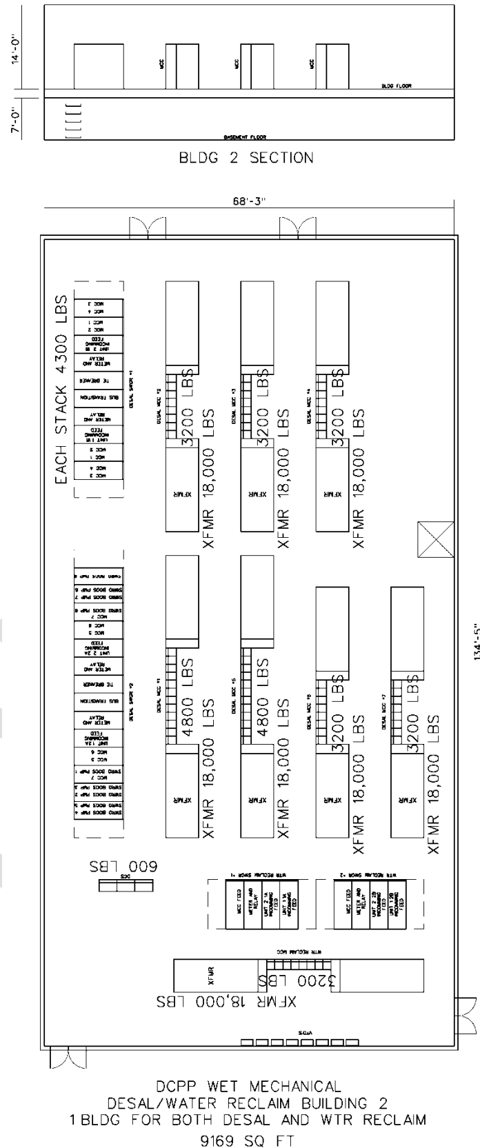
Figure 4.3-19. Wet Mechanical (Forced) Draft Cooling—Desalination/Water Reclaim Electrical Building
