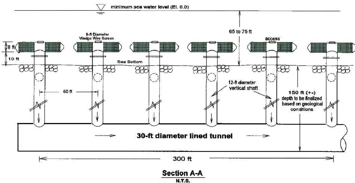
Figure 4.2-9. DCP 2-mm-Slot Modular Wedge Wire Screen Intake System (Sectional Views)
