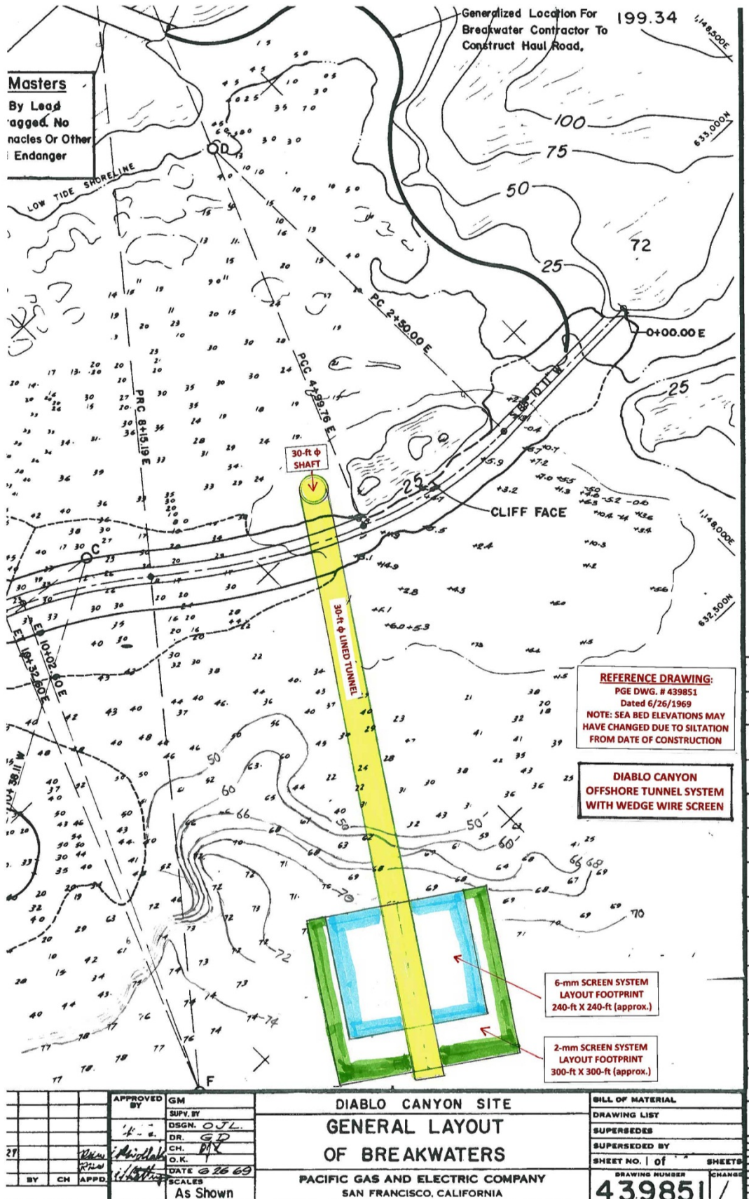
Figure 4.2-4. DCP General Layout of Breakwaters
