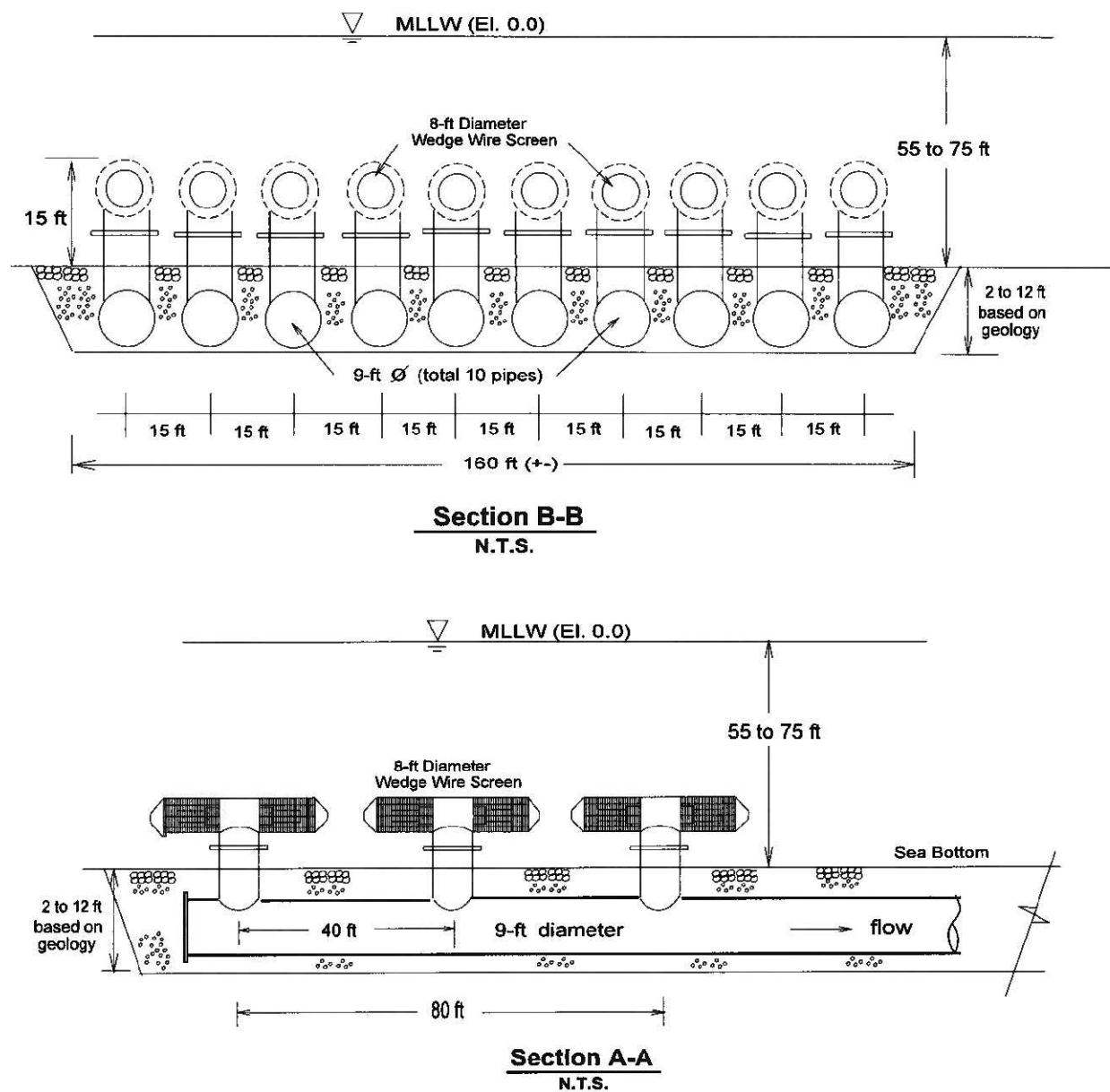
Figure 4.2-15. DCP6 6-mm-Slot Modular Wedge Wire Screen Intake Assembly (Sectional Views)
