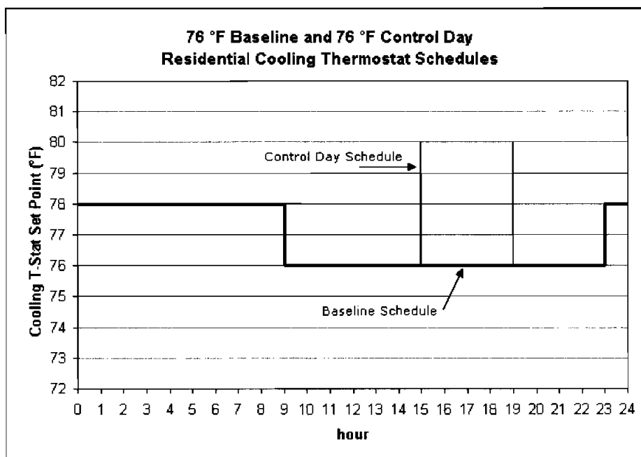
Figure 7. Residential Baseline and Control day cooling thermostat schedule
