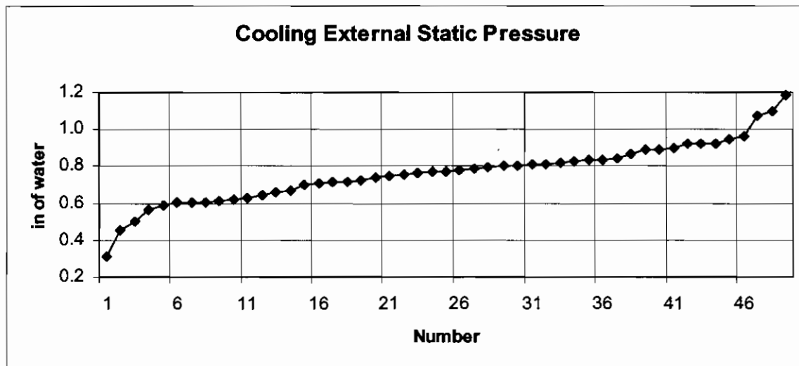
Figure 3. California New Construction Field Test Furnace Cooling External Static Pressure
