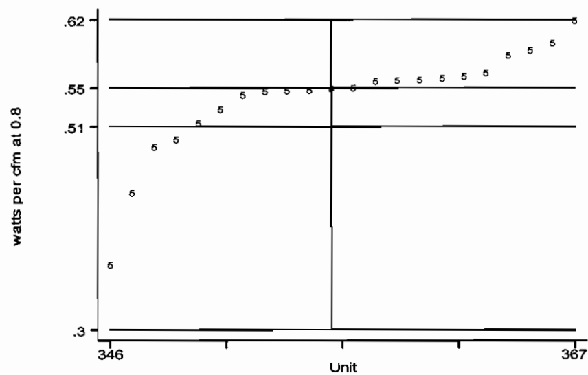
Figure 7. Five Ton High Speed PSC at 0.80 IWC
