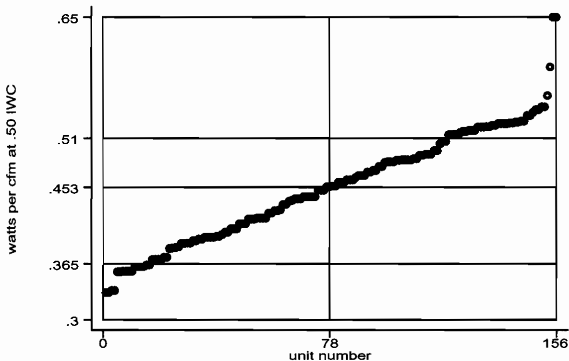
Figure 4. High Speed PSC Air Handler/Furnace Power at 0.50 IWC External Static
