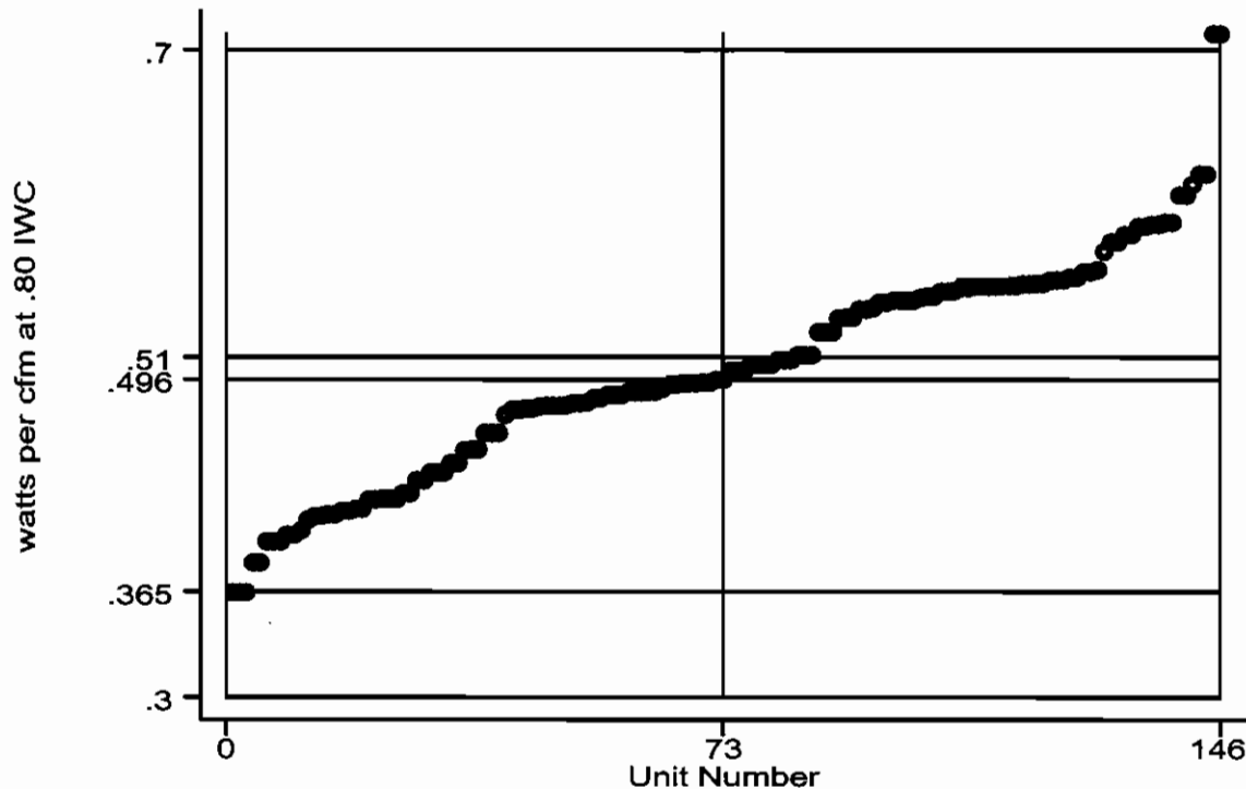
Figure 5. High Speed PSC Air Handler/Furnace Power at 0.80 IWC External Static
