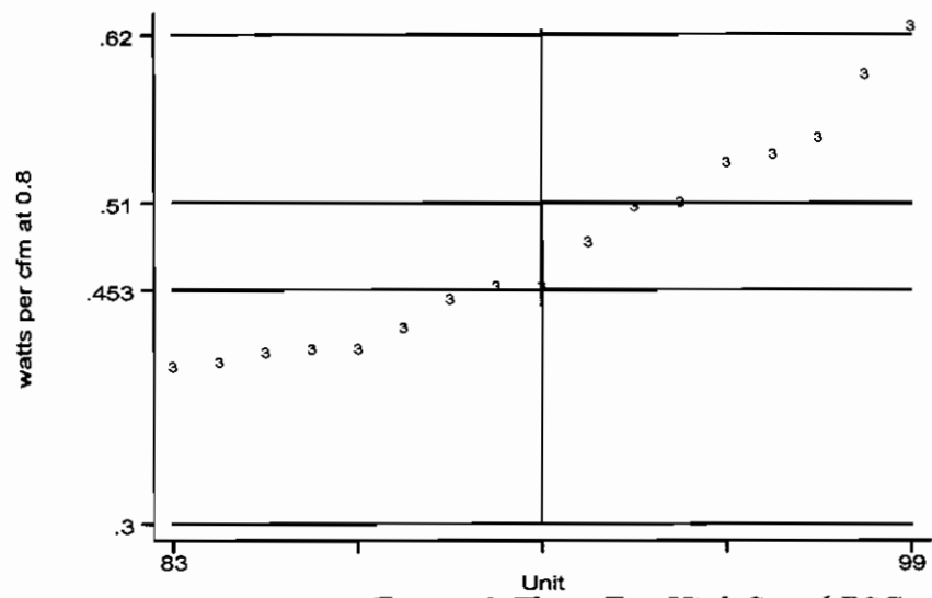
Figure 6. Three Ton High Speed PSC at 0.80 IWC
