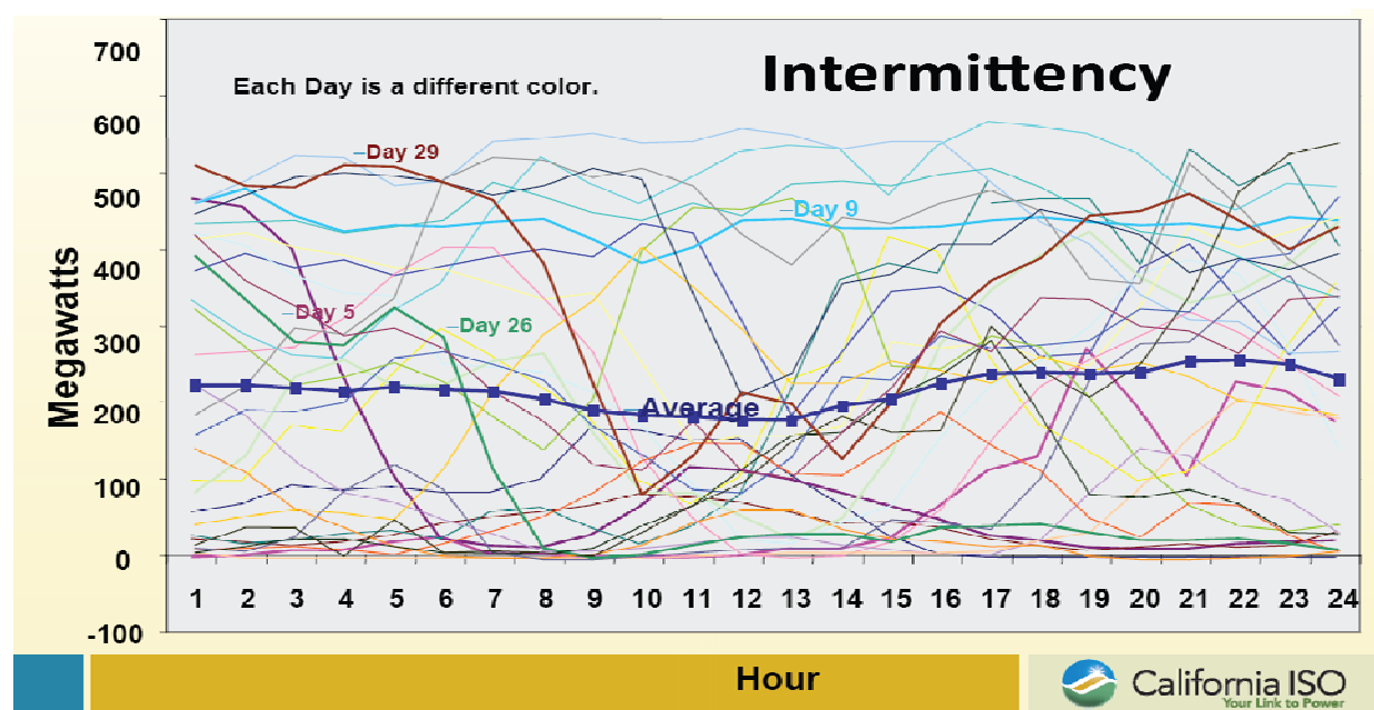
Figure 1: Tehachapi Wind Generation (April 2005)
