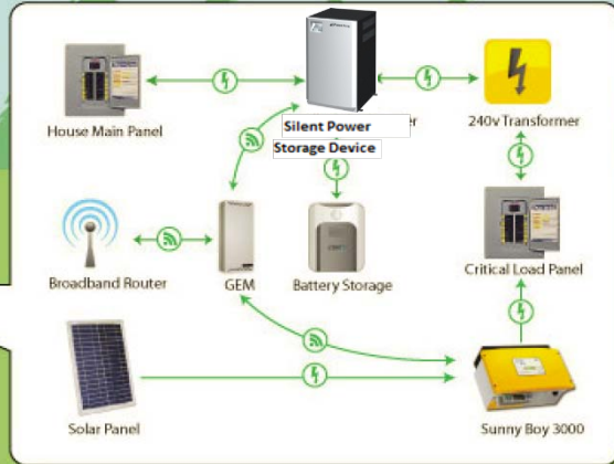
Community Energy Storage (CES) Group: Grid Tied with Battery Storage
