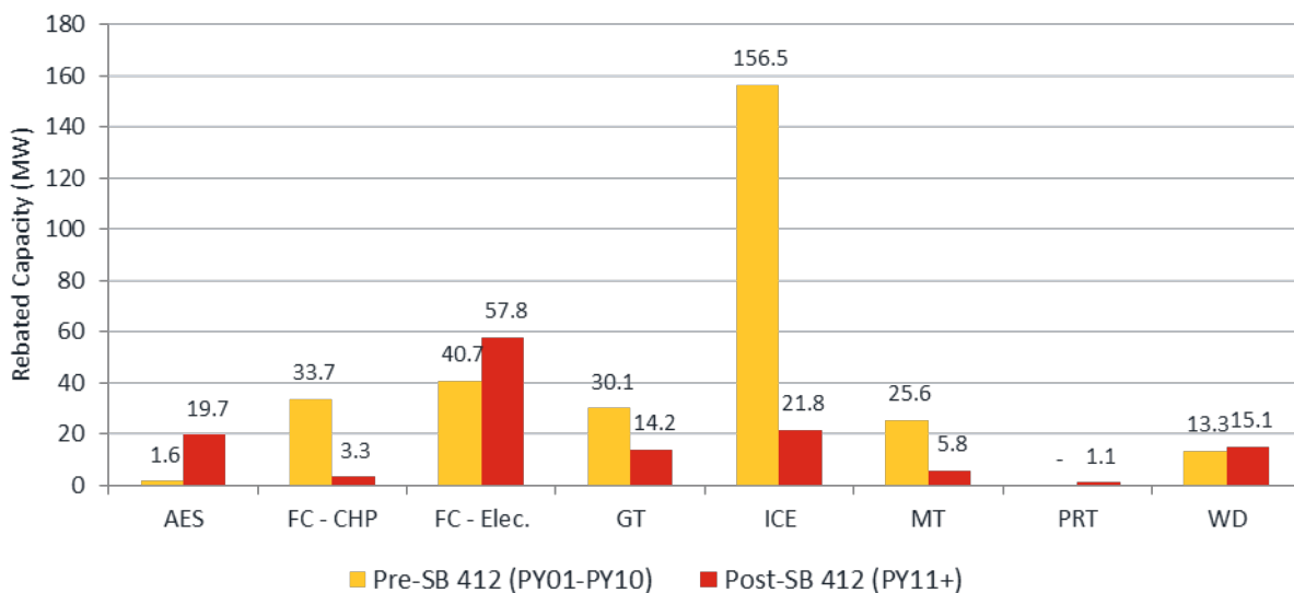
Figure 3-3: Rebated Capacity by Technology Type Pre/Post-SB 412
