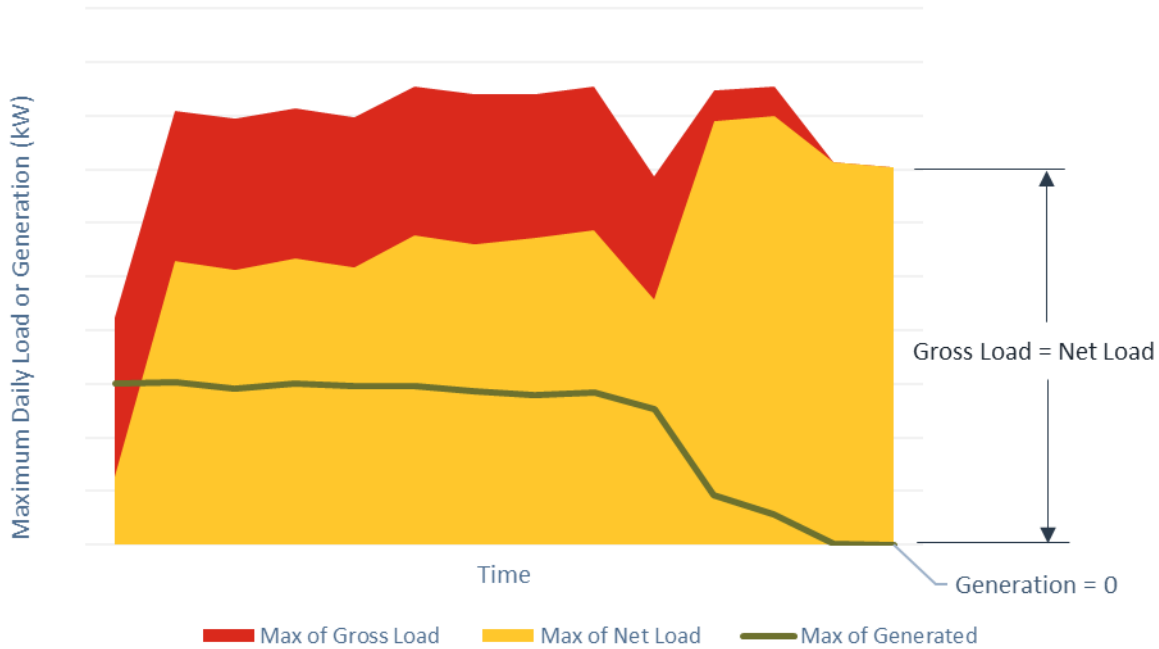
Figure 5-23: Demand Impact from Generator with Outage
