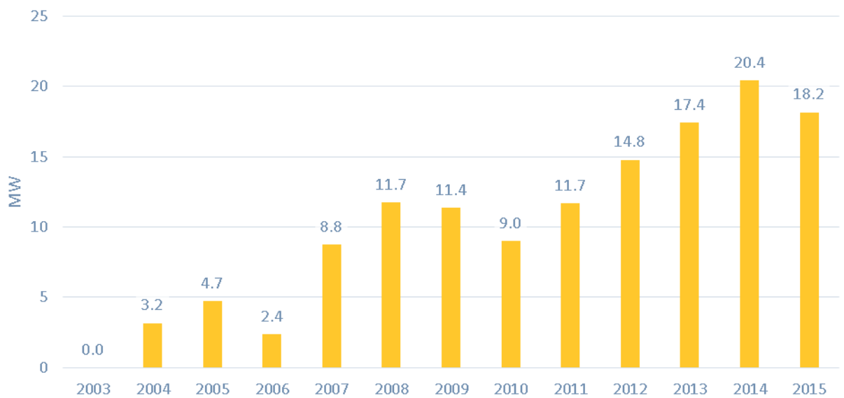
Figure B-9: SDG&E Peak Hour Generation by Calendar Year
