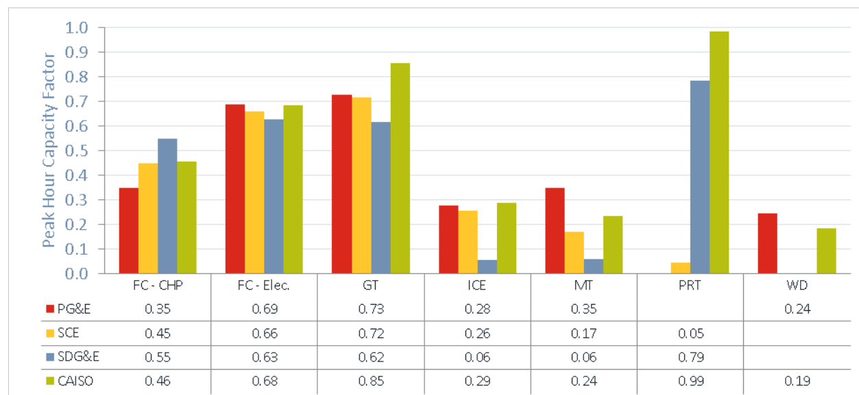
Figure 5-34: 2014 CAISO and IOU Peak Hour Capacity Factors by Technology
