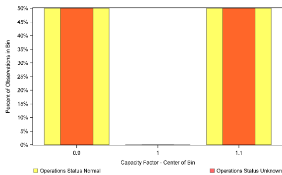
Figure E-9: MCS Distribution – PRT Coincident Peak Output
