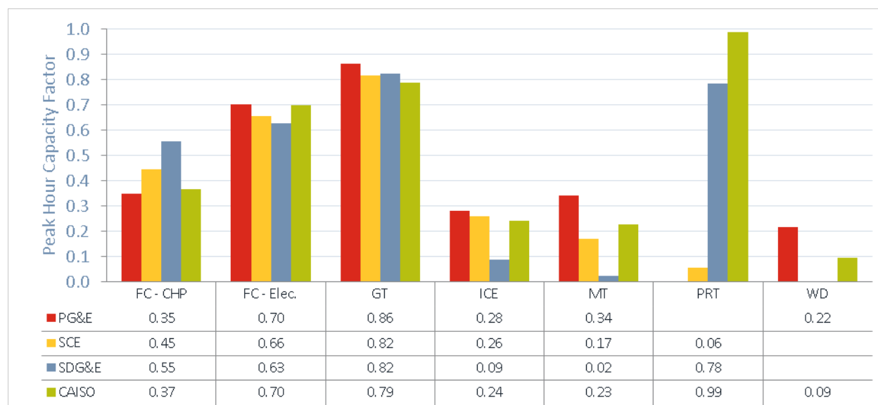
Figure 5-35: 2015 CAISO and IOU Peak Hour Capacity Factors by Technology
