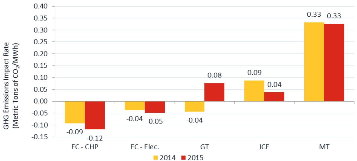
Figure 7-6: Greenhouse Gas Impact Rate by Technology Type and Calendar Year (Non-renewable Fuel)
