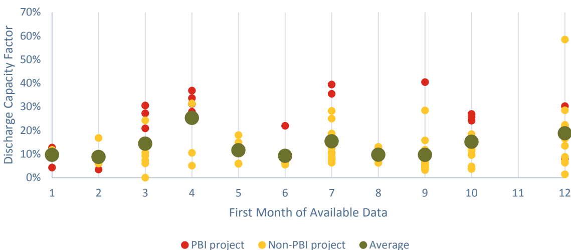
Figure 6-8: Non-residential AES Discharge Capacity Factor by Starting Month of Data, 2015
