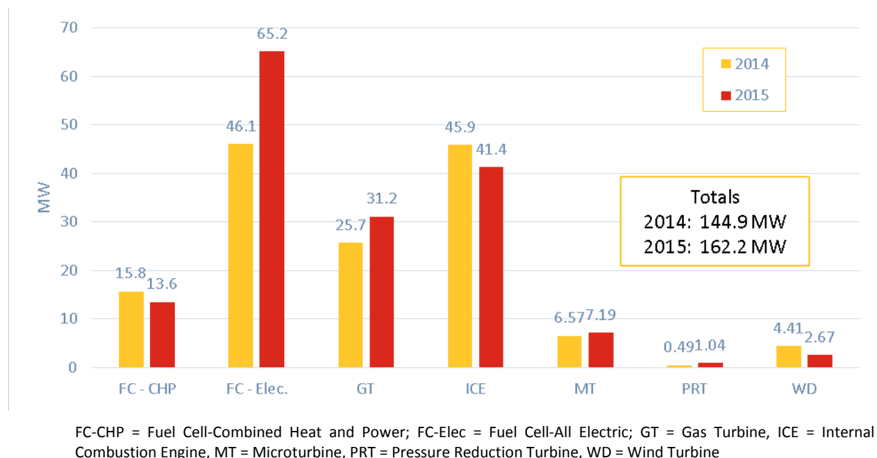
Figure 1-2: 2014 and 2015 CAISO Peak Hours Generation by Technology (MW)
