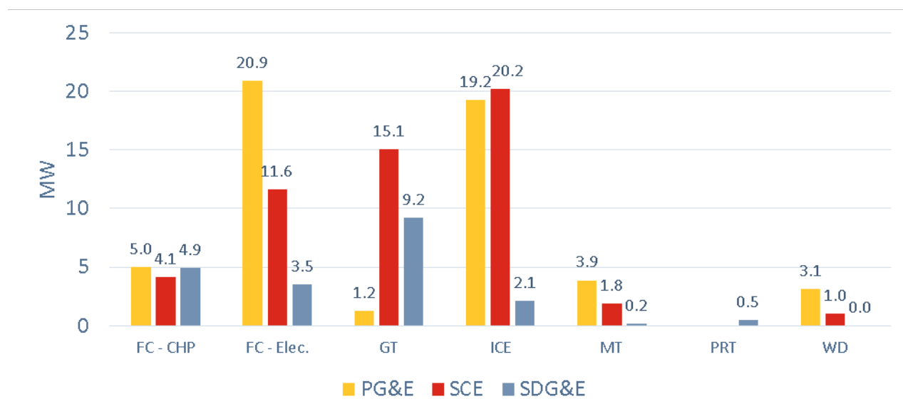
Figure 5-15: 2014 Peak Hour Generation by Technology
