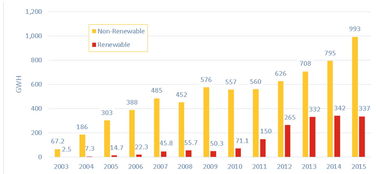
Figure 5-6: Annual Electric Generation by Fuel
