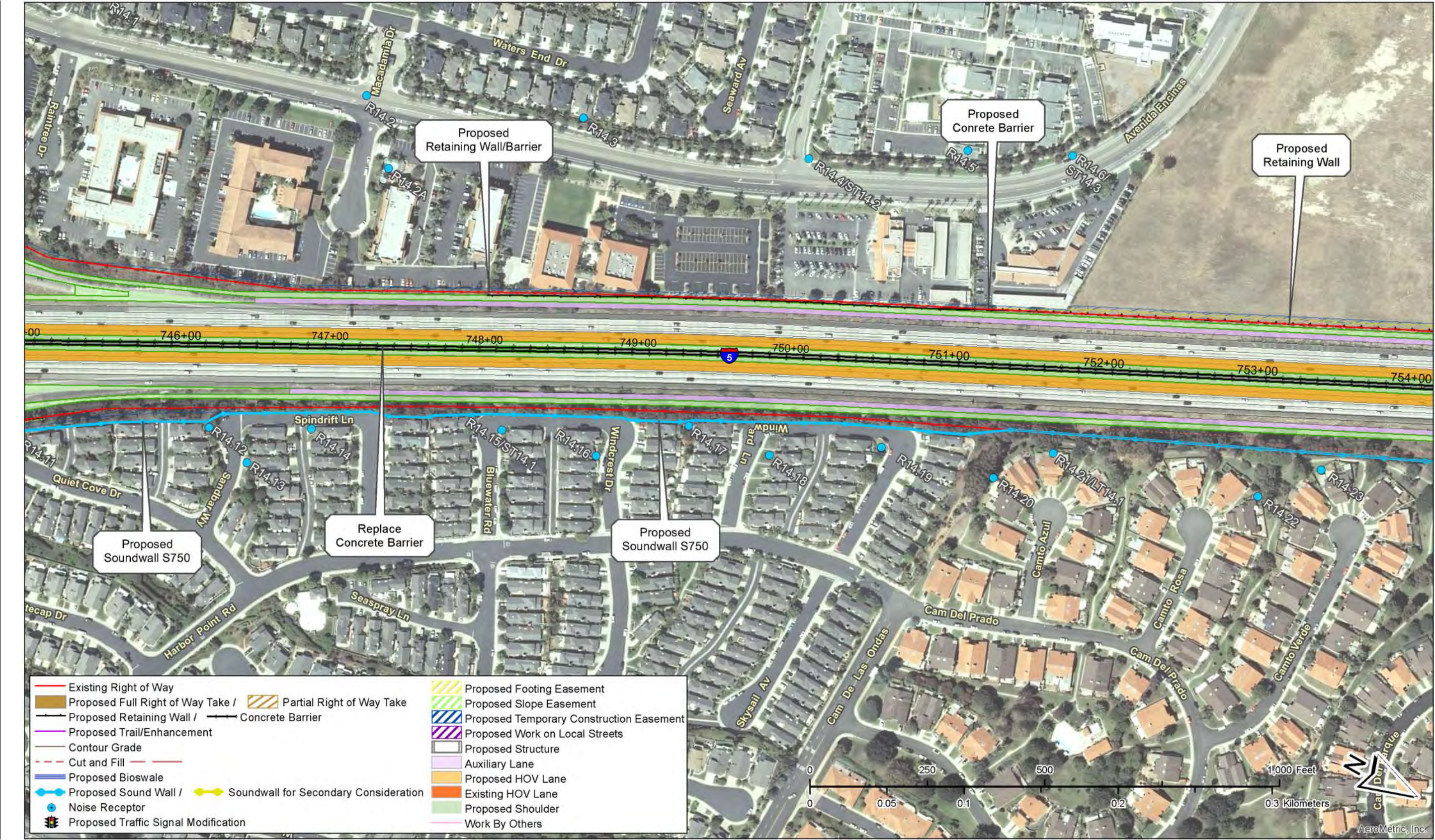
Figure 2-2.3, Sheet 44 of 67 – Project Features Map: 8+4 Buffer (Preferred Alternative) Soundwalls for secondary consideration are not part of the project. See Executive Summary (ES.5.15 Noise).
