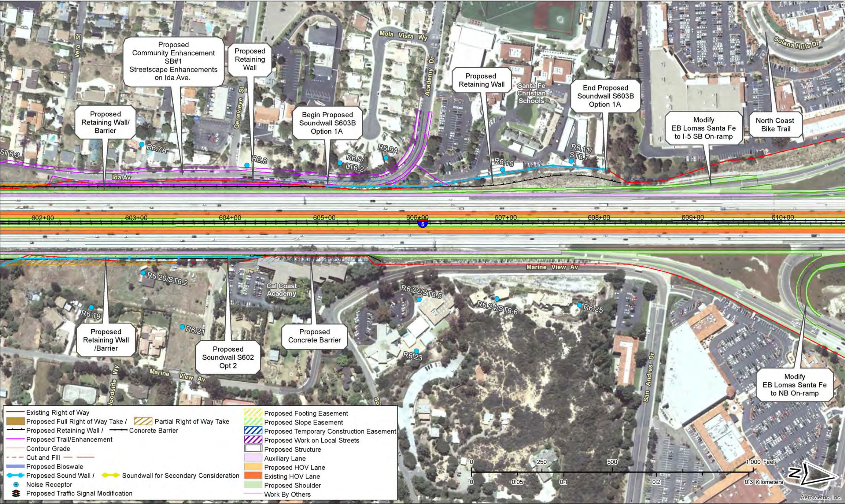
Figure 2-2.3, Sheet 22 of 67 – Project Features Map: 8+4 Buffer (Preferred Alternative) Soundwalls for secondary consideration are not part of the project. See Executive Summary (ES.5.15 Noise).
