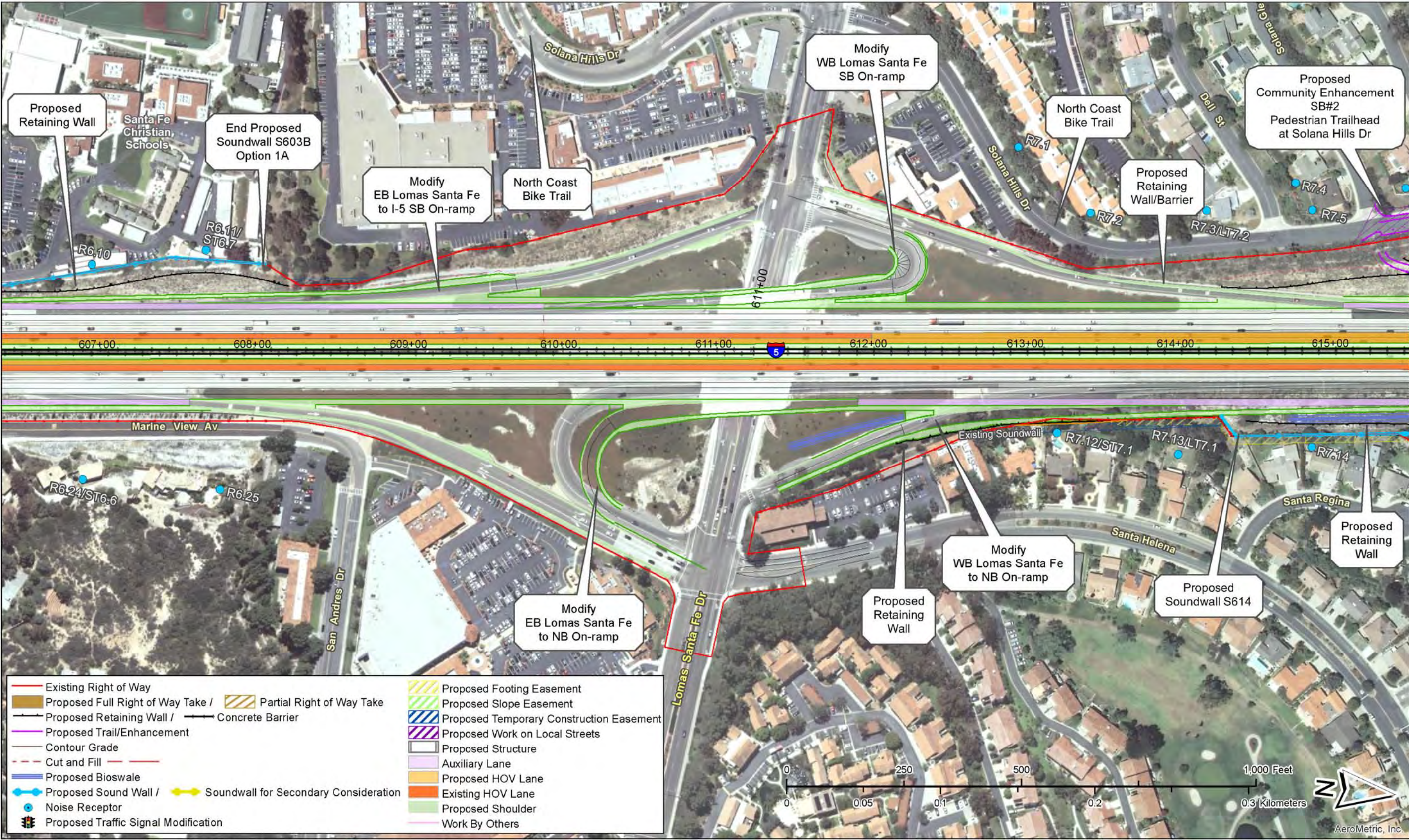
Figure 2-2.3, Sheet 23 of 67 – Project Features Map: 8+4 Buffer (Preferred Alternative) Soundwalls for secondary consideration are not part of the project. See Executive Summary (ES.5.15 Noise).
