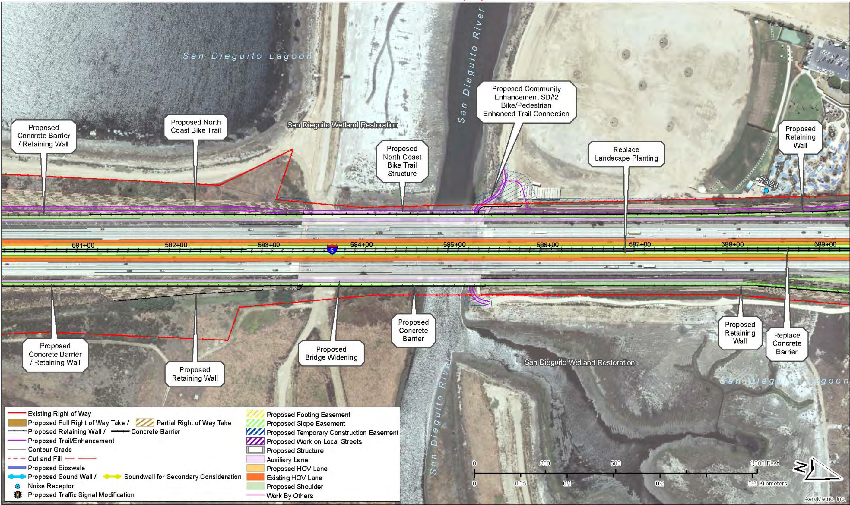
Figure 2-2.3, Sheet 19 of 67 – Project Features Map: 8+4 Buffer (Preferred Alternative) Soundwalls for secondary consideration are not part of the project. See Executive Summary (ES.5.15 Noise).
