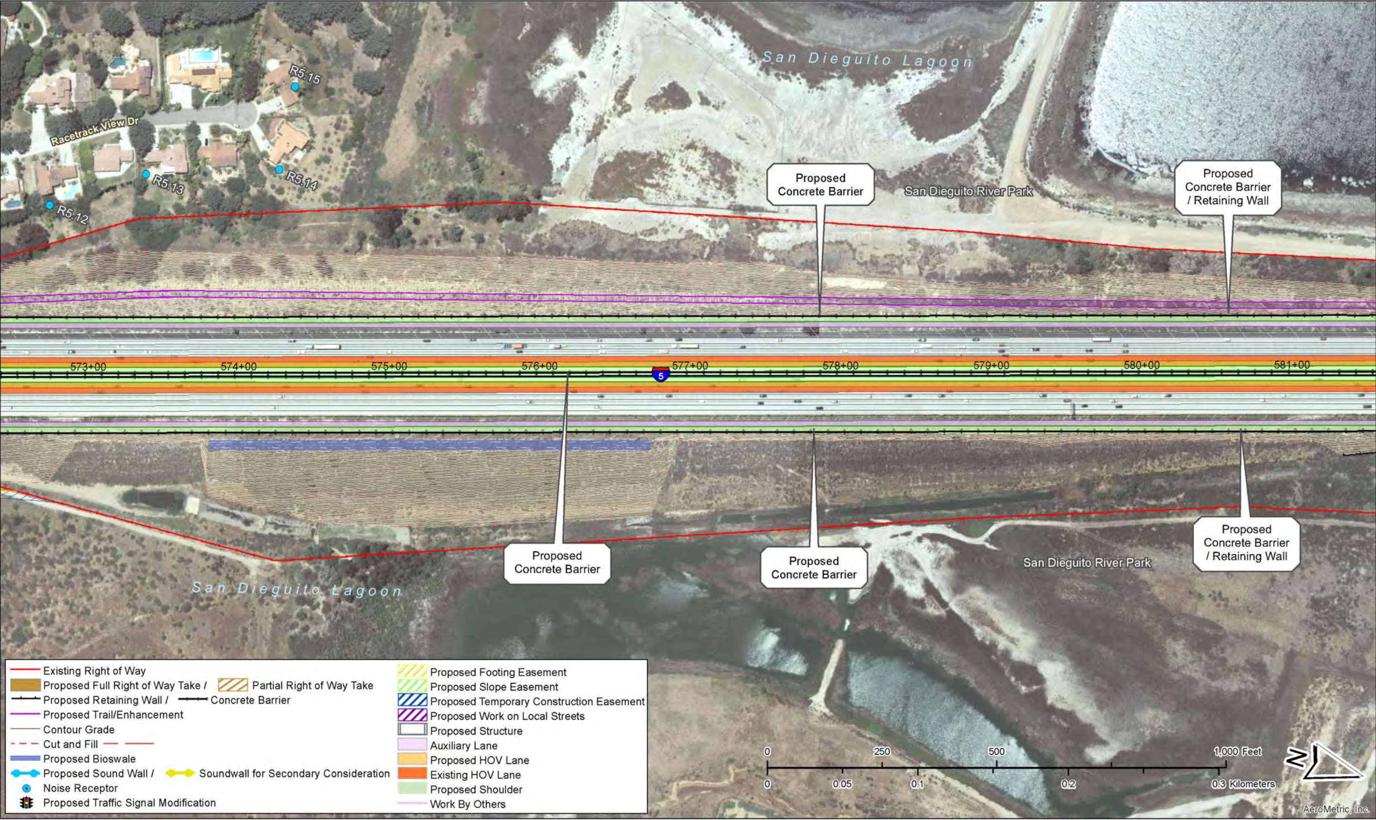
Figure 2-2.3, Sheet 18 of 67 – Project Features Map: 8+4 Buffer (Preferred Alternative) Soundwalls for secondary consideration are not part of the project. See Executive Summary (ES.5.15 Noise).
