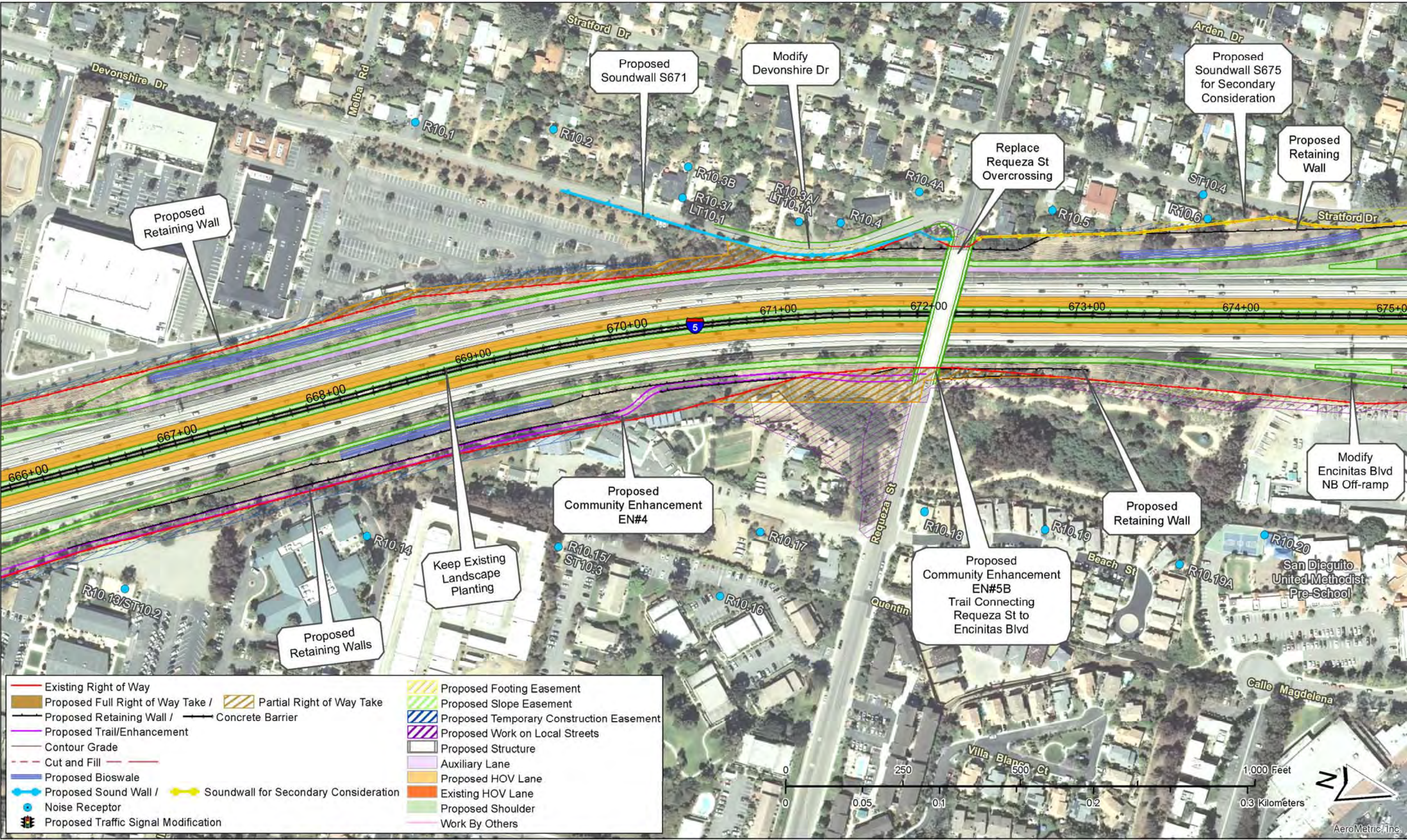
Figure 2-2.3, Sheet 33 of 67 – Project Features Map: 8+4 Buffer (Preferred Alternative) Soundwalls for secondary consideration are not part of the project. See Executive Summary (ES.5.15 Noise).
