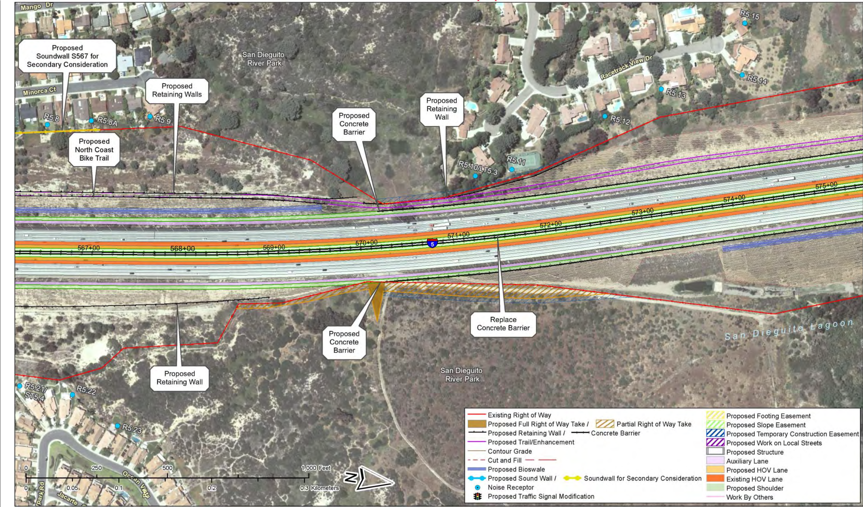
Figure 2-2.3, Sheet 17 of 67 – Project Features Map: 8+4 Buffer (Preferred Alternative) Soundwalls for secondary consideration are not part of the project. See Executive Summary (ES.5.15 Noise).
