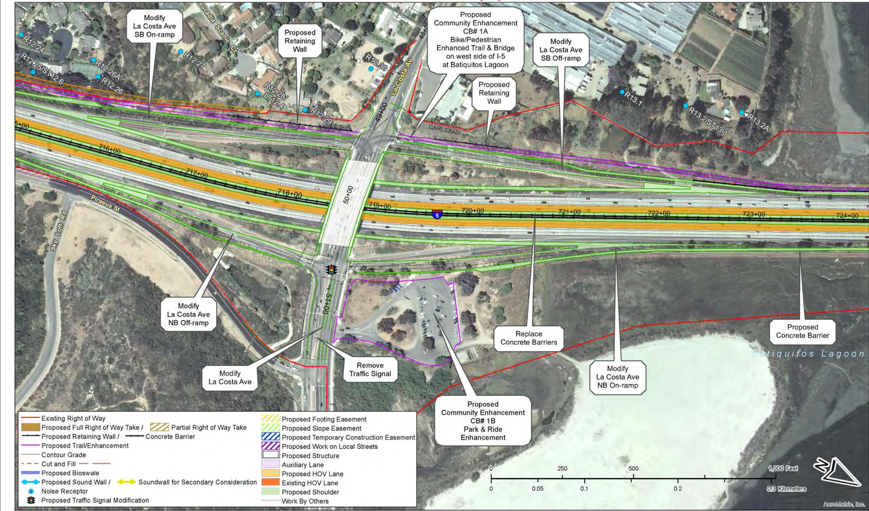
Figure 2-2.3, Sheet 40 of 67 – Project Features Map: 8+4 Buffer (Preferred Alternative) Soundwalls for secondary consideration are not part of the project. See Executive Summary (ES.5.15 Noise).
