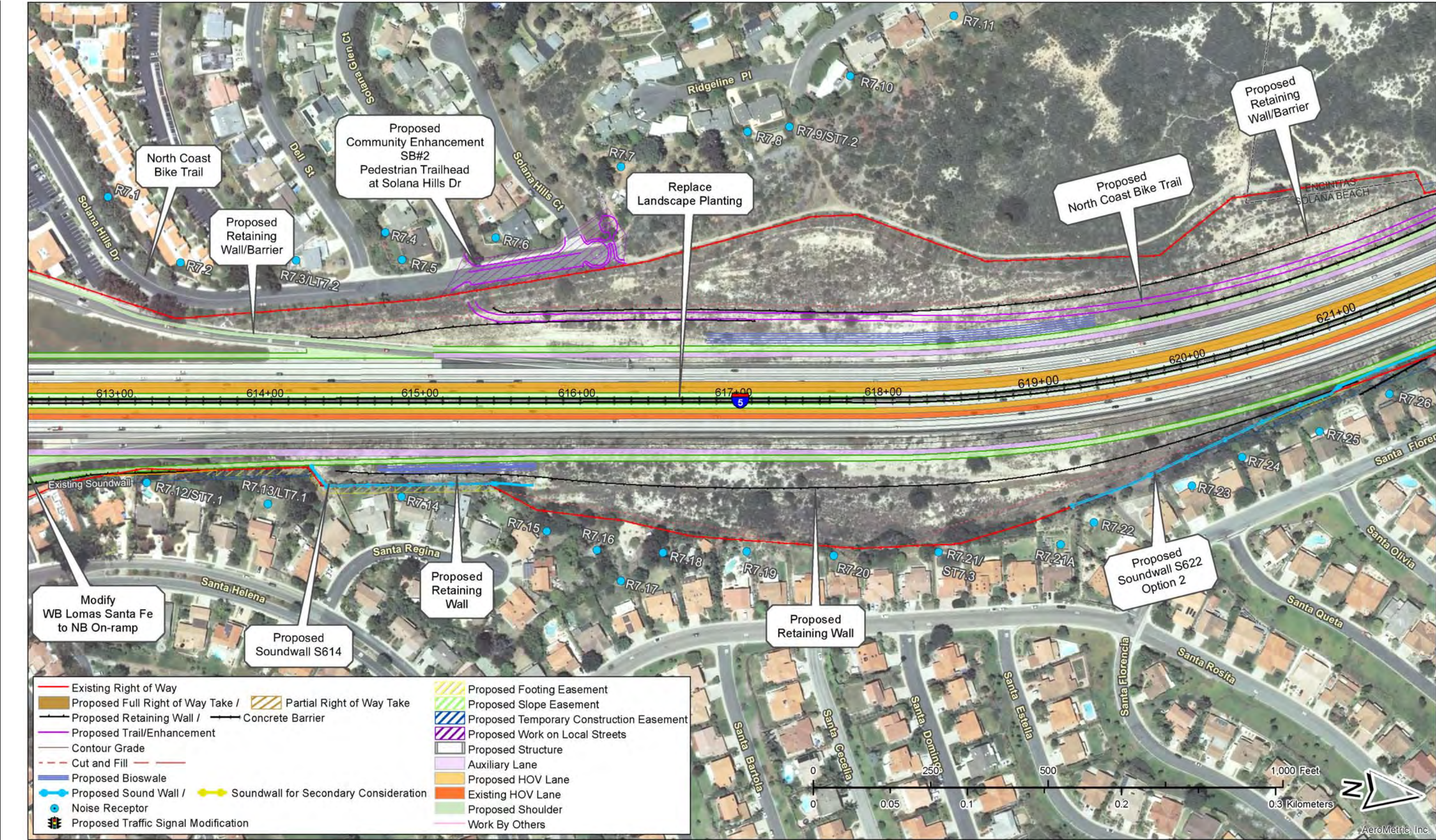
Figure 2-2.3, Sheet 24 of 67 – Project Features Map: 8+4 Buffer (Preferred Alternative) Soundwalls for secondary consideration are not part of the project. See Executive Summary (ES.5.15 Noise).
