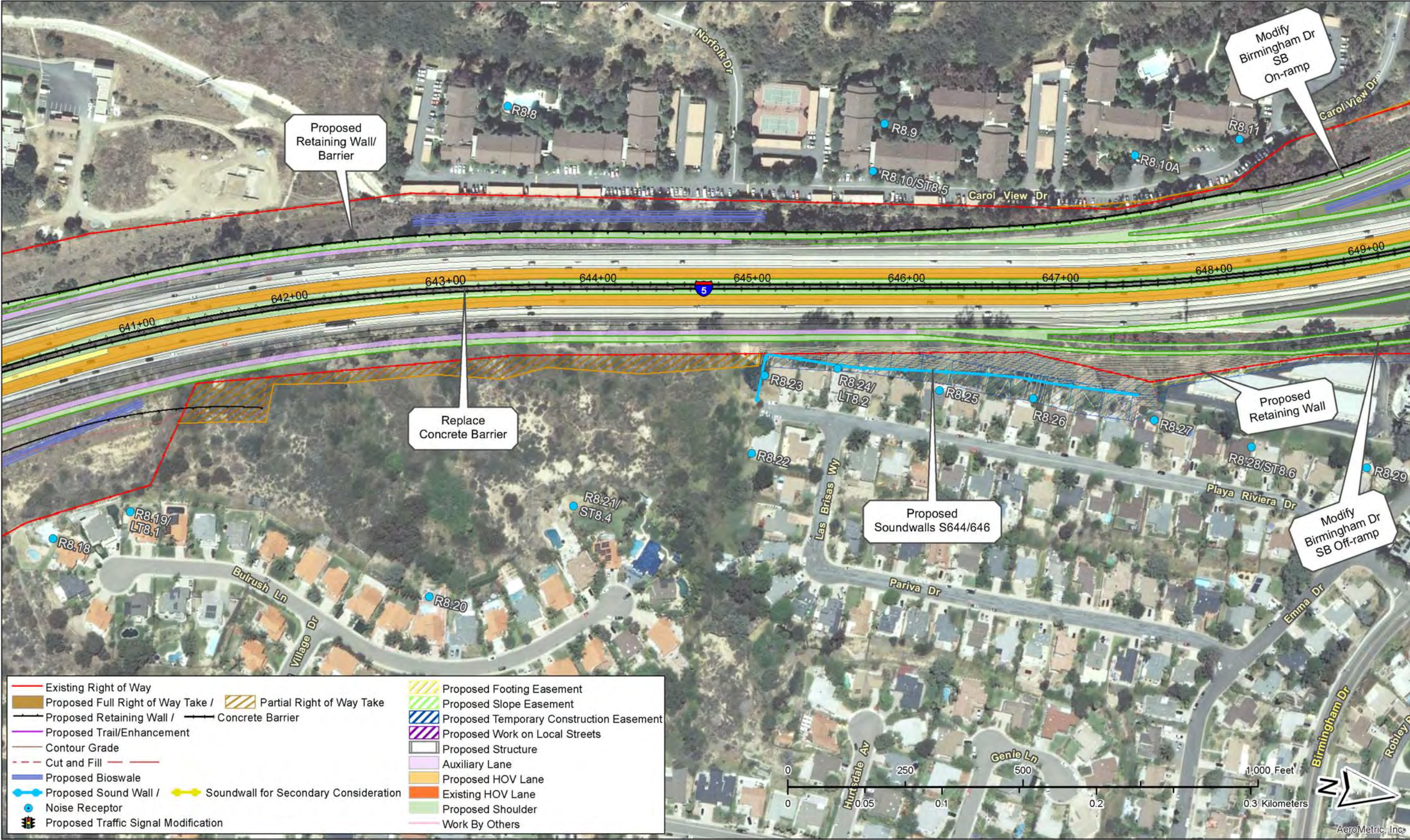
Figure 2-2.3, Sheet 29 of 67 – Project Features Map: 8+4 Buffer (Preferred Alternative) Soundwalls for secondary consideration are not part of the project. See Executive Summary (ES.5.15 Noise).
