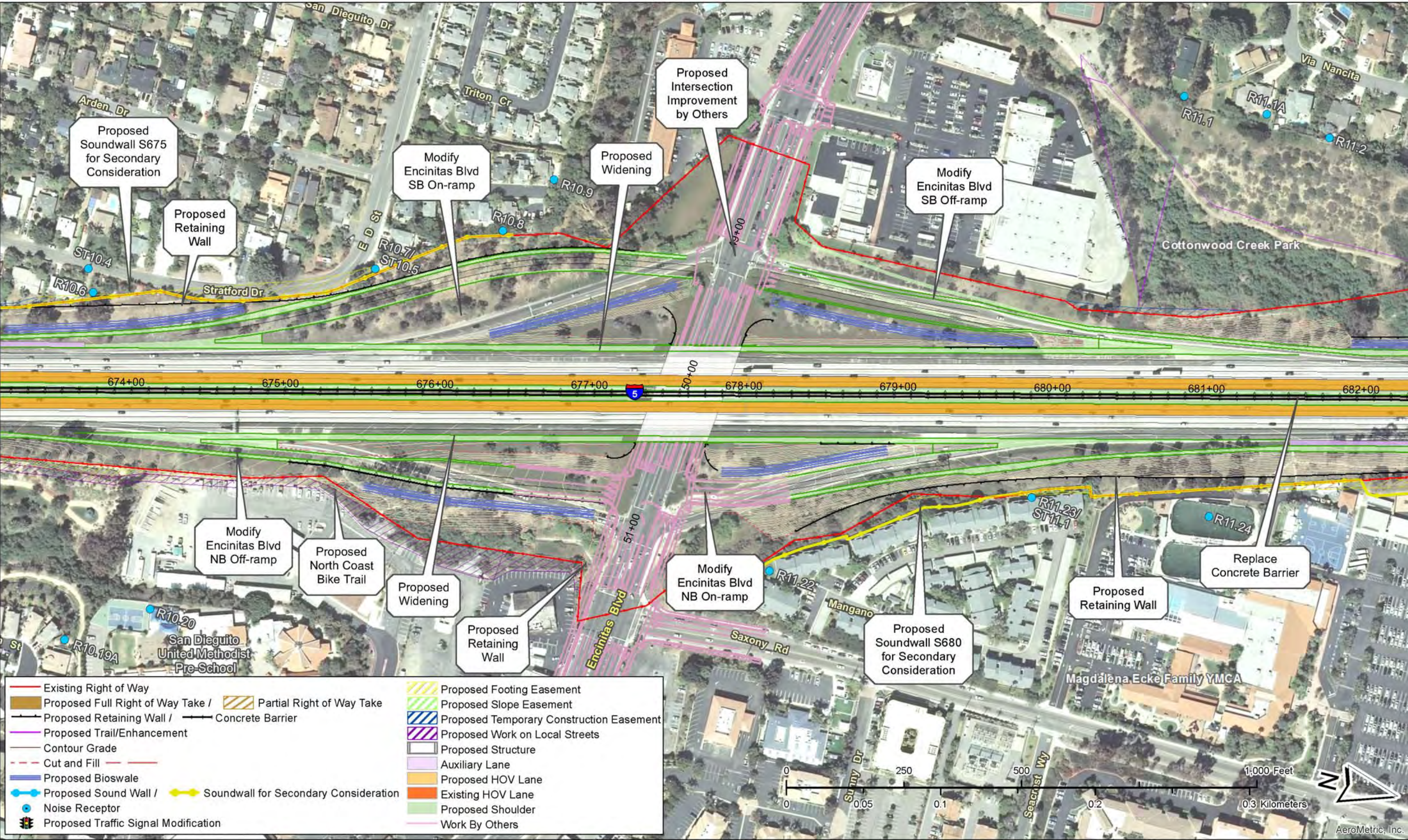
Figure 2-2.3, Sheet 34 of 67 – Project Features Map: 8+4 Buffer (Preferred Alternative) Soundwalls for secondary consideration are not part of the project. See Executive Summary (ES.5.15 Noise).
