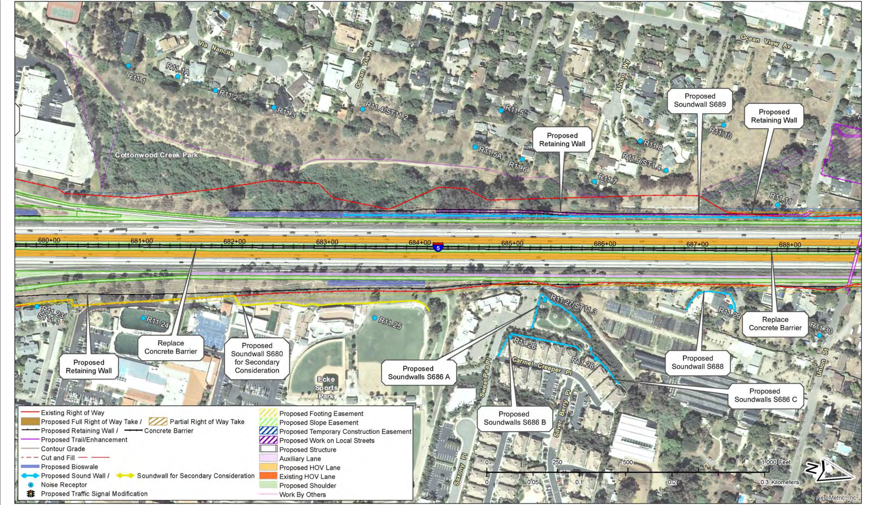
Figure 2-2.3, Sheet 35 of 67 – Project Features Map: 8+4 Buffer (Preferred Alternative) Soundwalls for secondary consideration are not part of the project. See Executive Summary (ES.5.15 Noise).
