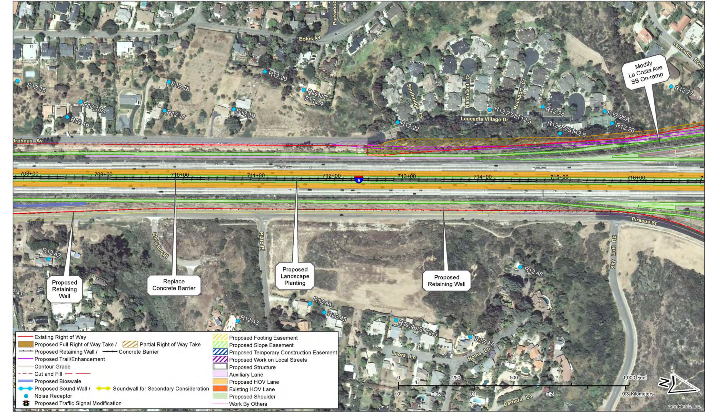
Figure 2-2.3, Sheet 39 of 67 – Project Features Map: 8+4 Buffer (Preferred Alternative) Soundwalls for secondary consideration are not part of the project. See Executive Summary (ES.5.15 Noise).
