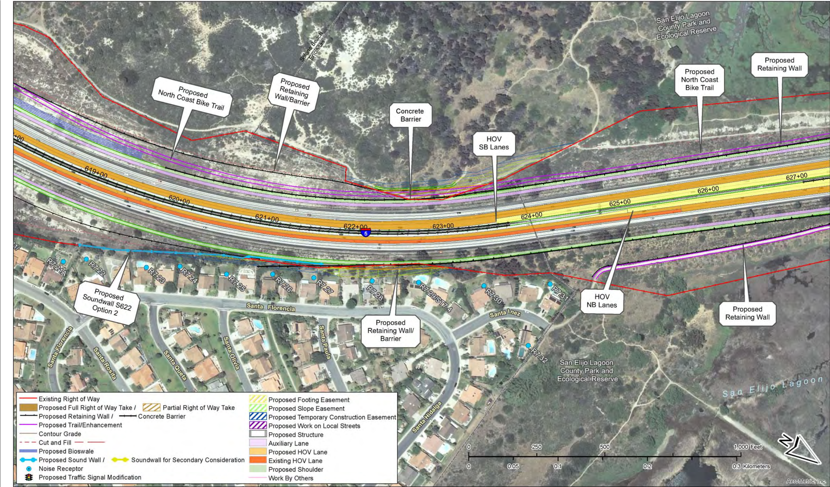
Figure 2-2.3, Sheet 25 of 67 – Project Features Map: 8+4 Buffer (Preferred Alternative) Soundwalls for secondary consideration are not part of the project. See Executive Summary (ES.5.15 Noise).
