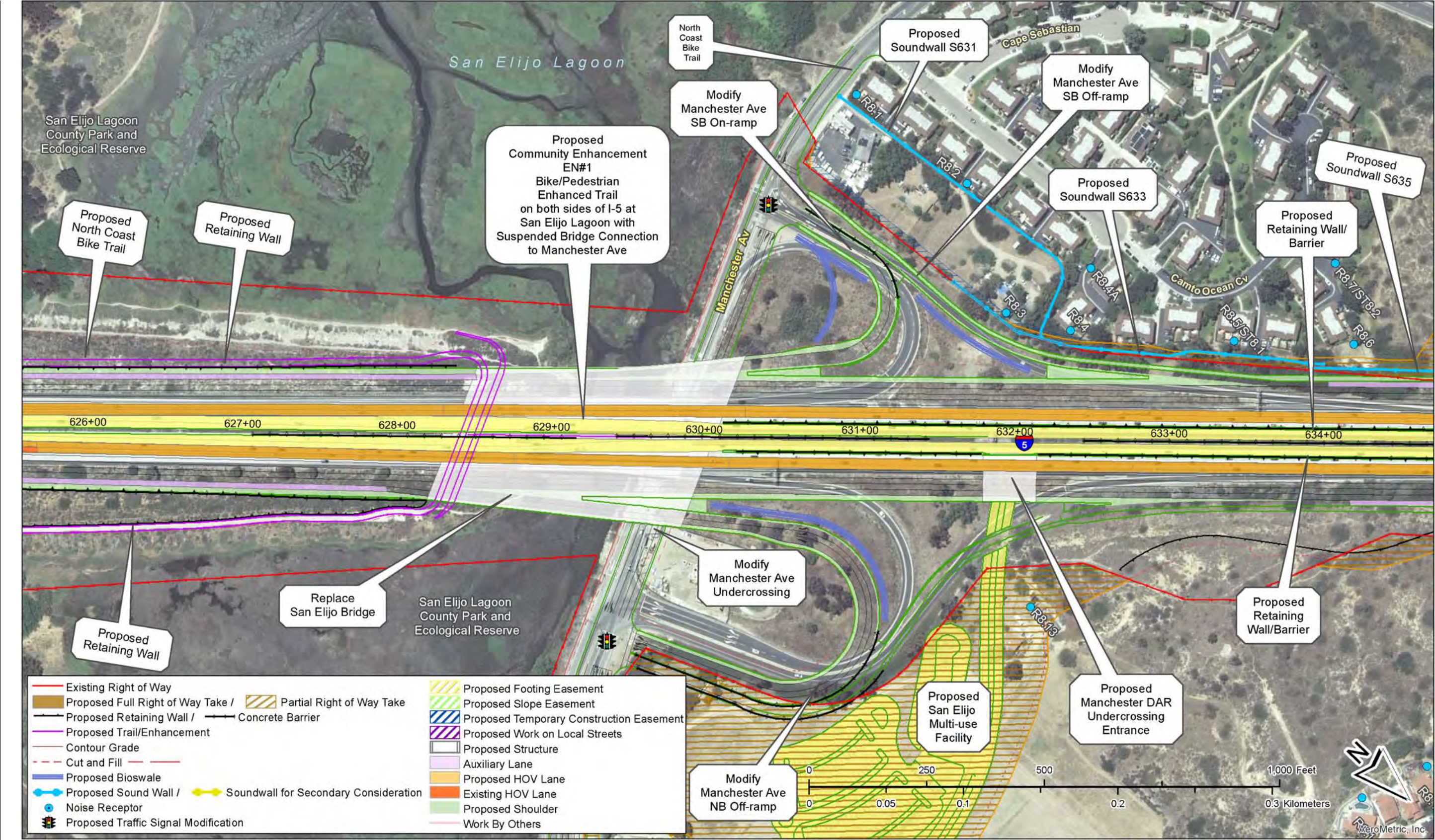
Figure 2-2.3, Sheet 26 of 67 – Project Features Map: 8+4 Buffer (Preferred Alternative) Soundwalls for secondary consideration are not part of the project. See Executive Summary (ES.5.15 Noise).
