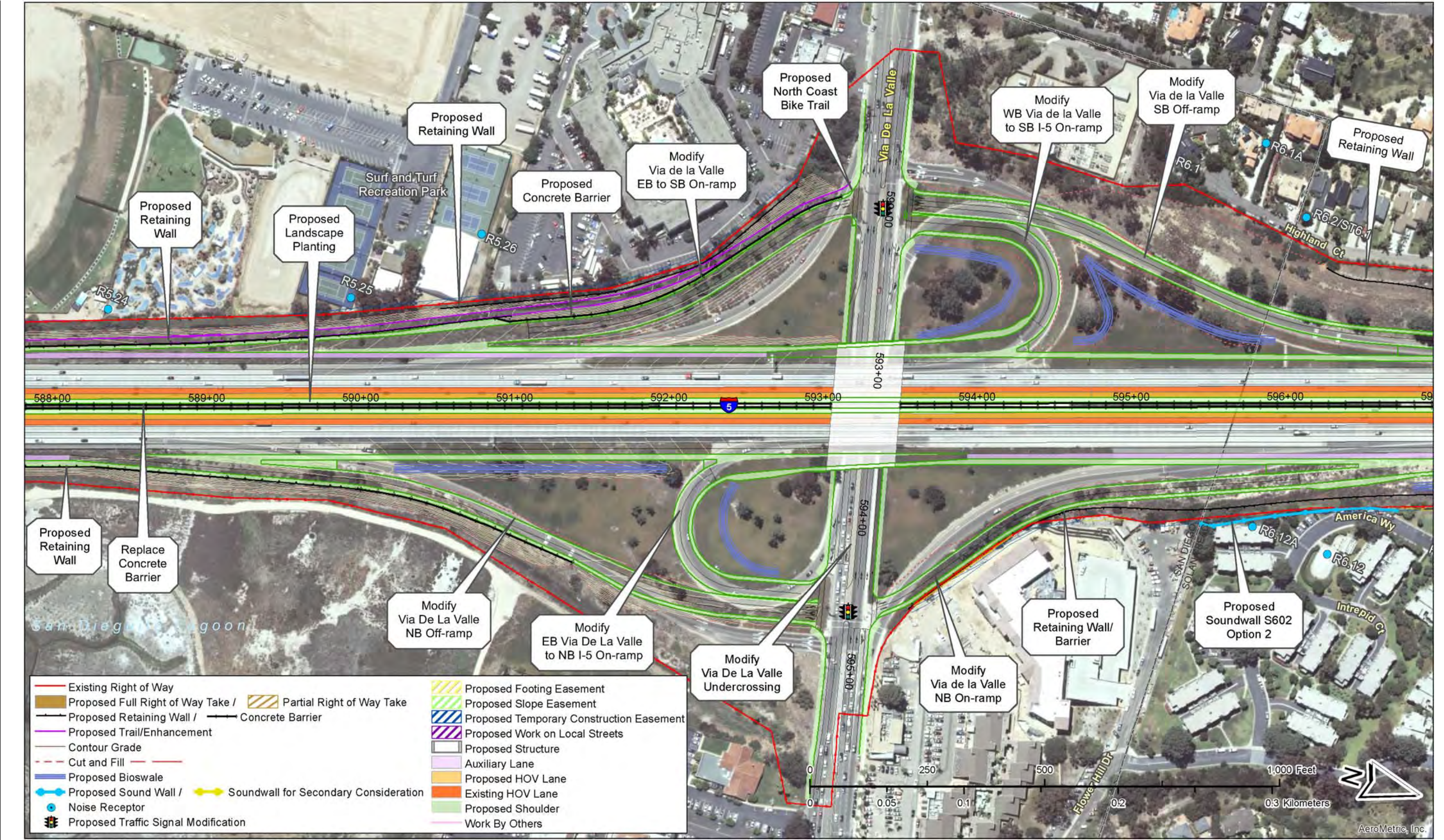
Figure 2-2.3, Sheet 20 of 67 – Project Features Map: 8+4 Buffer (Preferred Alternative) Soundwalls for secondary consideration are not part of the project. See Executive Summary (ES.5.15 Noise).
