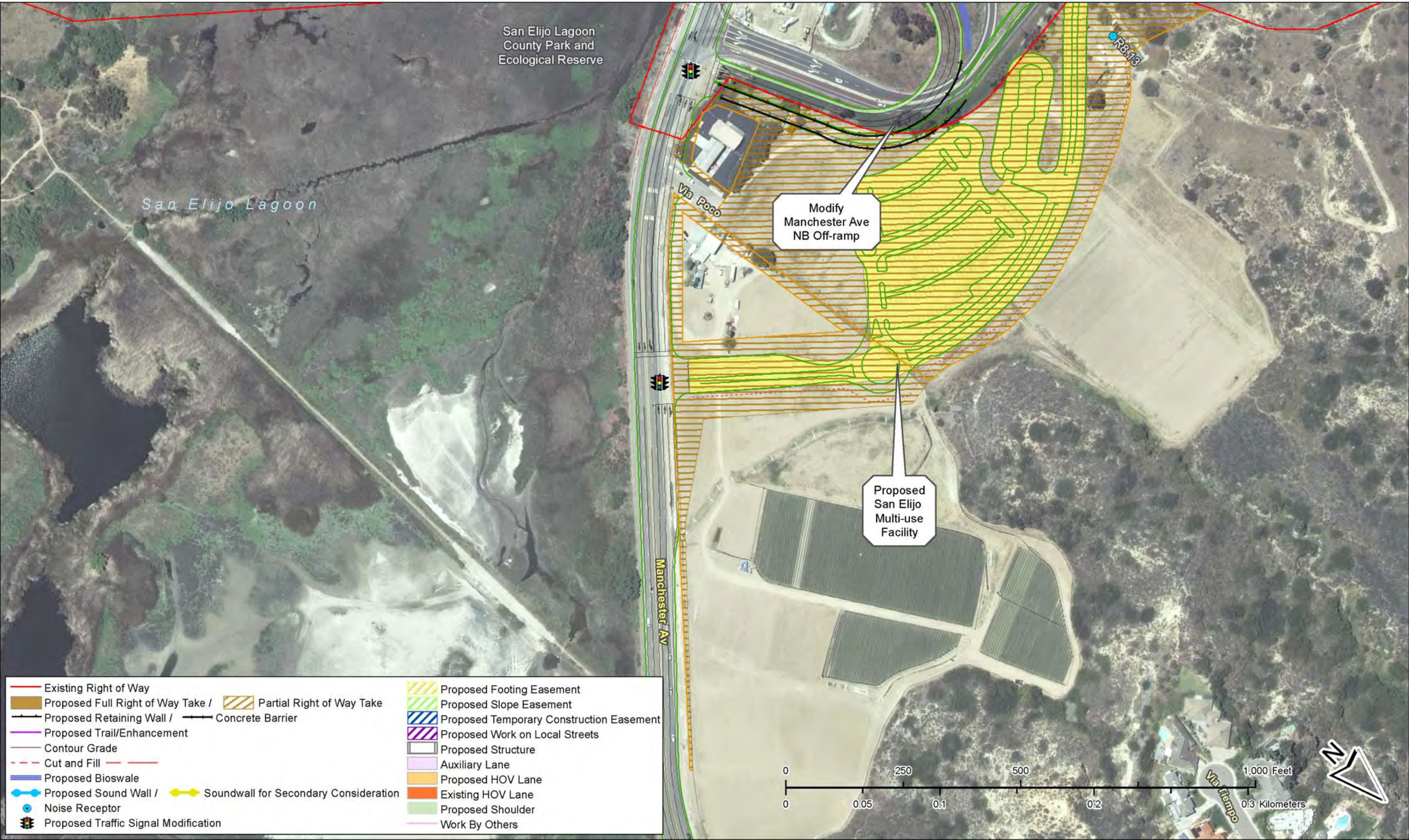
Figure 2-2.3, Sheet 27 of 67 – Project Features Map: 8+4 Buffer (Preferred Alternative) Soundwalls for secondary consideration are not part of the project. See Executive Summary (ES.5.15 Noise).
