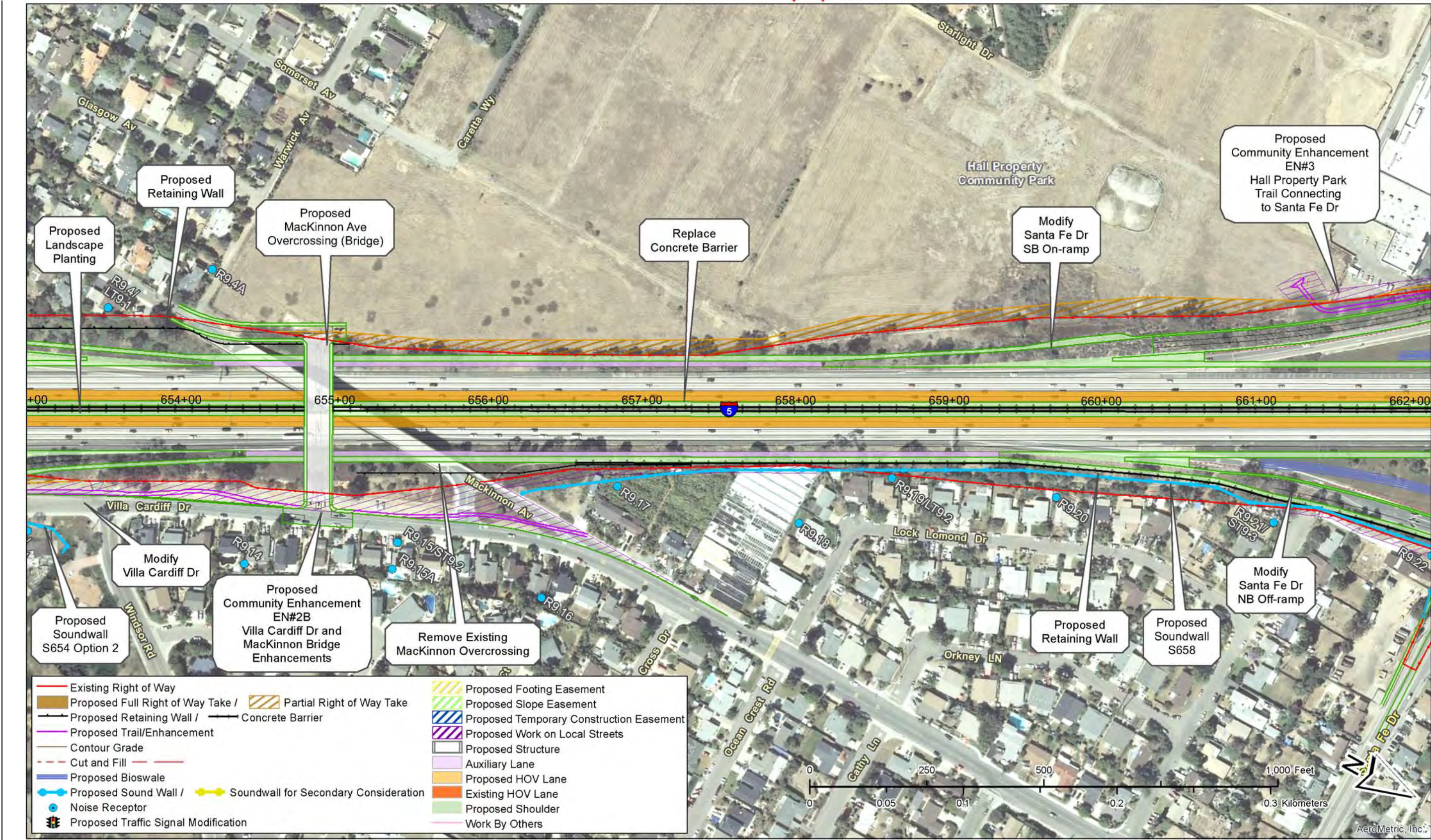
Figure 2-2.3, Sheet 31 of 67 – Project Features Map: 8+4 Buffer (Preferred Alternative) Soundwalls for secondary consideration are not part of the project. See Executive Summary (ES.5.15 Noise).
