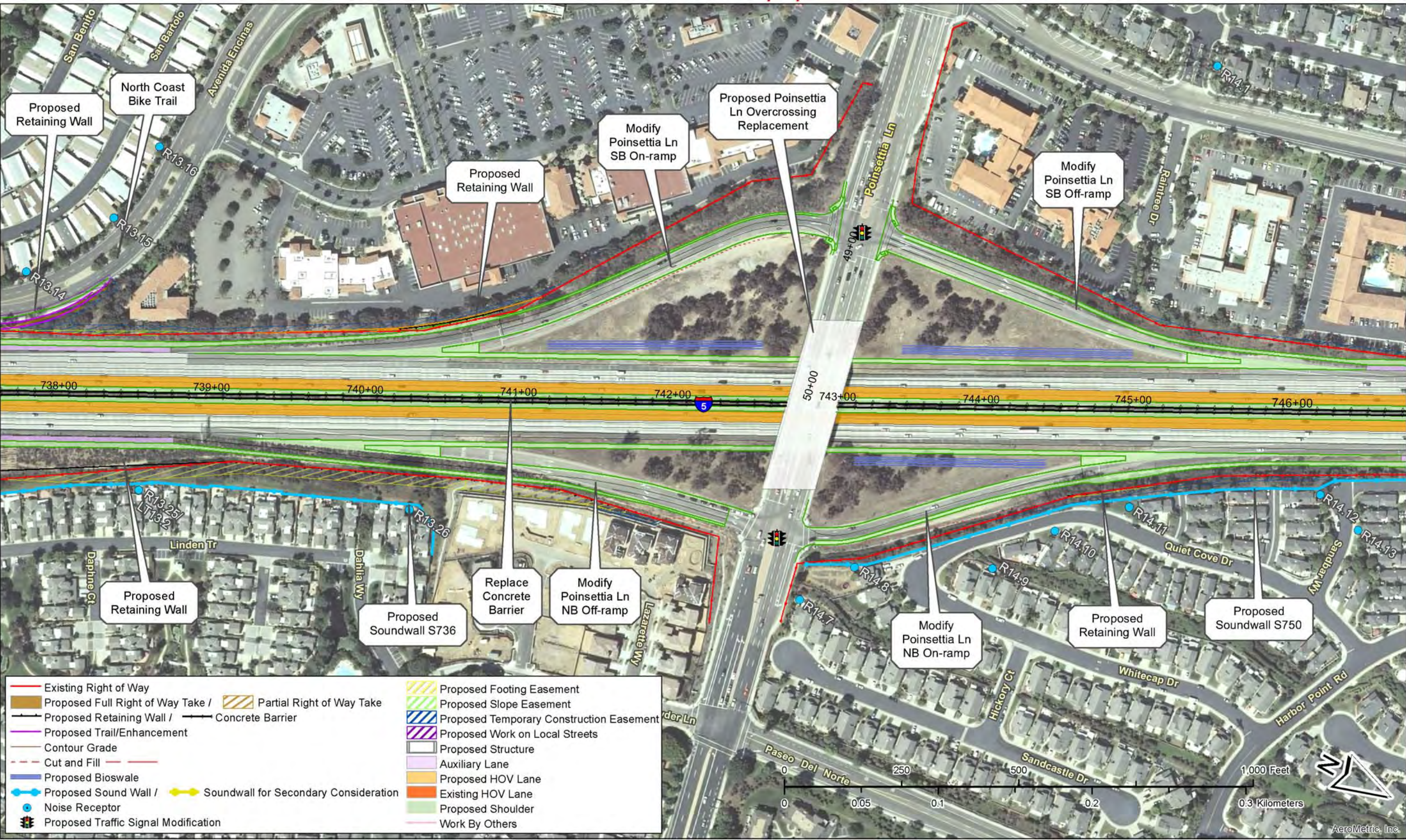
Figure 2-2.3, Sheet 43 of 67 – Project Features Map: 8+4 Buffer (Preferred Alternative) Soundwalls for secondary consideration are not part of the project. See Executive Summary (ES.5.15 Noise).
