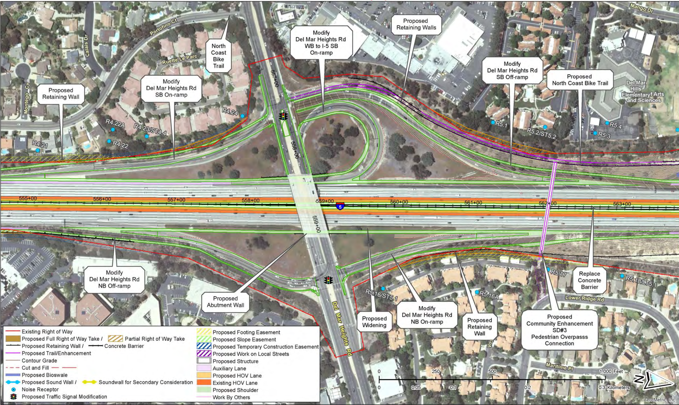
Figure 2-2.3, Sheet 15 of 67 – Project Features Map: 8+4 Buffer (Preferred Alternative) Soundwalls for secondary consideration are not part of the project. See Executive Summary (ES.5.15 Noise).
