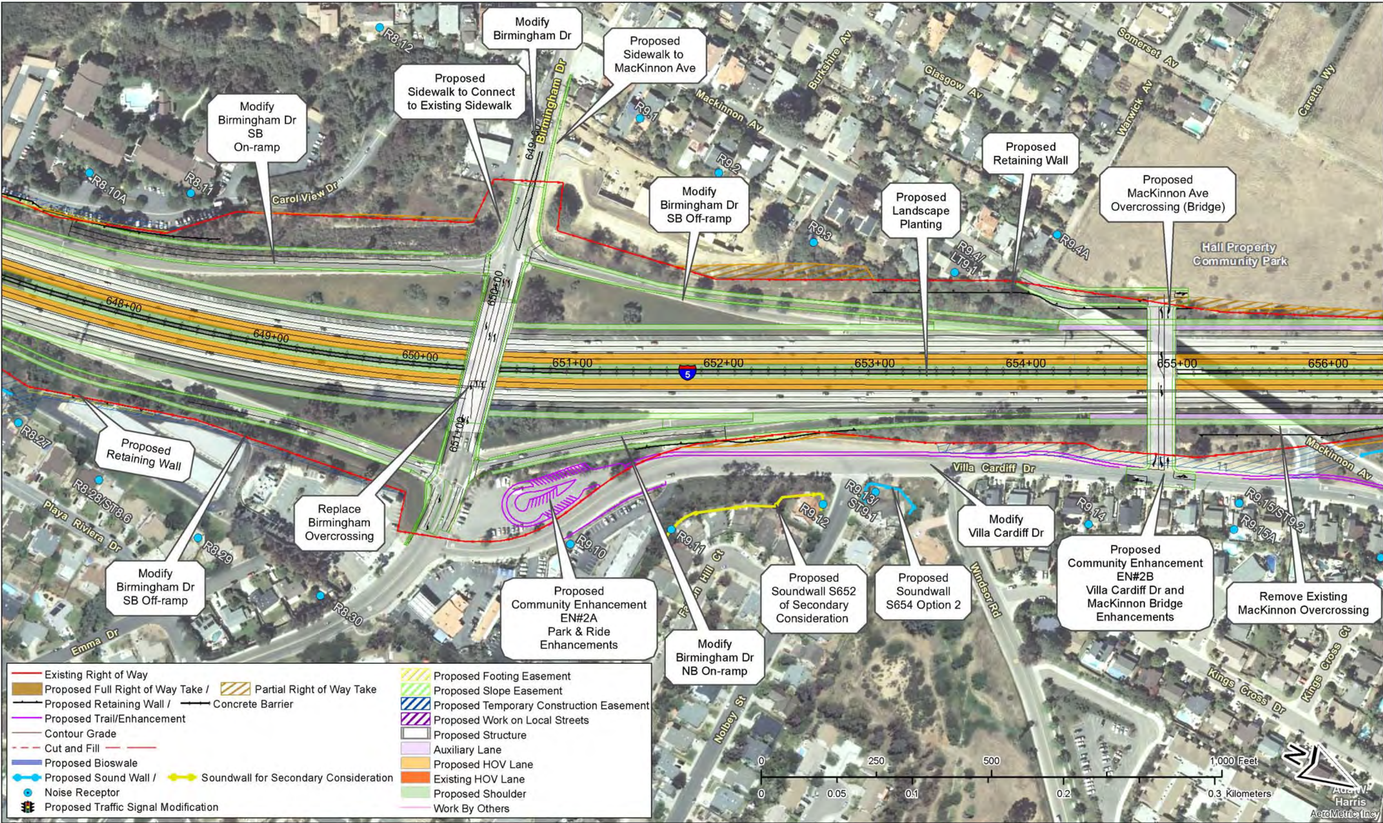
Figure 2-2.3, Sheet 30a of 67 – Project Features Map: 8+4 Buffer (Preferred Alternative) Soundwalls for secondary consideration are not part of the project. See Executive Summary (ES.5.15 Noise).
