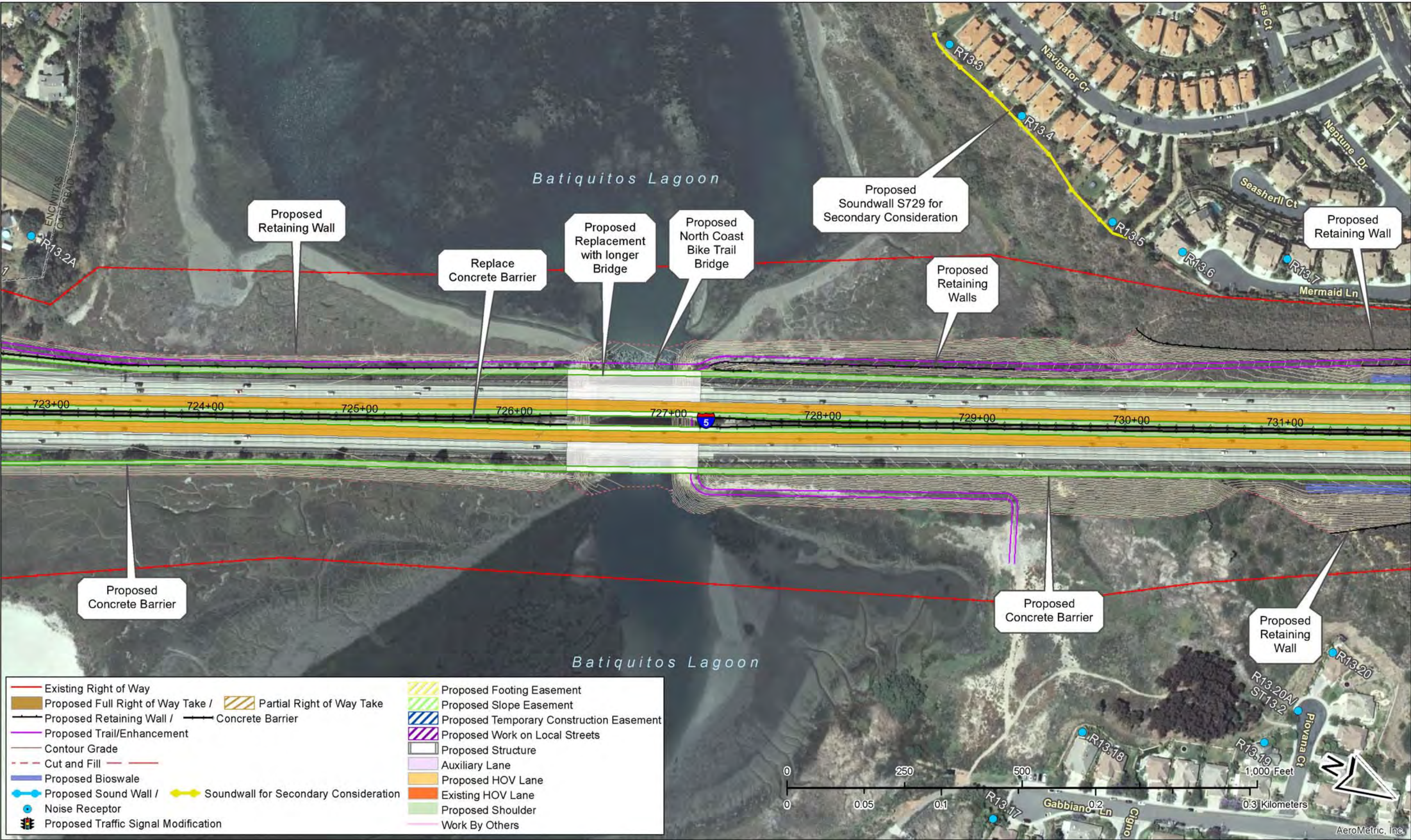
Figure 2-2.3, Sheet 41 of 67 – Project Features Map: 8+4 Buffer (Preferred Alternative) Soundwalls for secondary consideration are not part of the project. See Executive Summary (ES.5.15 Noise).
