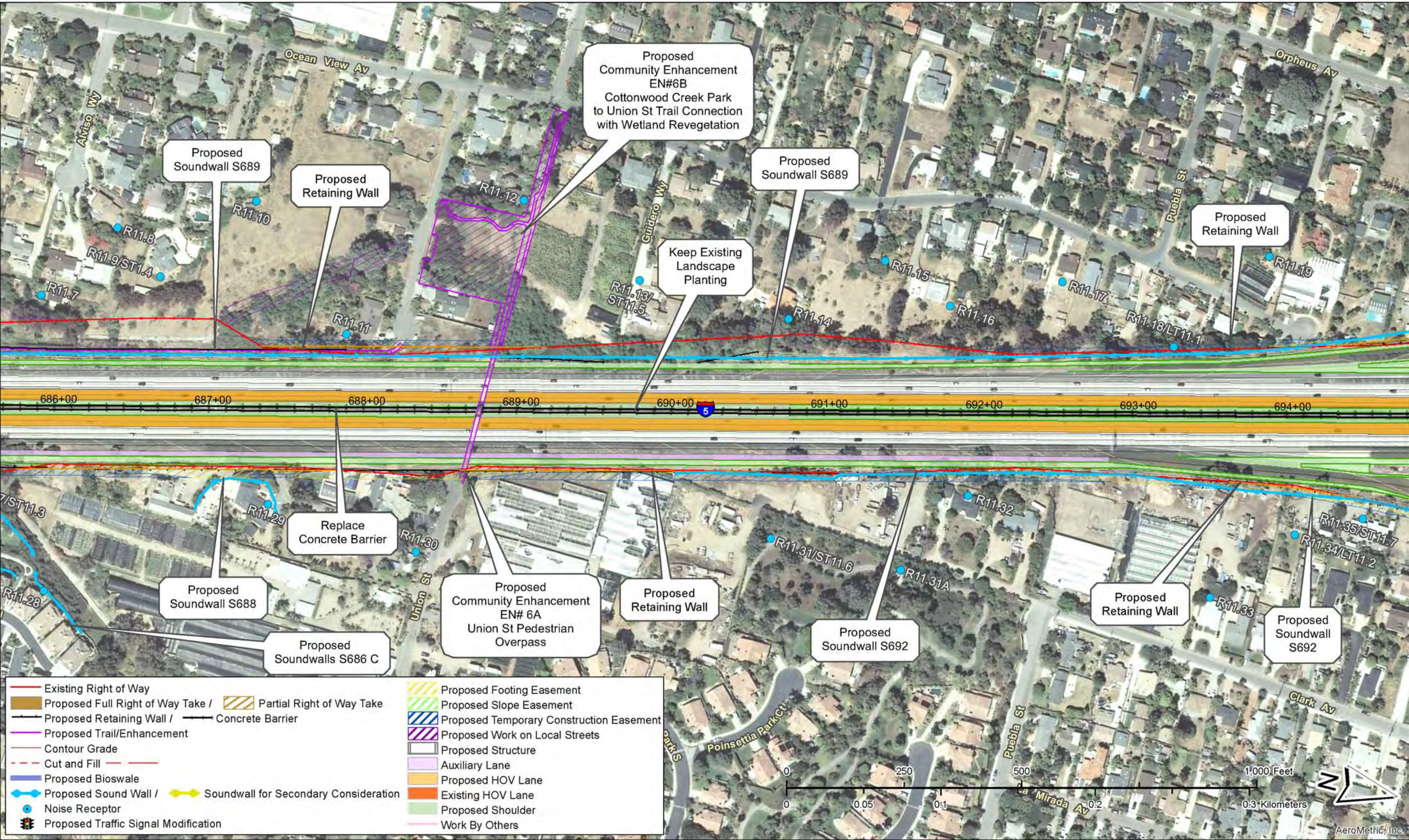
Figure 2-2.3, Sheet 36 of 67 – Project Features Map: 8+4 Buffer (Preferred Alternative) Soundwalls for secondary consideration are not part of the project. See Executive Summary (ES.5.15 Noise).
