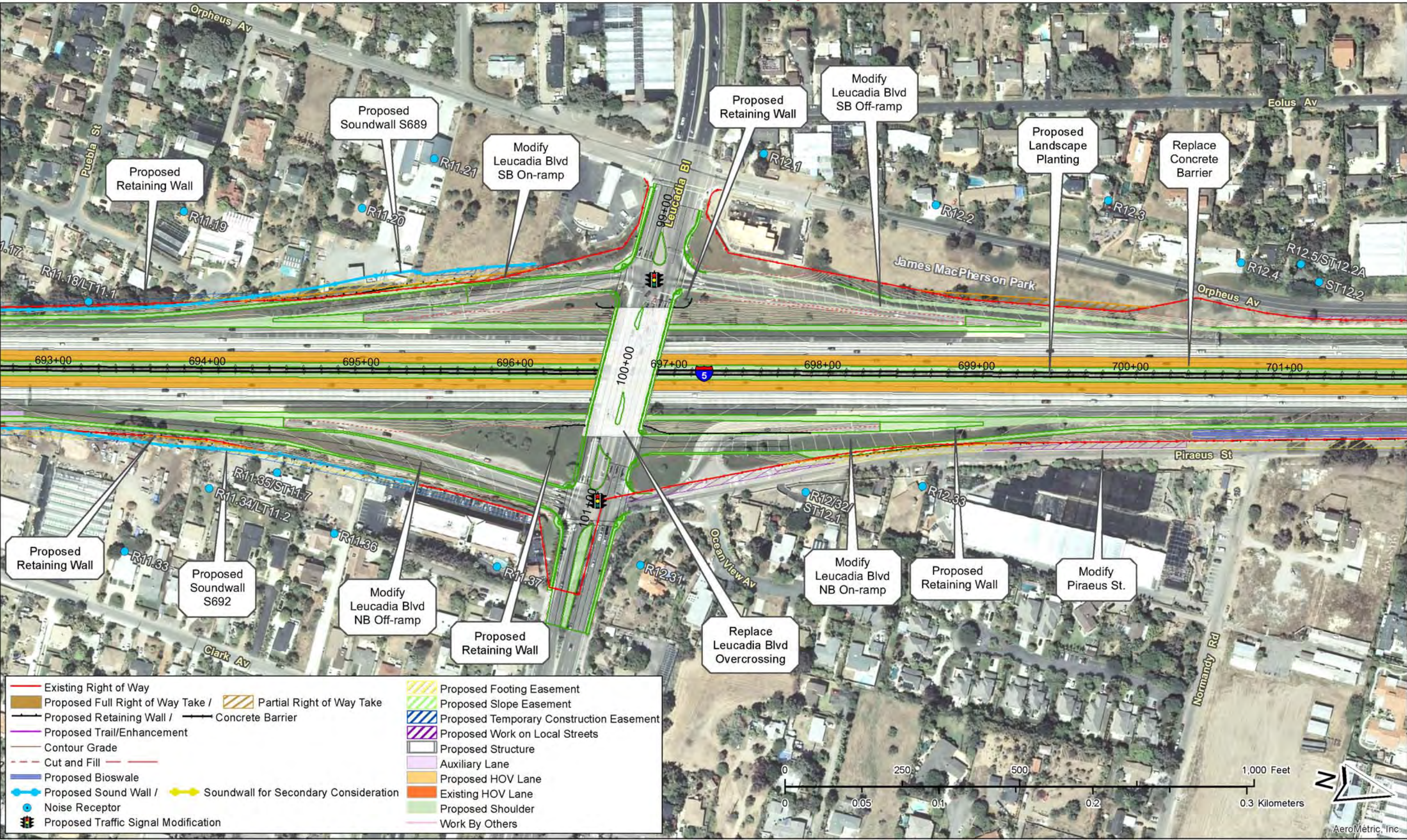
Figure 2-2.3, Sheet 37 of 67 – Project Features Map: 8+4 Buffer (Preferred Alternative) Soundwalls for secondary consideration are not part of the project. See Executive Summary (ES.5.15 Noise).
