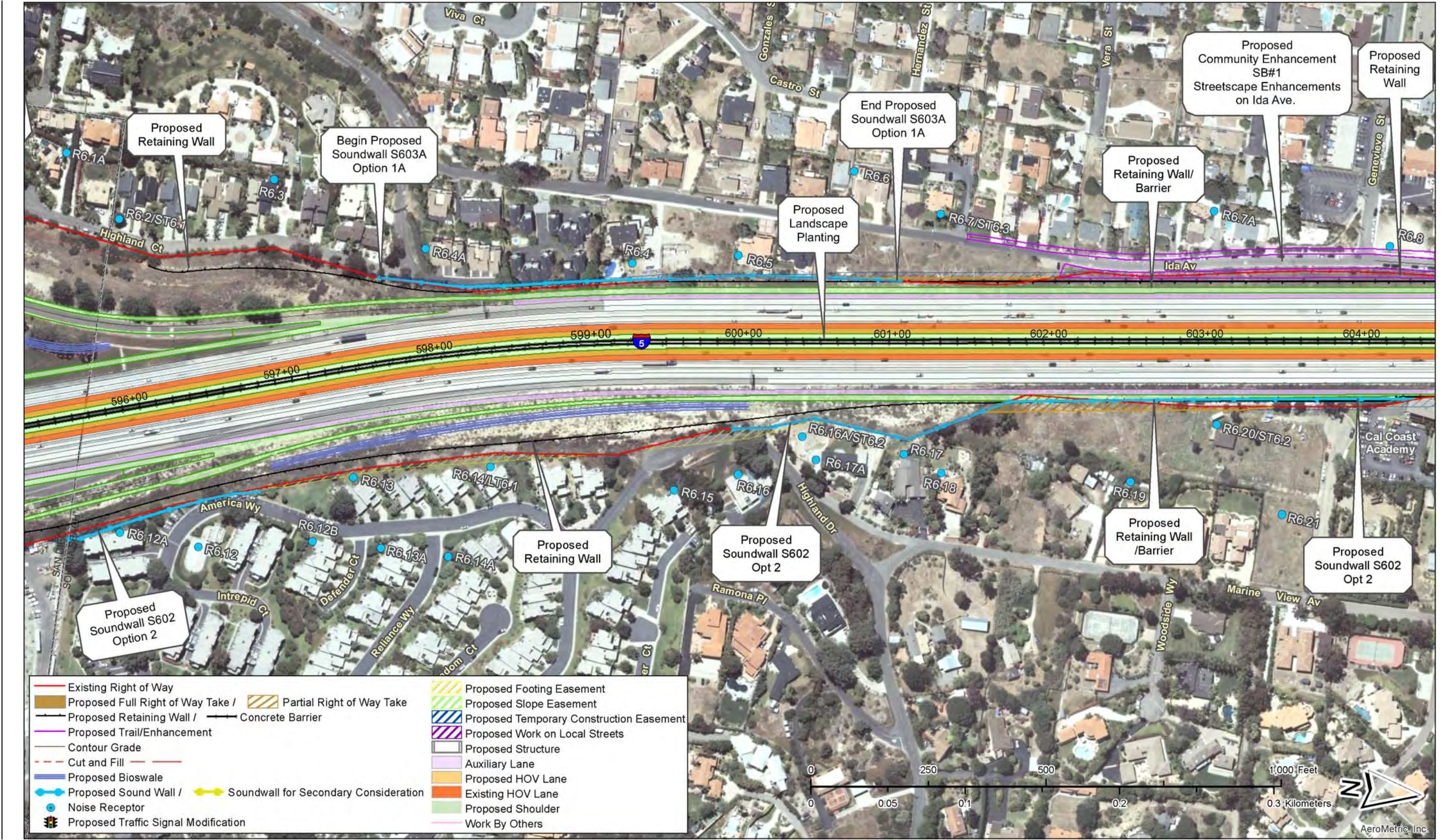
Figure 2-2.3, Sheet 21 of 67 – Project Features Map: 8+4 Buffer (Preferred Alternative) Soundwalls for secondary consideration are not part of the project. See Executive Summary (ES.5.15 Noise).
