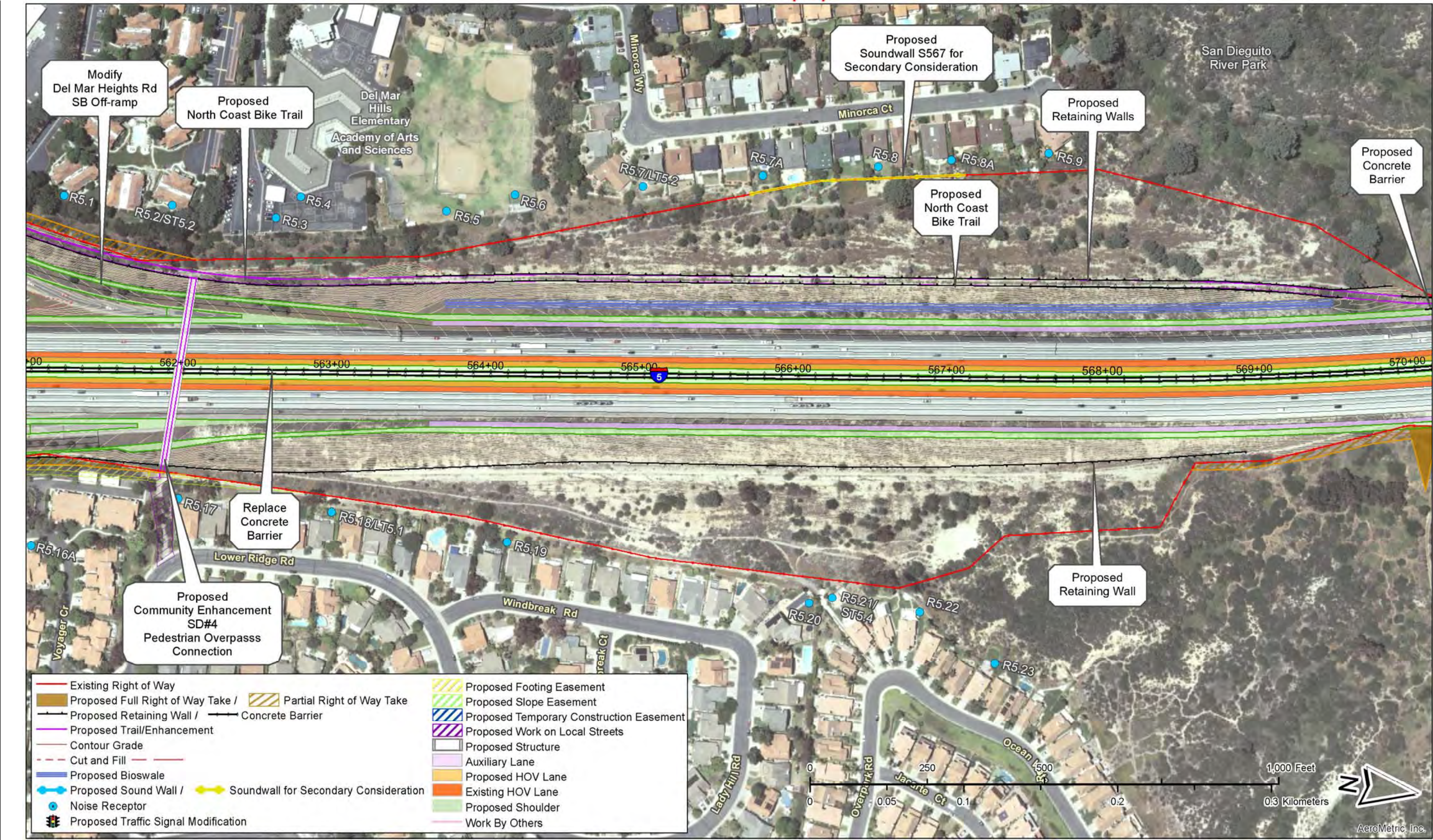
Figure 2-2.3, Sheet 16 of 67 – Project Features Map: 8+4 Buffer (Preferred Alternative) Soundwalls for secondary consideration are not part of the project. See Executive Summary (ES.5.15 Noise).
