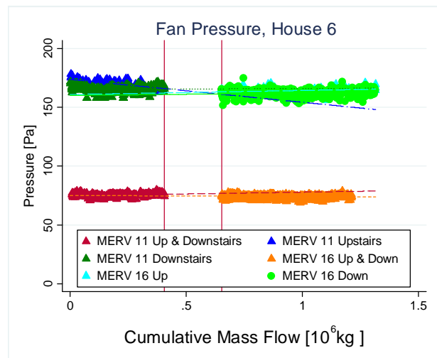
Figure 53: Pressure Across the Fan for House 6
