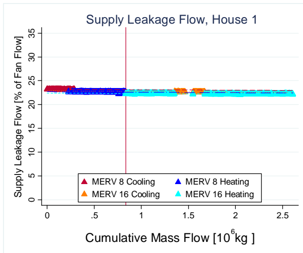
Figure 10: Supply Side Leakage for House 1
