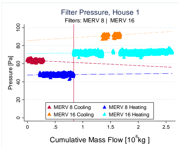
Figure 6: Pressure Across the Filter for House 1
