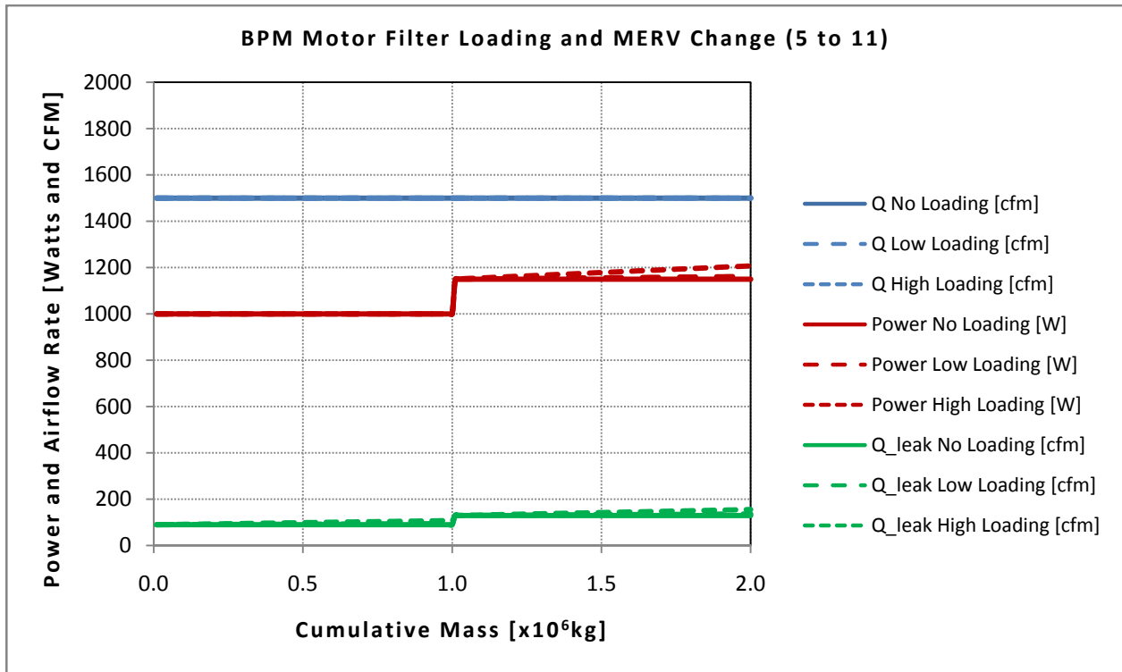
Figure 99: Filter Loading Effects on System Performance for A BPM Motor under No, Low and High Loading Conditions, with a Change in Filter from MERV 5 to MERV 11 after 106 Kg of Cumulative Air Mass Flow
