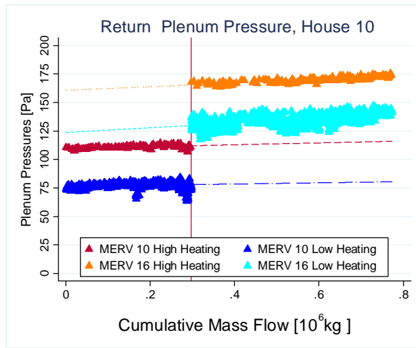
Figure 93: Return Plenum Pressure (relative to inside the house) for House 10
