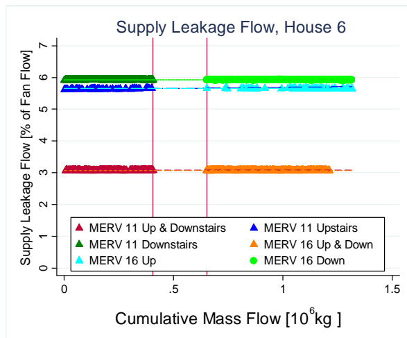
Figure 56: Supply Side Leakage for House 6
