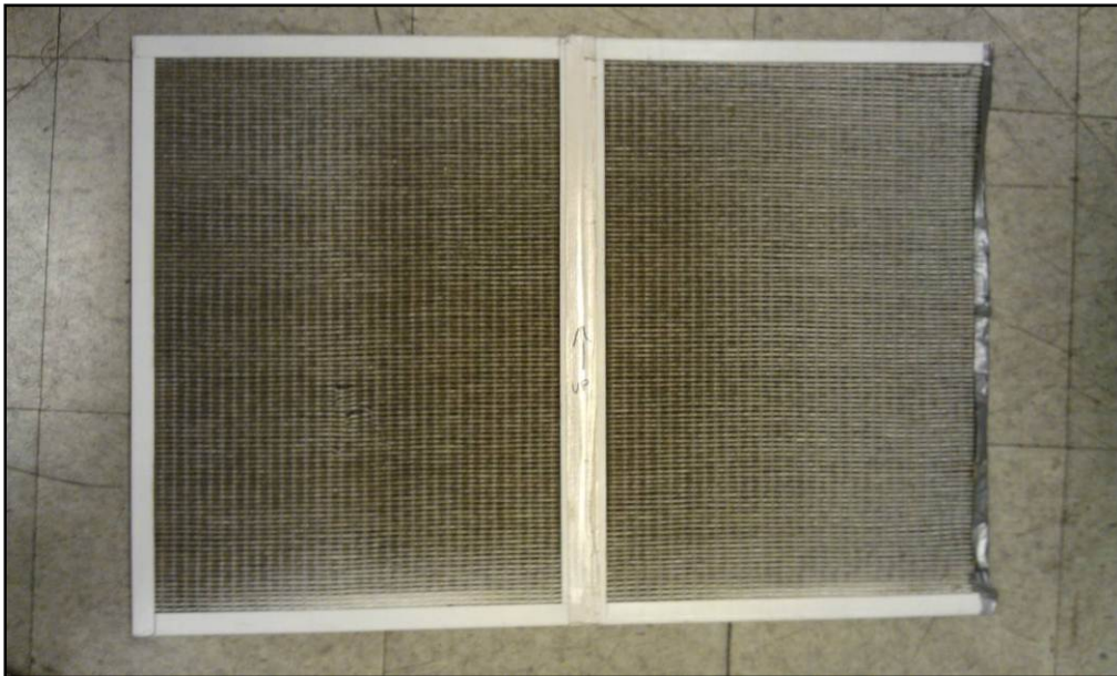
Figure 32: MERV 16 Filter Used in House 4 - Note the Discoloration
