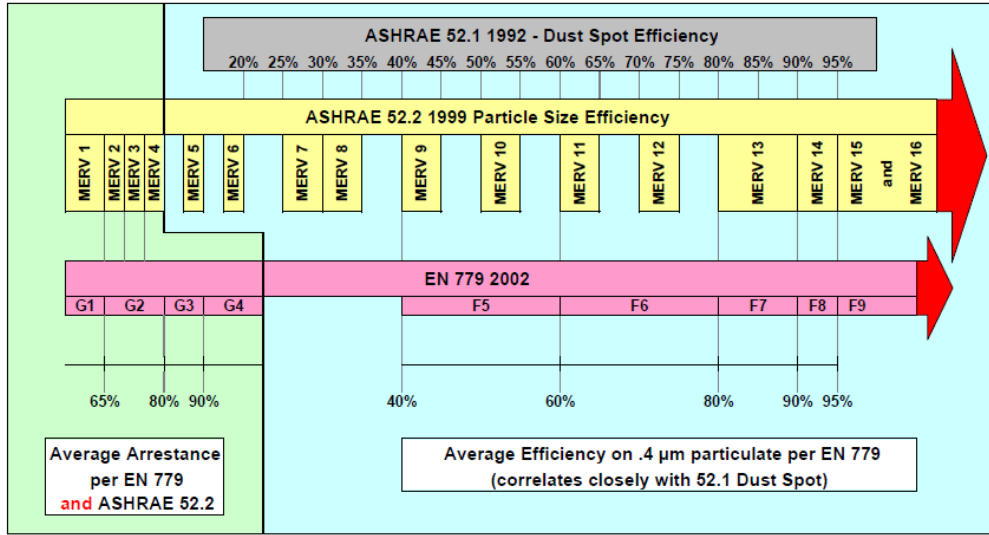
Figure 2: Comparison of EN 799 to ASHRAE MERV Ratings (by permission of Bob Burkhead)
