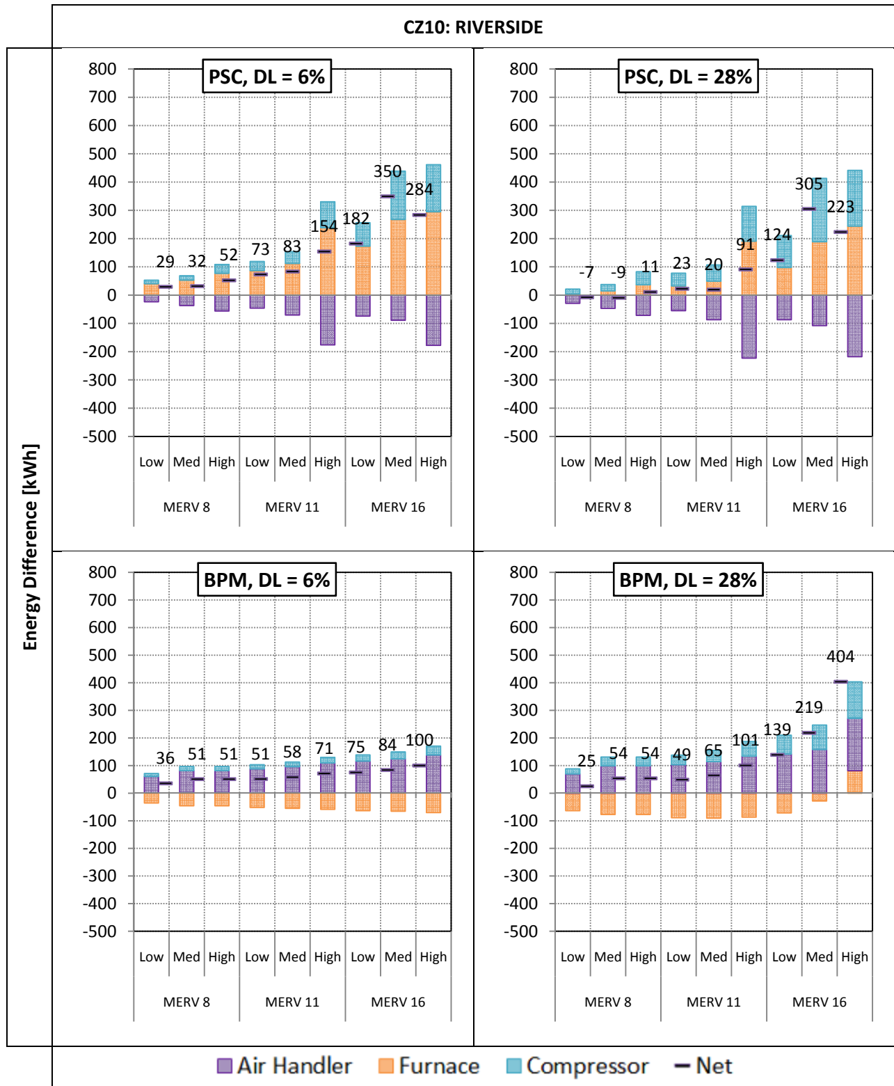
Figure 106: Filter Loading and Increasing MERV Effects on System Energy Performance in Climate Zone 10 Riverside. PSC and BPM Motors in Both New (6% Duct Leakage) and Old (28% Duct Leakage) Construction
