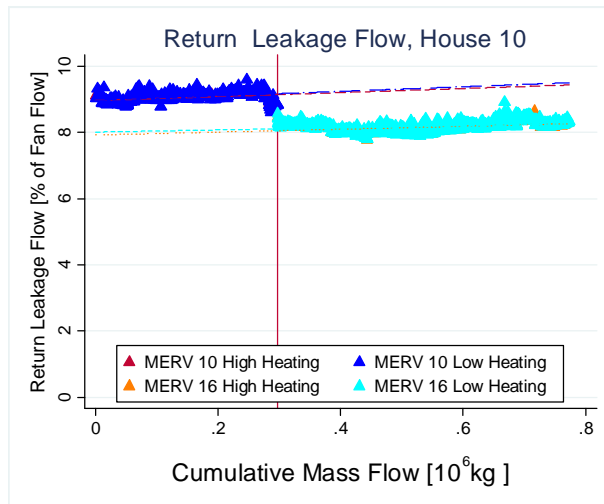
Figure 95: Return-Side Leakage for House 10
