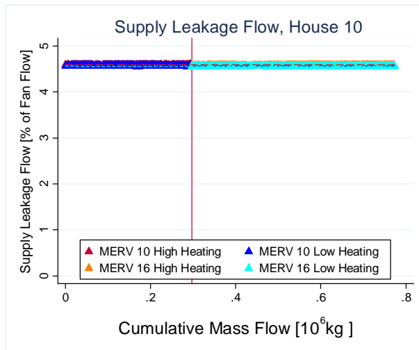
Figure 94: Supply-Side Leakage for House 10
