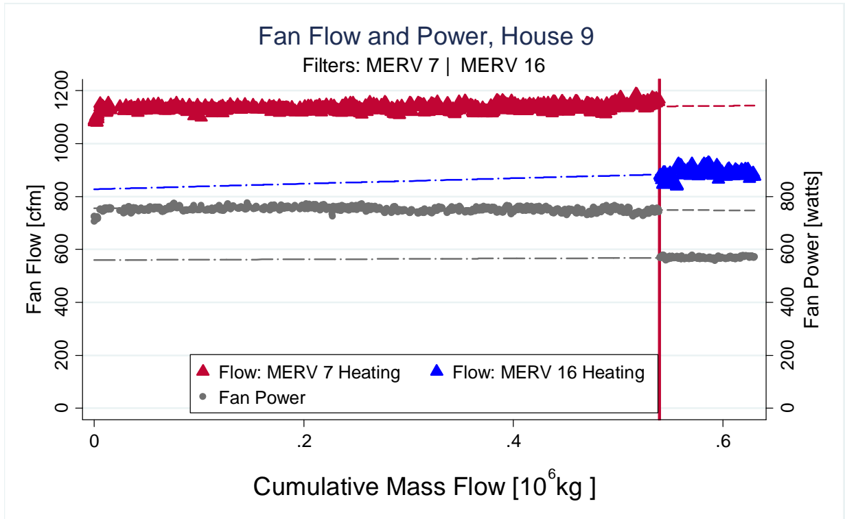
Figure 80: Fan Flow and Power Changes from House 9
