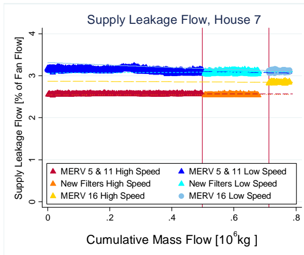
Figure 66: Supply-Side Leakage for House 7
