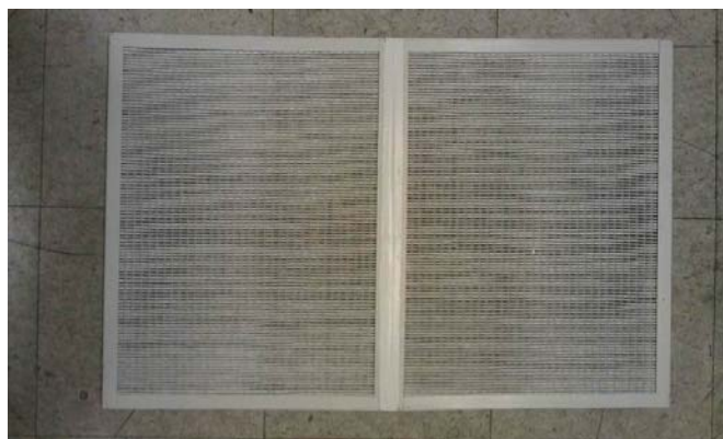
Figure 79: MERV 16 Filter after Removal from House 9
