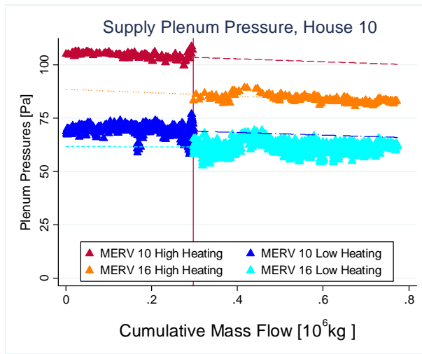
Figure 92: Supply Plenum Pressure (relative to inside the house) for House 10
