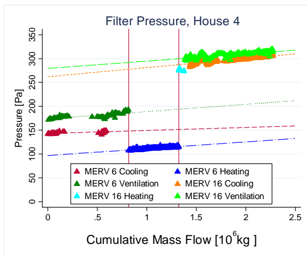
Figure 34: Pressure Across the Filter for House 4
