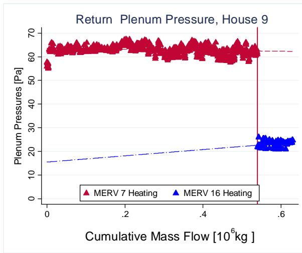
Figure 84: Return Plenum Pressure (relative to inside the house) for House 9
