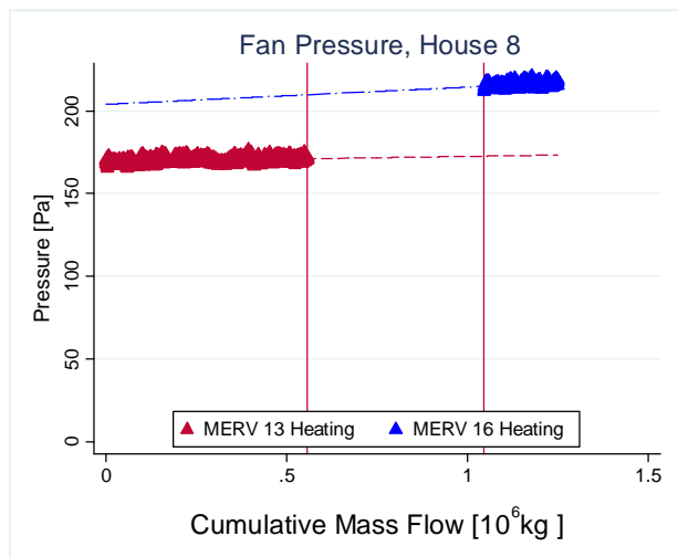
Figure 73: Pressure Across the Fan for House 8
