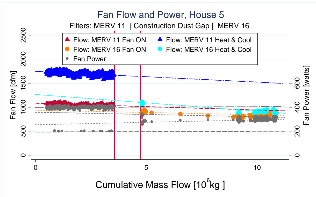
Figure 42: Fan Flow and Power changes from House 5
