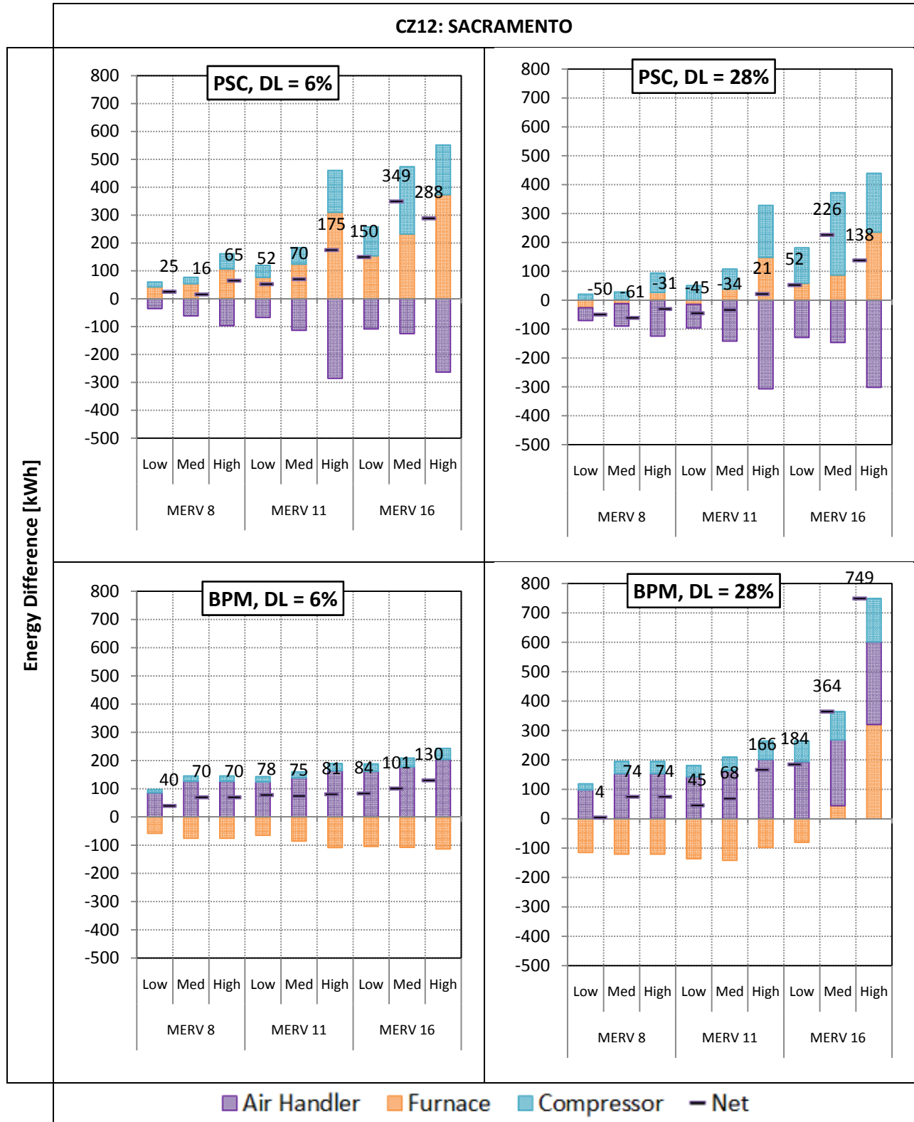
Figure 107: Filter Loading and Increasing MERV Effects on System Energy Performance in Climate Zone 12 Sacramento. PSC and BPM Motors in Both New (6% Duct Leakage) and Old (28% Duct Leakage) Construction
