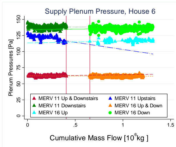
Figure 54: Supply Plenum Pressure (relative to inside the house) for House 6
