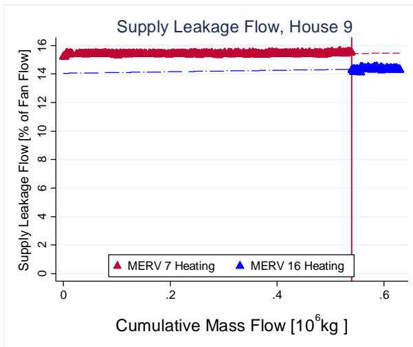
Figure 85: Supply-Side Leakage for House 9
