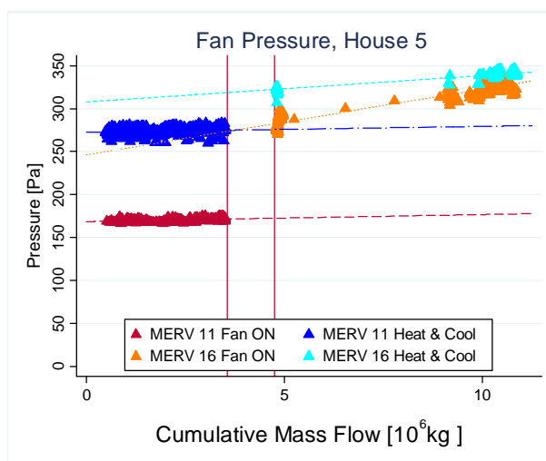
Figure 44: Pressure Across the Fan for House 5
