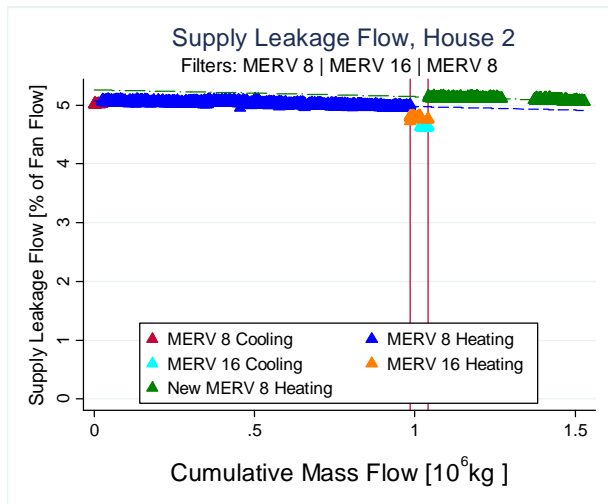
Figure 19: Supply Side Leakage for House 2
