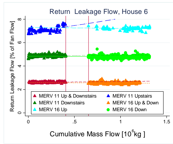
Figure 57: Return Side Leakage for House 6
