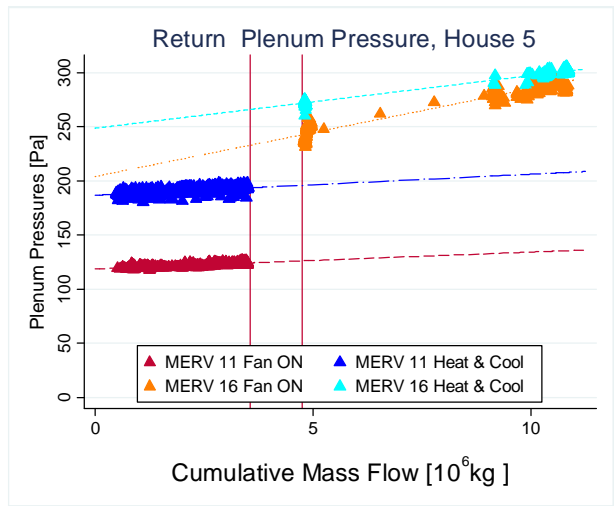
Figure 46: Return Plenum Pressure (relative to inside the house) for House 5
