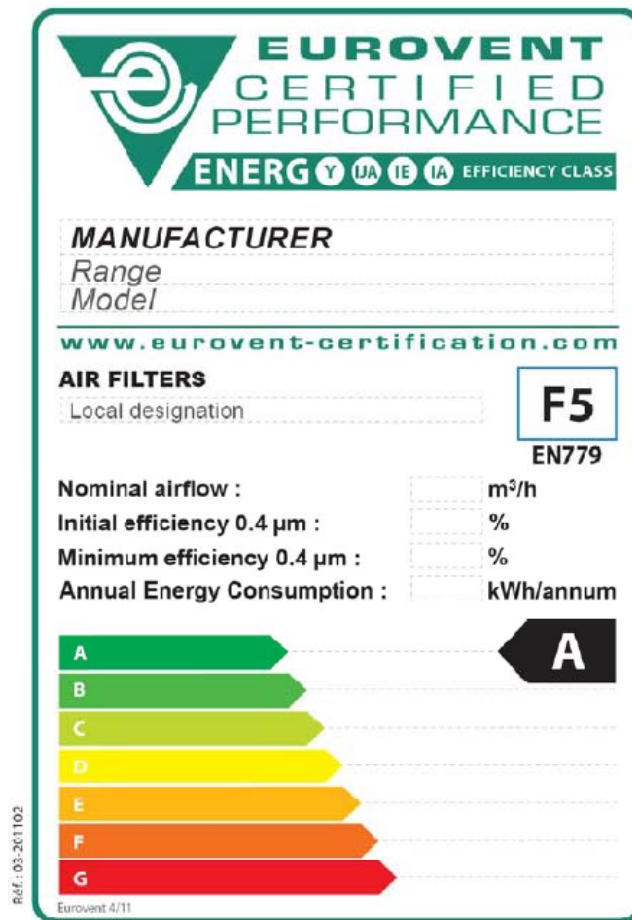
Figure 1: Example of EUROVENT Filter Label from EN 779
