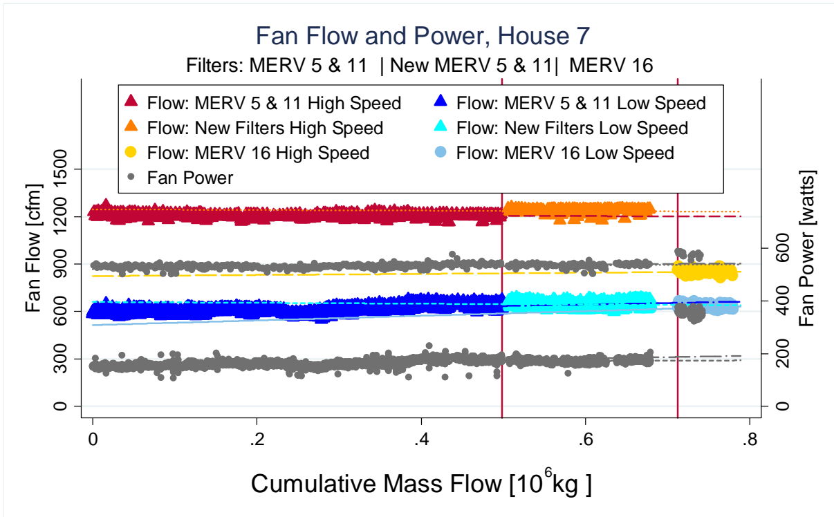
Figure 60: Fan Flow and Power Changes from House 7
