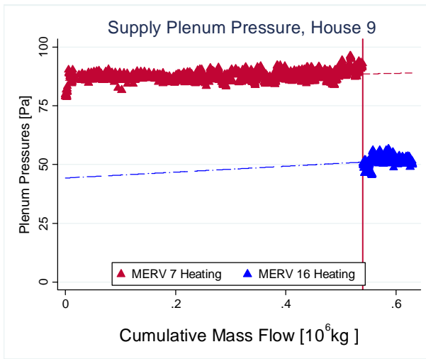
Figure 83: Supply Plenum Pressure (relative to inside the house) for House 9
