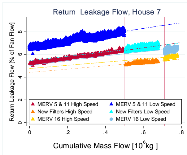
Figure 67: Return-Side Leakage for House 7
