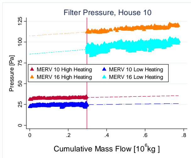
Figure 90: Pressure Across the Filter for House 10
