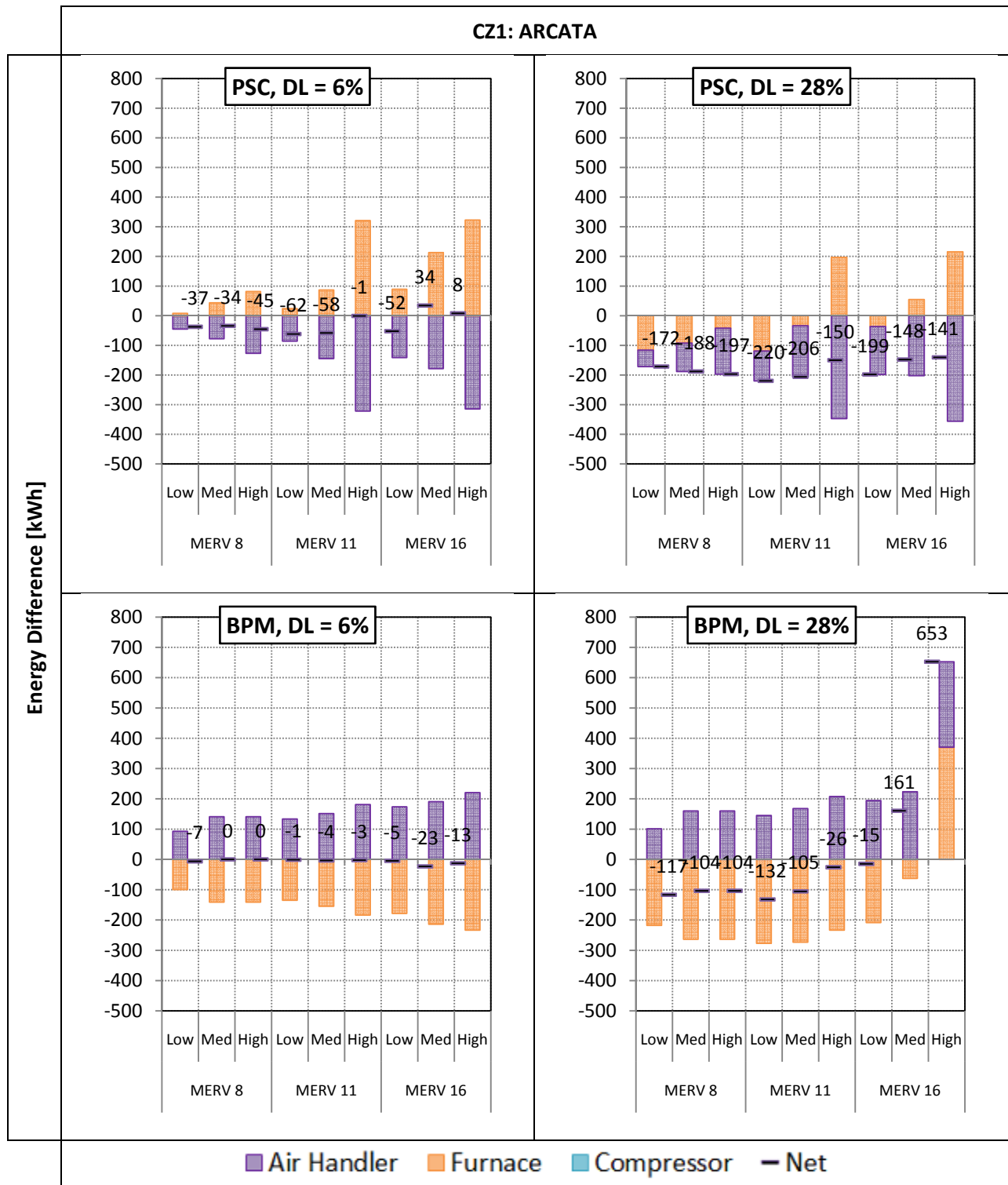
Figure 104: Filter Loading and Increasing MERV Effects on System Energy Performance in Climate Zone 1 Arcata. PSC and BPM Motors in Both New (6% Duct Leakage) and Old (28% Duct Leakage) Construction
