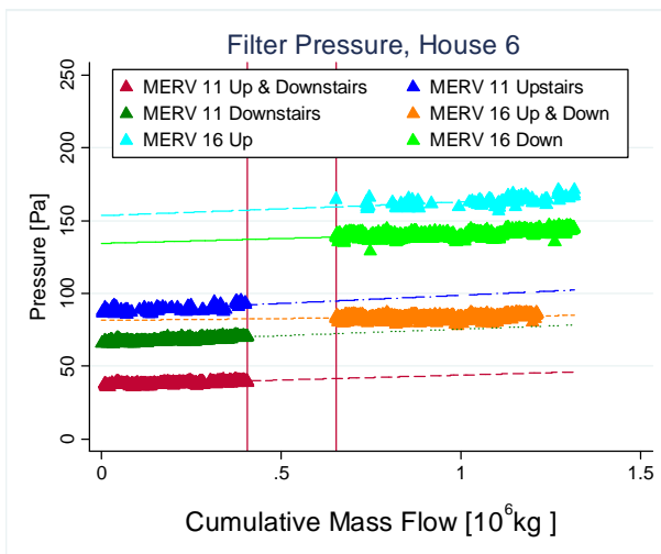
Figure 52: Pressure Across Filter for House 6
