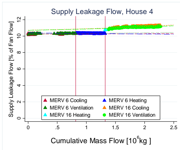
Figure 38: Supply Side Leakage for House 4
