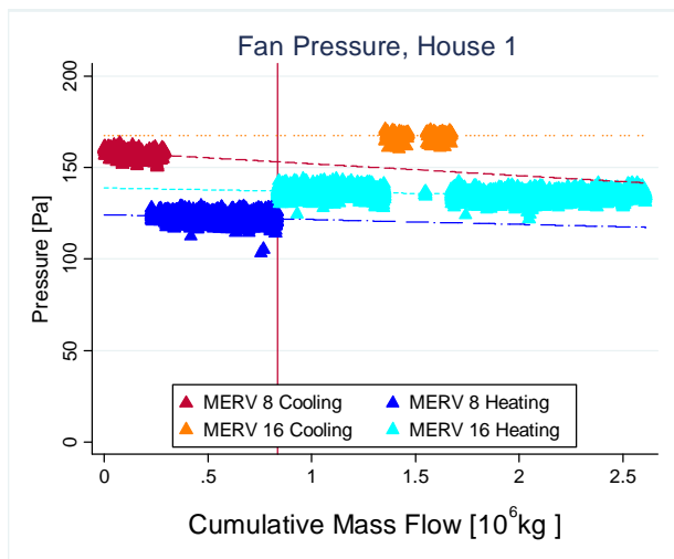
Figure 7: Pressure Across the Fan for House 1
