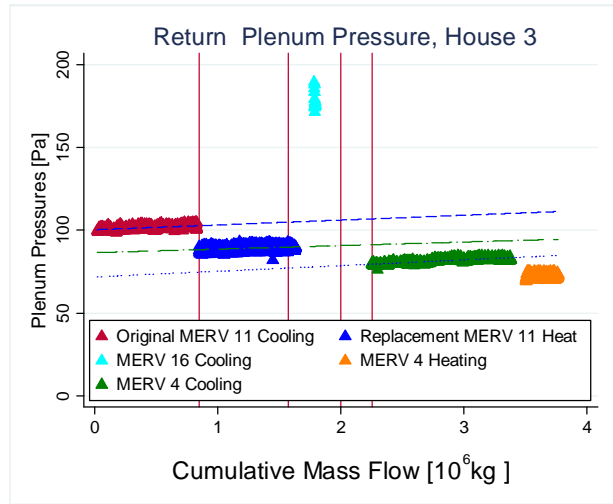
Figure 28: Return Plenum Pressure for House 3
