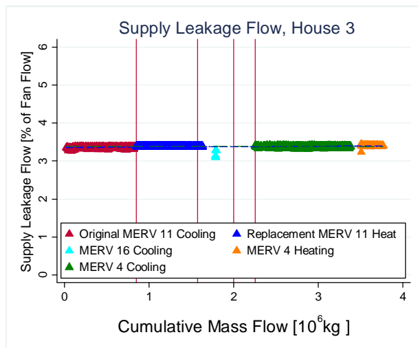
Figure 29: Supply Side Leakage for House 3
