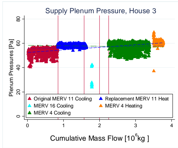
Figure 27: Supply Plenum Pressure for House 3
