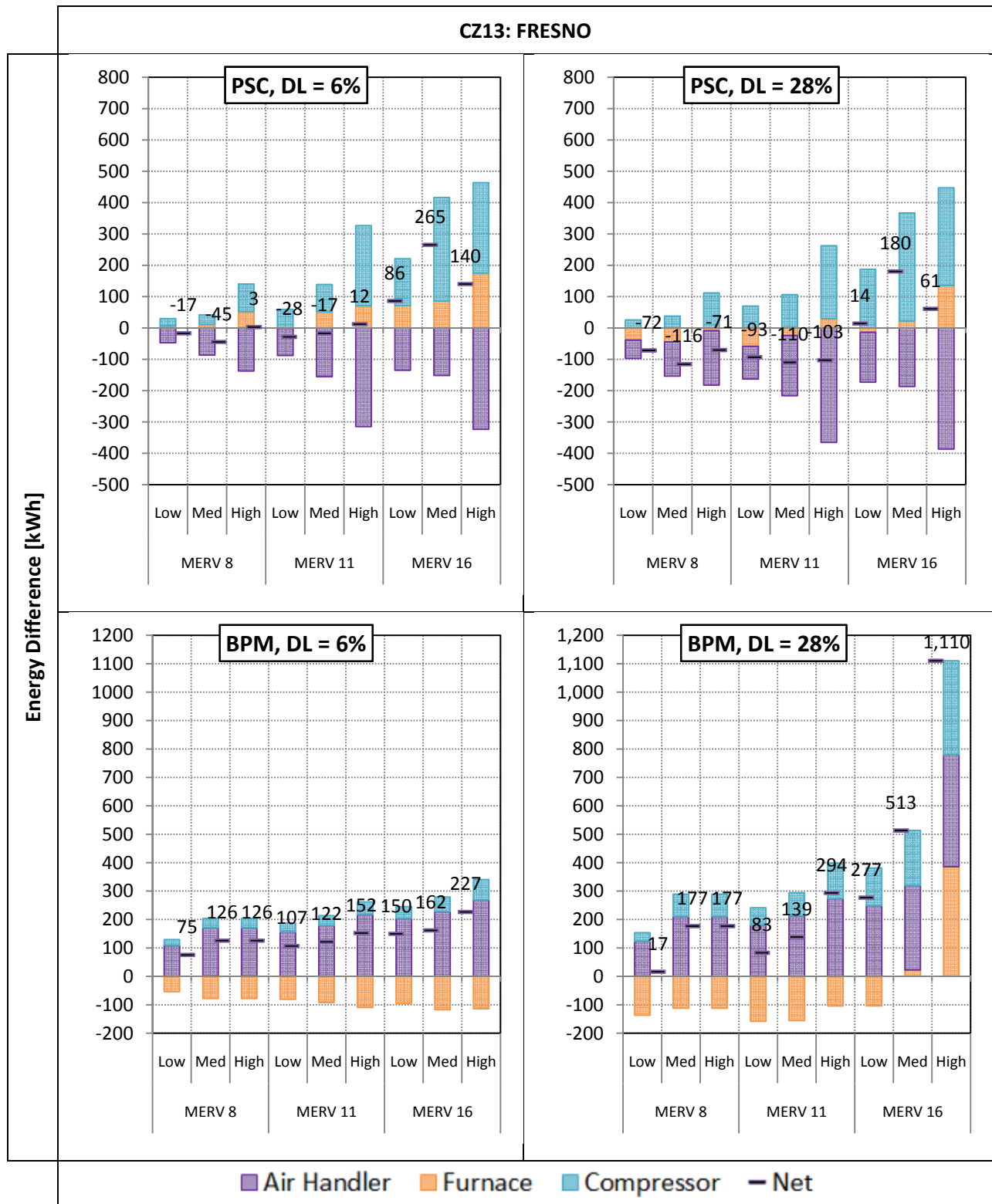
Figure 108: Filter Loading and Increasing MERV Effects on System Energy Performance In Climate Zone 13 Fresno. PSC and BPM Motors in Both New (6% Duct Leakage) and Old (28% Duct Leakage) Construction. (Note the Scale Change for the BPM Motor)
