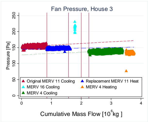
Figure 26: Pressure Across the Fan for House 3
