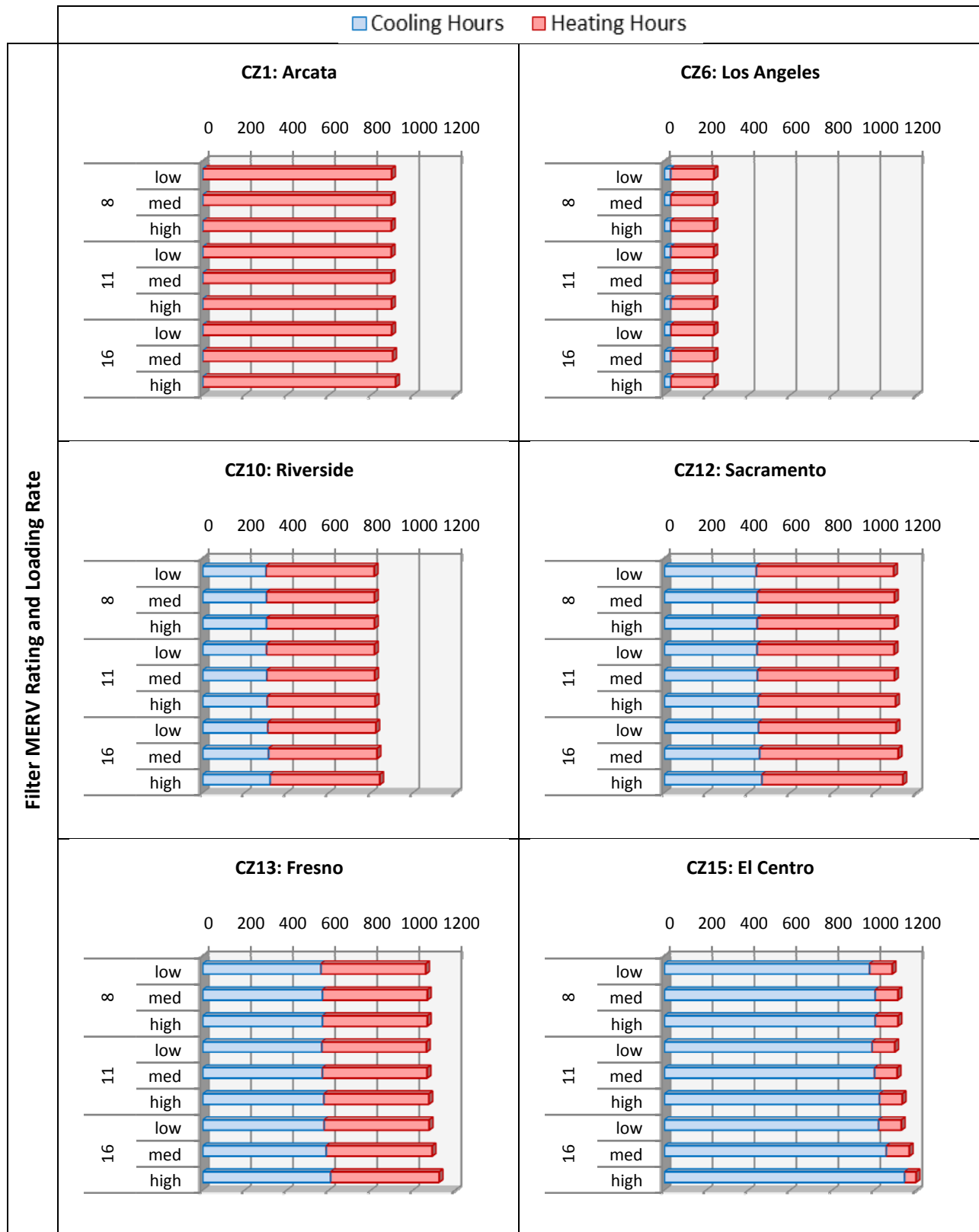
Figure 101: Annual Air Handler Operation Time (H) For BPM Motor with 28% Duct Leakage
