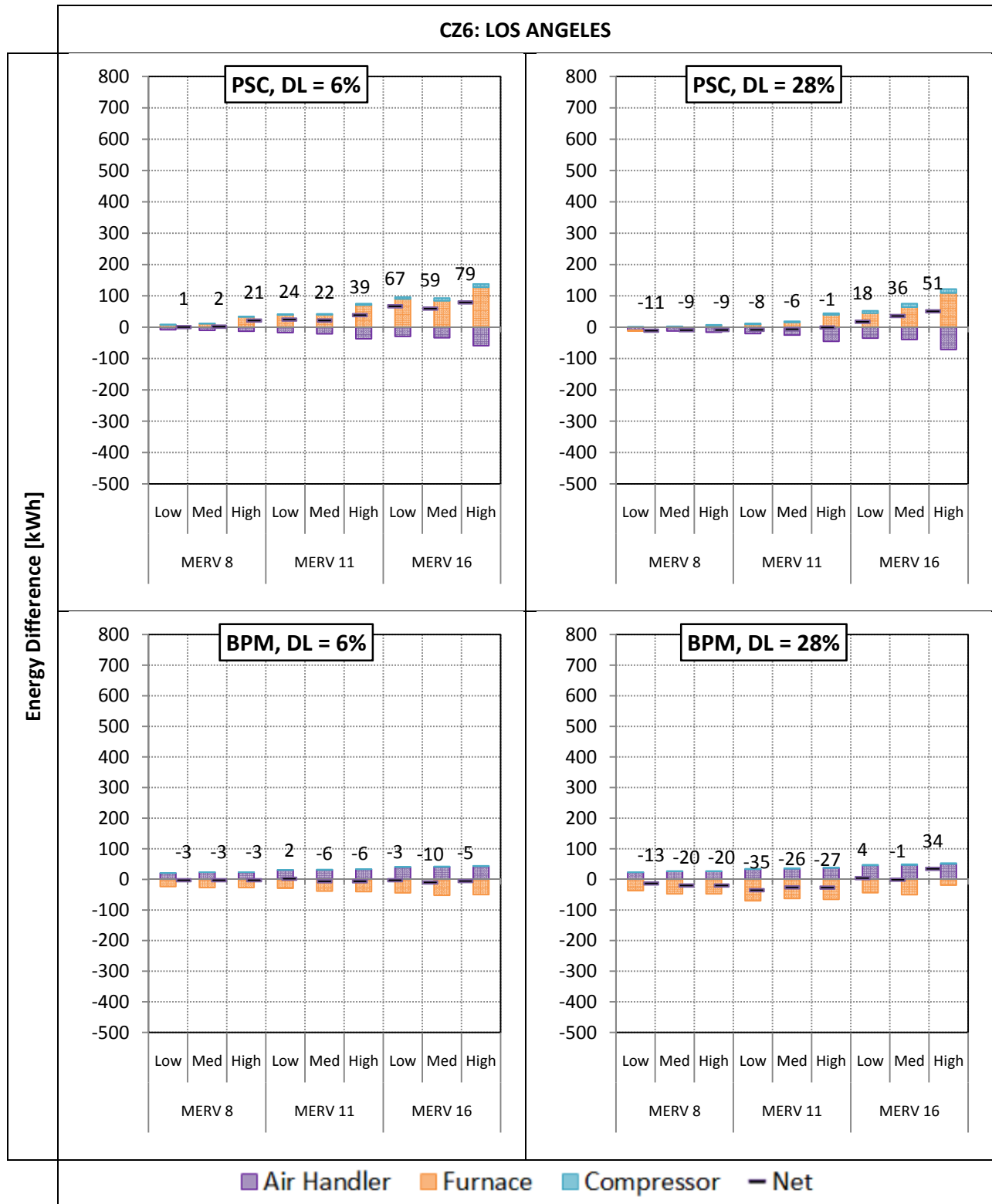
Figure 105: Filter Loading and Increasing MERV Effects on System Energy Performance in Climate Zone 6 LA. PSC and BPM Motors in Both New (6% Duct Leakage) and Old (28% Duct Leakage) Construction
