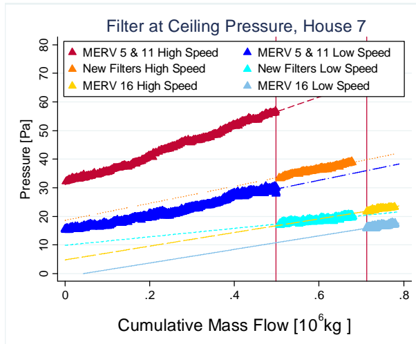
Figure 61: Pressure Across the Ceiling Filter for House 7
