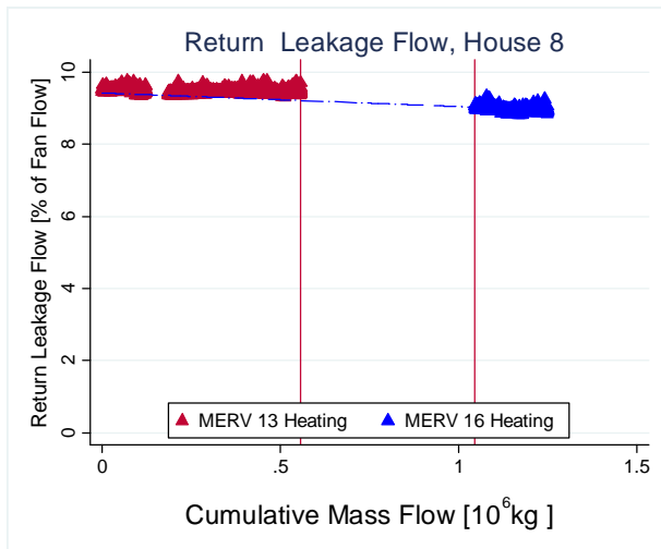
Figure 77: Return-Side Leakage for House 8
