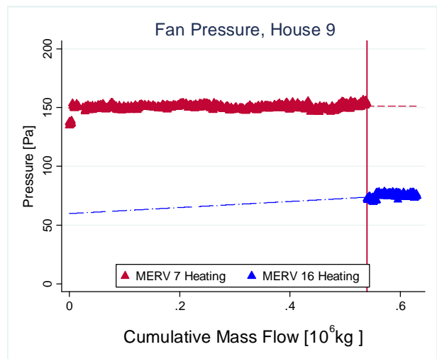
Figure 82: Pressure Across the Fan for House 9
