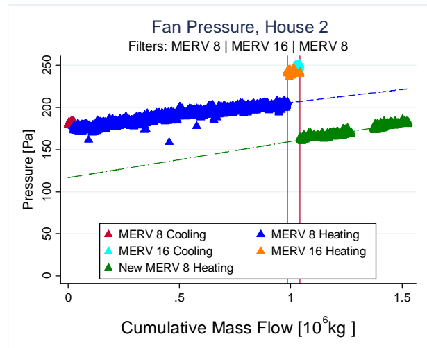
Figure 16: Pressure Across the Fan for House 2.
