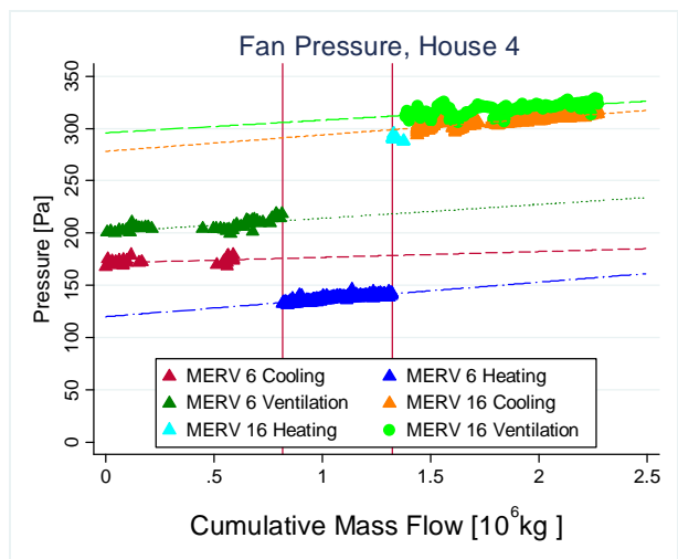
Figure 35: Pressure Across the Fan for House 4
