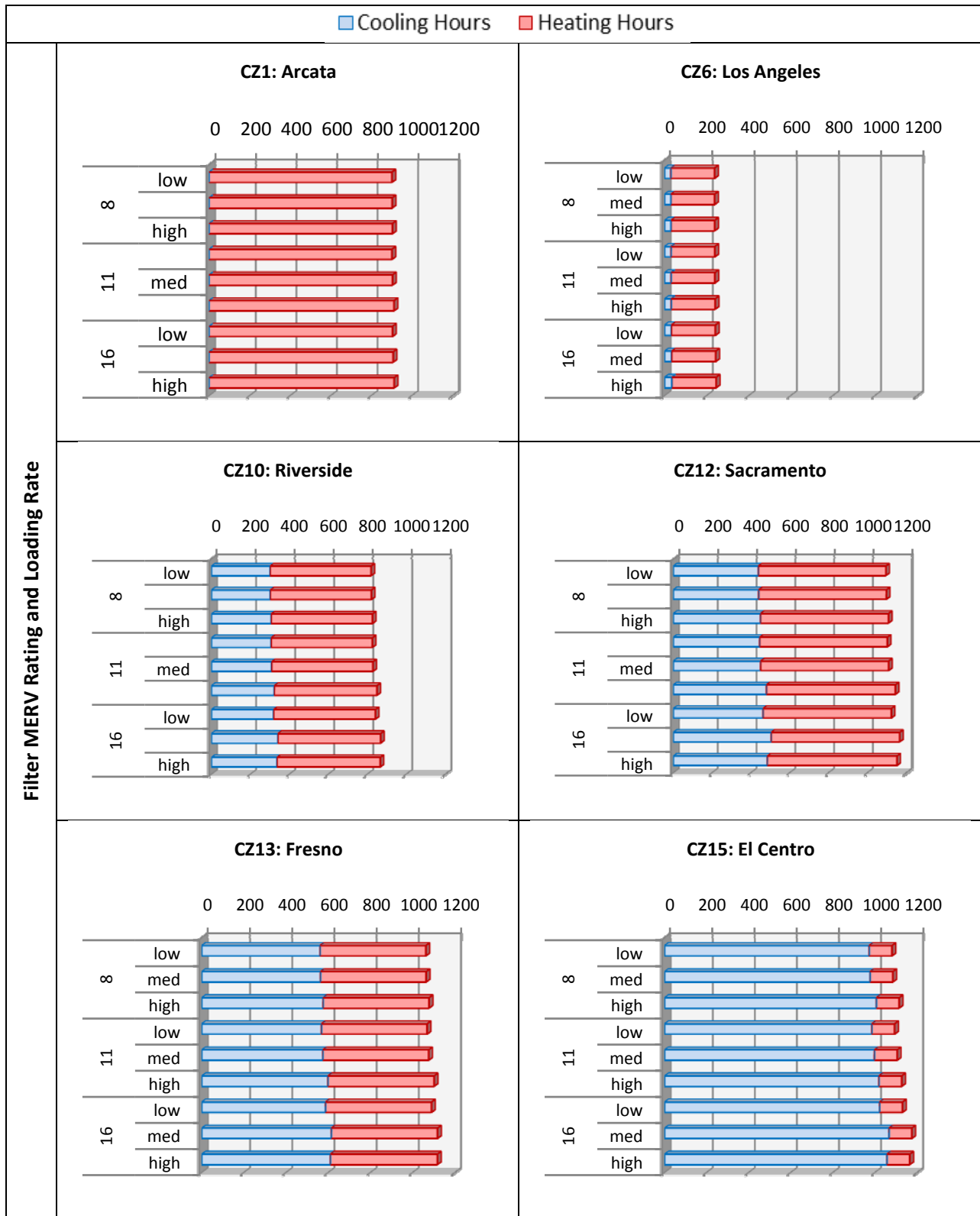
Figure 100: Annual Air Handler Operation Time (H) For PSC Motor with 28% Duct Leakage
