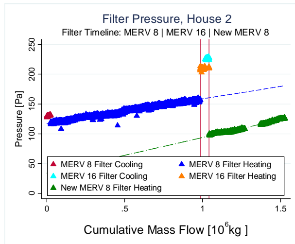
Figure 15: Pressure Across the Filter for House 2
