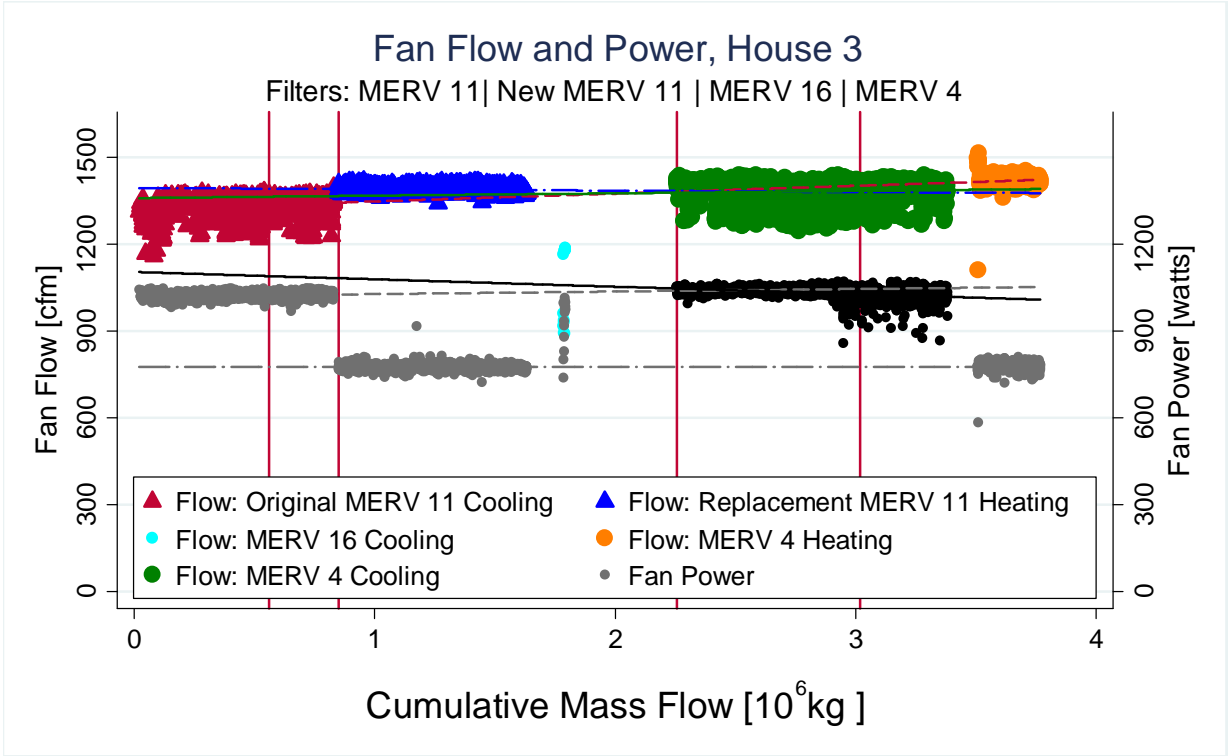
Figure 24: Gaps in Data before the MERV 16 Filter are from a Few Days with New MERV 11 Filters Which Look Similar to the Longer Time Periods Shown.
