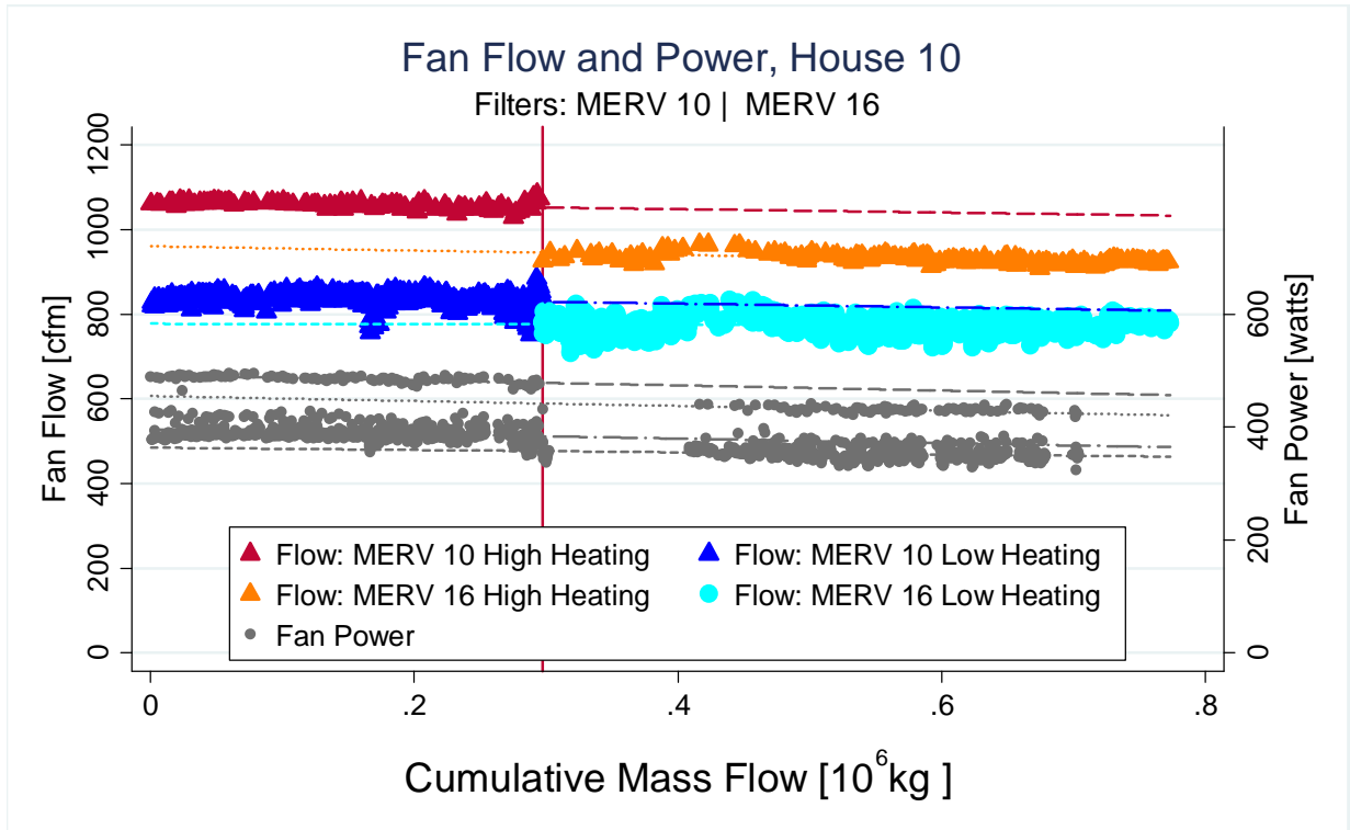
Figure 89: Fan Flow and Power Changes from House 10
