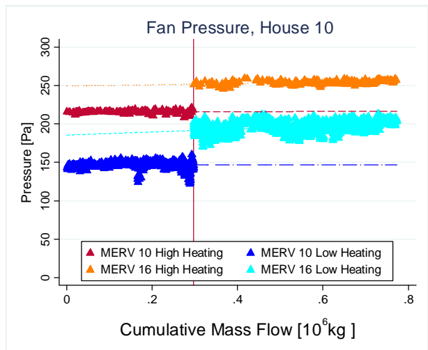
Figure 91: Pressure Across the Fan for House 10
