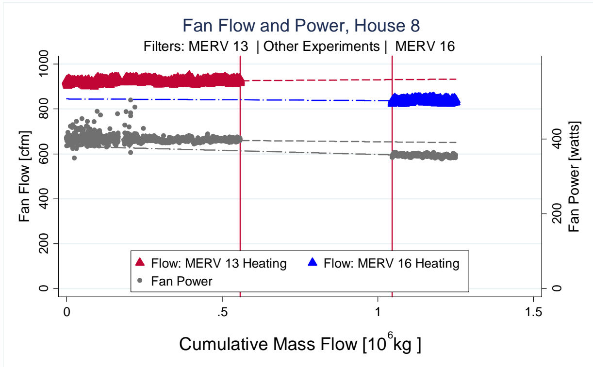
Figure 71: Fan Flow and Power Changes from House 8
