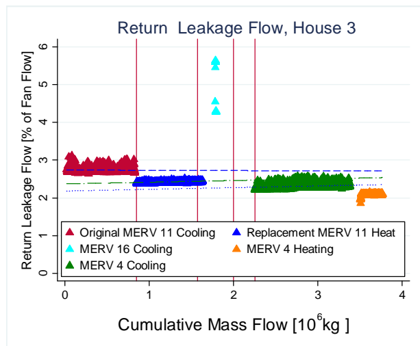
Figure 30: Return Side Leakage for House 3
