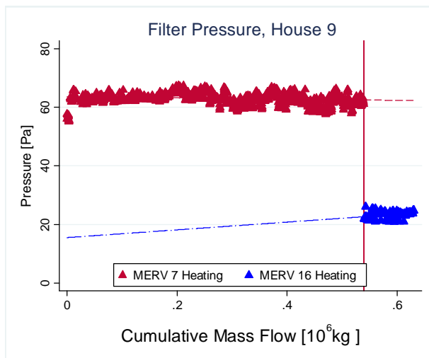
Figure 81: Pressure Across the Filter for House 9
