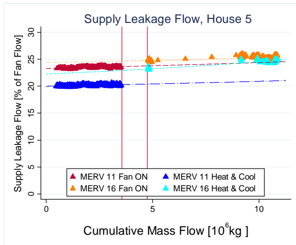
Figure 47: Supply Side Leakage for House 5
