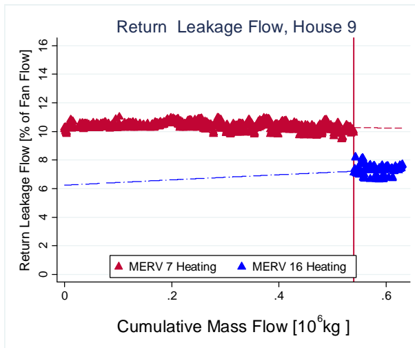
Figure 86: Return-Side Leakage for House 9
