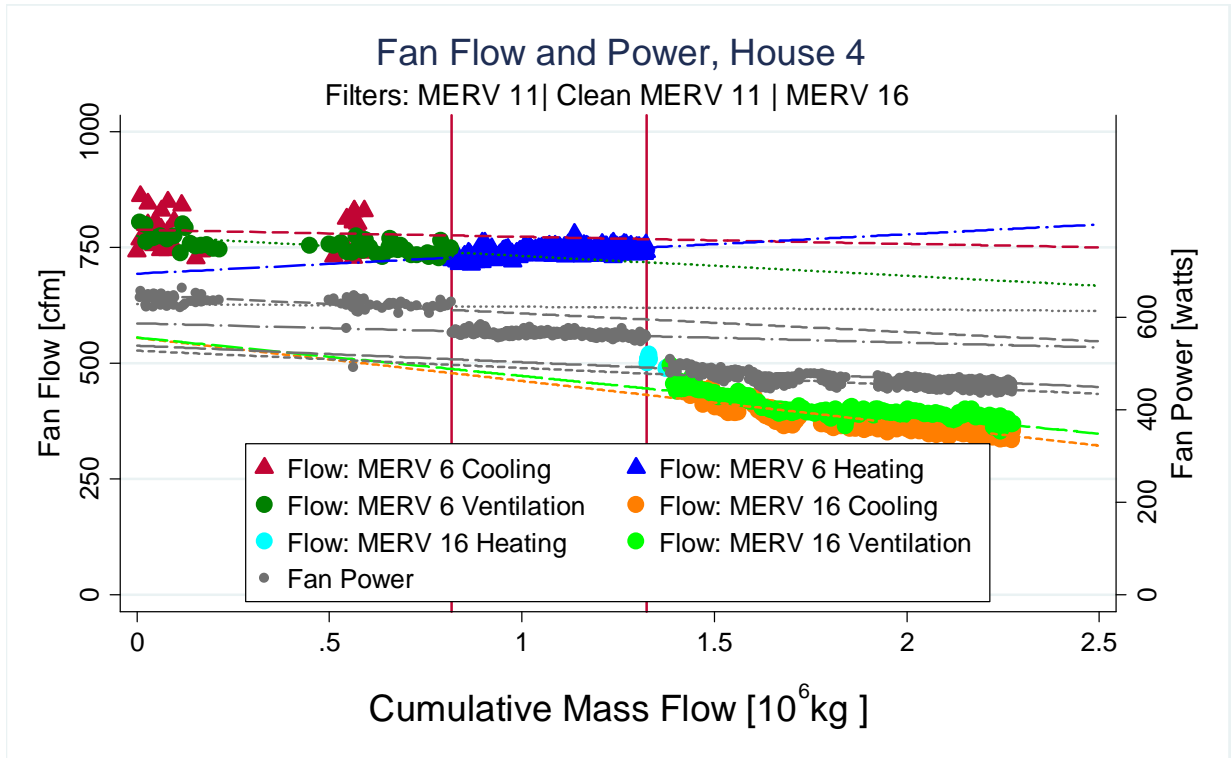
Figure 33: Fan Flow and Power Changes from House 4
