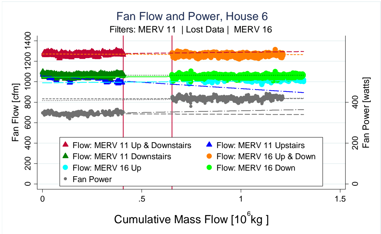
Figure 51: Fan Flow and Power Changes from House 6
