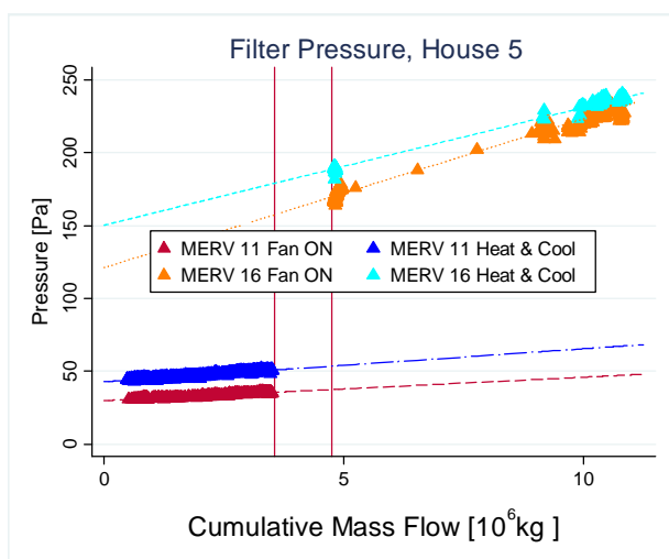
Figure 43: Pressure Across the Filter for House 5
