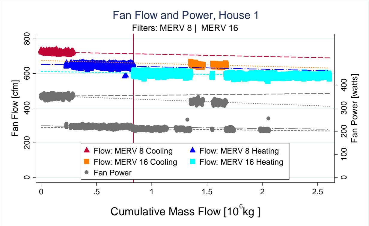
Figure 5: Fan Flow and Power Changes from House 1
