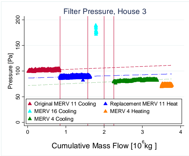
Figure 25: Pressure Across the Filter for House 3
