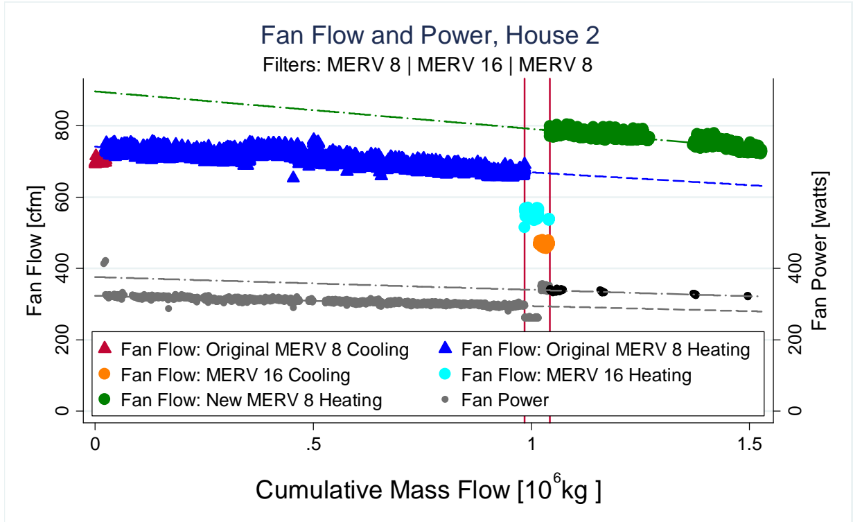
Figure 14: Fan Flow and Power Changes from House 2
