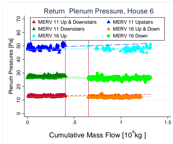
Figure 55: Return Plenum Pressure (relative to inside the house) for House 6
