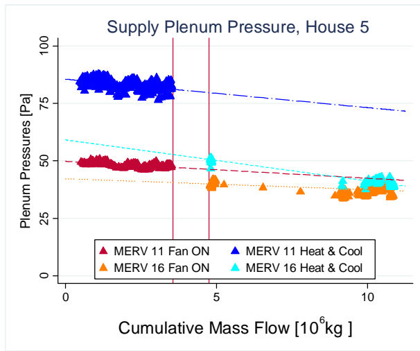
Figure 45: Supply Plenum Pressure (relative to inside the house) for House 5
