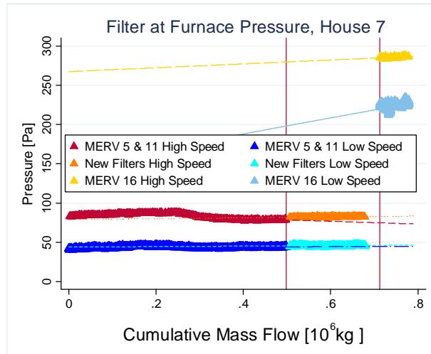
Figure 62: Pressure across the plenum filter for House 7
