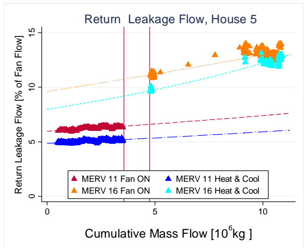
Figure 48: Return Side Leakage for House 5
