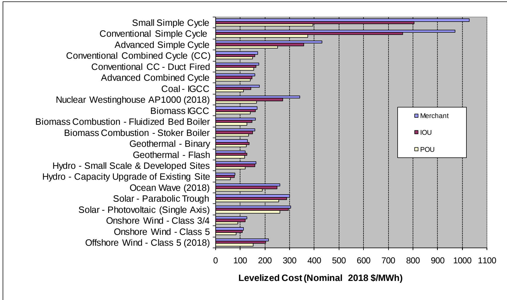
Figure 7: Summary of Average Levelized Costs—In-Service in 2018
