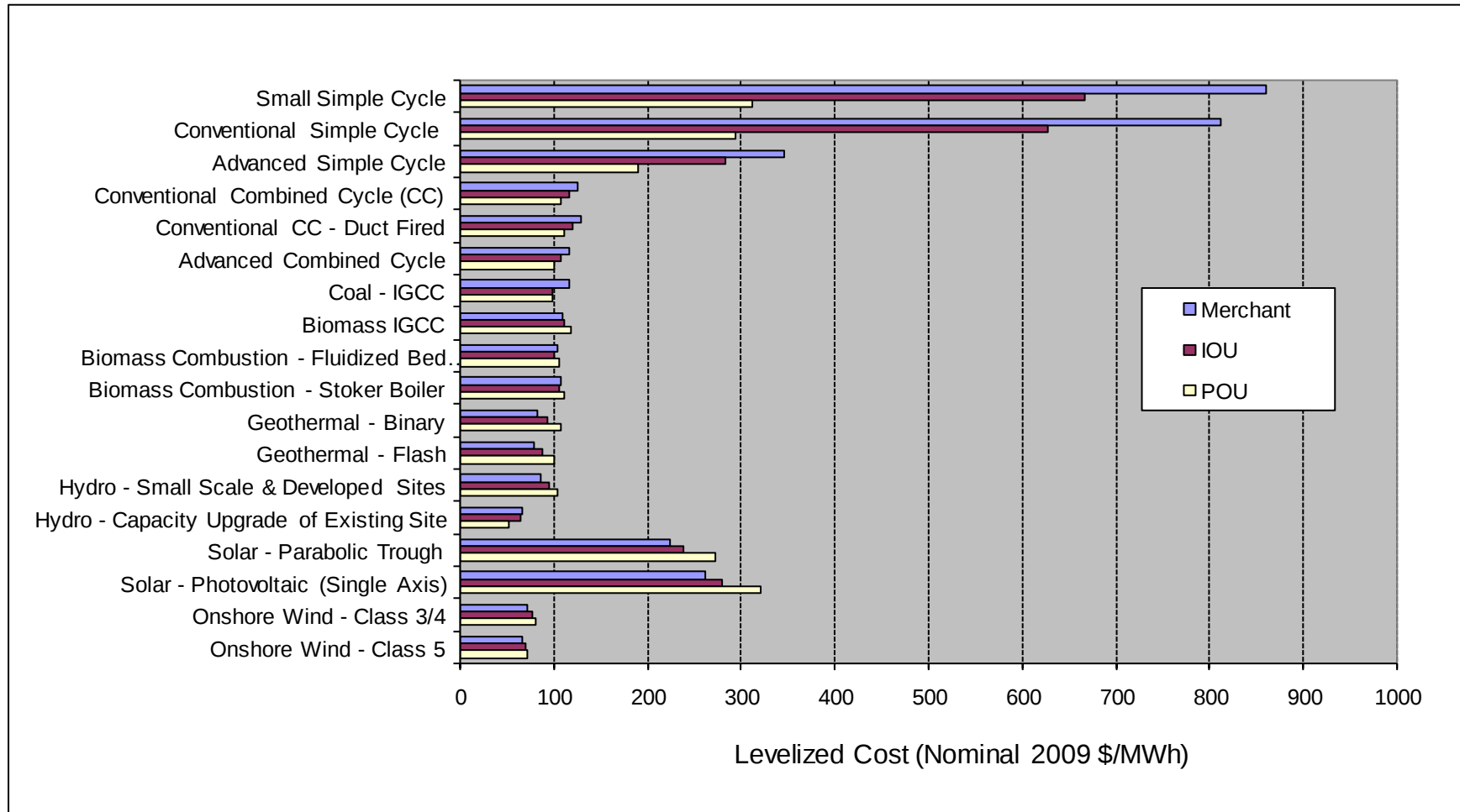
Figure 6: Summary of Average Levelized Costs—In-Service 2009
