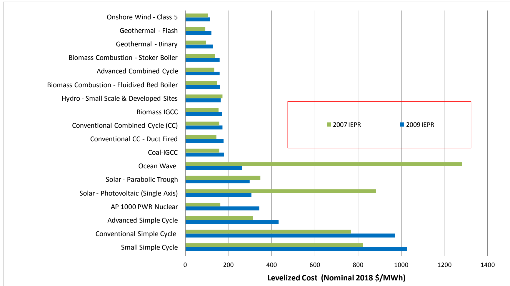
Figure 20: Comparing 2009 IEPR Levelized Costs to 2007 IEPR—In-Service in 2018
