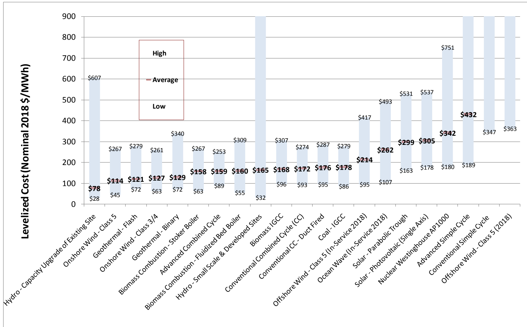
Figure 18: Range of Levelized Cost for Merchant Plant In-Service in 2018—Enlarged
