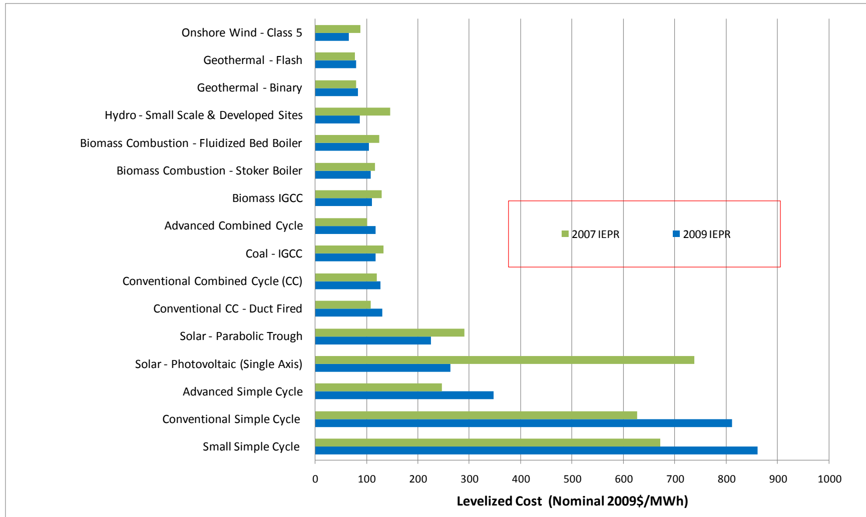
Figure 4: Comparing 2009 Average Levelized Costs to 2007 IEPR Results (In-Service in 2009)
