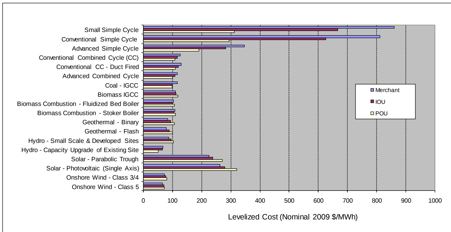
Figure 1: Summary of Average Levelized Costs—In-Service in 2009
