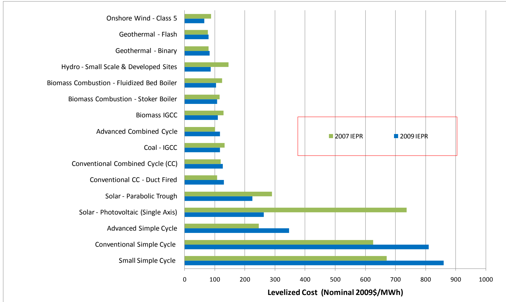
Figure 19: Comparing 2009 IEPR Levelized Costs to 2007 IEPR—In-Service in 2009
