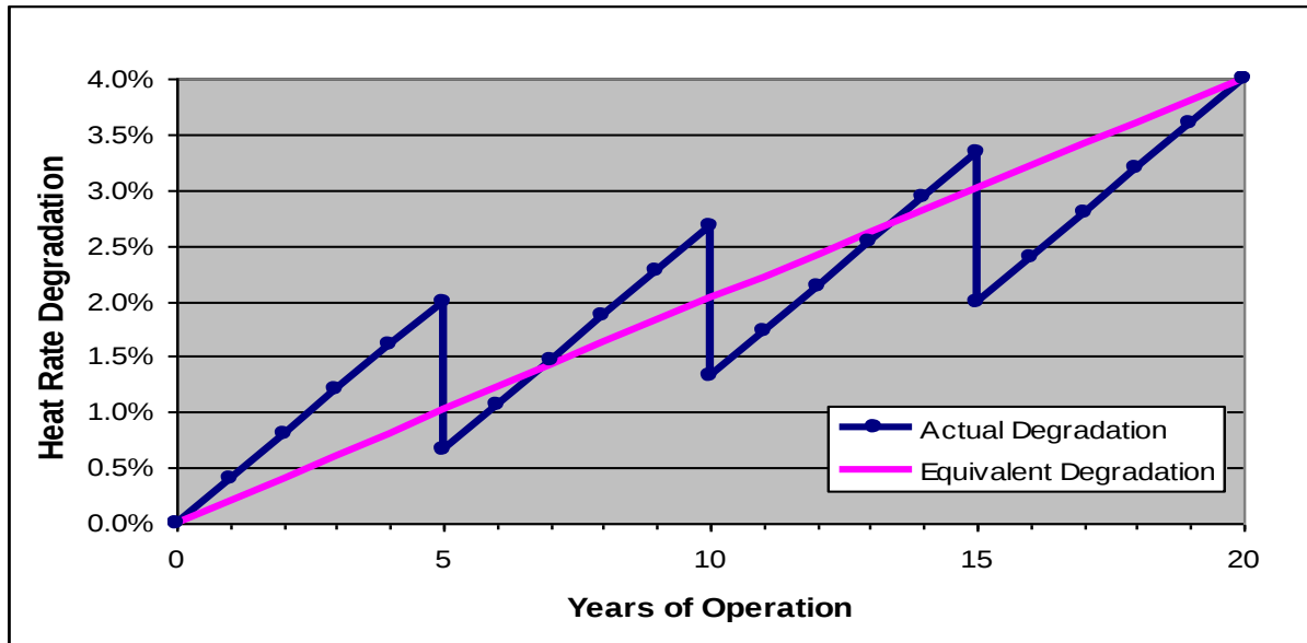
Figure C-8: Combined Cycle Heat Rate Degradation
