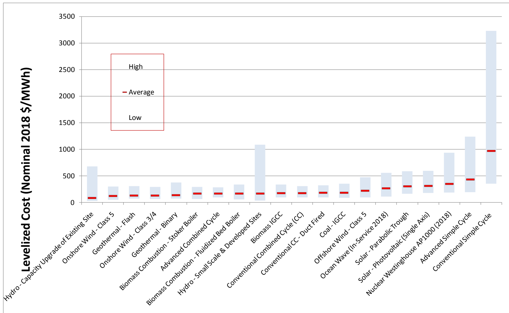
Figure 17: Range of Levelized Cost for Merchant Plant In-Service in 2018
