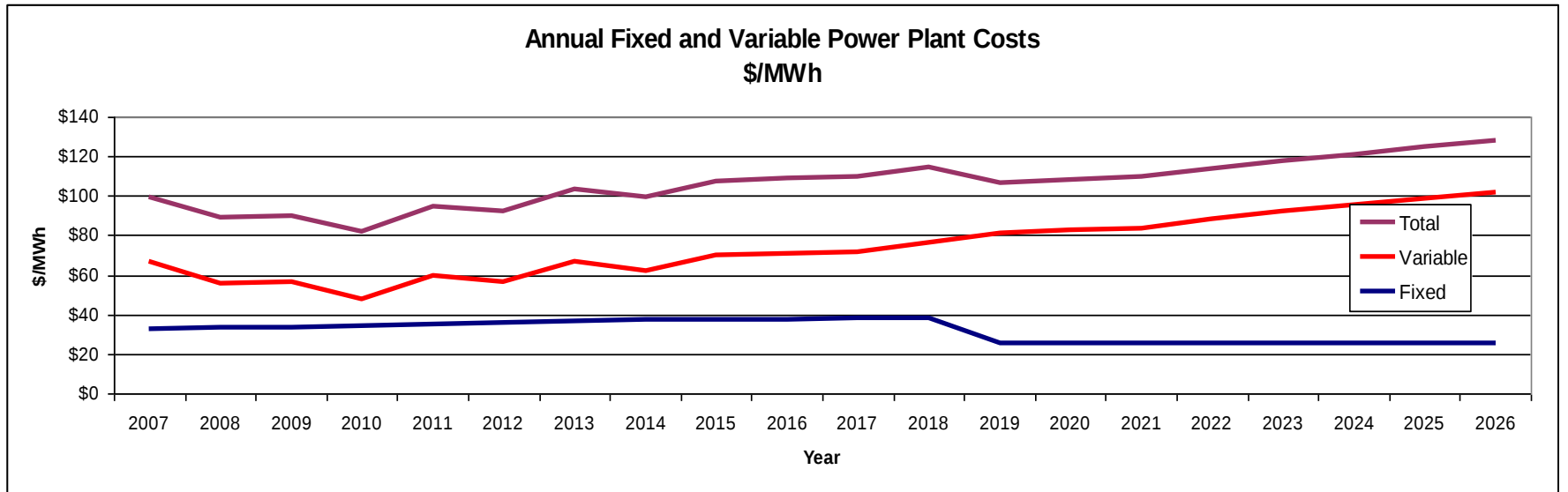
Figure A-5: Annual Costs—Merchant Combined Cycle Plant
