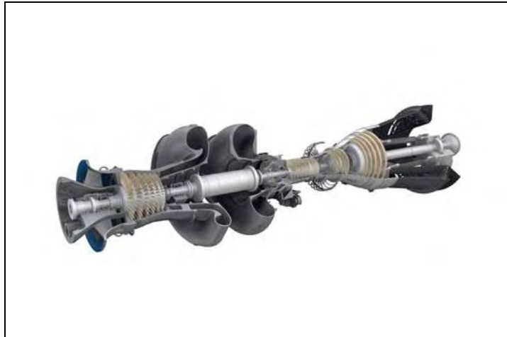
Figure C-2: LMS100 Gas Turbine
