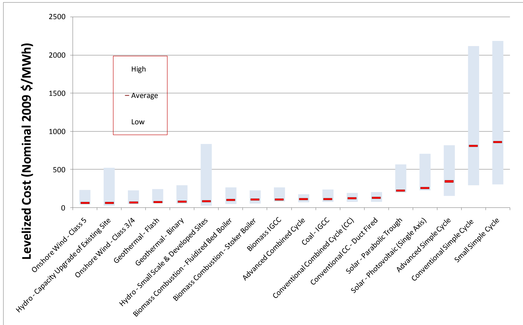
Figure 2: Range of Levelized Cost for a Merchant Plant In-Service in 2009 (Nominal $/MWh)
