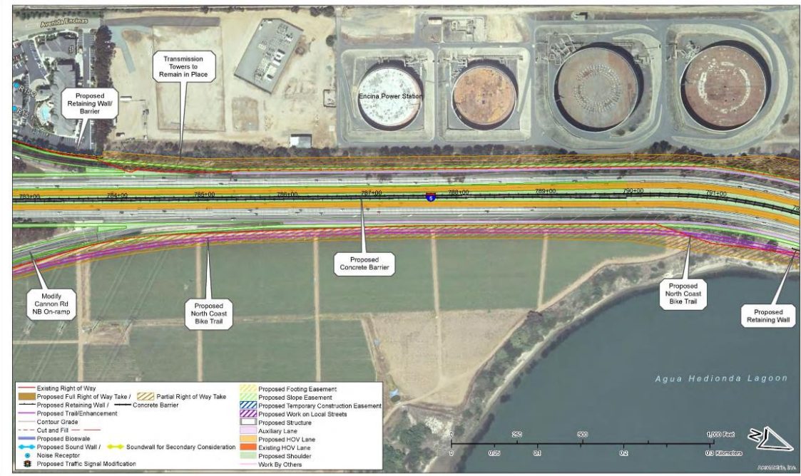
Figure 2-2.3, Sheet 50 of 67 – Project Features Map: 8+4 Buffer (Preferred Alternative) Soundwalls for secondary consideration are not part of the project. See Executive Summary (ES.5.15 Noise).
