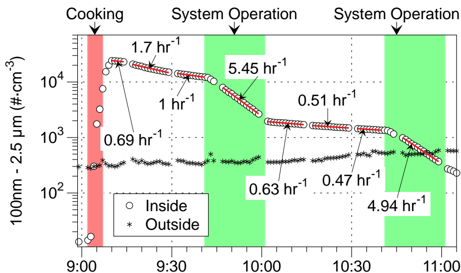
Figure 3.30. Time series of number concentrations of 100 nm to 2.5 \mu\text{m} diameter particles during cooking experiment with System D on July 16, 2014.
