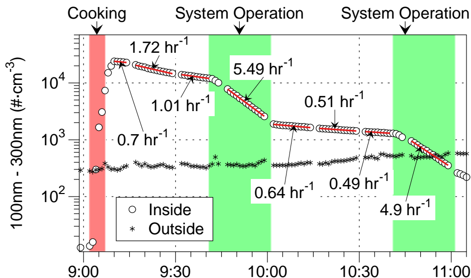
Figure 3.32. Time series of number concentrations of 100-300 nm diameter particles during cooking experiment with System D on July 16, 2014.
