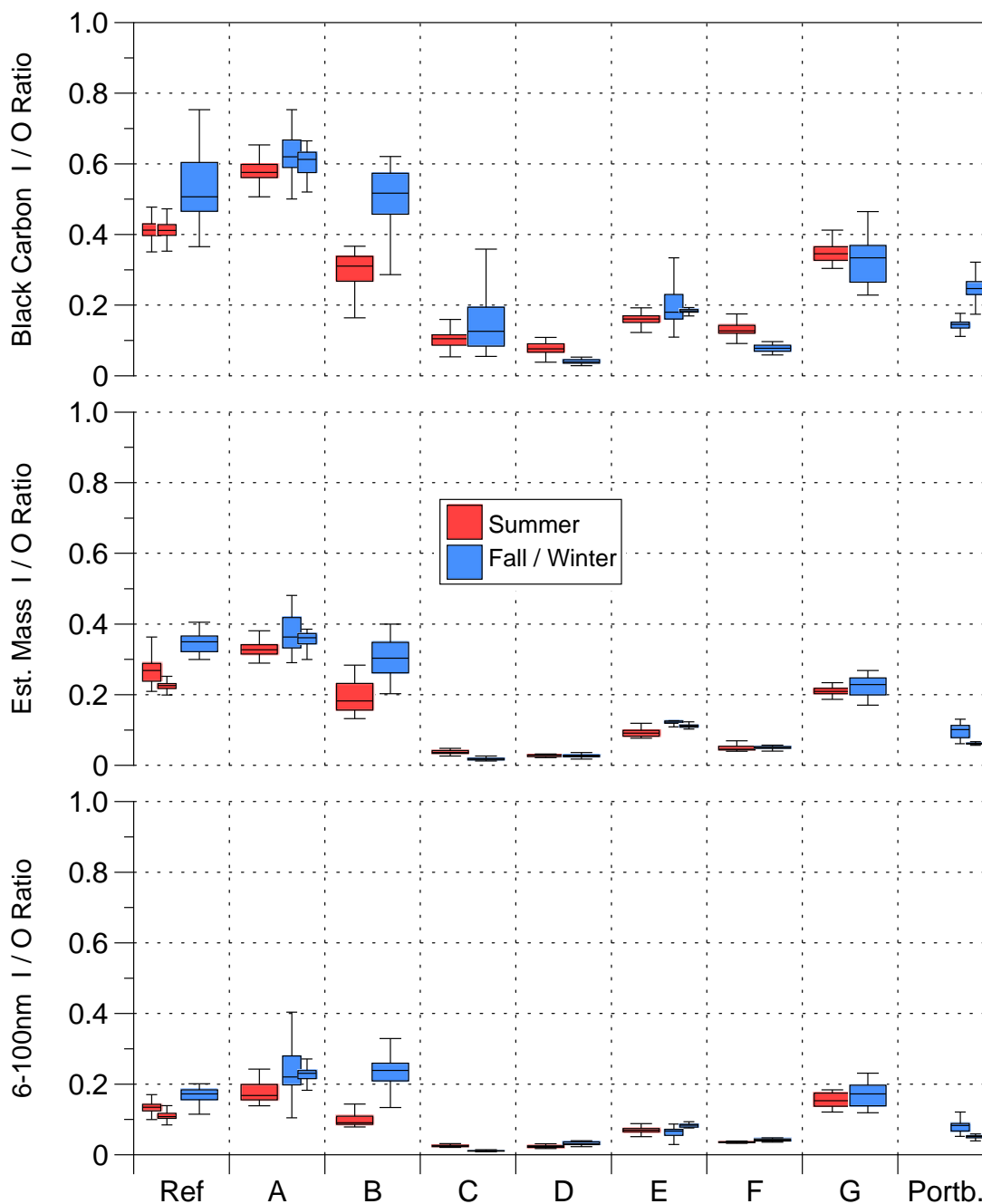
Figure 3.21. Distribution of running 24h average indoor/outdoor ratios for black carbon, estimated PM_{2.5} mass, and ultrafine particles (6-100 nm) for each system operating over multi-day periods in fall/winter (FW) and summer (SU) seasons.
