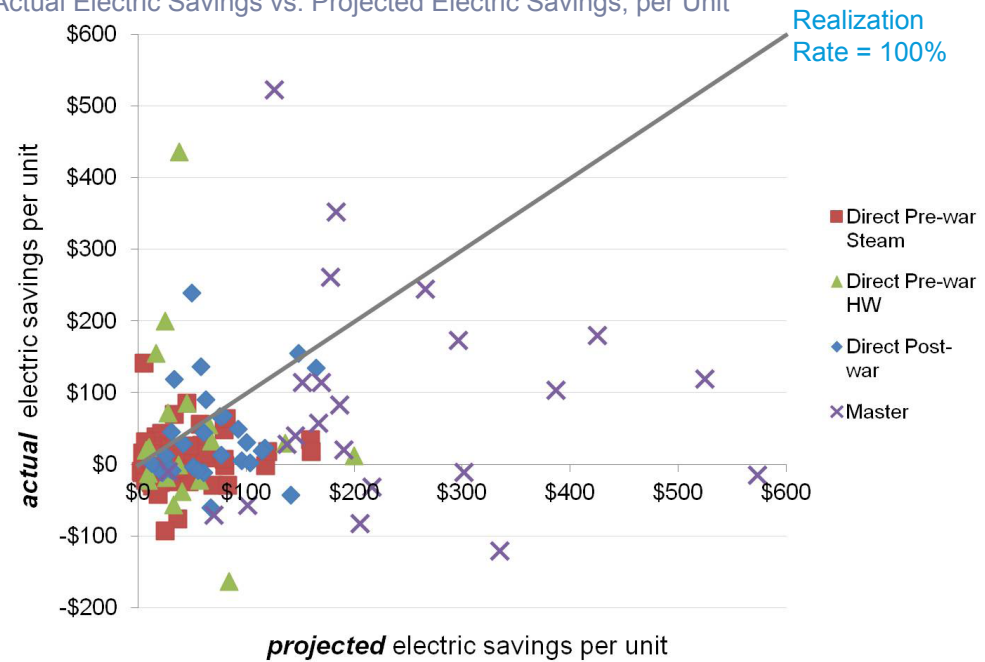
Figure 21: Electric Realization Rates Exhibited Wide Variation Actual Electric Savings vs. Projected Electric Savings, per Unit
