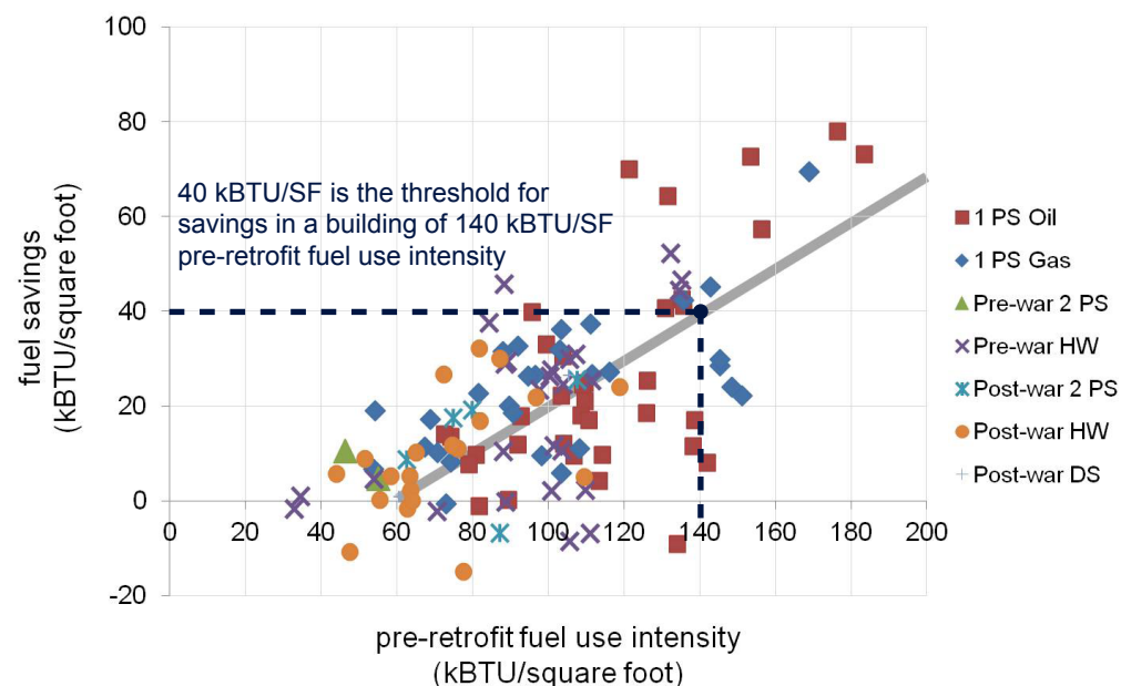
Figure 17: Historical Pre-retrofit Fuel Use Intensity Indicates a Threshold for Likely Savings
