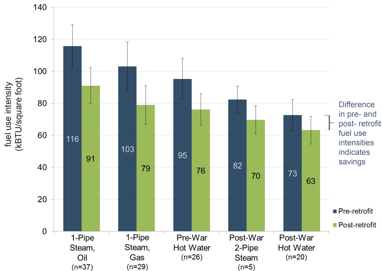
Figure 8: Pre- and Post-retrofit Fuel Use Intensity, by Comparative Group
