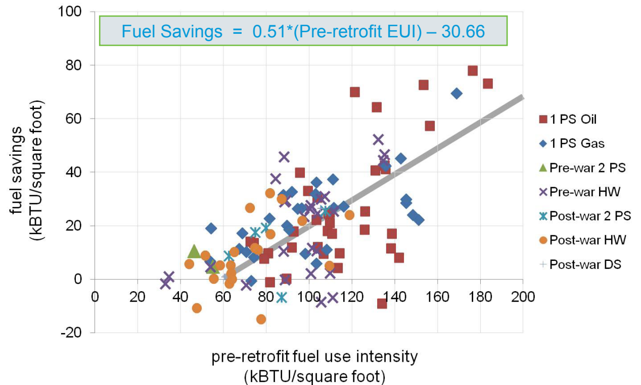
Figure 12: Relationship Between Buildings' Actual Post-retrofit Savings and Pre-retrofit Fuel Consumption
