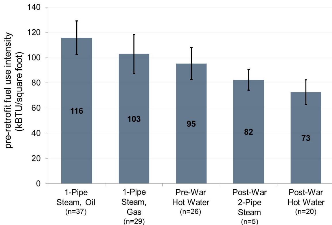
Figure 13: Pre-retrofit Fuel Use Intensity by Comparative Group
