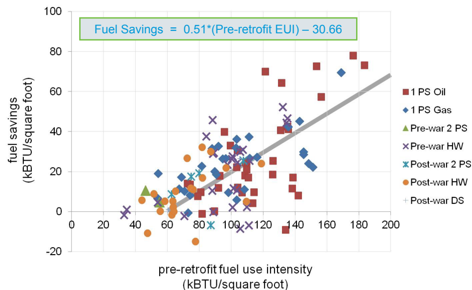
Relationship Between Buildings' Actual Post-retrofit Savings and Pre-retrofit Fuel Consumption Actual Fuel Savings vs. Projected Fuel Savings
