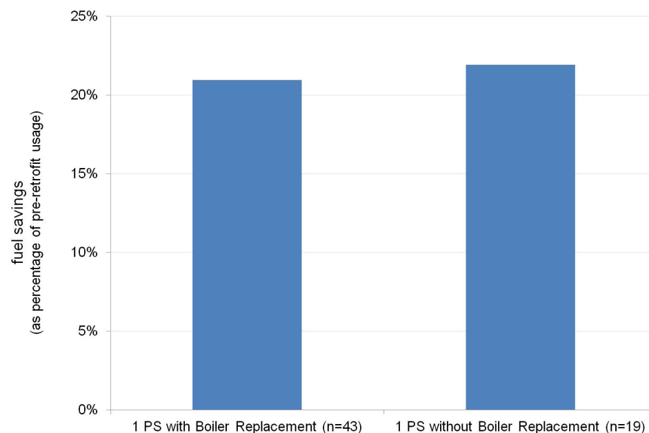
Figure 25: Fuel Savings for One-pipe Steam Buildings With and Without Boiler Replacements
