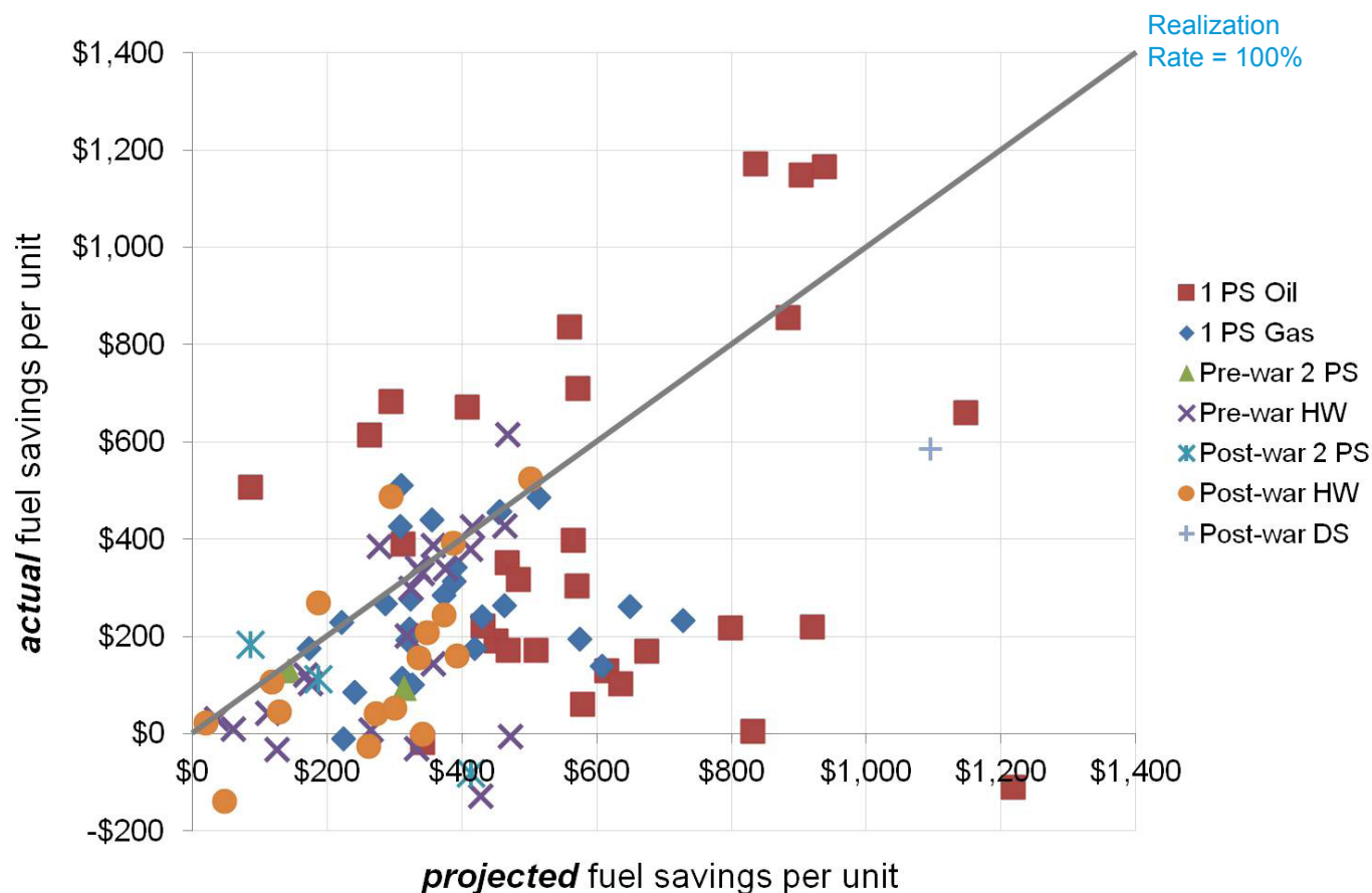
Figure 14: Actual Fuel Savings vs. Projected Fuel Savings, per Unit
