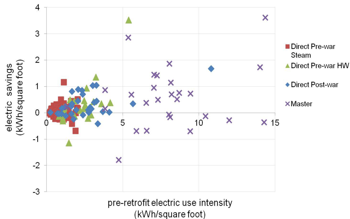
Figure 10: Electric Savings by Comparative Group vs. Pre-retrofit Electric Use Intensity
