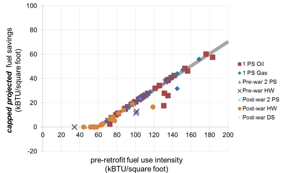
Figure 19: Projections Greater Than the Threshold Are Adjusted Down to the Trend Line, Based On Pre-retrofit Fuel Use Intensity
