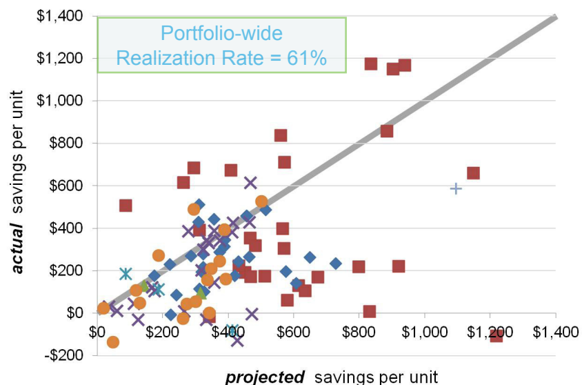
Figure 14: Projected Fuel Savings vs. Actual Fuel Savings, per Unit
