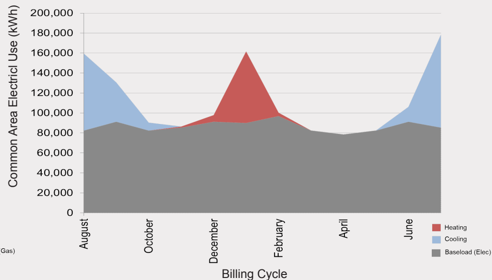
Figure 6: Electric Billing Cycle, Common Area Electric Use
