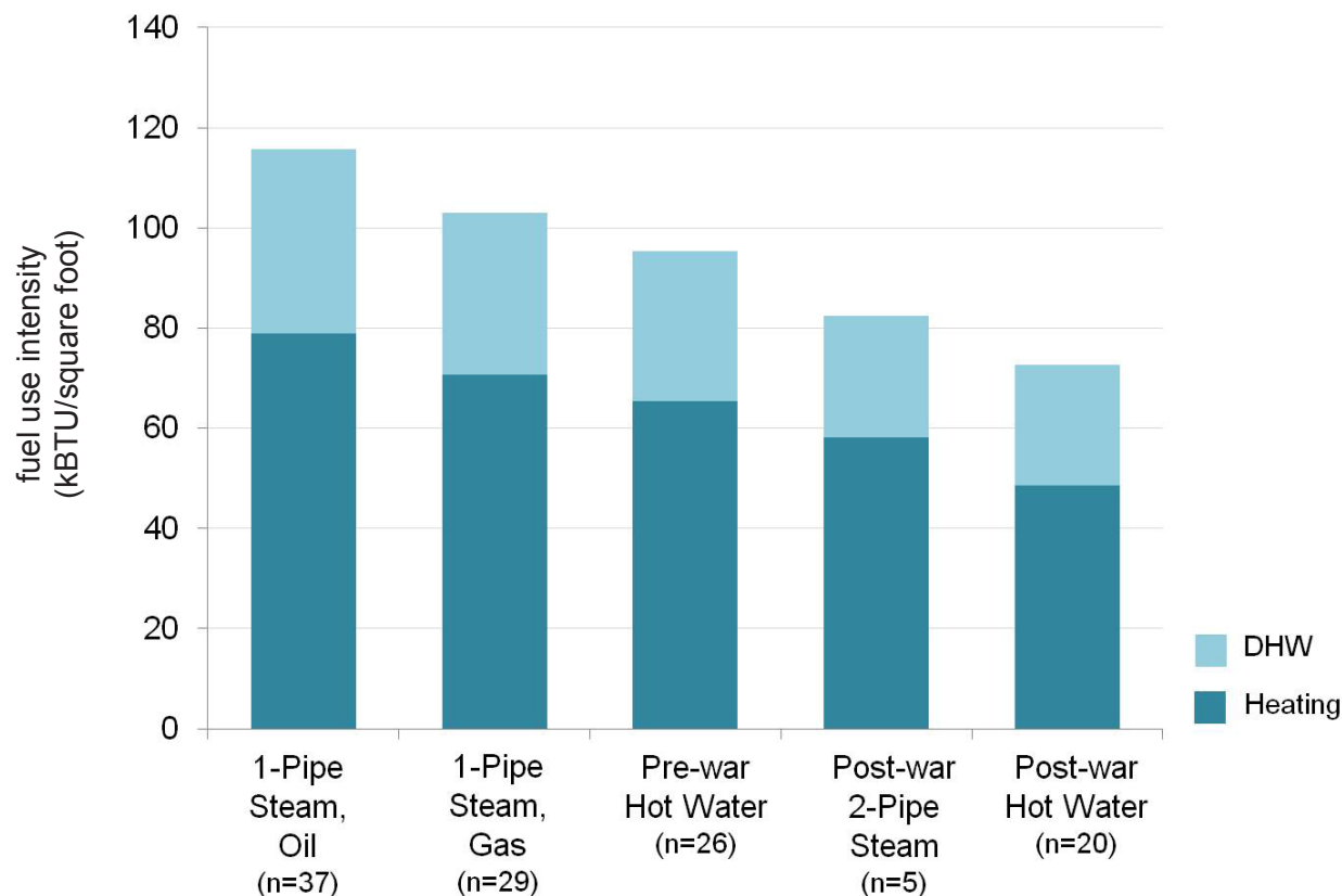
Figure 9: Fuel Use Intensity by Comparative Group, Domestic Hot Water vs. Heating
