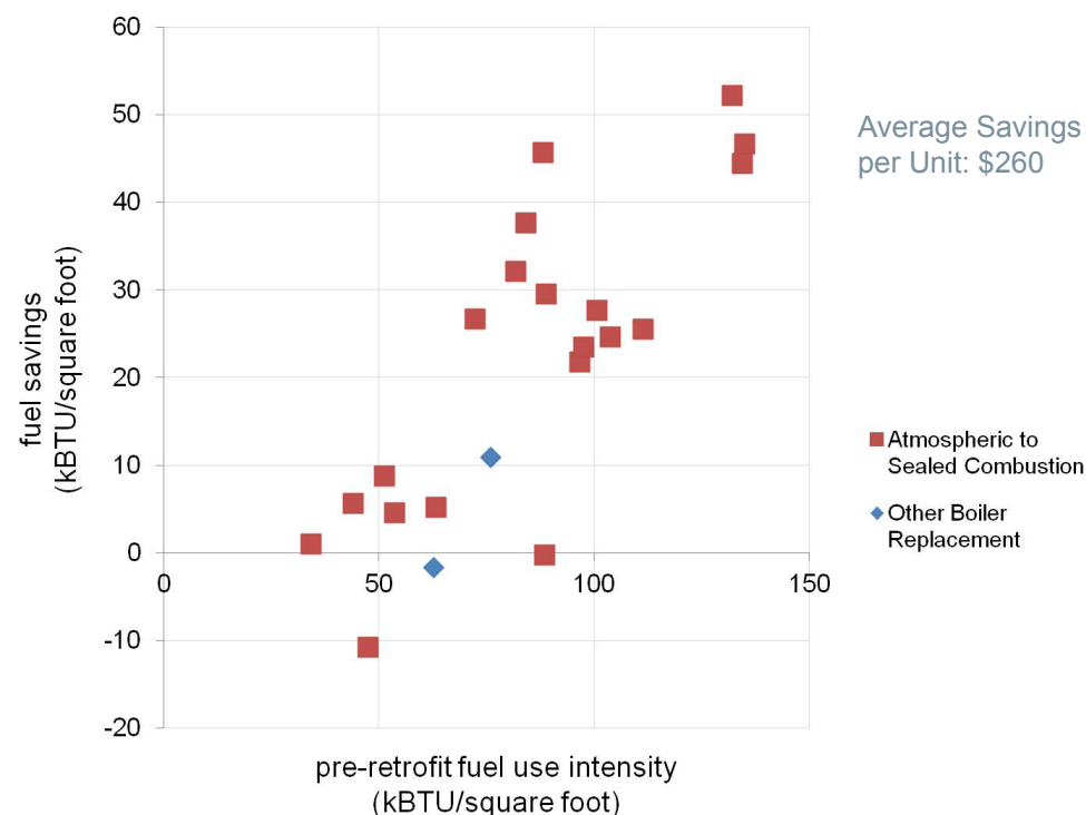
Figure 22: Fuel Savings vs. Pre-retrofit Fuel Use Intensity, Atmospheric Boiler to Sealed Combustion Unit
