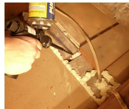
Combination of air sealing and blown-in insulation
