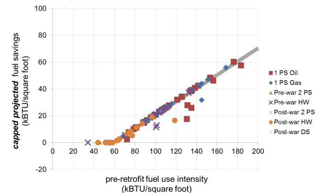
Figure 18: Capped Projected Fuel Savings vs. Pre-Retrofit Fuel Use Intensity
