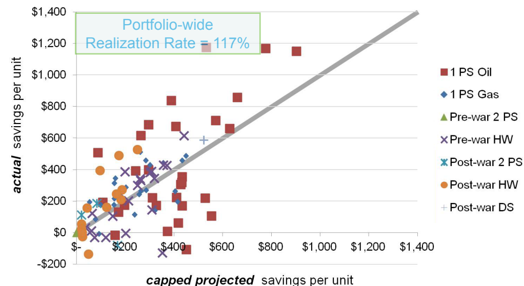
Figure 20: Capped Projected Fuel Savings Increase Portfolio Realization Rate Capped Projected Savings vs. Actual Savings, per Unit
