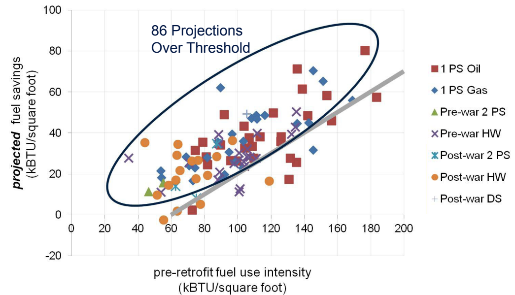
Figure 18: Buildings' Projected Fuel Savings are Compared to the Threshold, Based On Their Pre-retrofit Fuel Use Intensity
