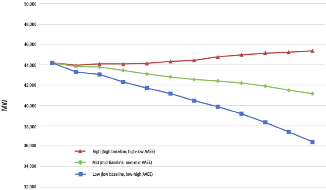
Figure 47: Adjusted Demand Cases for Peak, Combined IOU Service Territories
