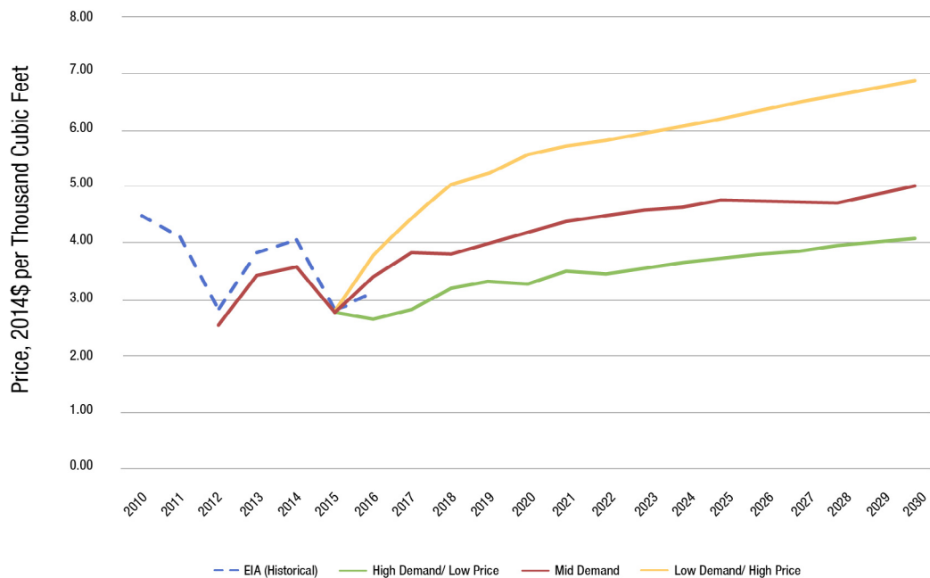
Figure 47: Adjusted Demand Cases for Peak, Combined IOU Service Territories
