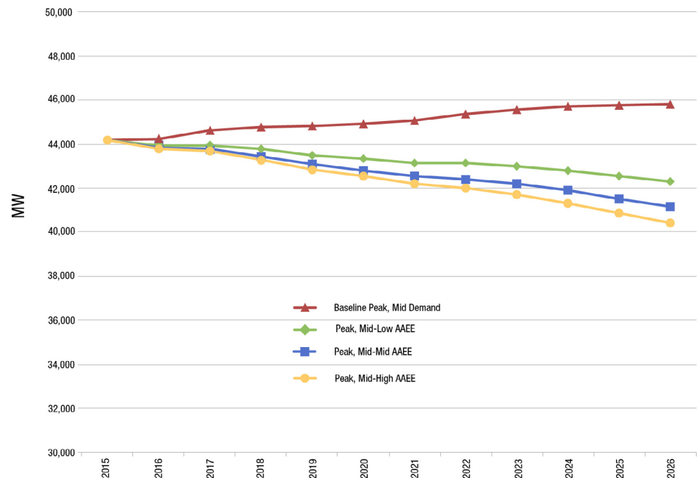
Figure 45: Mid Baseline Demand and Adjusted Peaks, Combined IOU Service Territories
