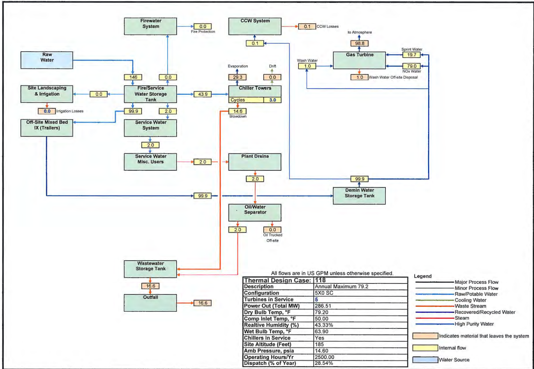
PROJECT DESCRIPTION - FIGURE 11 Mission Rock Energy Center - Water Balance - Annual Maximum
