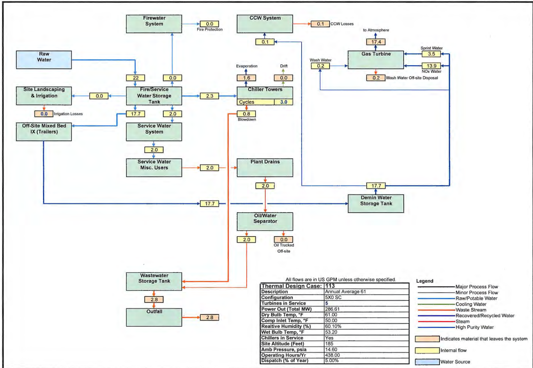
PROJECT DESCRIPTION - FIGURE 10 Mission Rock Energy Center - Water Balance - Annual Average
