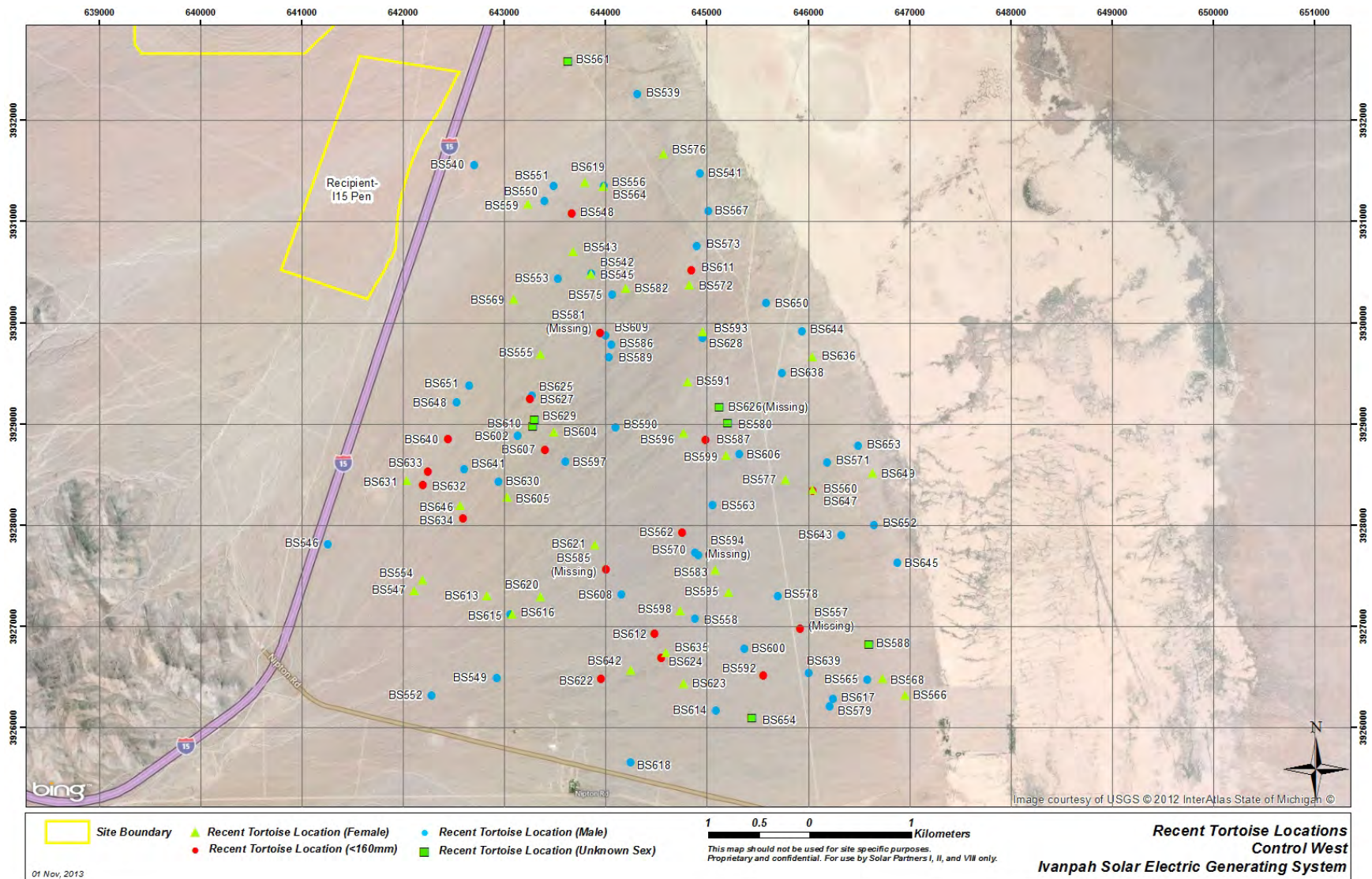
Figure 10. ISEGS Current Tortoise Locations - West Control Site.
