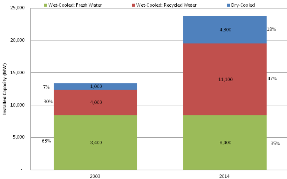
Figure 13: Cooling Process for Operating Power Plants That Have a Steam Cycle Operating Power Plants with Steam Cycle
