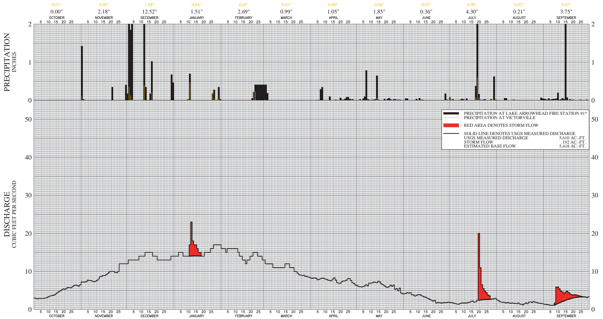
DISCHARGE OF MOJAVE RIVER AT LOWER NARROWS, PRECIPITATION AT LAKE ARROWHEAD FIRE STATION #1, AND PRECIPITATION AT VICTORVILLE WATER YEAR 2014-15
