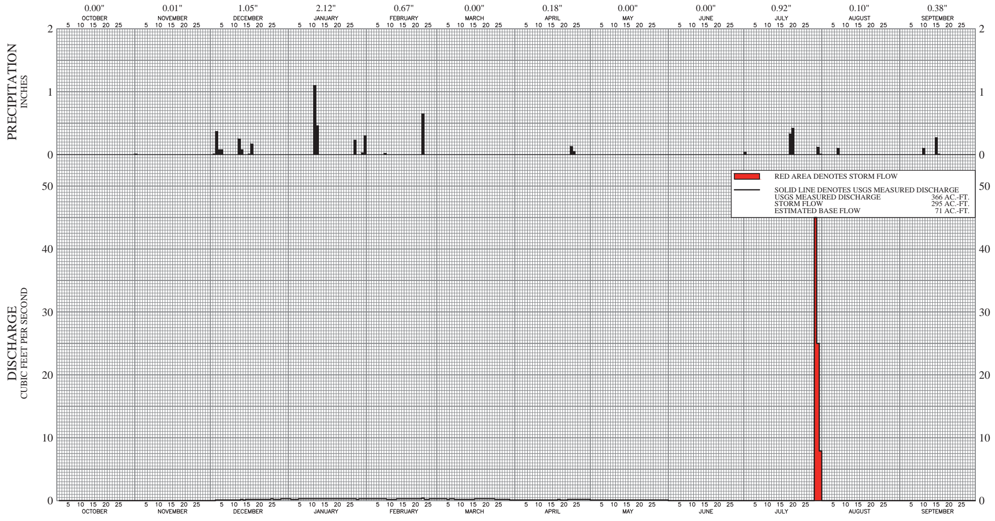
DISCHARGE OF MOJAVE RIVER AT AFTON AND PRECIPITATION AT BARSTOW WATER YEAR 2014-15
