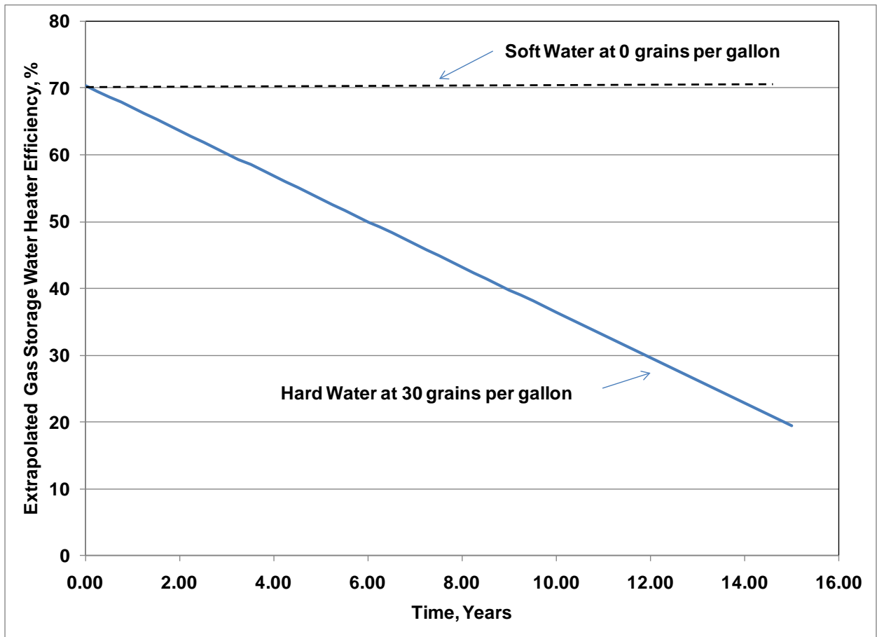
Figure 5-12. Predicted efficiency of a gas storage water heaters operating on soft water (0 grains per gallon) versus one operating on unsoftened water with a hardness of 30 grains per gallon.
