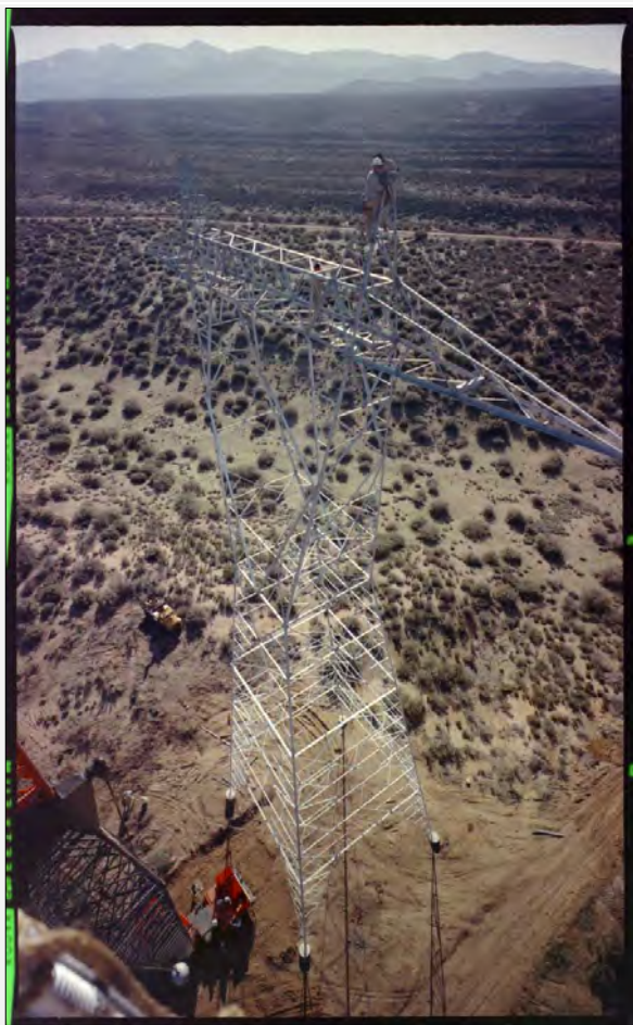
Exhibit 1. Lugo-Vincent 500kV towers under construction, 1968
