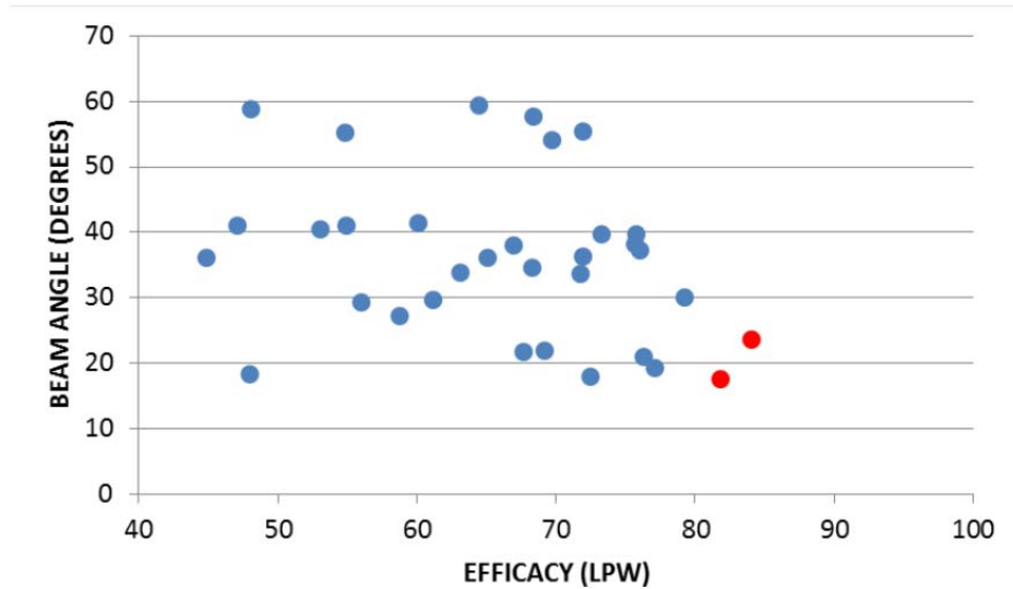
Figure 1: Beam Angele Vs Efficacy
