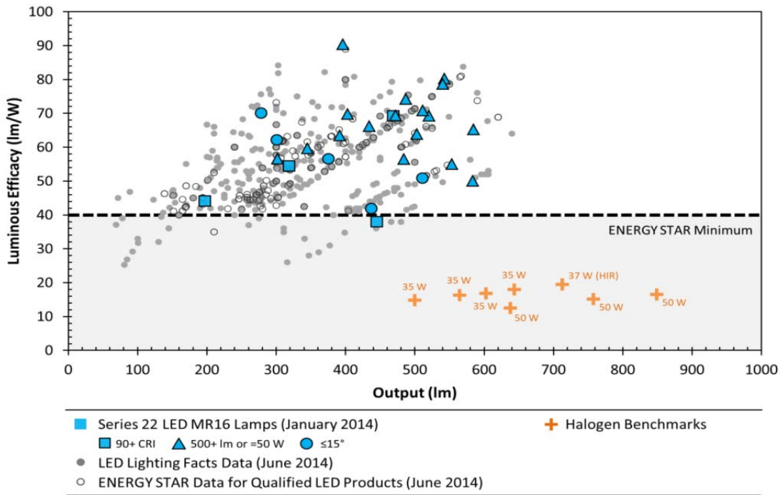
Figure 7: Luminous Efficacy vs. Lumen Output
