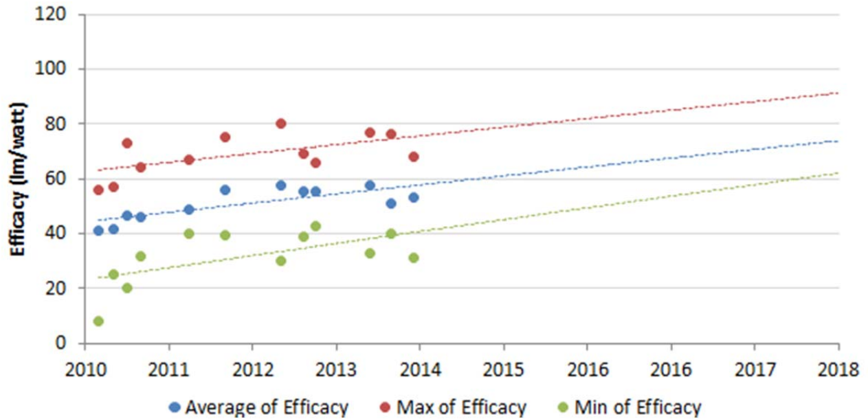
Figure 8: Efficacy over Time
