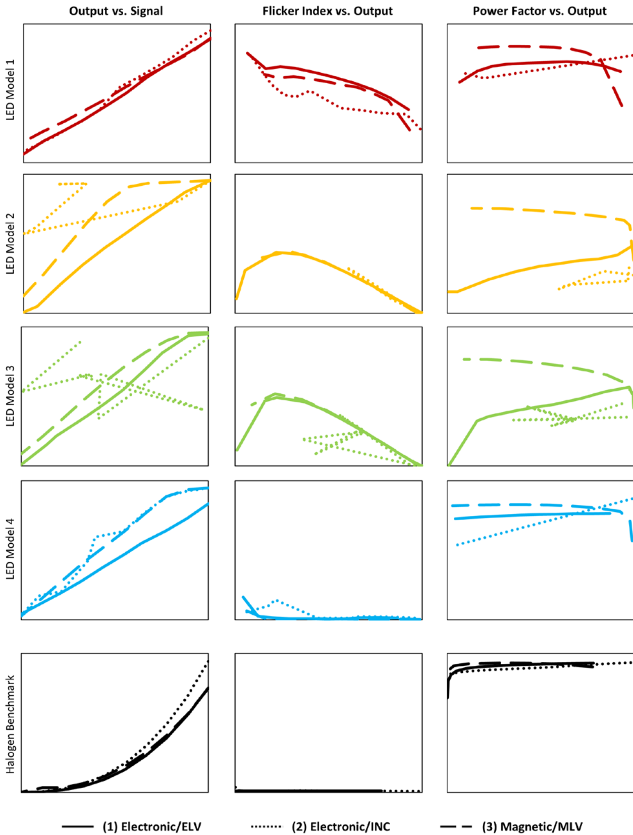
Figure 14. Graphical representation of performance for four LED MR16s lamps and one halogen benchmark lamp, scenarios one through three. Each lamp model is identified by a color, but the line colors do not correspond to the other charts in this report. For some of the LED lamps, the change in performance due to operation with different transformer-and-dimmer combinations was minimal, but for others it was substantial.
