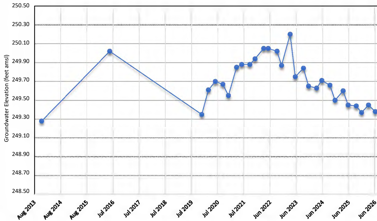
Chart 11 6S/22E-19N2S Well Hydrograph
