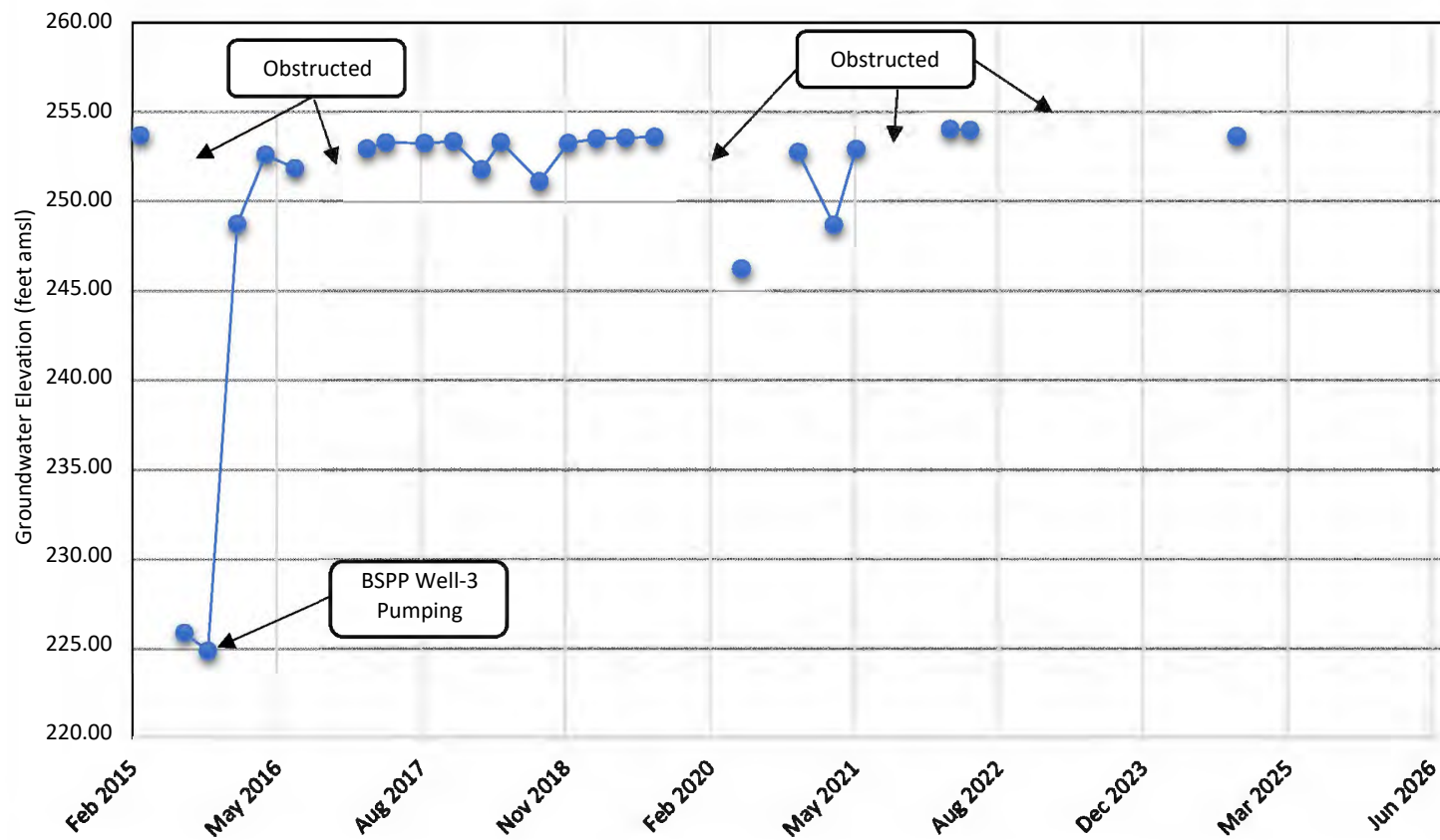
Chart 3 BSPP Well-3 Hydrograph
