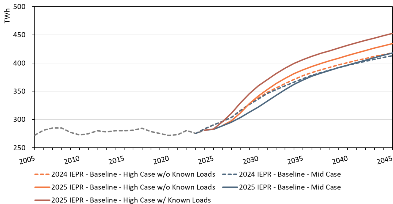
Figure 18: Statewide Baseline Electricity Consumption
