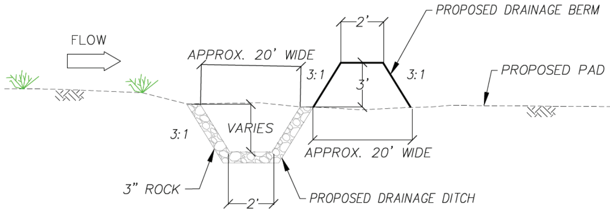
Figure 2 | Typical Berm and Swale Section
