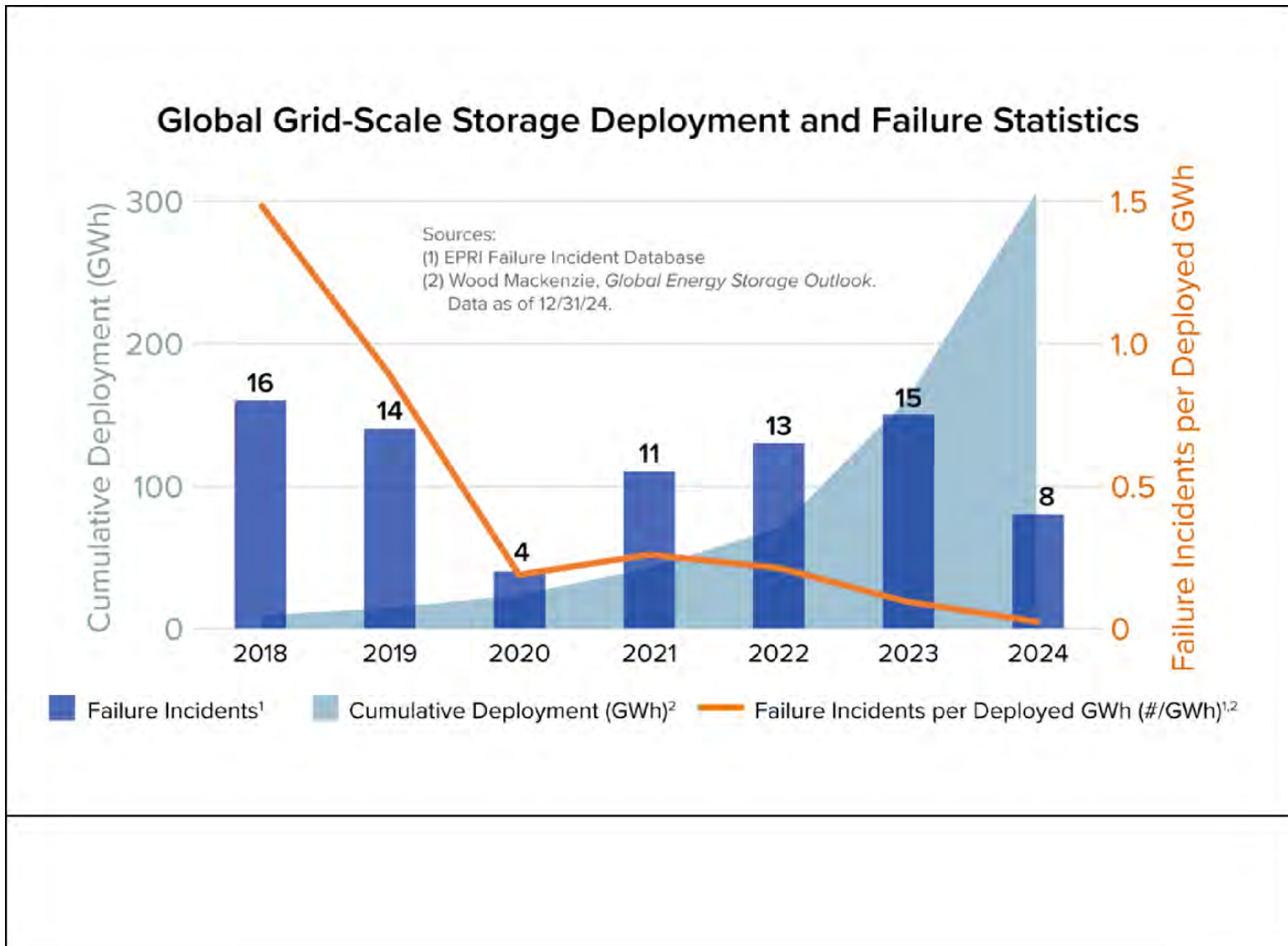
Figure 4.4-2 Global Grid-Scale Deployment and Failure Statistics
