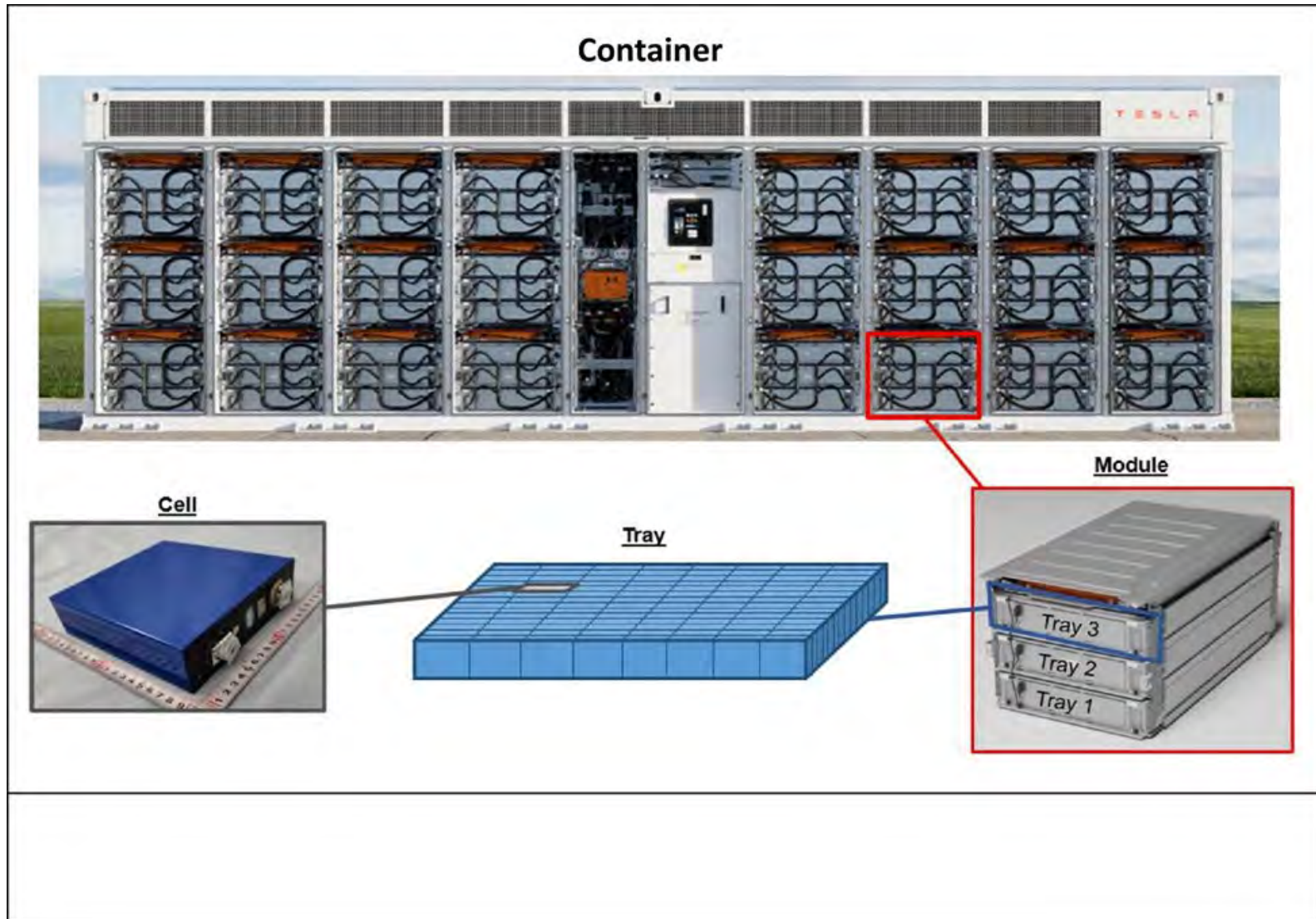
Figure 4.4-1 Cells and Battery Modules
