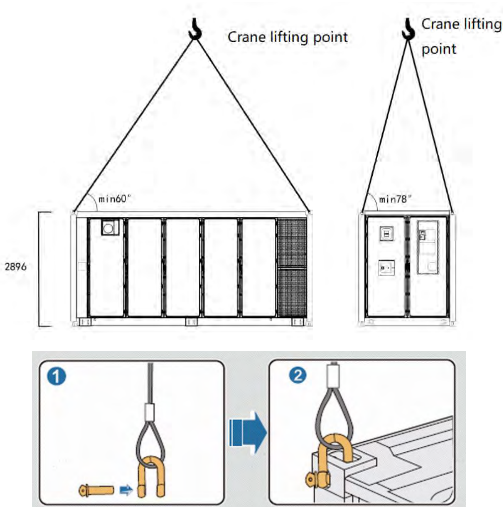
Figure 6-3: Crane lifting
