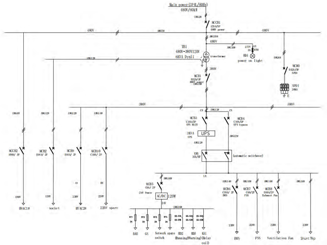
Figure 8-7: Auxiliary connection (for reference only)
