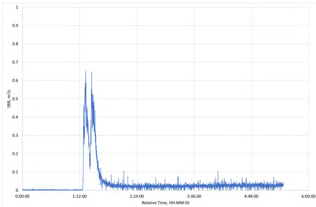
Figure 19. Smoke release rate versus time.
