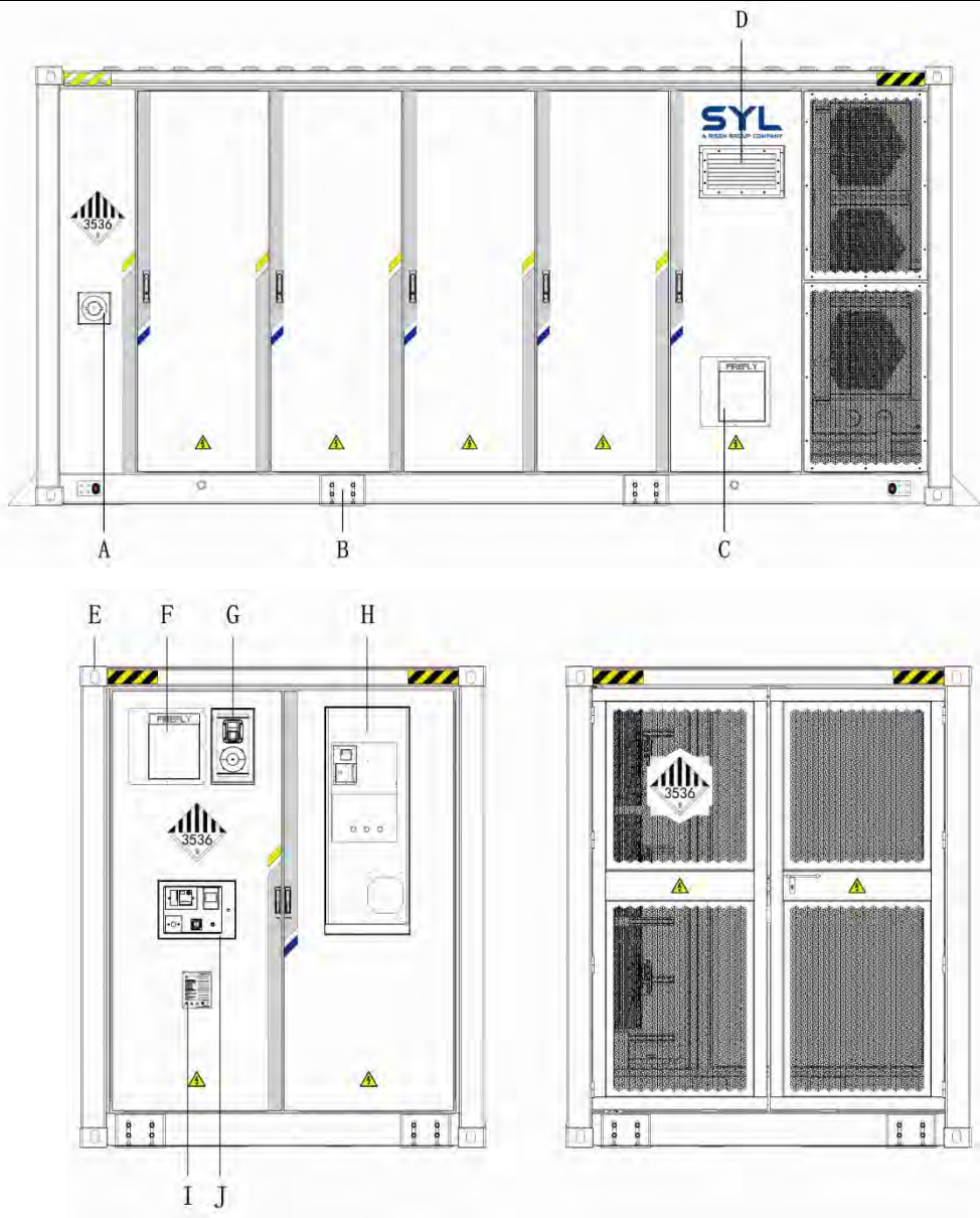
Figure 4-1: Appearance
