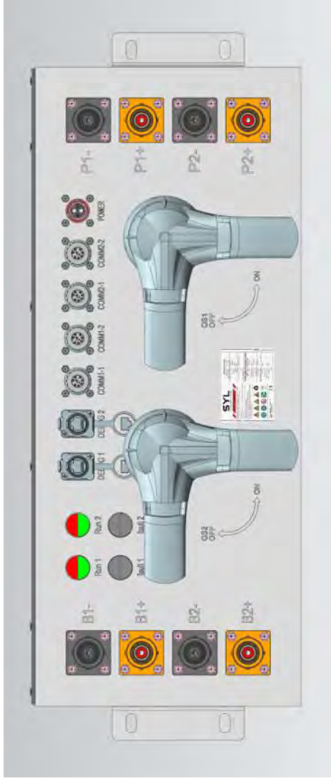
Figure 7-5: DC switchgear interface
