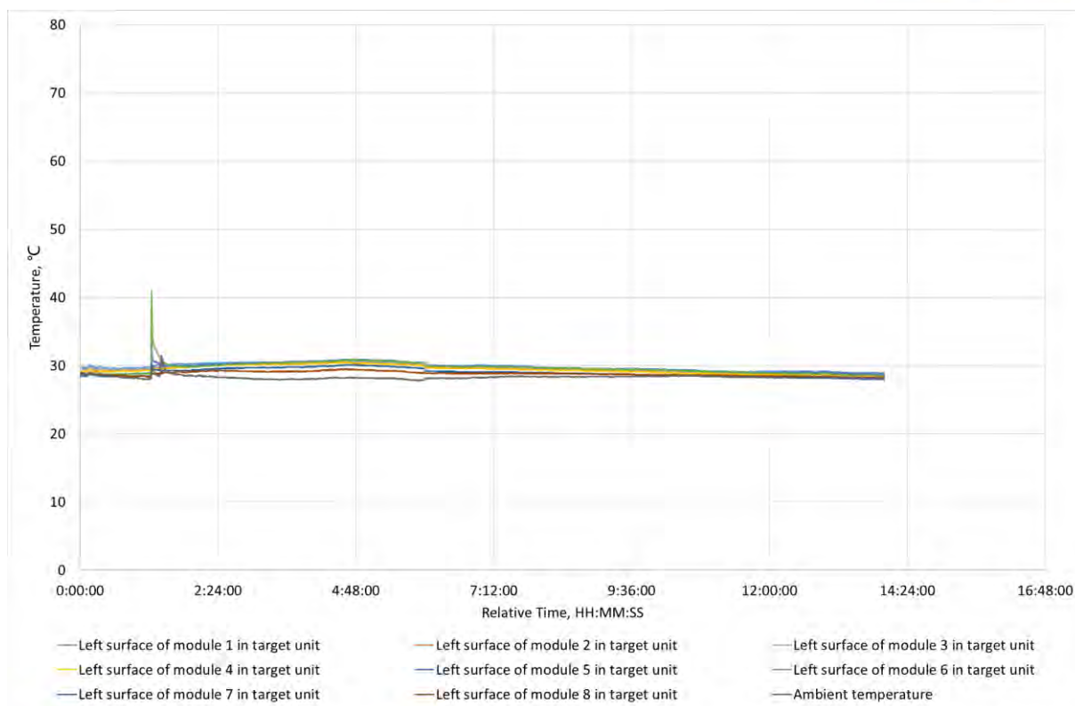
Figure 33. Temperature measurements in target BESS units
