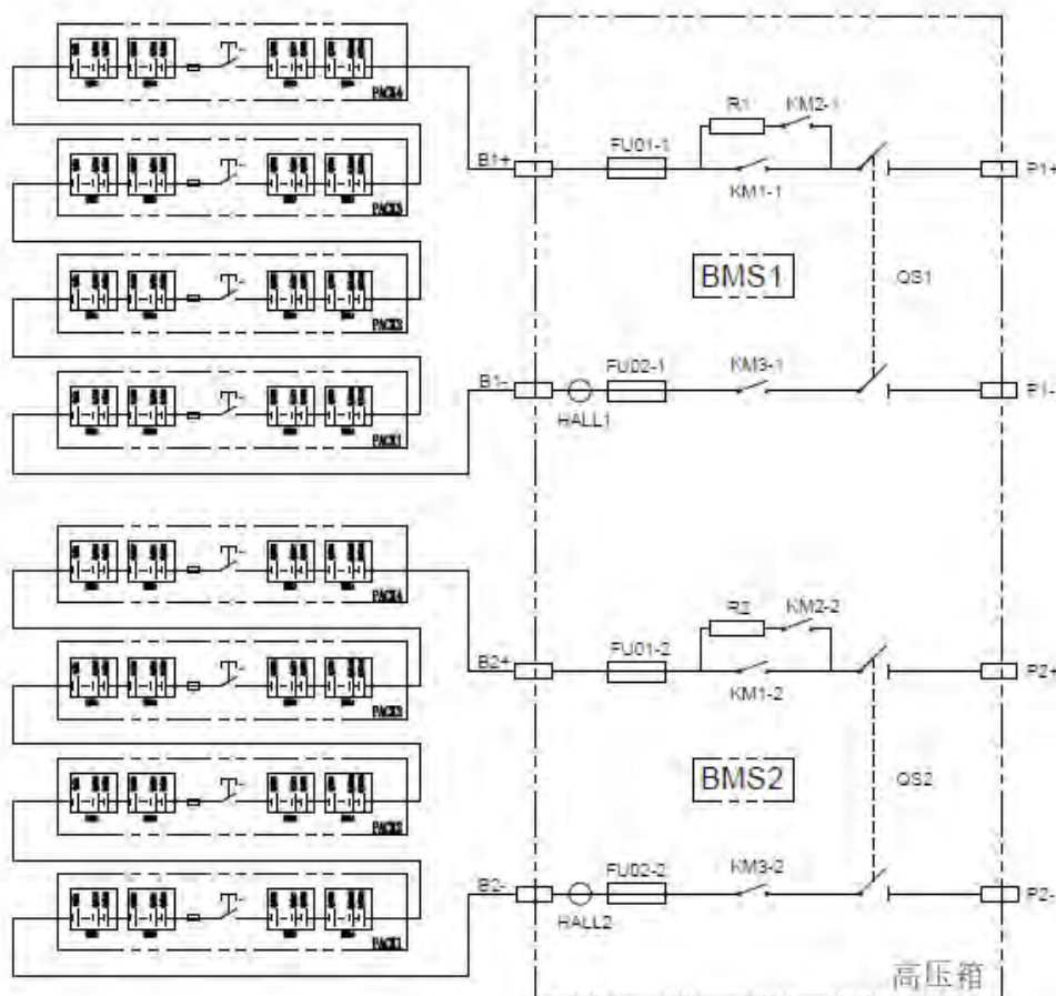
Figure 10. Electrical configuration of battery system
