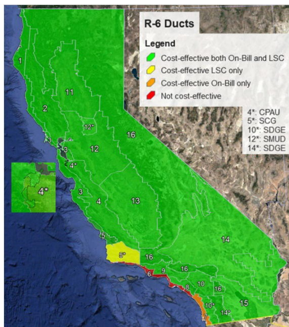
Figure 10: R-6 Ducts
