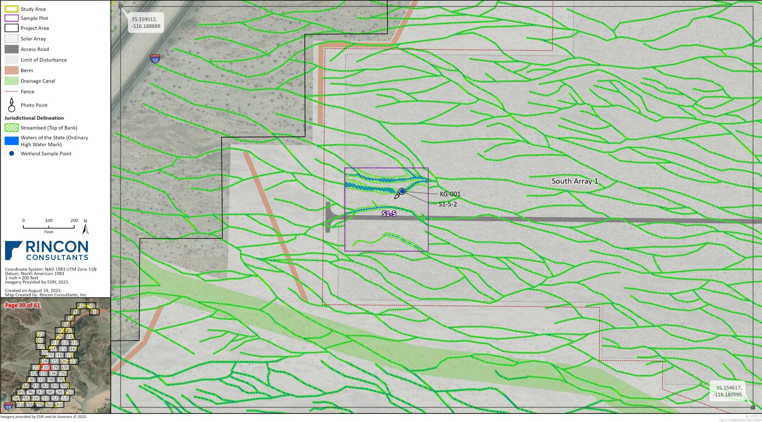
Figure 10 Potential Jurisdictional Aquatic Resources within the Study Area (Page 30)
