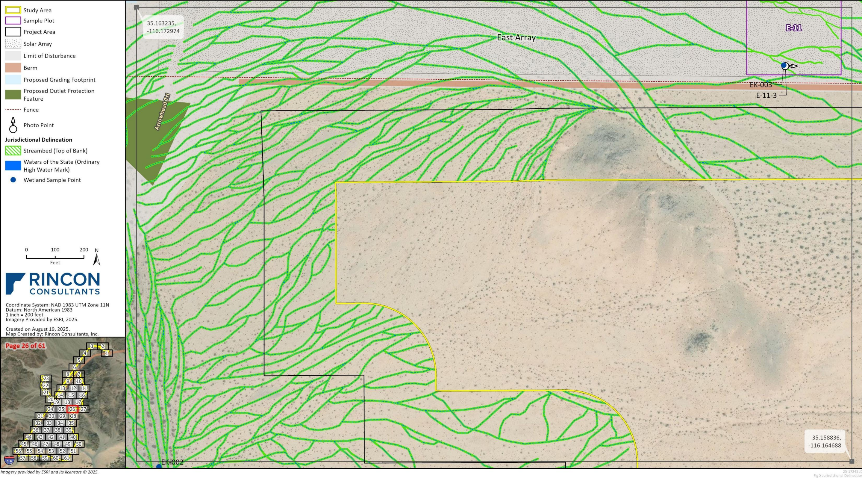
Figure 10 Potential Jurisdictional Aquatic Resources within the Study Area (Page 26)
