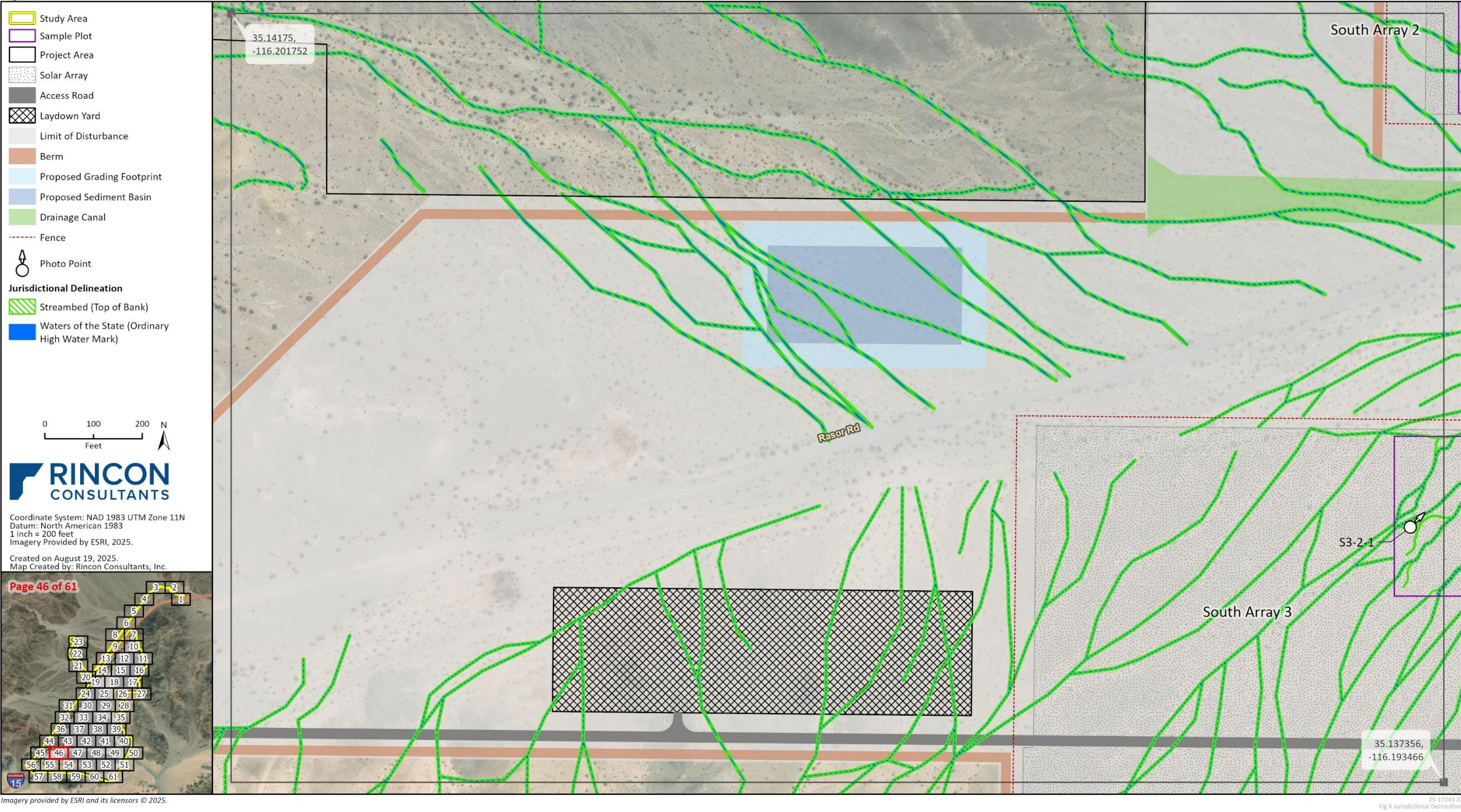
Figure 10 Potential Jurisdictional Aquatic Resources within the Study Area (Page 46)
