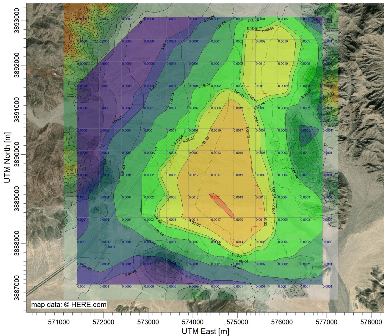
PLOT FILE OF ANNUAL VALUES AVERAGED ACROSS 1 YEARS FOR SOURCE GROUP: ALL Max: 2.1E-03 [ug/m 3 ] at (574405.52, 3889083.87) ug/m 3
