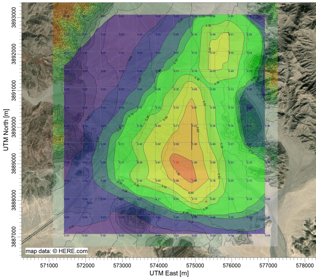
PLOT FILE OF ANNUAL VALUES AVERAGED ACROSS 1 YEARS FOR SOURCE GROUP: ALL Max: 1.09 [ug/m^3] at (574405.52, 3889083.87) ug/m^3
