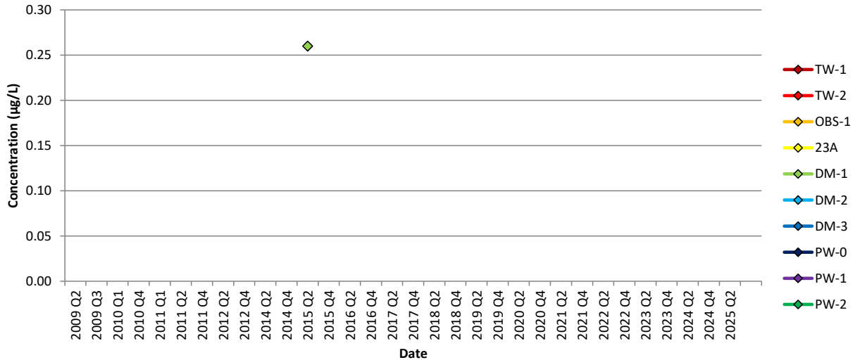
Chart 21: Mercury
