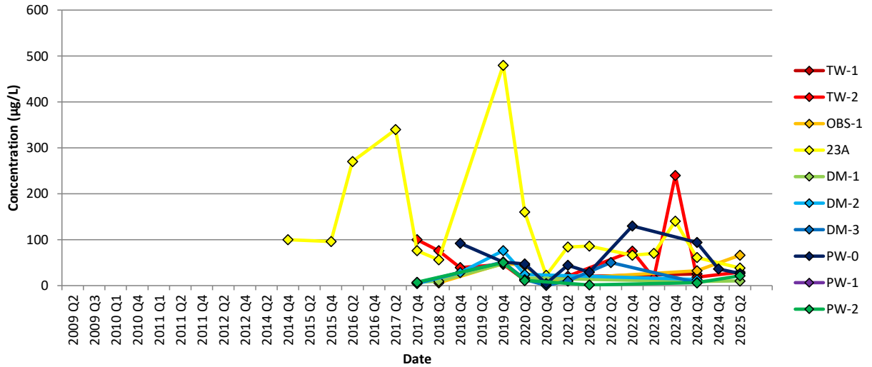
Chart 20: Zinc
