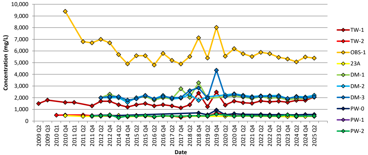
Chart 2: Sulfate (SO 4 )
