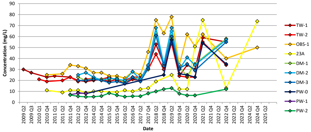
Chart 7: Potassium
