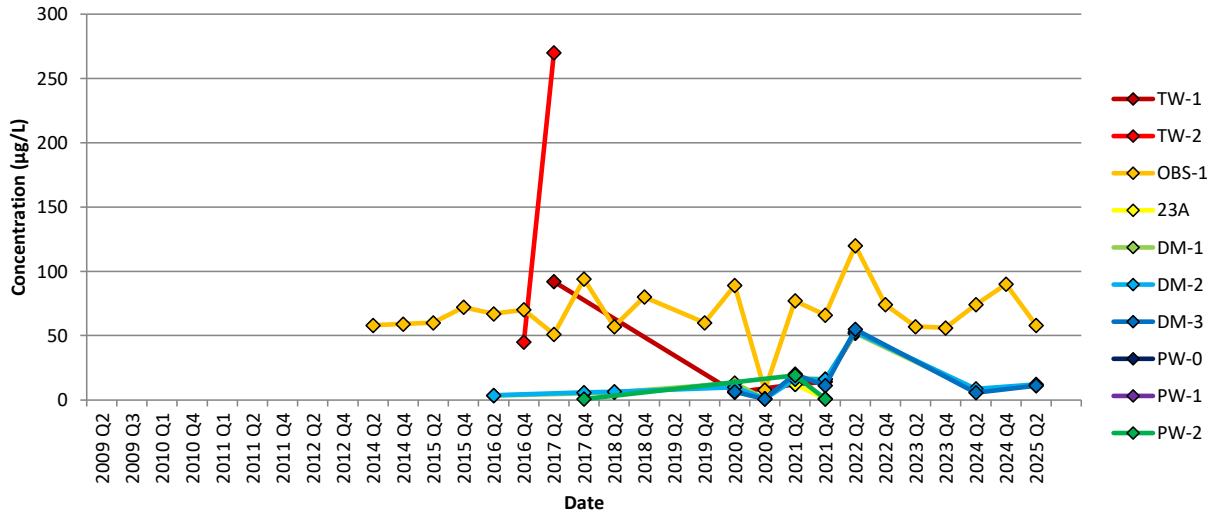
Chart 19: Selenium
