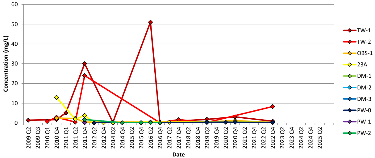
Chart 8: Iron
