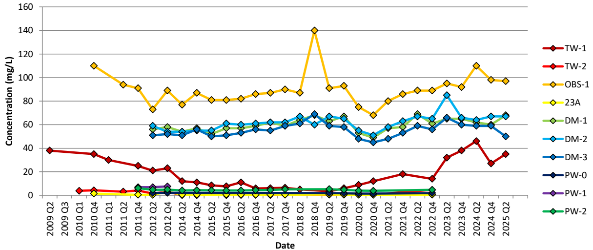
Chart 9: Magnesium
