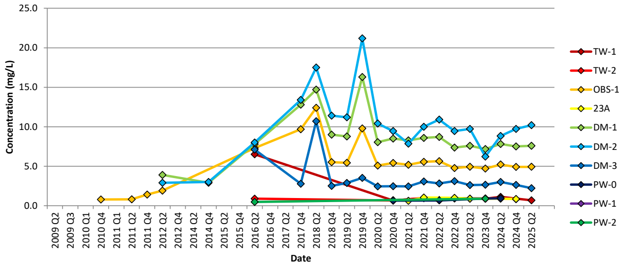
Chart 3: Nitrate (NO 3 )
