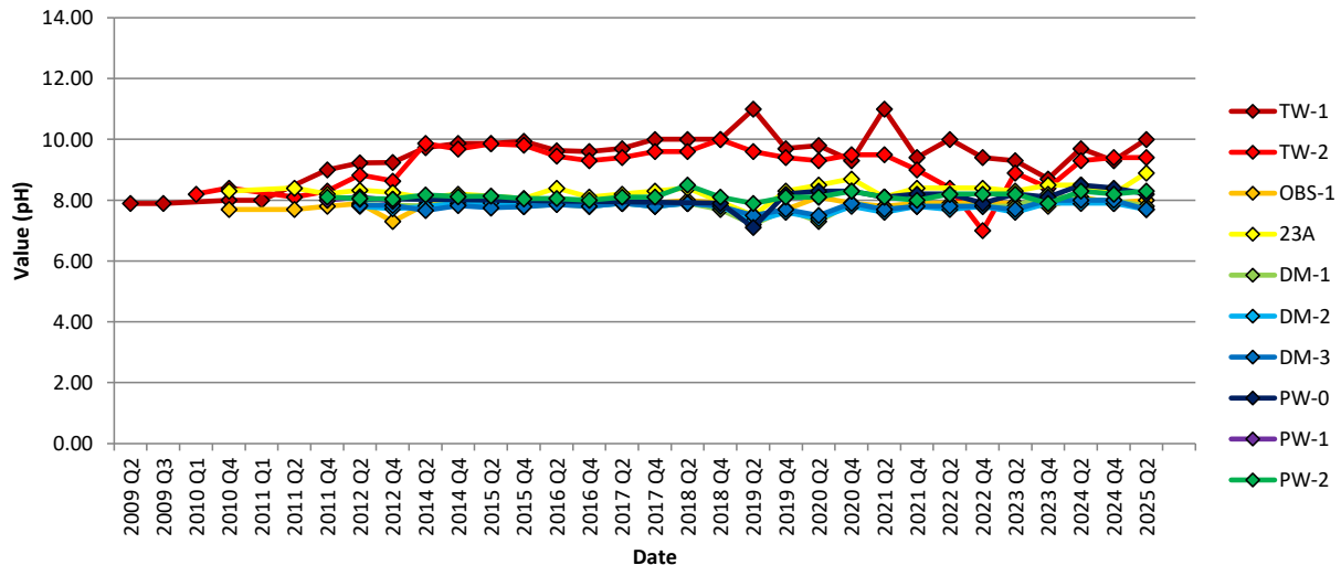
Chart 24: pH
