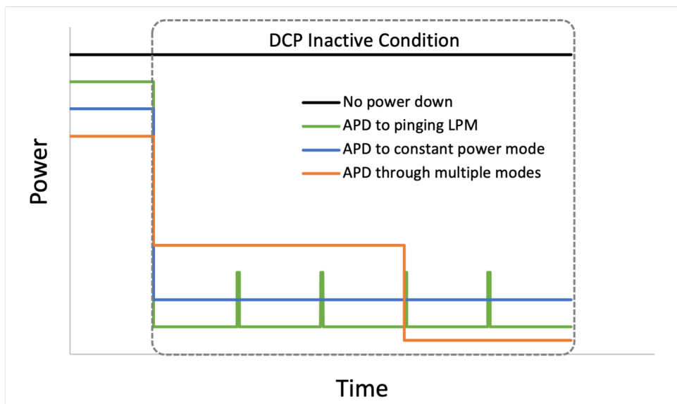
Figure 3: Illustrative examples of power behavior that might be encountered during testing. The dashed box indicates the DCP inactive condition power draw in each of the following scenarios:
