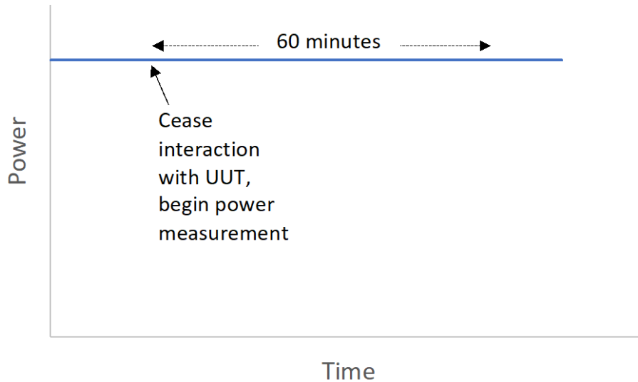
Figure 7: Example of power as a function of time if the UUT does not exhibit APD. The power measurement begins when the tester ceases interaction with the UUT. Average power is calculated by averaging power for 60 minutes after the tester has ceased interaction with the UUT.
