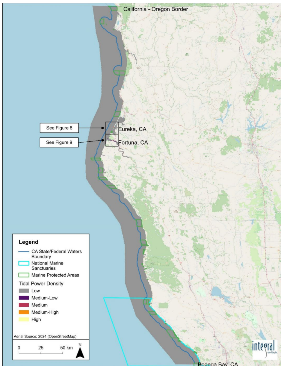
Figure 7: Annual-Averaged Tidal Power Density: Northern California Coastline
