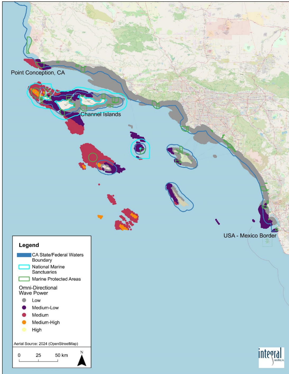
Figure 11: Annual-Averaged, Omnidirectional Wave Power: Southern California Coastline
