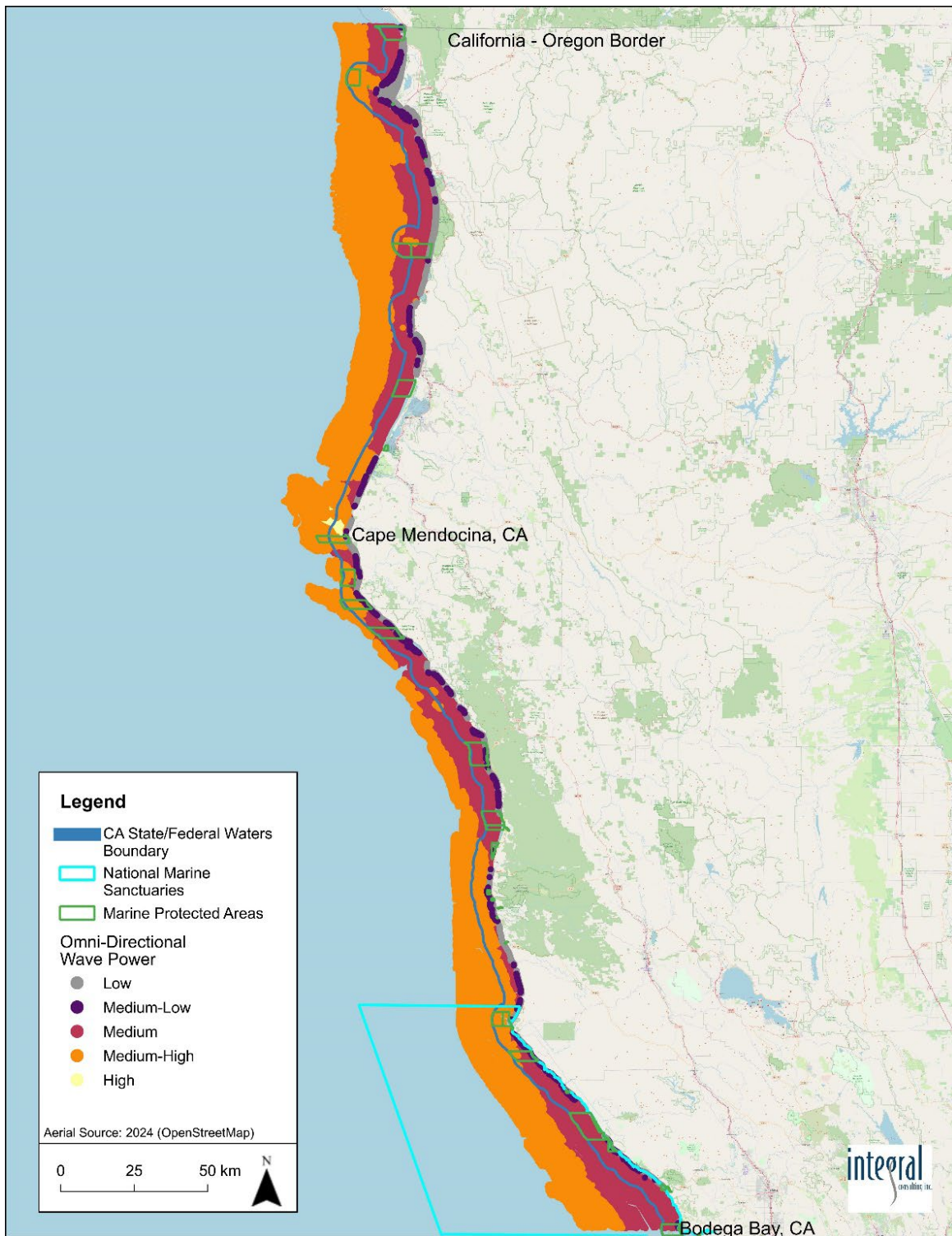
Figure 17: Annual-Averaged, Omnidirectional Wave Power: Northern California Coastline
