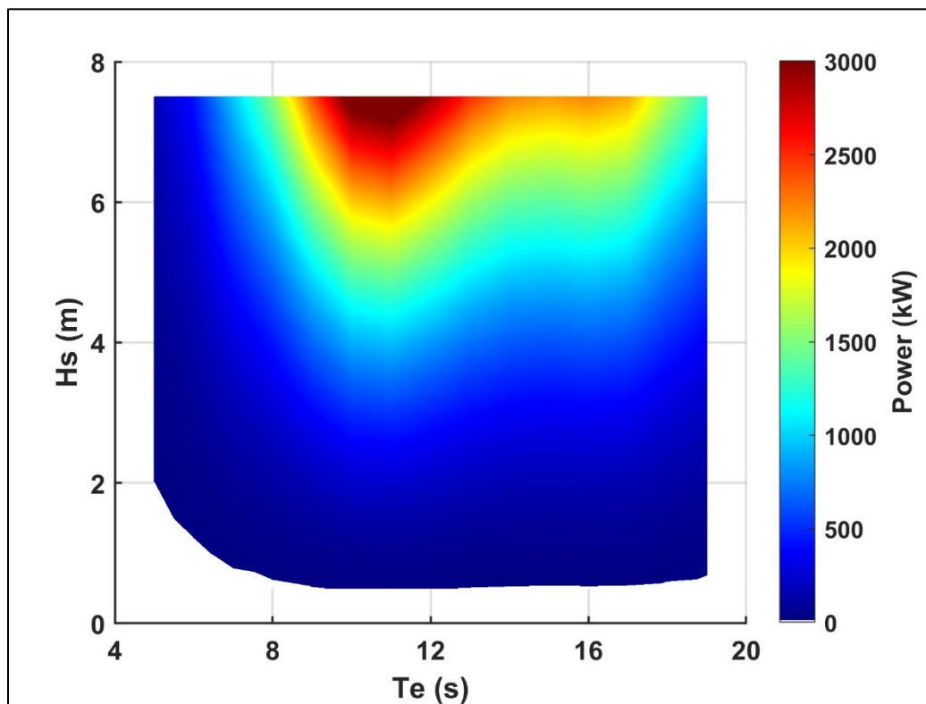
Figure 2: Mechanical Power Matrix Illustrating Device Power Output in kW for a Range of Significant Wave Heights ( H_s ) and Wave Energy Periods ( T_e ) for a Hypothetical Model Wave Energy Converter
