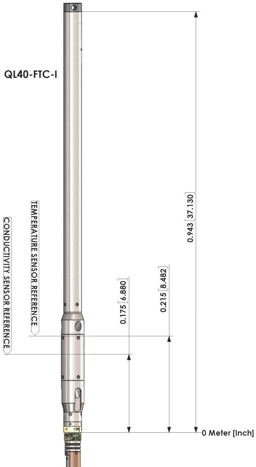
Figure 2: Concept illustration of FTC probe
