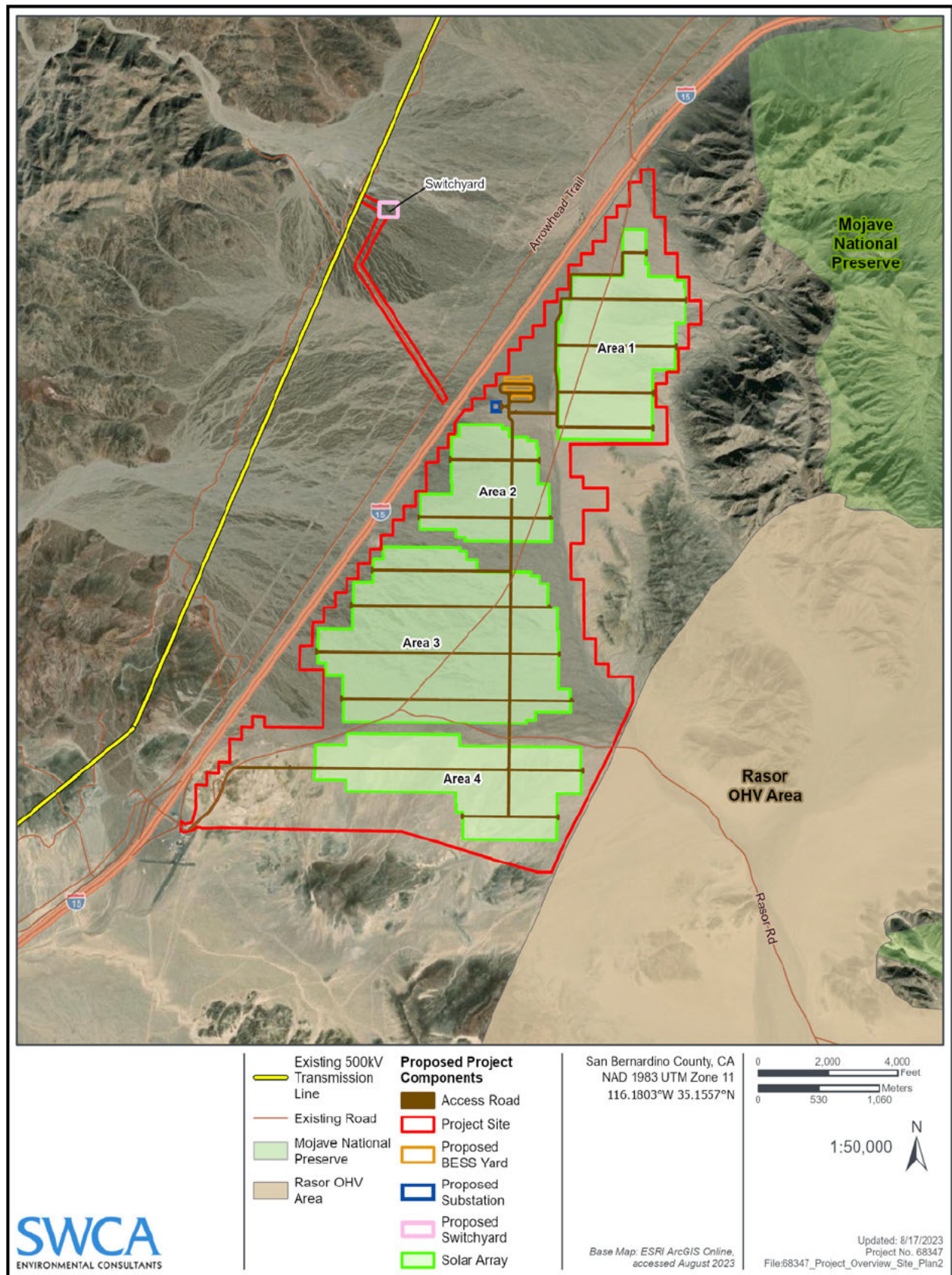
Figure 2. Site plan.
