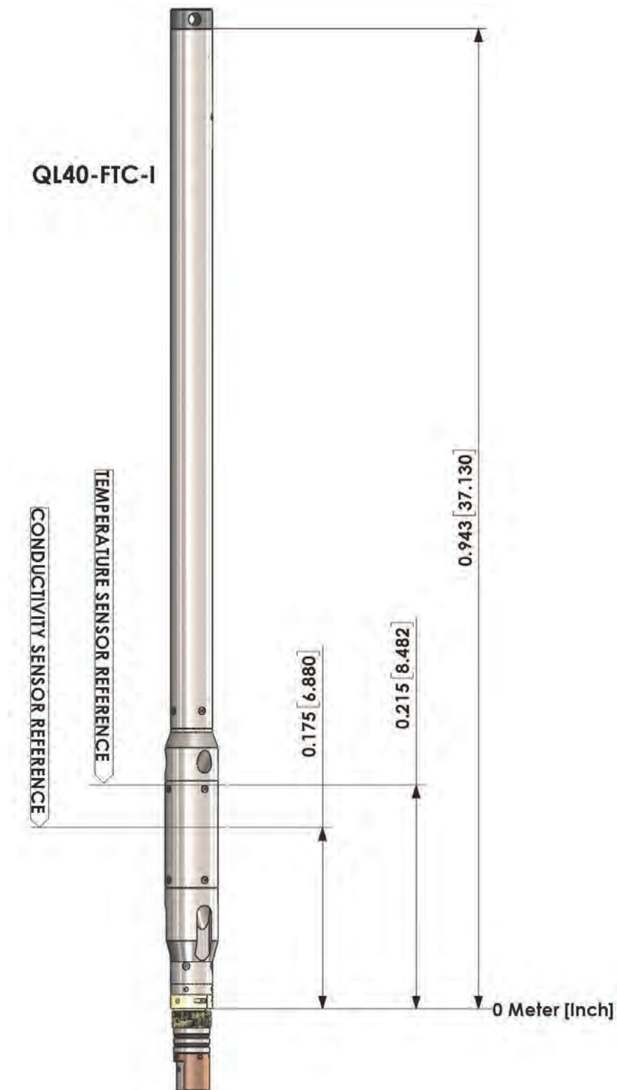
Figure 2: Concept illustration of FTC probe
