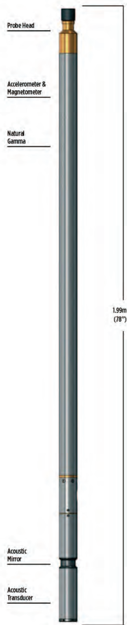
Figure 1: Concept illustration of televIEWER probe
