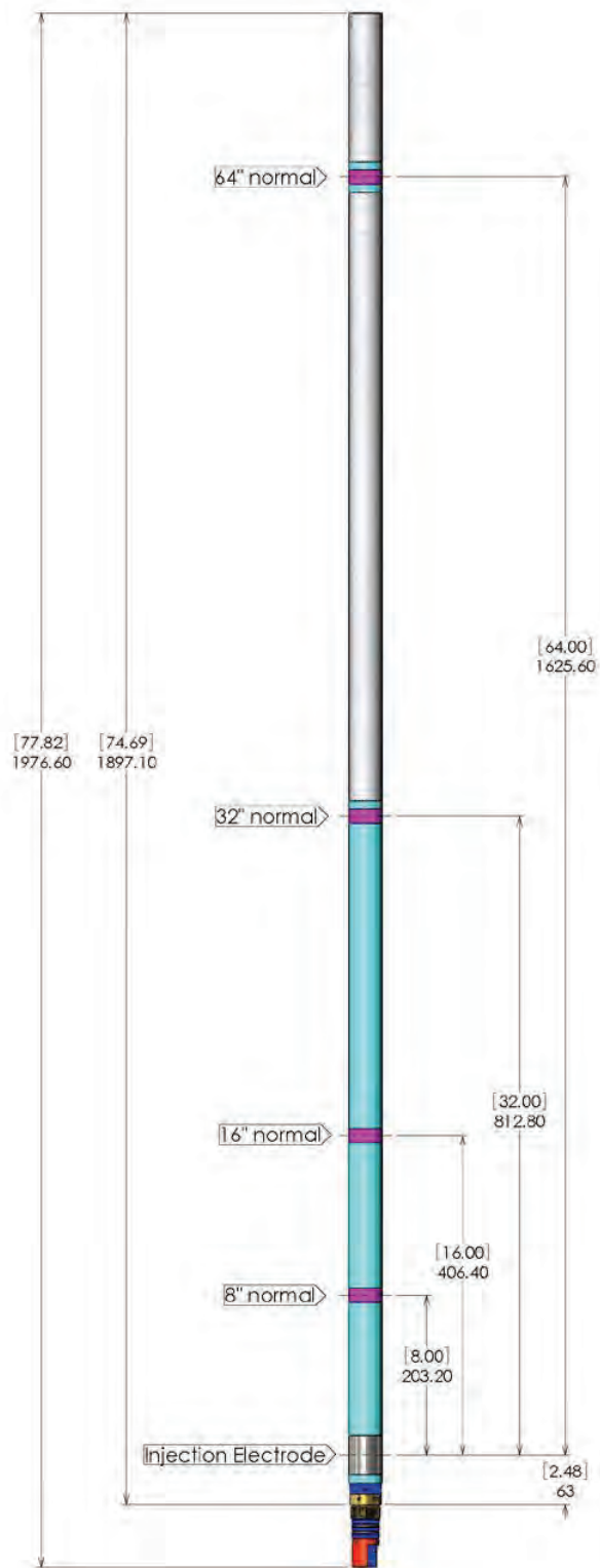
Figure 3: Concept illustration of Elog probe
