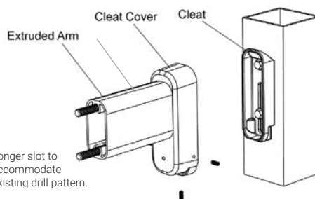
RETROFIT QUICK MOUNT BRACKET (RQMB)
