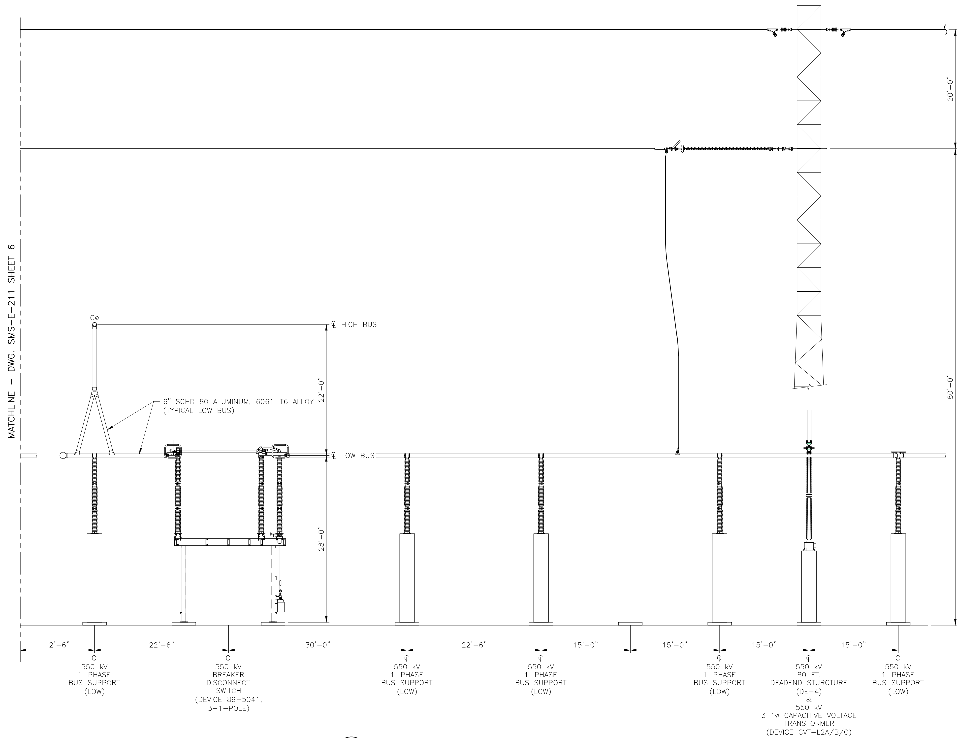
C-C ELEVATION - 500 kV SWITCH AND BUS-BAY 2 PARTIAL SCALE: 1/8" = 1'-0"
