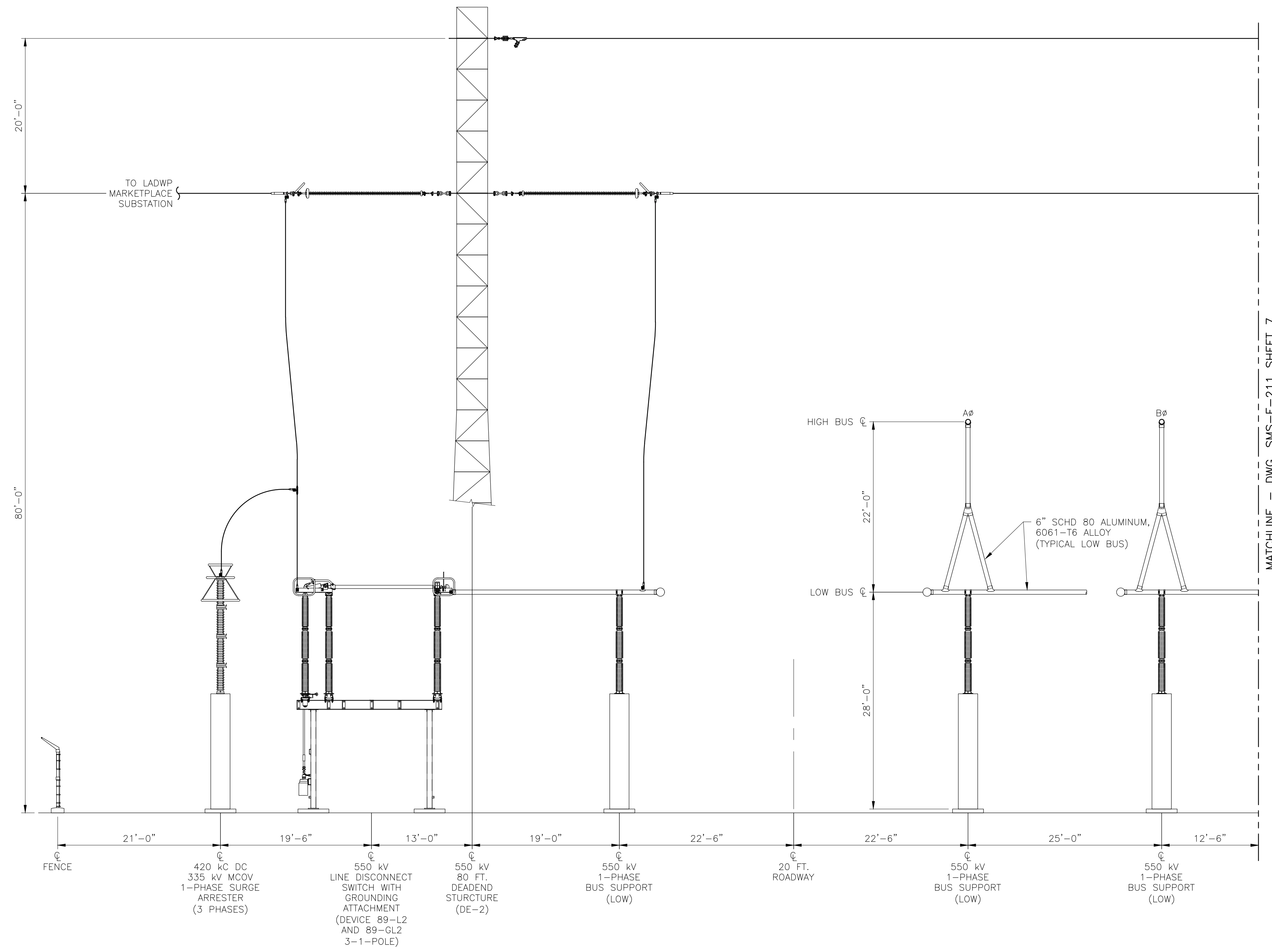
C-C ELEVATION - 500 kV SWITCH AND BUS-BAY 2 PARTIAL SCALE: 1/8" = 1'-0"
