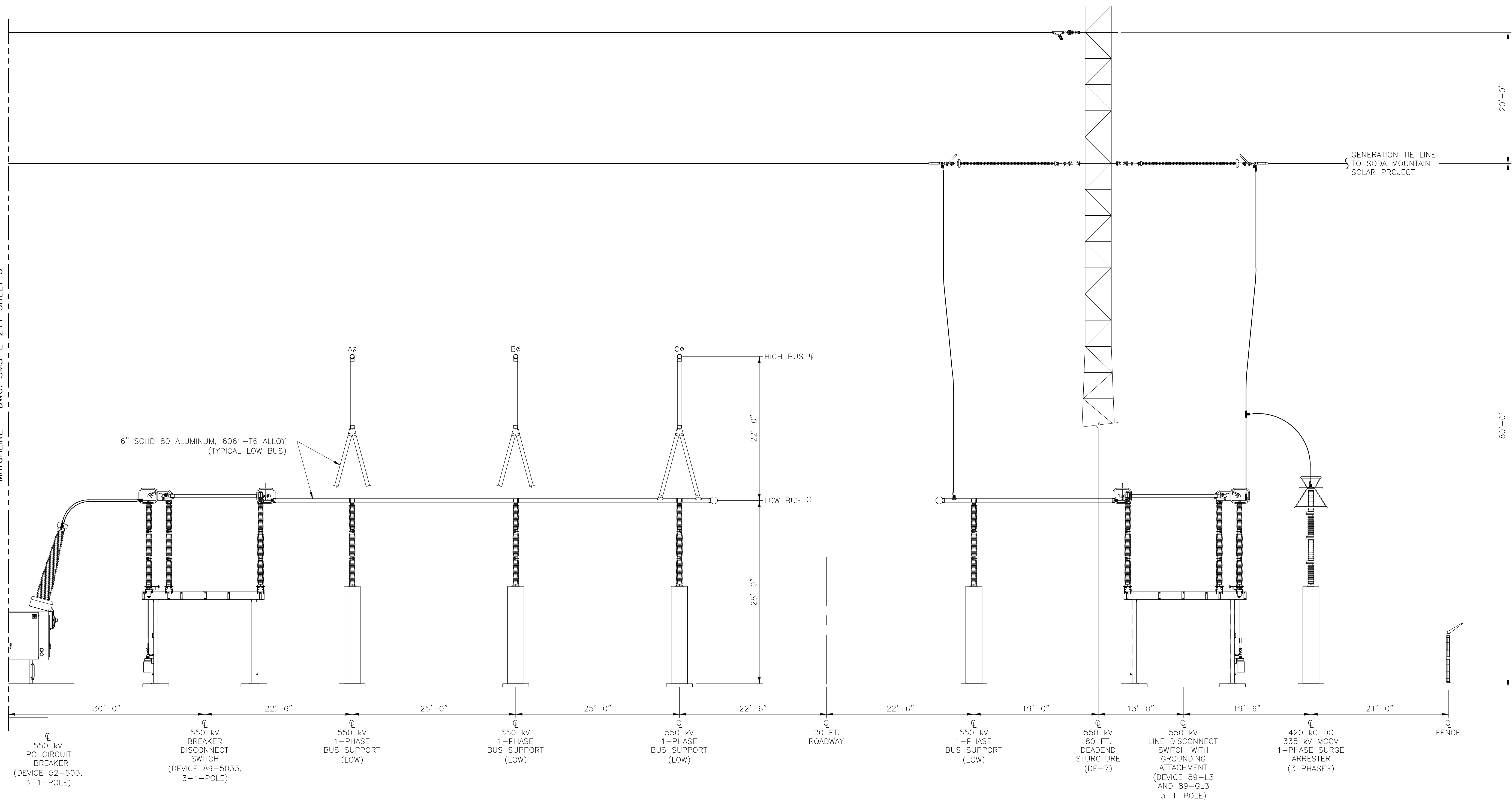
A-A ELEVATION - 500 kV SWITCH AND BUS-BAY 1 SCALE: 1/8" = 1'-0"
